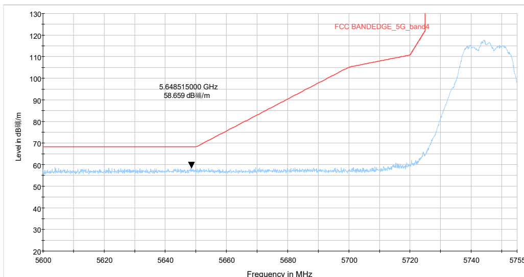
5.6-5.755GHz_5G WIFI_a CH149 6M_Y_TP19_MIMO
