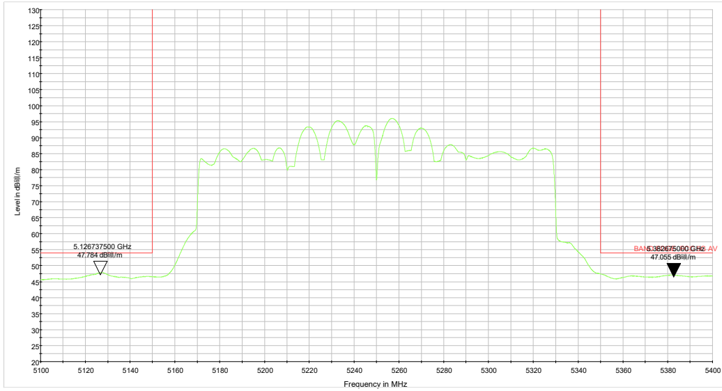
ax160 CH50_5.1-5.4GHz_TP15_0320_AV.wmf
