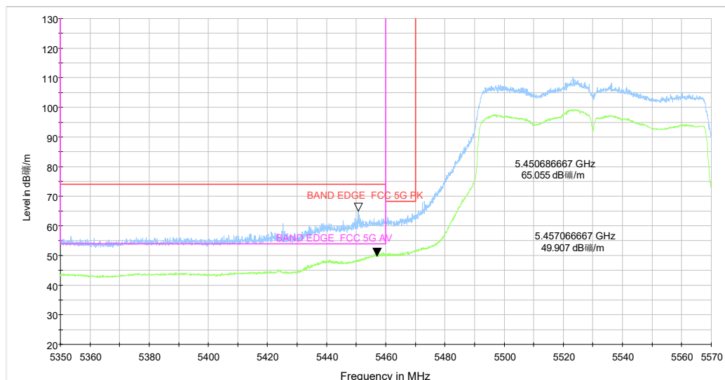
5.35-5.57GHz_5G WIFI_ac(80) CH106 MCS-0_Y_TP16_MIMO
