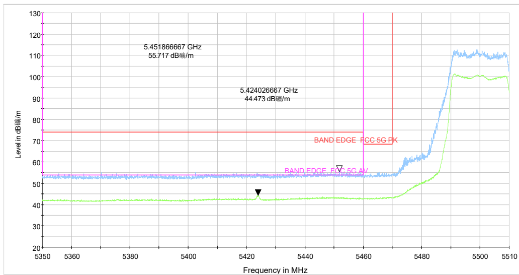
5.35-5.51GHz_5G WIFI_ax(20) CH100 MCS-0_Y_TP15_MIMO
