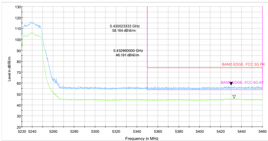
5.23-5.46GHz_5G WIFI_n(20) CH48 MCS-0_Y_TP17_MIMO
