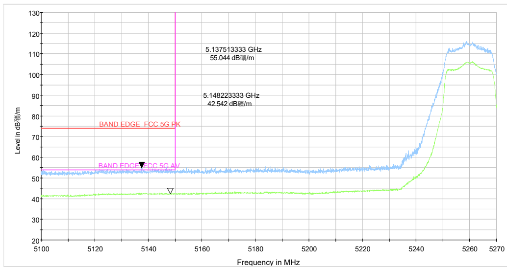
5.1-5.27GHz_5G WIFI_n(20) CH52 MCS-0_Y_TP17_MIMO
