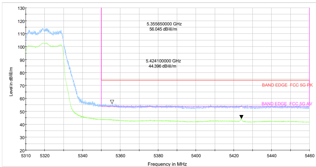
5.31-5.46GHz_5G WIFI_ax(20) CH64 MCS-0_Y_TP15_MIMO
