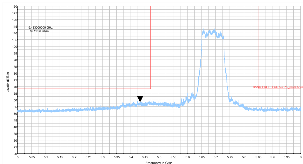
ax80 CH138_5-6GHz_TP15
