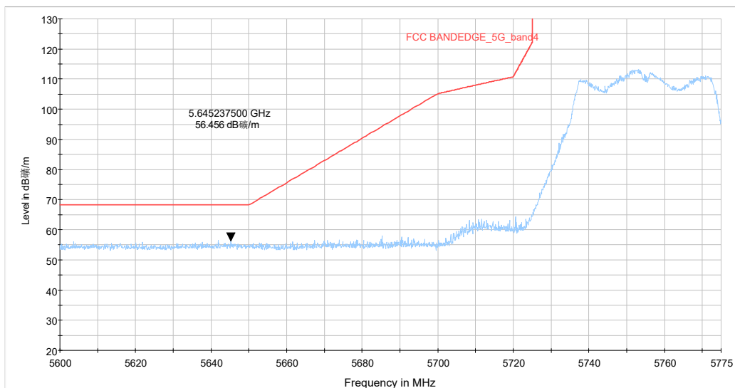
5.6-5.775GHz_5G WIFI_ac(40) CH151 MCS-0_Y_TP16_MIMO
