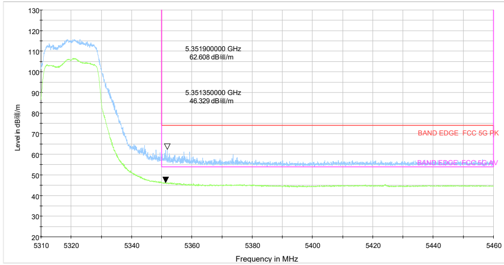
5.31-5.46GHz_5G WIFI_n(20) CH64 MCS-0_Y_TP17_MIMO
