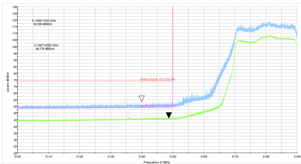
ax20 CH36_5.1-5.19GHz_TP15
