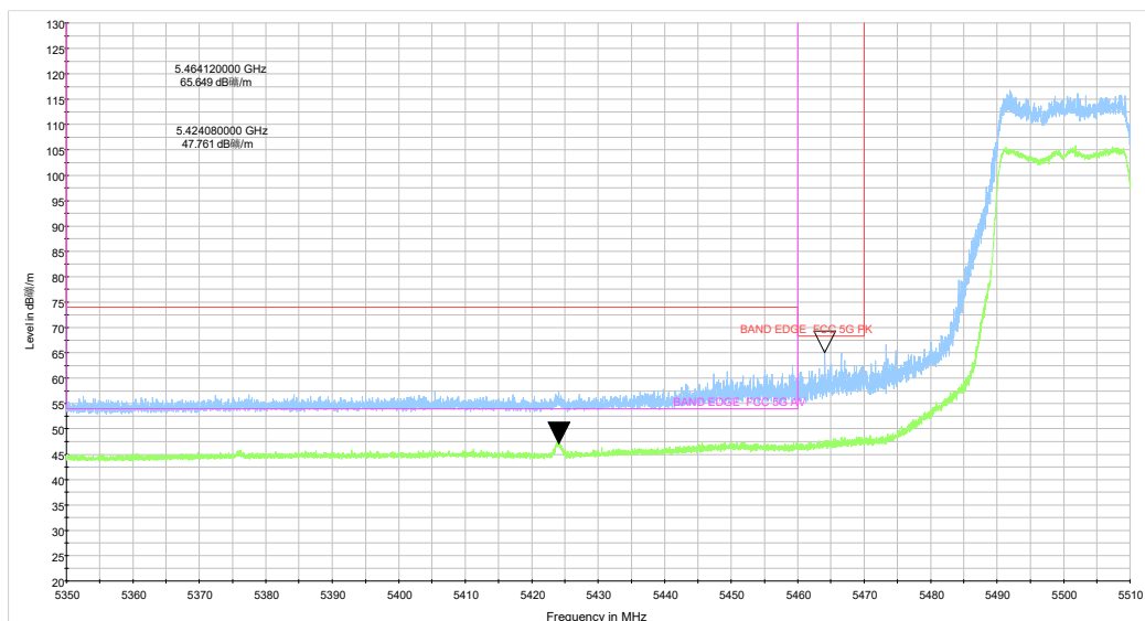
ax20 CH100_5.35-5.51GHz_TP15
