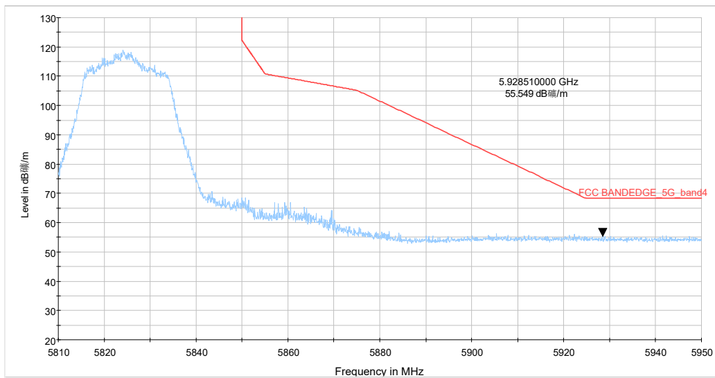
5.81-5.95GHz_5G WIFI_ax(20) CH165 MCS-0_Y_TP15_MIMO
