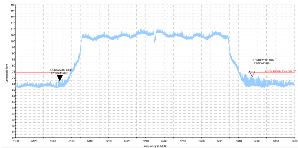
ax160 CH50_5.1-5.4GHz_TP15_0320_PK.wmf
