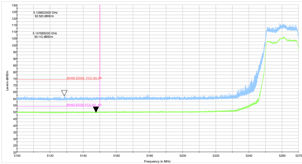
be20 CH52_5.1-5.27GHz_TP14
