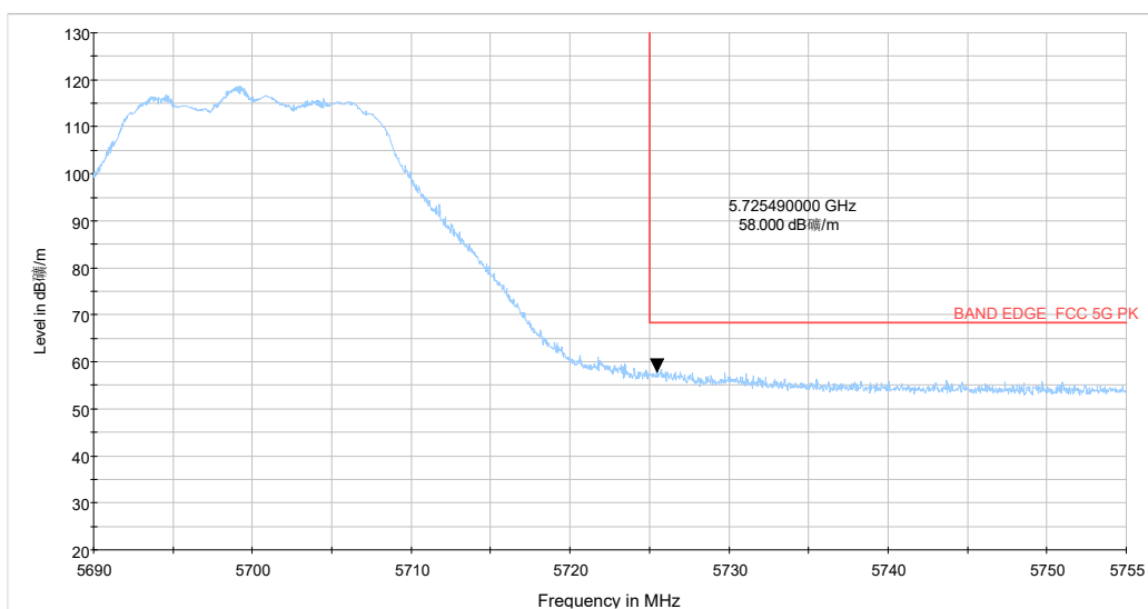
5.69-5.755GHz_5G WIFI_a CH140 6M_Y_TP19_MIMO
