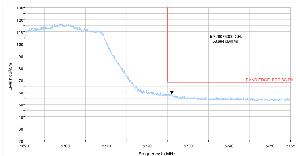
5.69-5.755GHz_5G WIFI_ax(20) CH140 MCS-0_Y_TP15_MIMO
