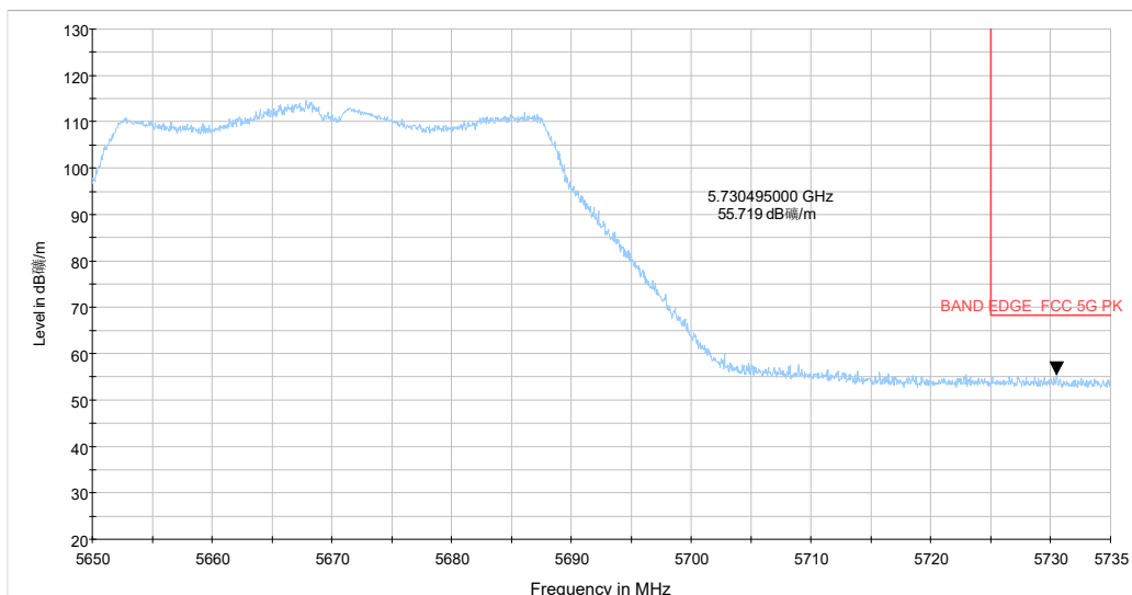
5.65-5.735GHz_5G WIFI_n(40) CH134 MCS-0_Y_TP17_MIMO
