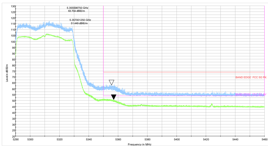
ax40 CH62_5.29-5.46GHz_TP15
