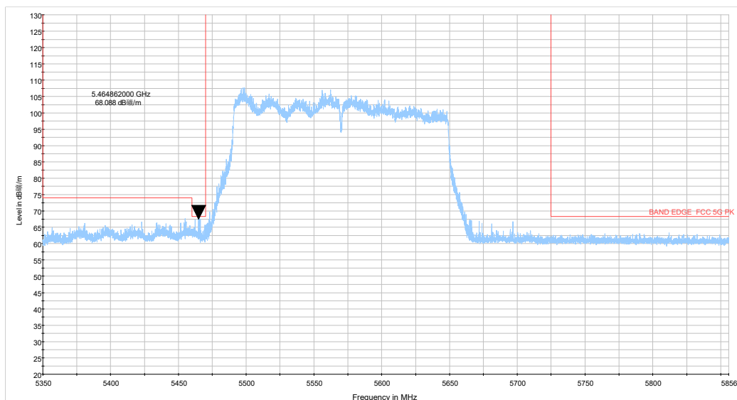
ax160 CH114_5.35-5.856GHz_TP14_0320_PK.wmf
