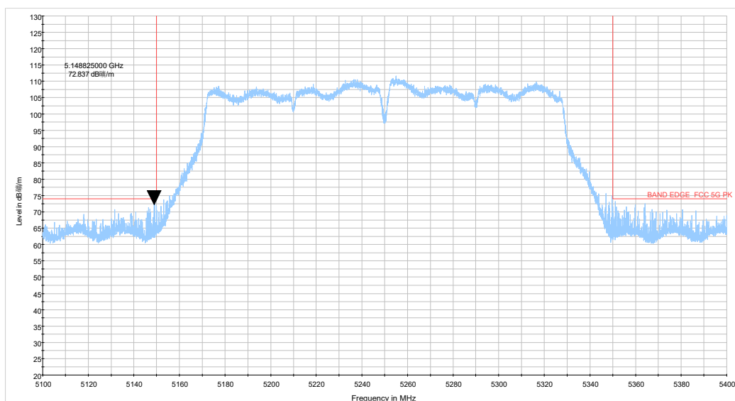
ac160 CH50_5.1-5.4GHz_TP16_0320_PK.wmf
