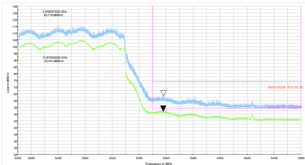
ax80 CH58_5.25-5.46GHz_TP15
