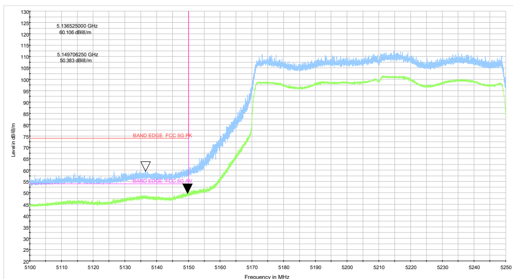
be80 CH42_5.1-5.25GHz_TP14
