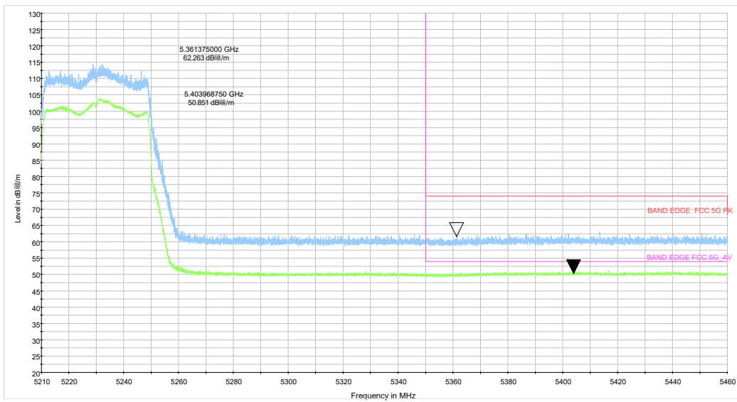
be40 CH46_5.21-5.46GHz_TP14
