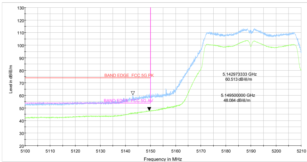
5.1-5.21GHz_5G WIFI_ac(40) CH38 MCS-0_Y_TP16_MIMO
