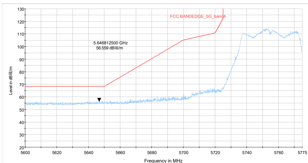
5.6-5.775GHz_5G WIFI_n(40) CH151 MCS-0_Y_TP17_MIMO
