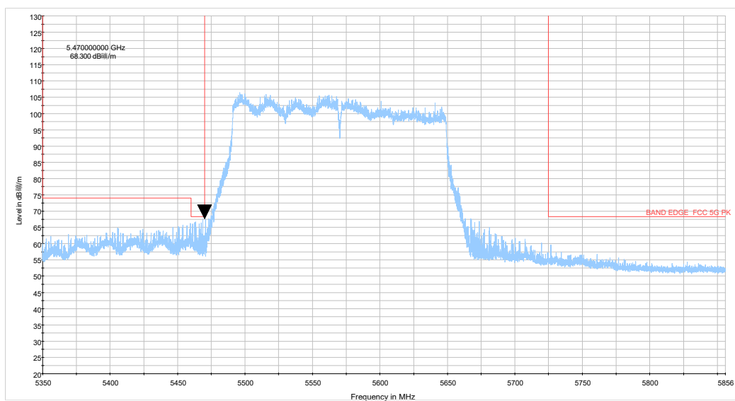
be160 CH114_5.35-5.856GHz_TP12_0320_PK.wmf
