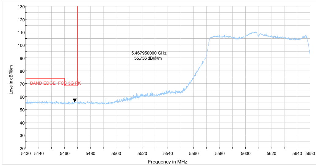
5.43-5.65GHz_5G WIFI_ac(80) CH122 MCS-0_Y_TP16_MIMO
