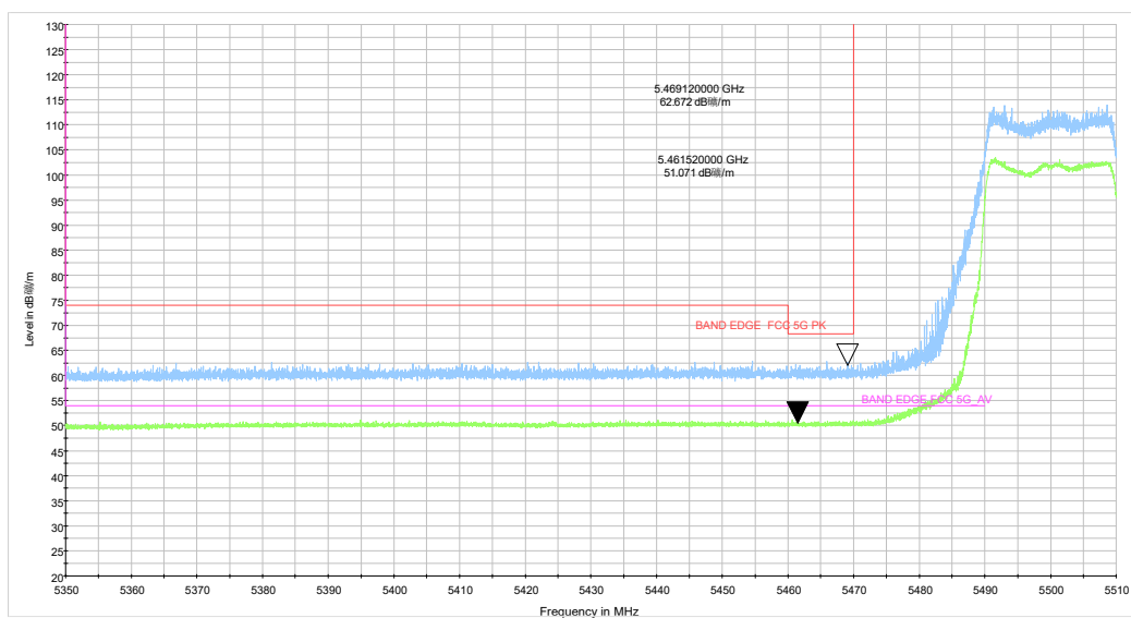
be20 CH100_5.35-5.51GHz_TP14
