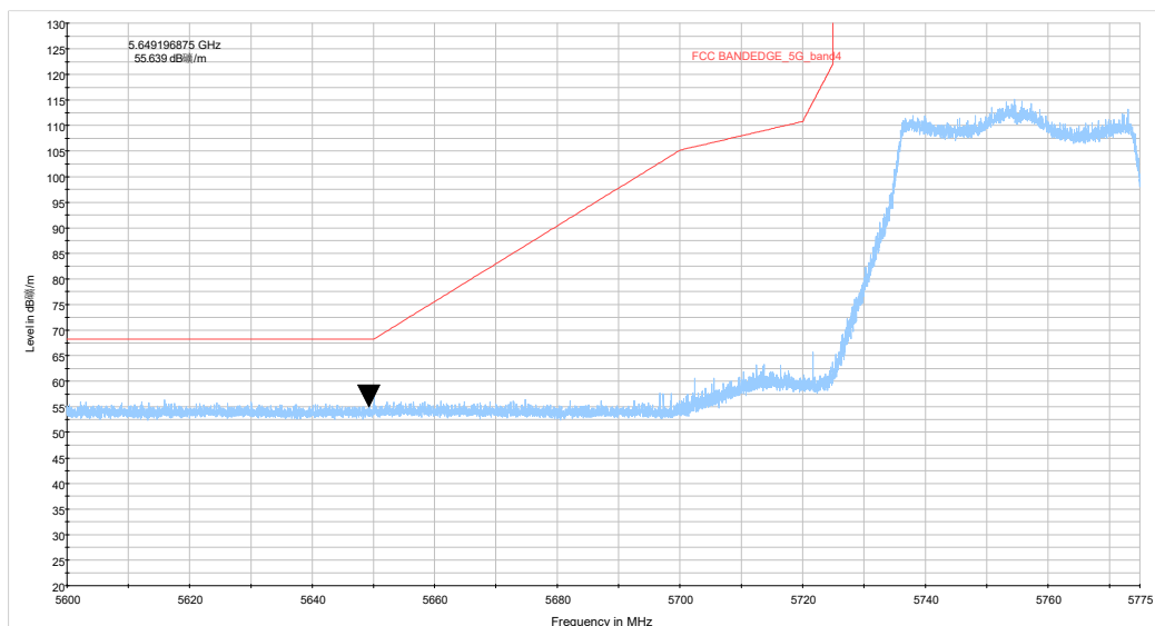
be40 CH151_5.6-5.775GHz_TP14
