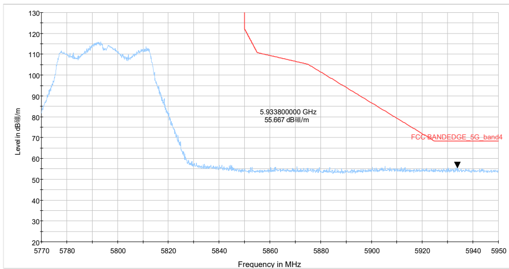
5.77-5.95GHz_5G WIFI_n(40) CH159 MCS-0_Y_TP17_MIMO
