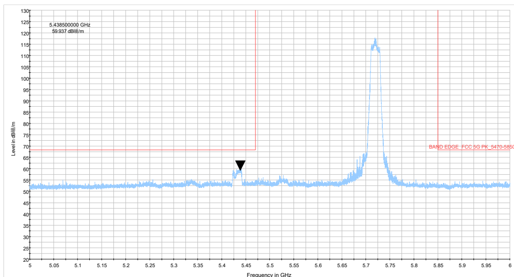
ax20 CH144_5-6GHz_TP15
