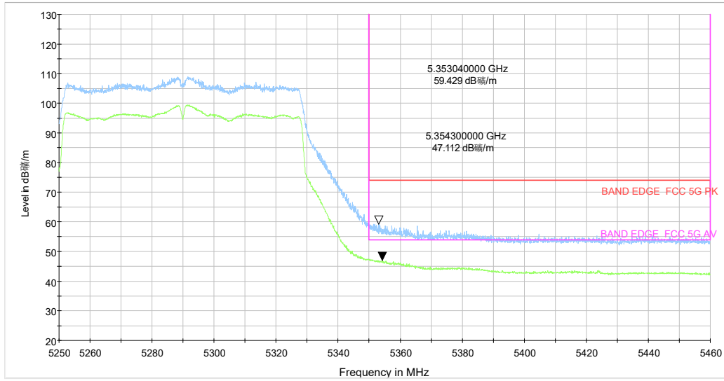
5.25-5.46GHz_5G WIFI_ac(80) CH58 MCS-0_Y_TP16_MIMO
