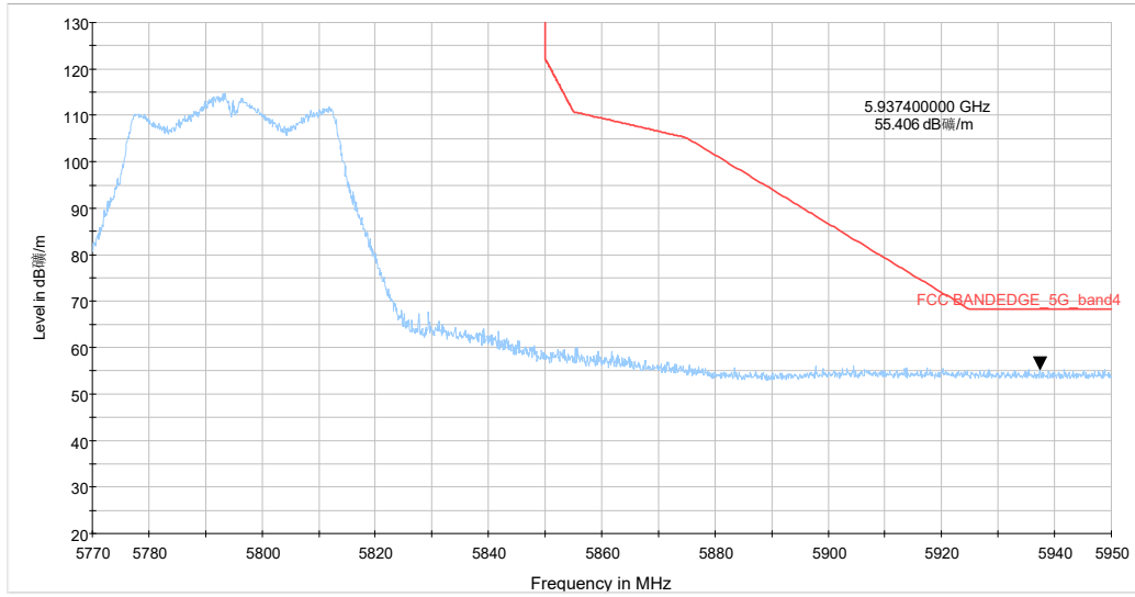
5.77-5.95GHz_5G WIFI_ac(40) CH159 MCS-0_Y_TP16_MIMO
