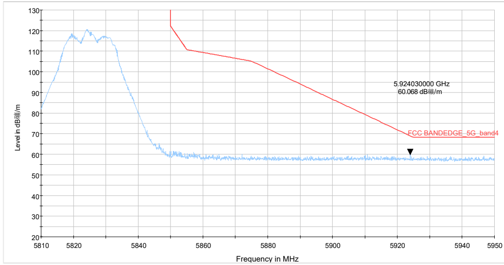
5.81-5.95GHz_5G WIFI_a CH165 6M_Y_TP19_MIMO
