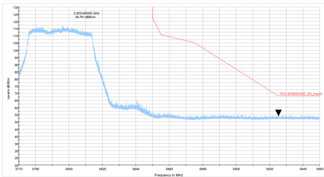
ax40 CH159_5.77-5.95GHz_TP15
