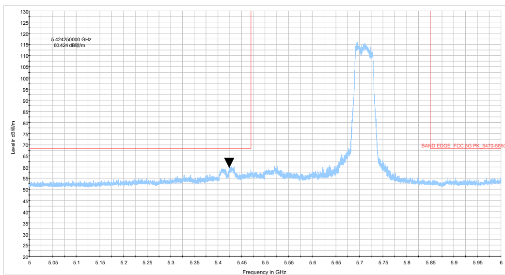
ax40 CH142_5-6GHz_TP15
