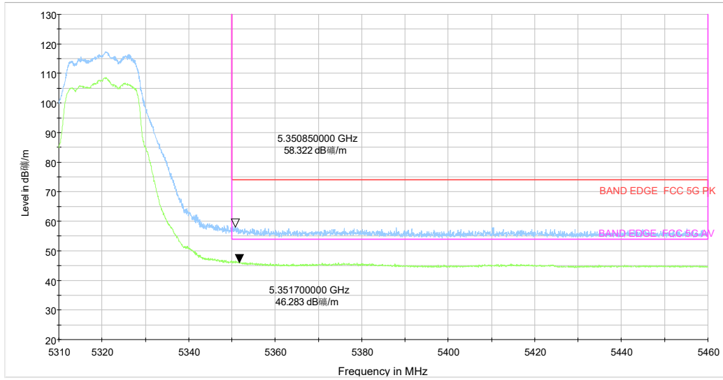
5.31-5.46GHz_5G WIFI_a CH64 6M_Y_TP19_MIMO
