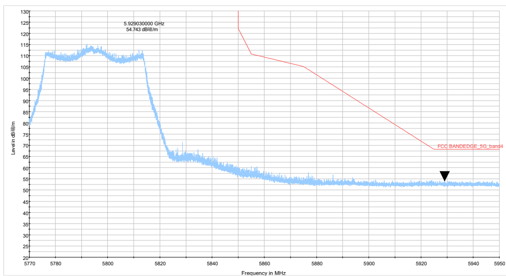
be40 CH159_5.77-5.95GHz_TP14
