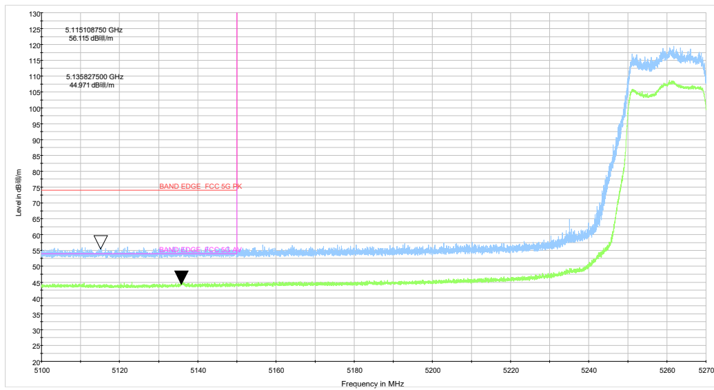
ax20 CH52_5.1-5.27GHz_TP15
