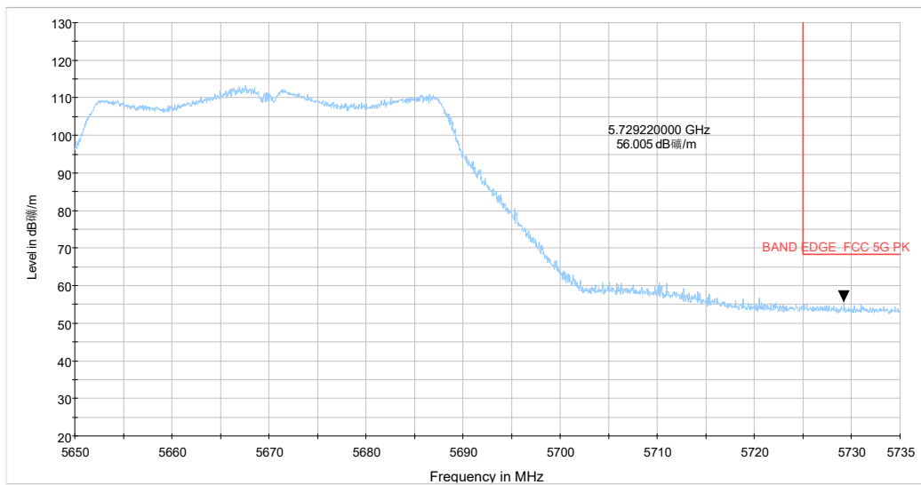
5.65-5.735GHZ_5G WIFI_ac(40) CH134 MCS-0_Y_TP16_MIMO
