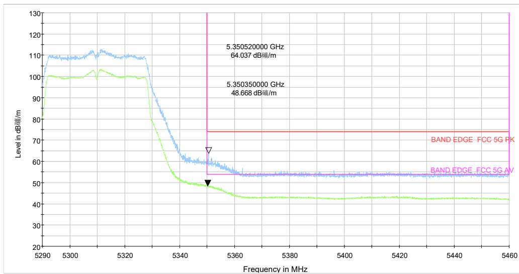
5.29-5.46GHz_5G WIFI_n(40) CH62 MCS-0_Y_TP17_MIMO
