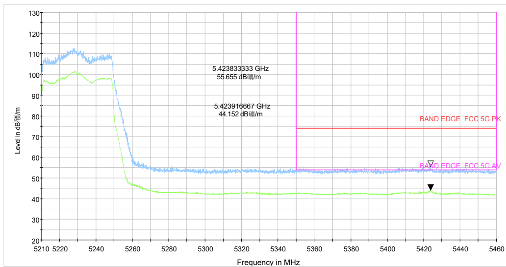
5.21-5.46GHz_5G WIFI_ax(40) CH46 MCS-0_Y_TP15_MIMO
