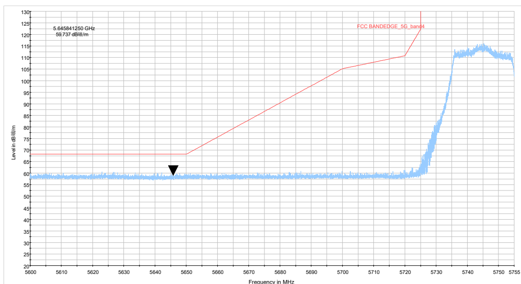
be20 CH149_5.6-5.755GHz_TP14
