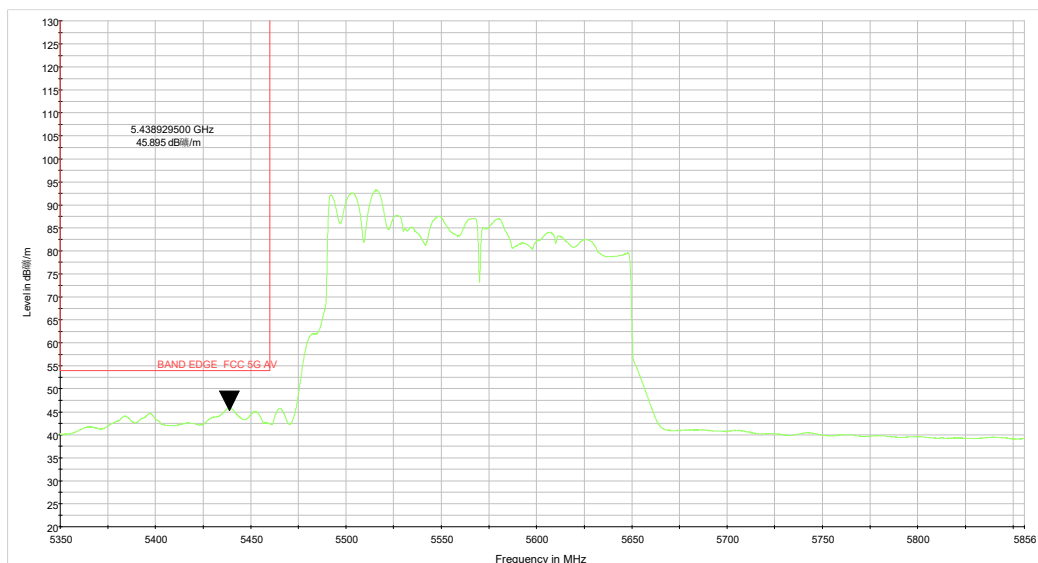
be160 CH114_5.35-5.856GHz_TP13_0320_AV.wmf
