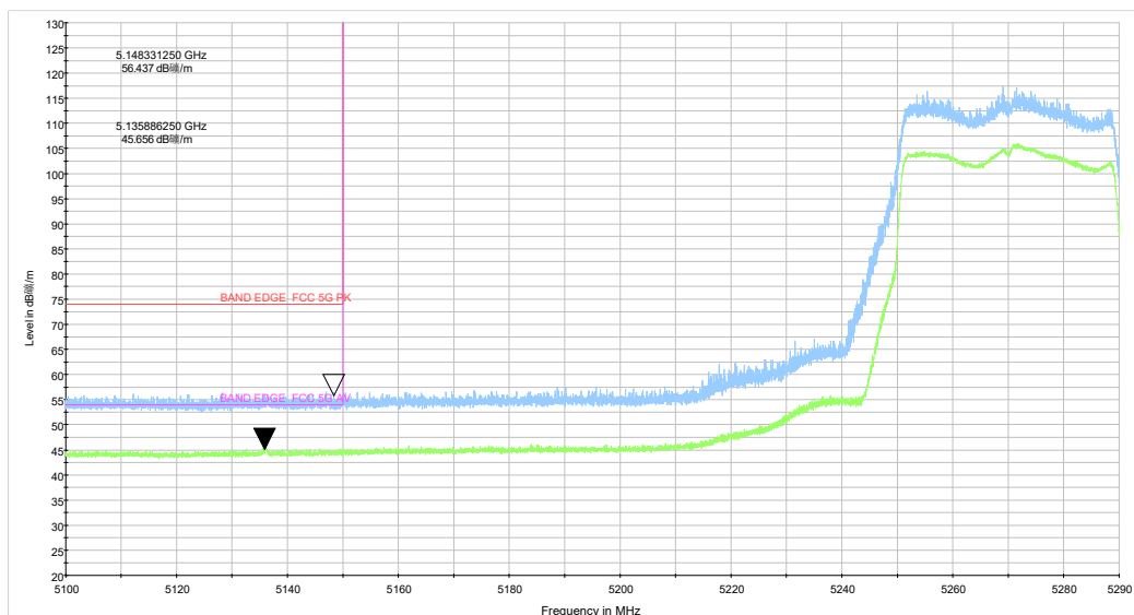
ax40 CH54_5.1-5.29GHz_TP15
