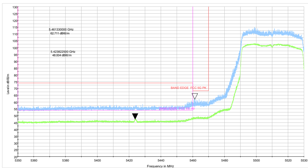
ax40 CH102_5.35-5.53GHz_TP15
