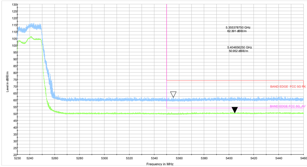
be20 CH48_5.23-5.46GHz_TP14
