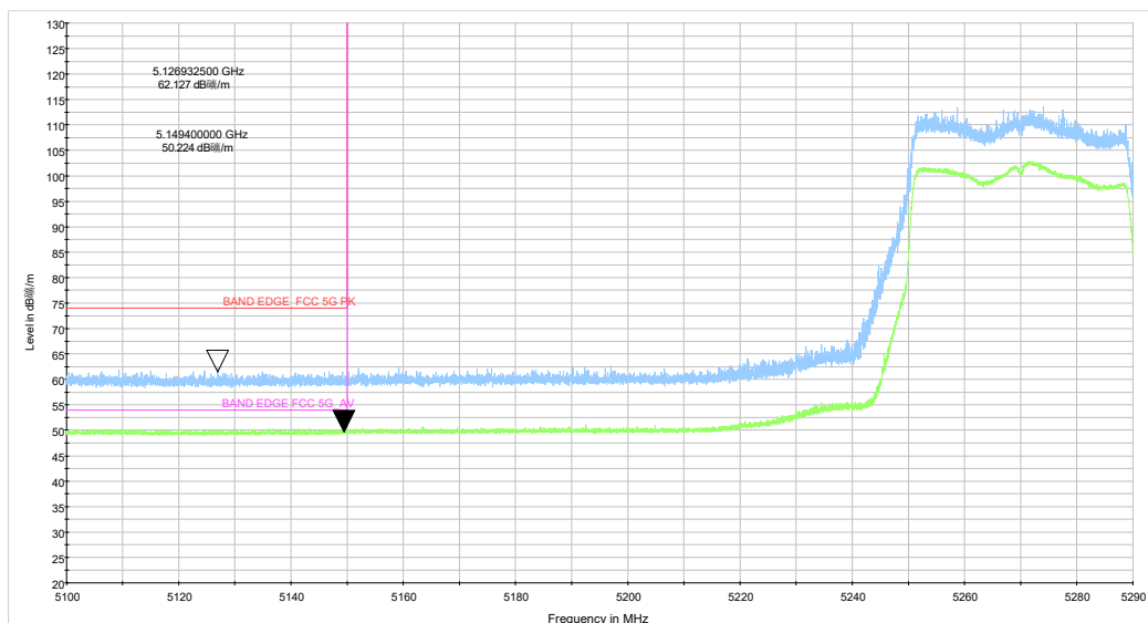
be40 CH54_5.1-5.29GHz_TP14
