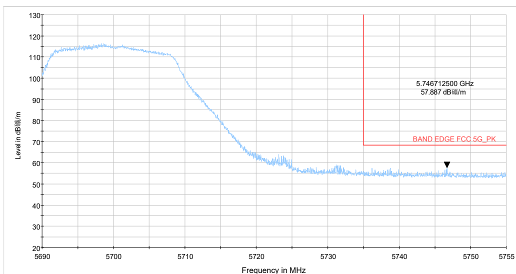
5.69-5.755GHz_5G WIFI_n(20) CH140 MCS-0_Y_TP17_MIMO
