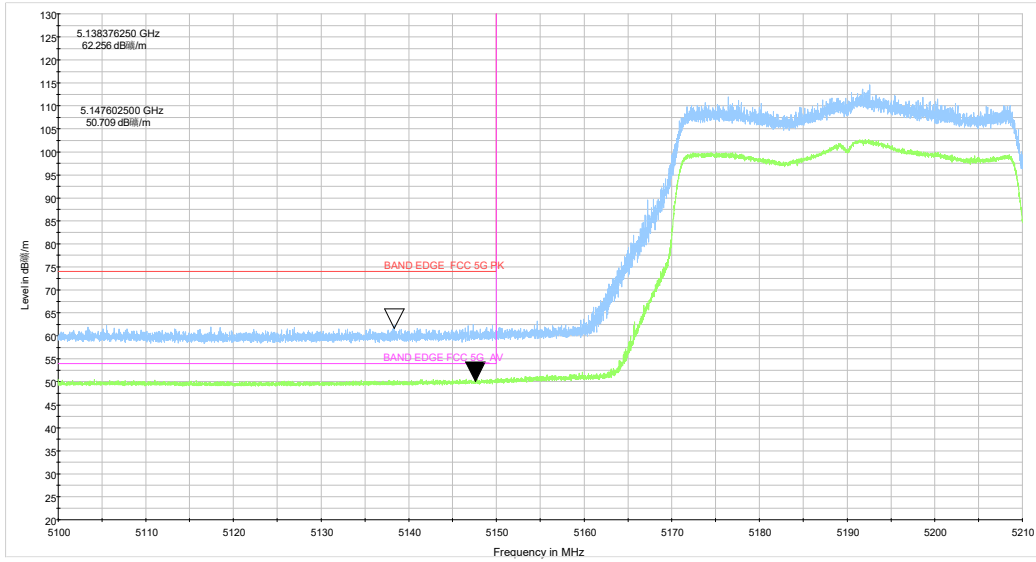
be40 CH38_5.1-5.21GHz_TP14
