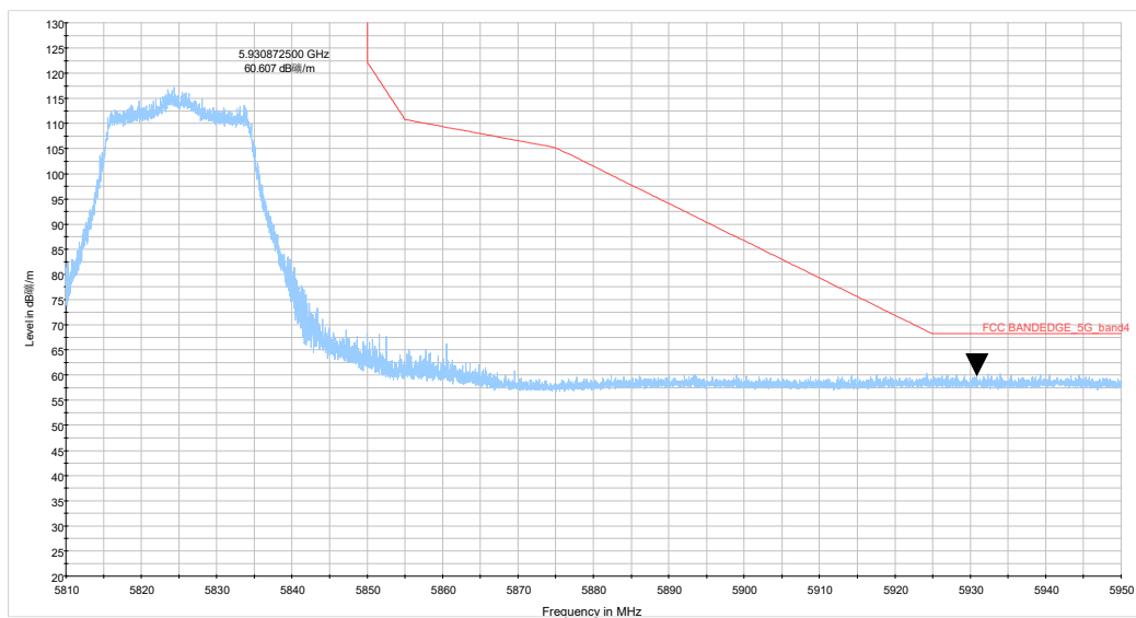
be20 CH165_5.81-5.95GHz_TP14
