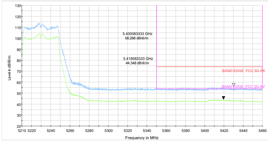
5.21-5.46GHz_5G WIFI_n(40) CH46 MCS-0_Y_TP17_MIMO
