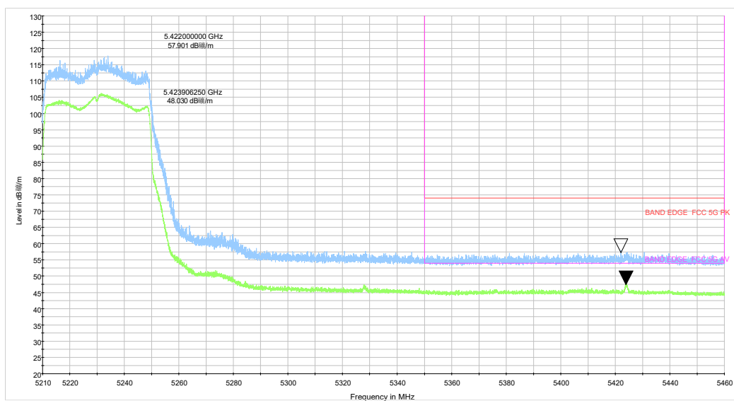
ax40 CH46_5.21-5.46GHz_TP15
