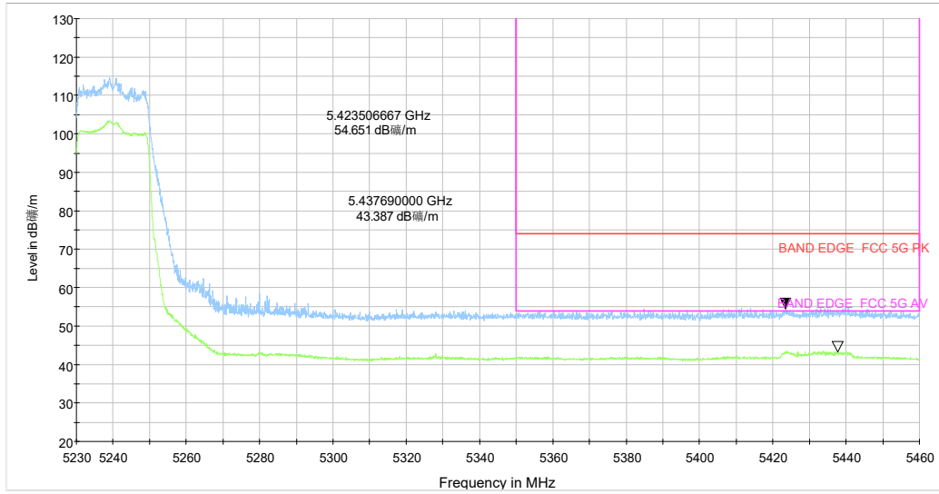
5.23-5.46GHz_5G WIFI_ax(20) CH48 MCS-0_Y_TP15_MIMO
