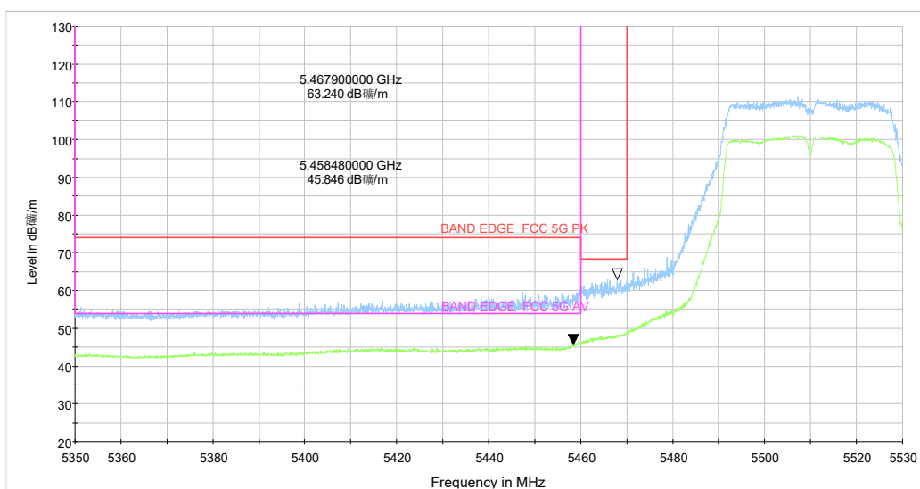
5.35-5.53GHz_5G WIFI_n(40) CH102 MCS-0_Y_TP17_MIMO
