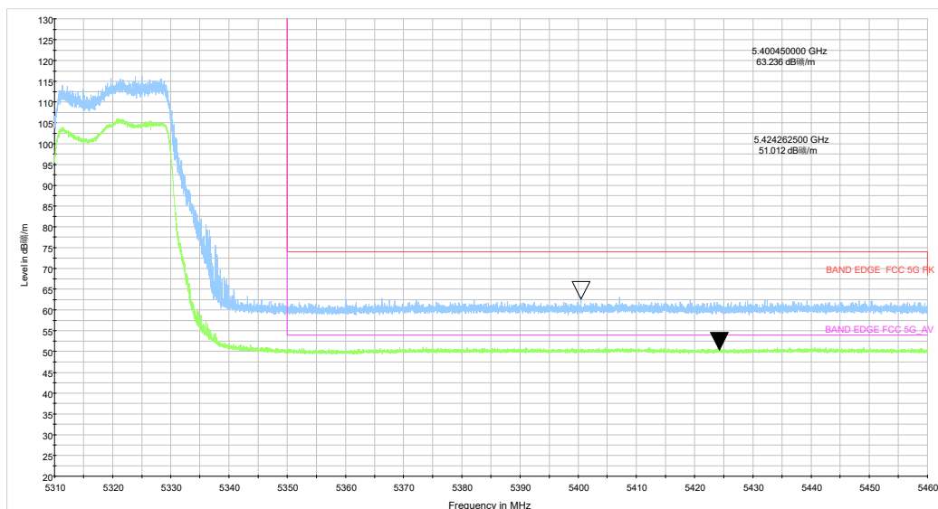
be20 CH64_5.31-5.46GHz_TP14
