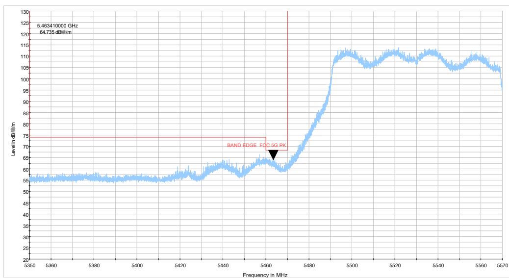
ax80 CH106_5.35-5.57GHz_TP15_0321_PK.wmf
