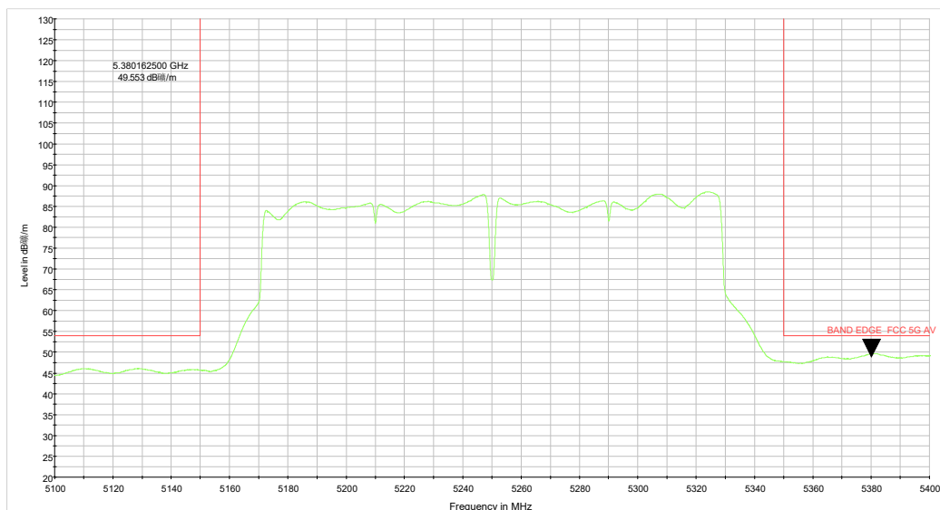
ac160 CH50_5.1-5.4GHz_TP16_0320_AV.wmf
