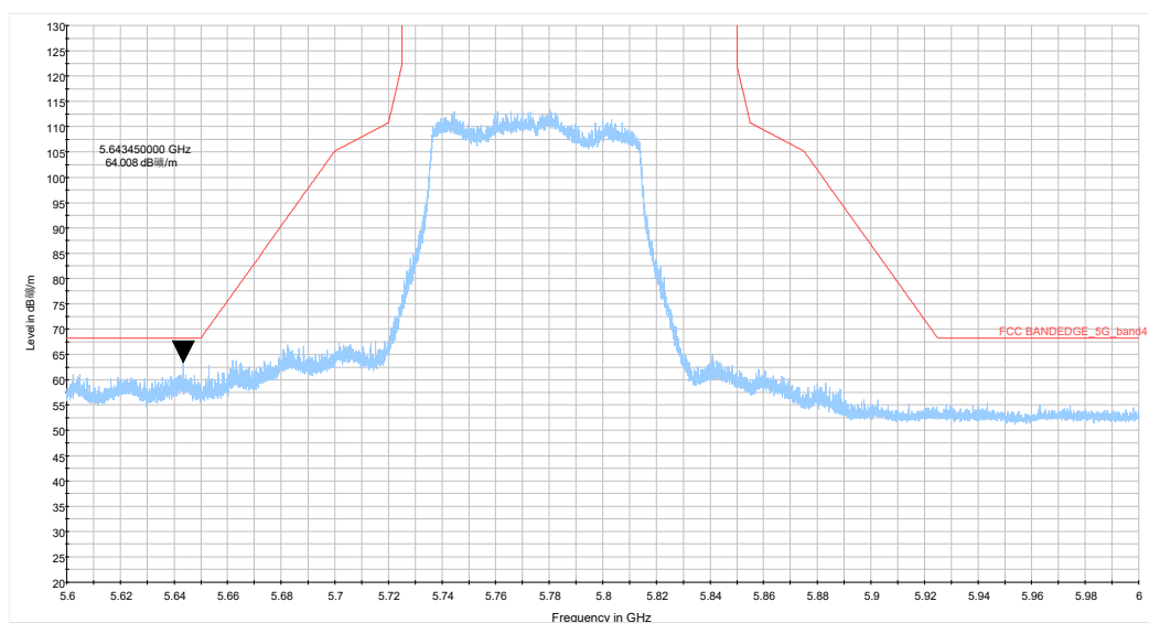
ax80 CH155_5.6-.6GHz_TP15
