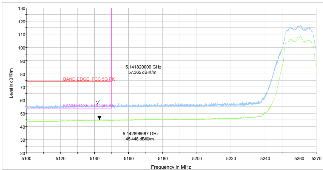
5.1-5.27GHz_5G WIFI_a CH52 6M_Y_TP19_MIMO_031.5.wmf
