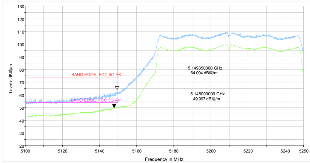
5.1-5.25GHz_5G WIFI_ac(80) CH42MCS-0_Y_TP16_MIMO
