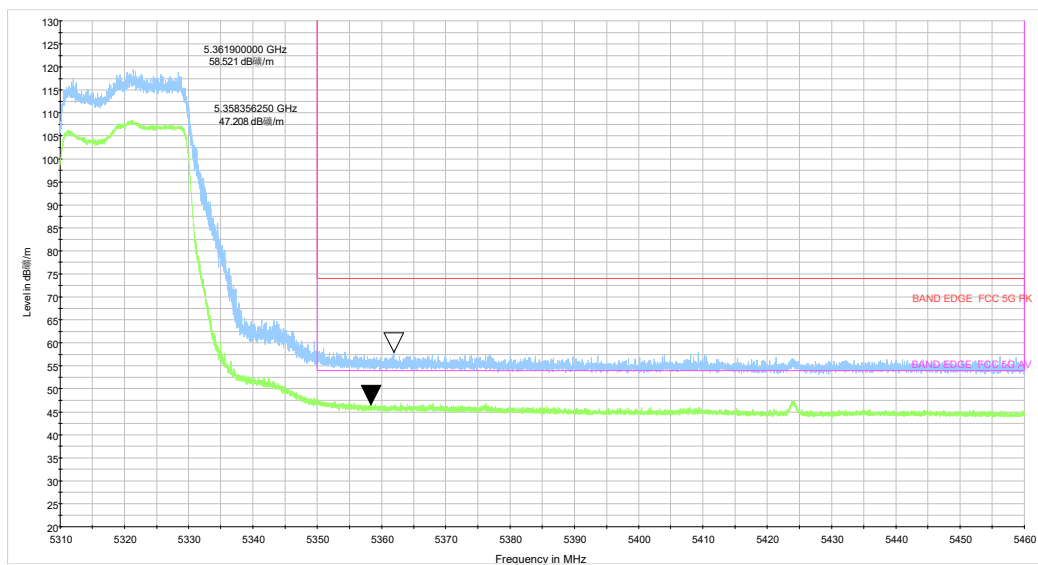
ax20 CH64_5.31-5.46GHz_TP15
