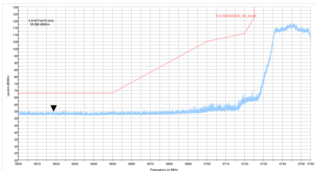
ax20 CH149_5.6-5.755GHz_TP15
