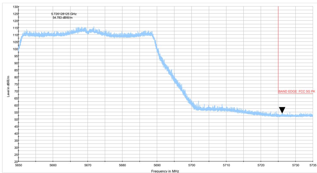
be40 CH134_5.65-5.735GHz_TP14
