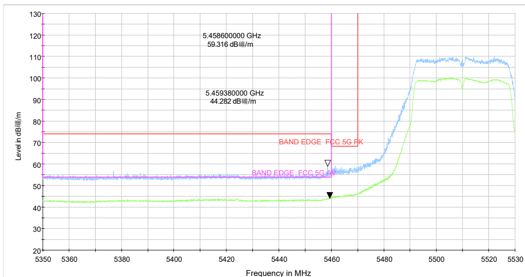
5.35-5.53GHz_5G WIFI_ac(40) CH102 MCS-0_Y_TP16_MIMO
