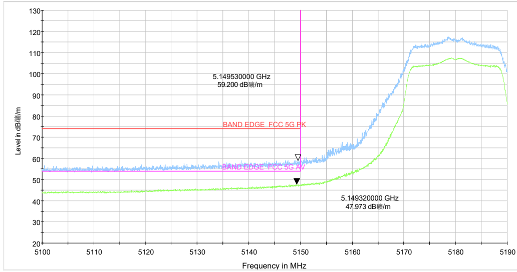
5.1-5.19GHz_5G WIFI_n(20) CH36 MCS-0_Y_TP17_MIMO
