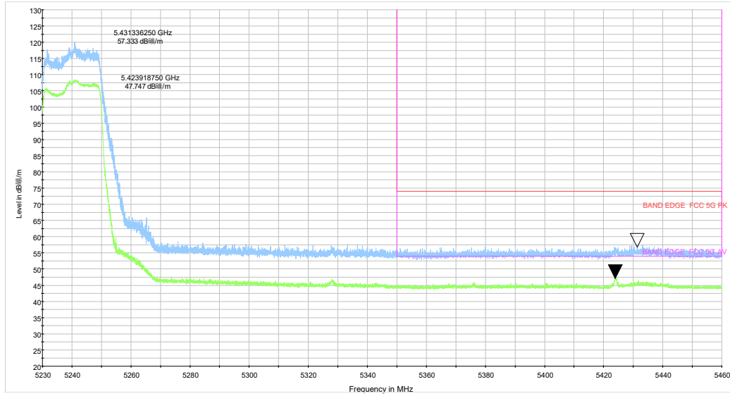
ax20 CH48_5.23-5.46GHz_TP15
