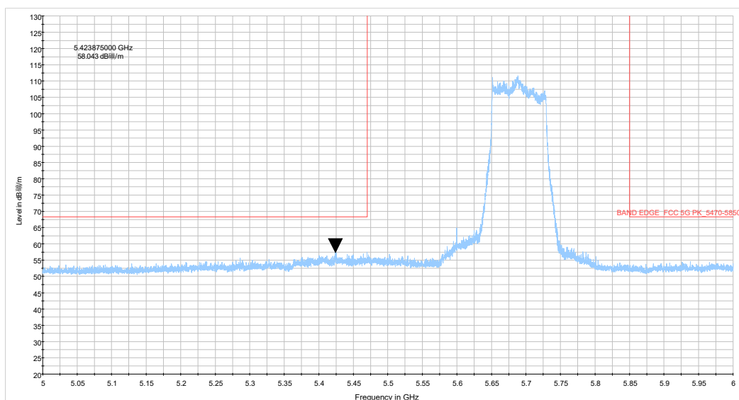
be80 CH138_5-6GHz_TP14
