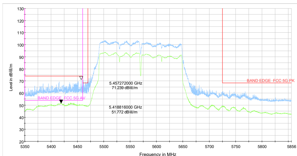
5.35-5.856GHz_5G WIFI_ac(160) CH114 MCS-0_Y_TP15_MIMO
