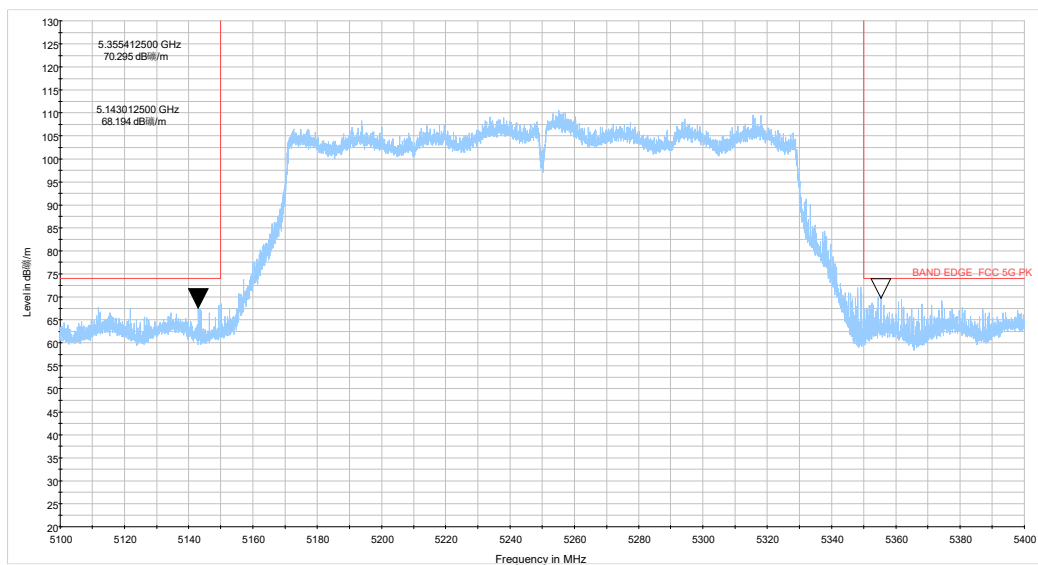
be160 CH50_5.1-5.4GHz_TP14_0320_PK.wmf
