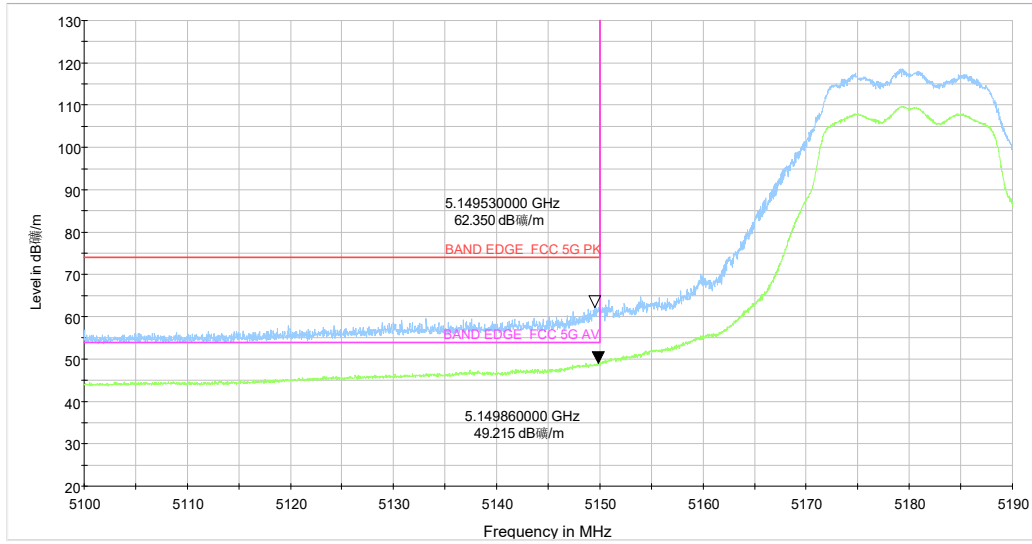
5.1-5.19GHz_5G WIFI_a CH36 6M_Y_TP19_MIMO
