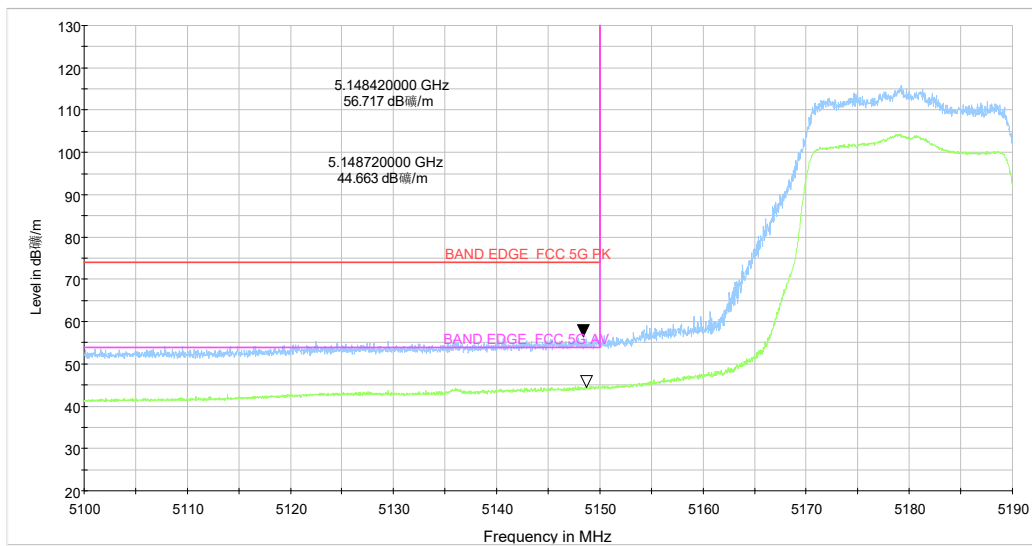
5.1-5.19GHz_5G WIFI_ax(20) CH36 MCS-0_Y_TP15_MIMO
