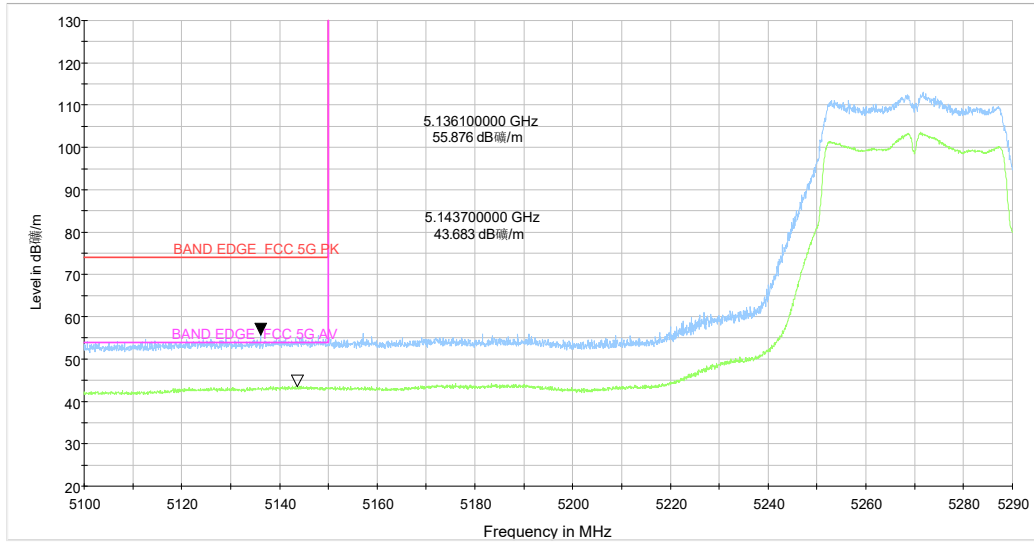
5.1-5.29GHz_5G WIFI_n(40) CH54 MCS-0_Y_TP17_MIMO
