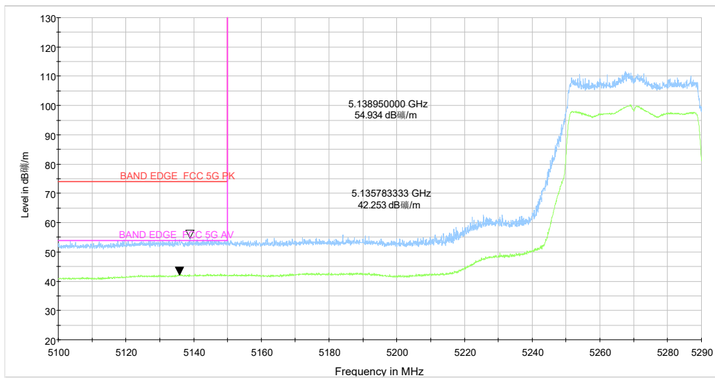
5.1-5.29GHz_5G WIFI_ax(40) CH54 MCS-0_Y_TP15_MIMO
