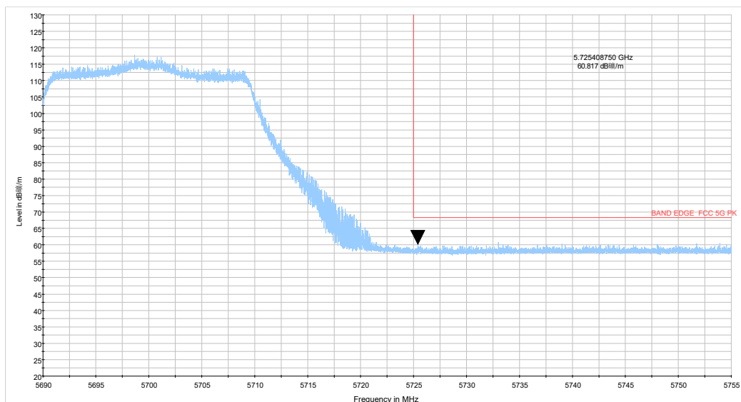
be20 CH140_5.69-5.755GHz_TP14
