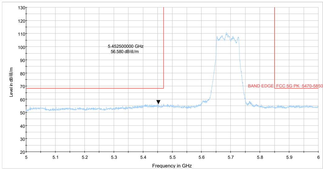
5-6GHZ_5G WIFI_ac(80) CH138 MCS-0_Y_TP16_MIMO
