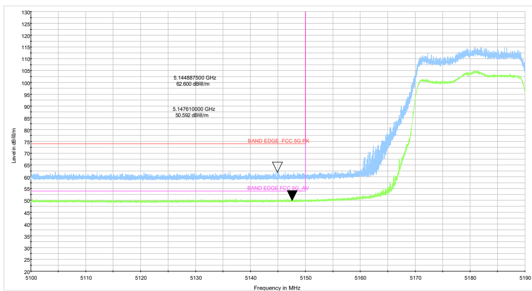
be20 CH36_5.1-5.19GHz_TP14
