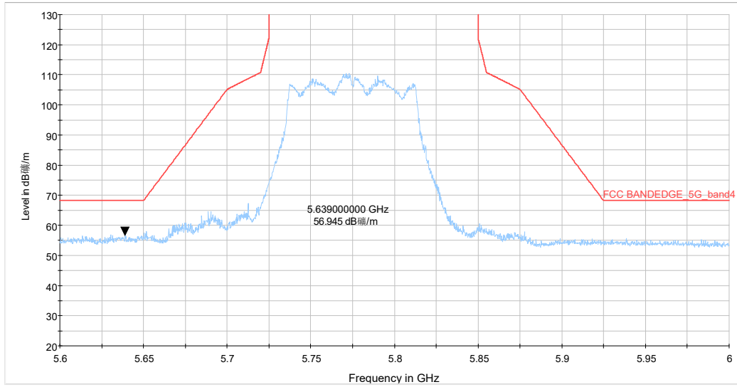
5.6-6GHZ_5G WIFI_ac(80) CH155 MCS-0_Y_TP16_MIMO
