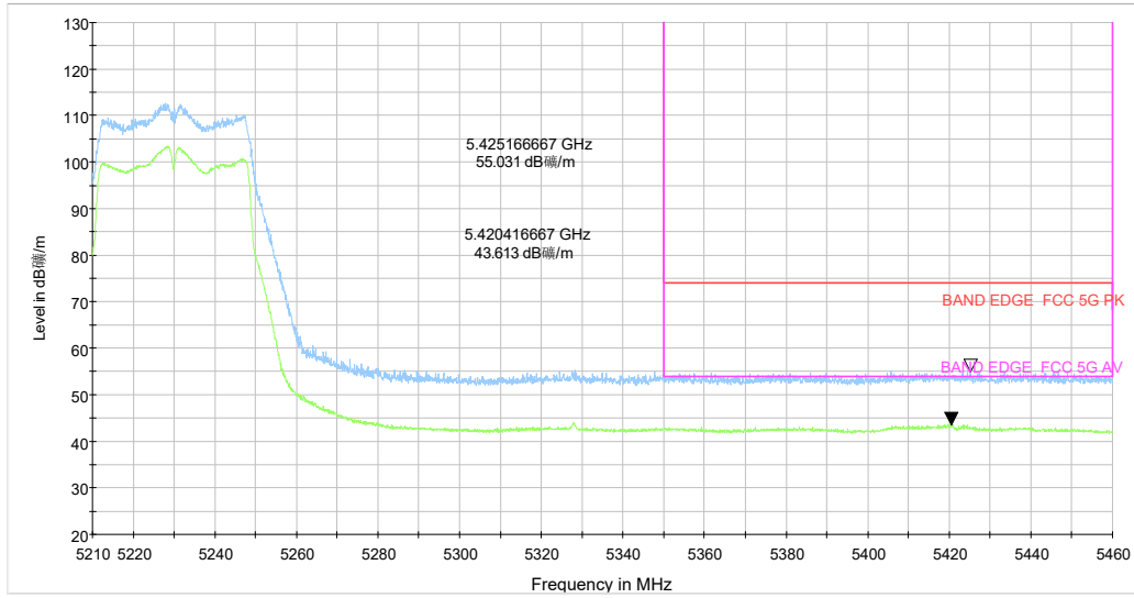
5.21-5.46GHz_5G WIFI_ac(40) CH46 MCS-0_Y_TP16_MIMO
