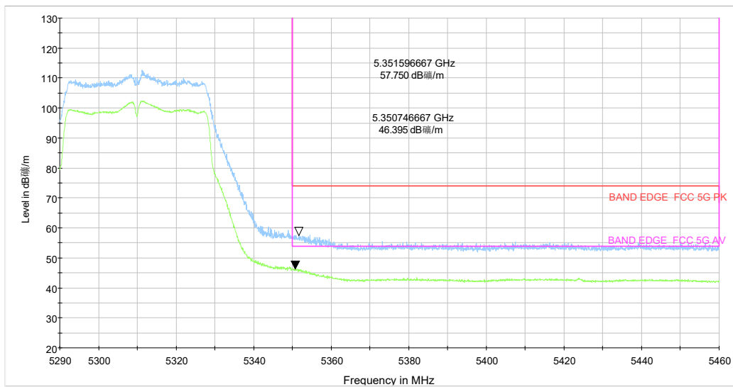
5.29-5.46GHz_5G WIFI_ac(40) CH62 MCS-0_Y_TP16_MIMO
