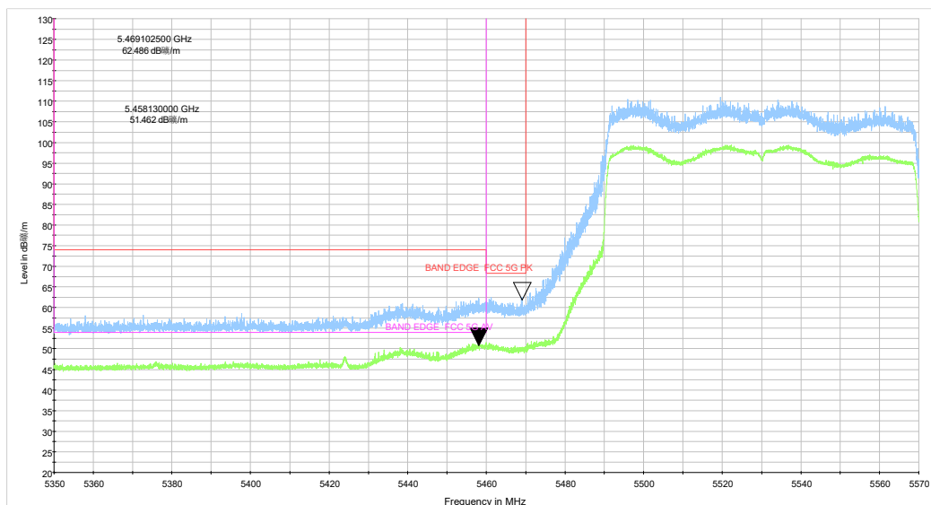
be80 CH106_5.35-5.57GHz_TP14
