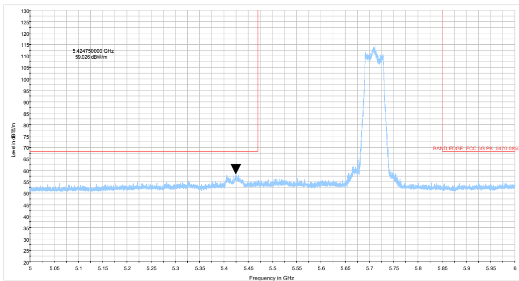
be40 CH142_5-6GHz_TP14
