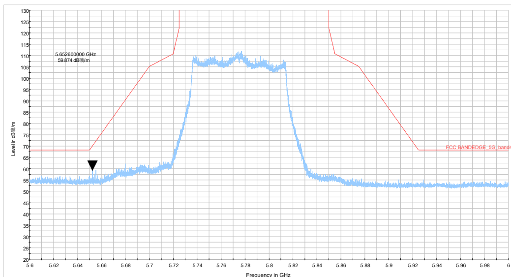
be80 CH155_5-6GHz_TP14
