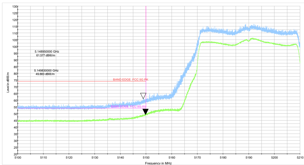
ax40 CH38_5.1-5.21GHz_TP15
