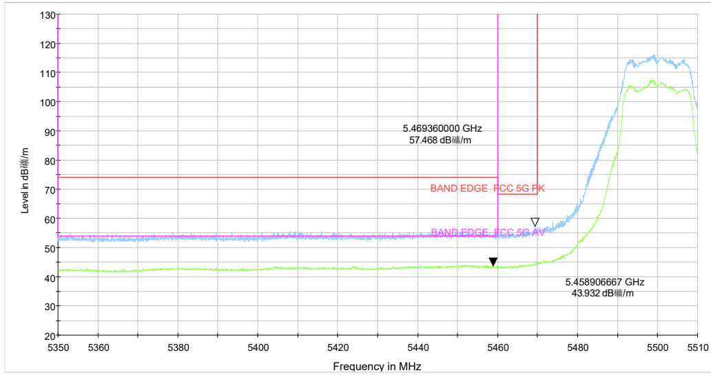
5.35-5.51GHz_5G WIFI_a CH100 6M_Y_TP19_MIMO
