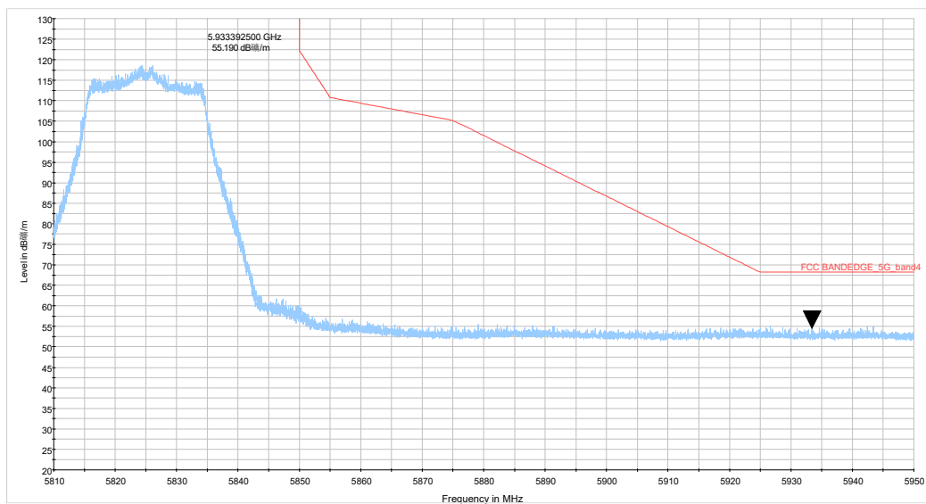
ax20 CH165_5.81-5.95GHz_TP15
