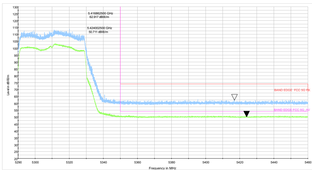
be40 CH62_5.29-5.46GHz_TP14
