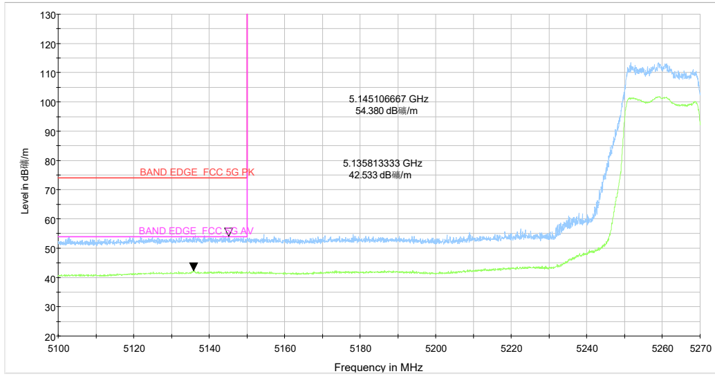
5.1-5.27GHz_5G WIFI_ax(20) CH52 MCS-0_Y_TP15_MIMO
