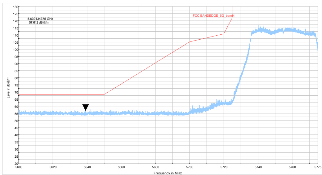
ax40 CH151_5.6-5.775GHz_TP15
