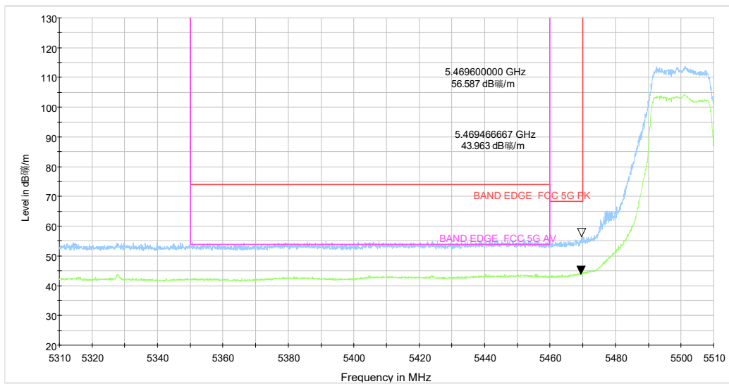
5.31-5.51GHz_5G WIFI_n(20) CH100 MCS-0_Y_TP17_MIMO
