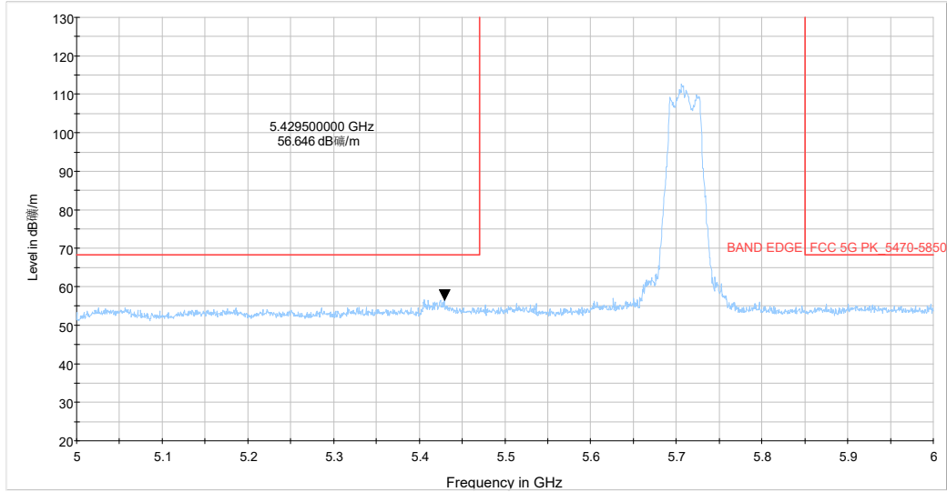
5-6GHZ_5G WIFI_ac(40) CH142 MCS-0_Y_TP16_MIMO
