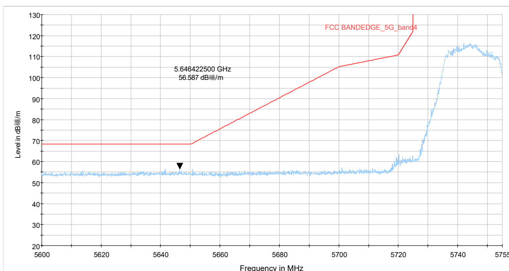
5.6-5.755GHz_5G WIFI_ax(20) CH149 MCS-0_Y_TP15_MIMO
