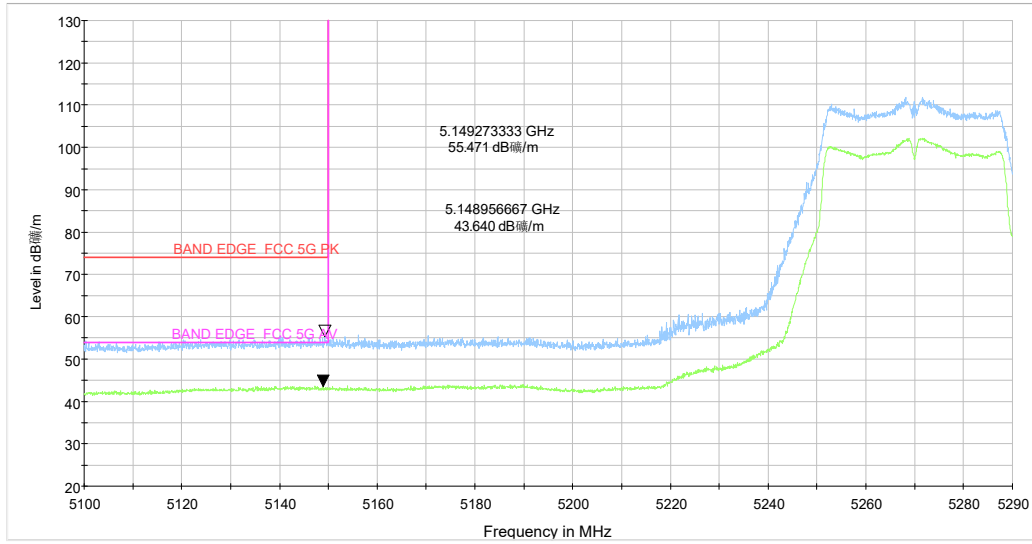
5.1-5.29GHz_5G WIFI_ac(40) CH54 MCS-0_Y_TP16_MIMO
