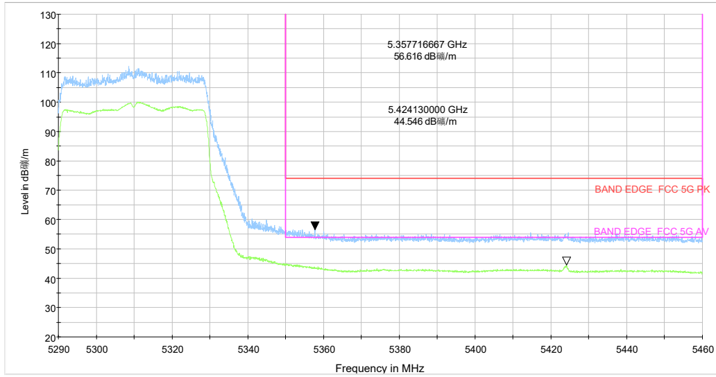
5.29-5.46GHz_5G WIFI_ax(40) CH62 MCS-0_Y_TP15_MIMO
