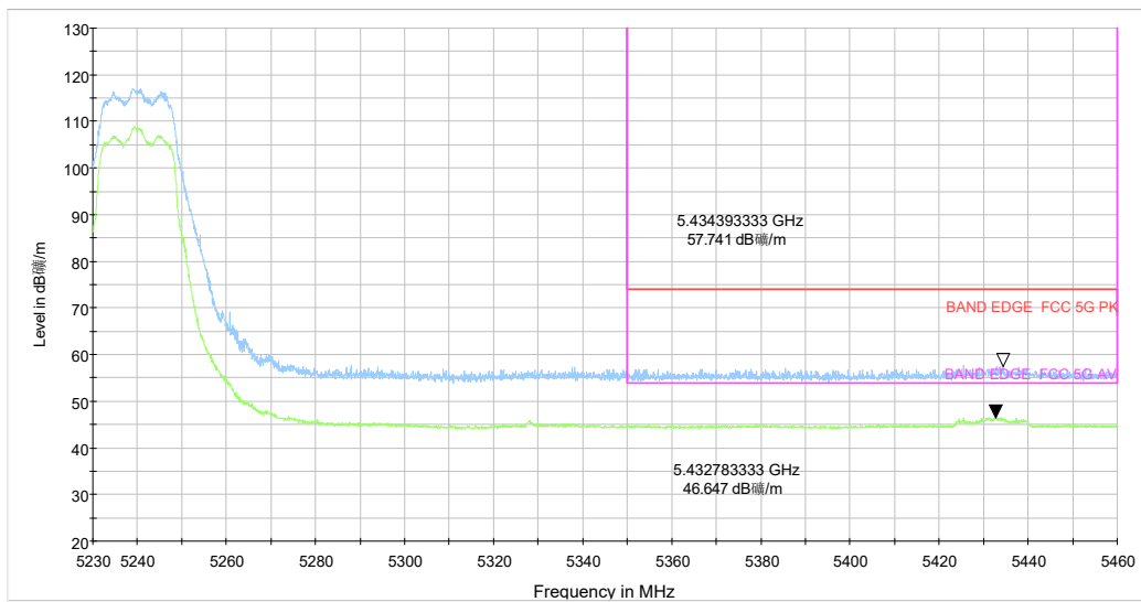
5.23-5.46GHz_5G WIFI_a CH48 6M_Y_TP19_MIMO
