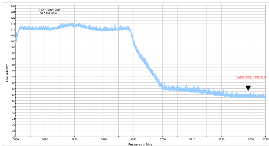
ax40 CH134_5.65-5.735GHz_TP15
