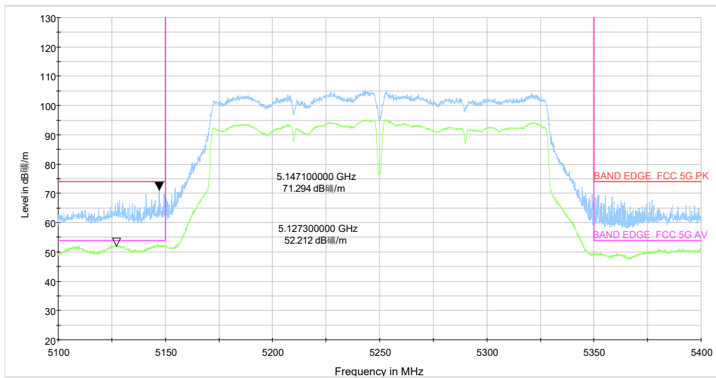
5.1-5.4GHz_5G WIFI_ac(160) CH50 MCS-0_Y_TP16_MIMO
