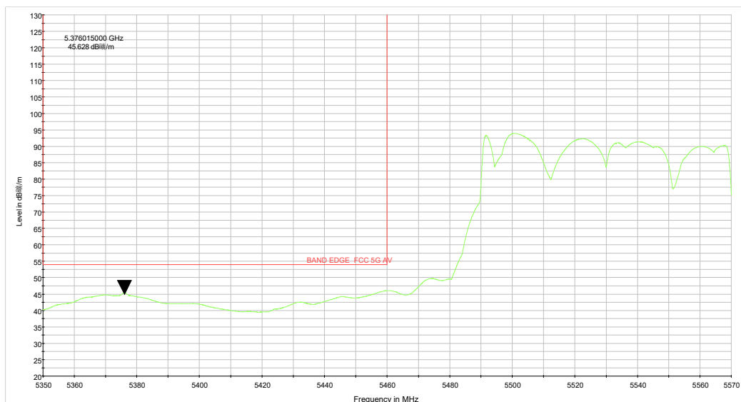
ax80 CH106_5.35-5.57GHz_TP15_0321_AV.wmf
