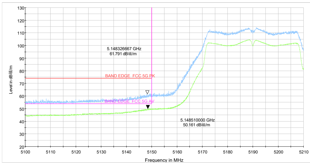
5.1-5.21GHz_5G WIFI_n(40) CH38 MCS-0_Y_TP17_MIMO
