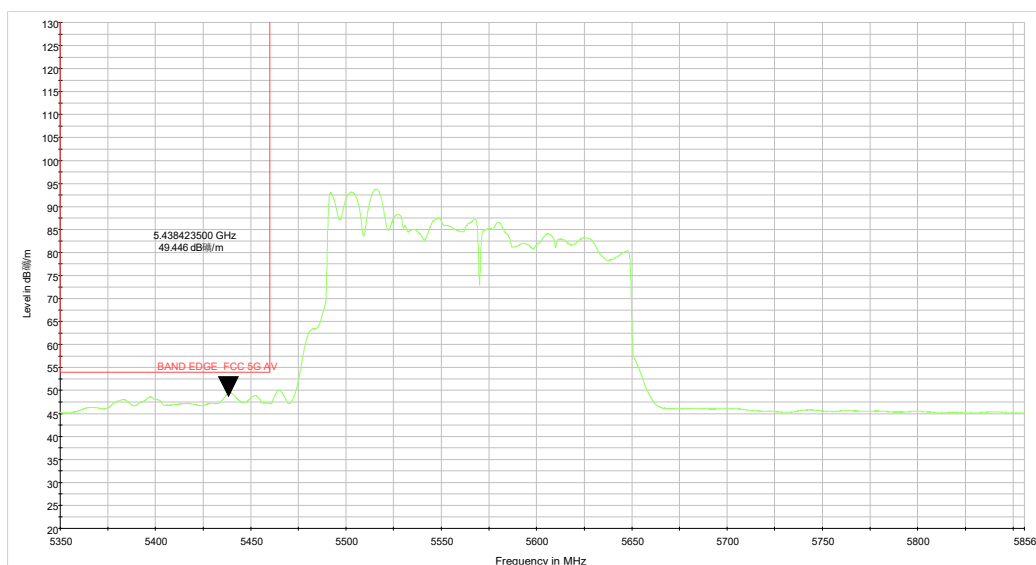
ax160 CH114_5.35-5.856GHz_TP15_0320_AV.wmf
