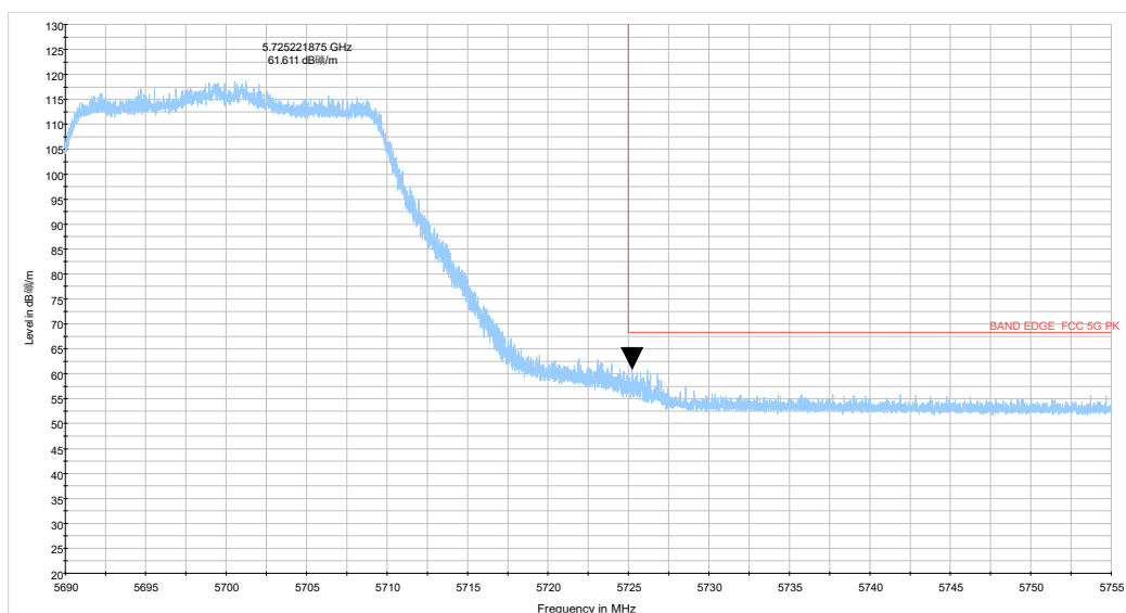
ax20 CH140_5.69-5.755GHz_TP15
