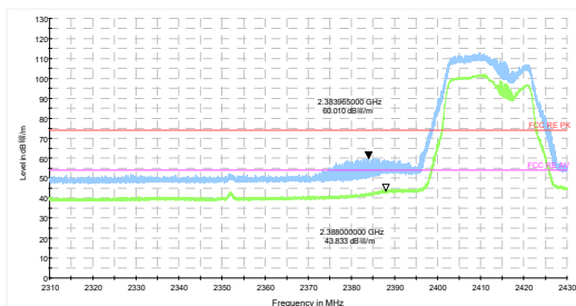
802.11be EHT20-Channel 1 Peak+ Average
