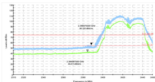
802.11be EHT40-Channel 3 Peak+ Average
