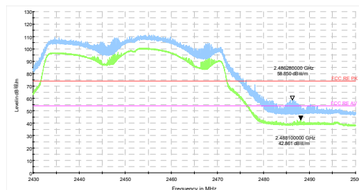
802.11be EHT40-Channel 9 Peak+ Average
