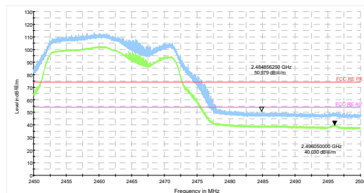
802.11be EHT20-Channel 11 Peak+ Average
