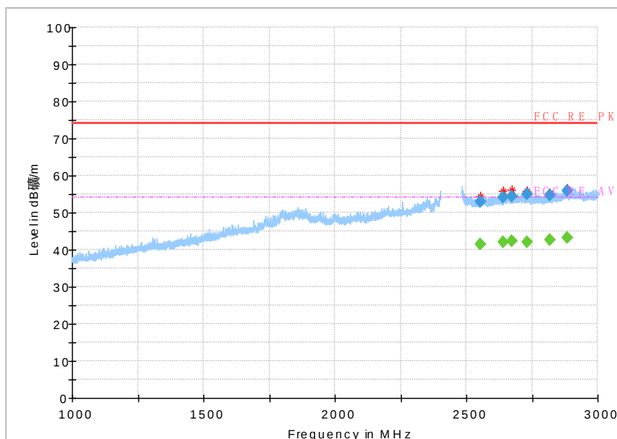
Fig 58. Radiated Spurious Emission (802.11b,Ch11,1GHz~3GHz)
