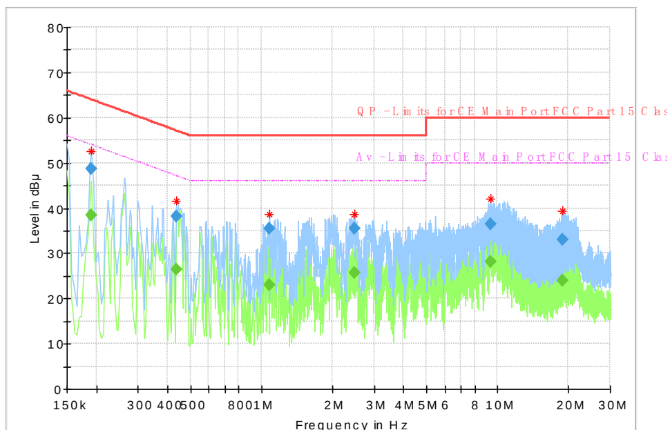
Fig 70. AC Powerline Conducted Emission
