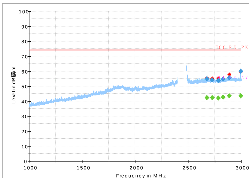
Fig 63. Radiated Spurious Emission (802.11g,Ch11,1GHz~3GHz)
