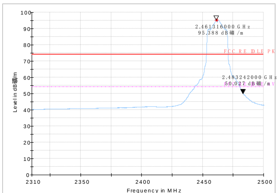
Fig 61. Bandedge: 802.11g, high channel
