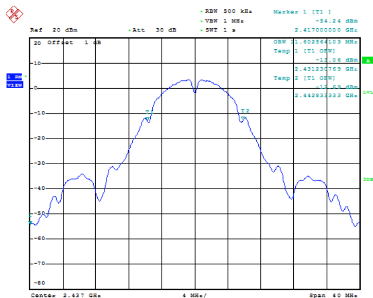
Fig 19. 99% Bandwidth (802.11b, Ch1)
