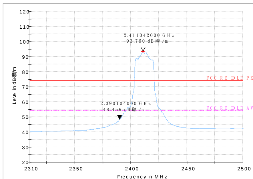
Fig 60. Bandedge: 802.11g, low channel
