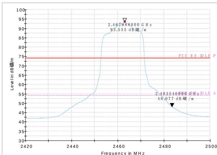
Fig 66. Bandedge: 802.11 n-20MHz, high channel
