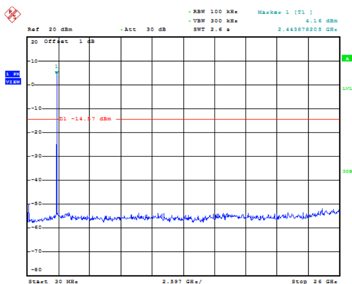
Fig 44. Conducted Spurious Emission (802.11g, Ch11)
