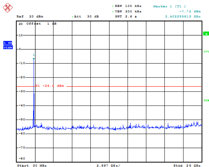
Fig 40. Conducted Spurious Emission (802.11g, Ch1)
