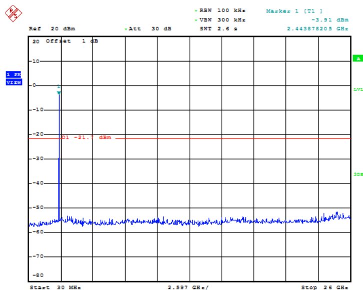
Fig 38. Conducted Spurious Emission (802.11b, Ch11)
