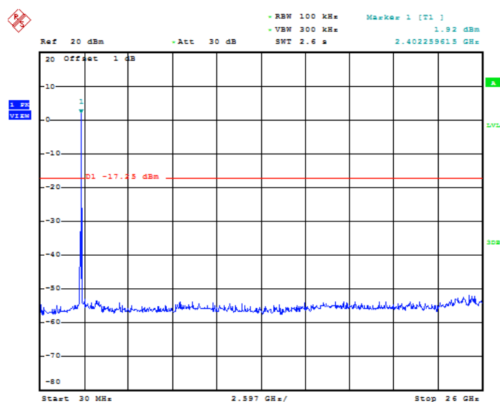
Fig 46. Conducted Spurious Emission (802.11n-20MHz, Ch1)
