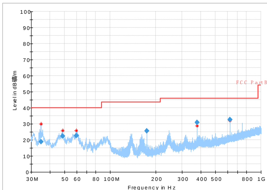
Fig 57. Radiated Spurious Emission (802.11b,Ch11,30MHz~1GHz)
