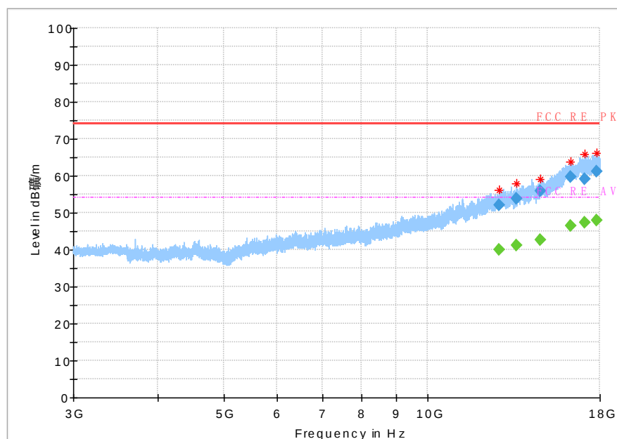
Fig 69. Radiated Spurious Emission (802.11 n-20MHz,Ch11, 3GHz~18GHz)
