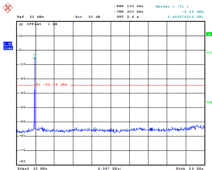
Fig 50. Conducted Spurious Emission (802.11n-20MHz, Ch11)
