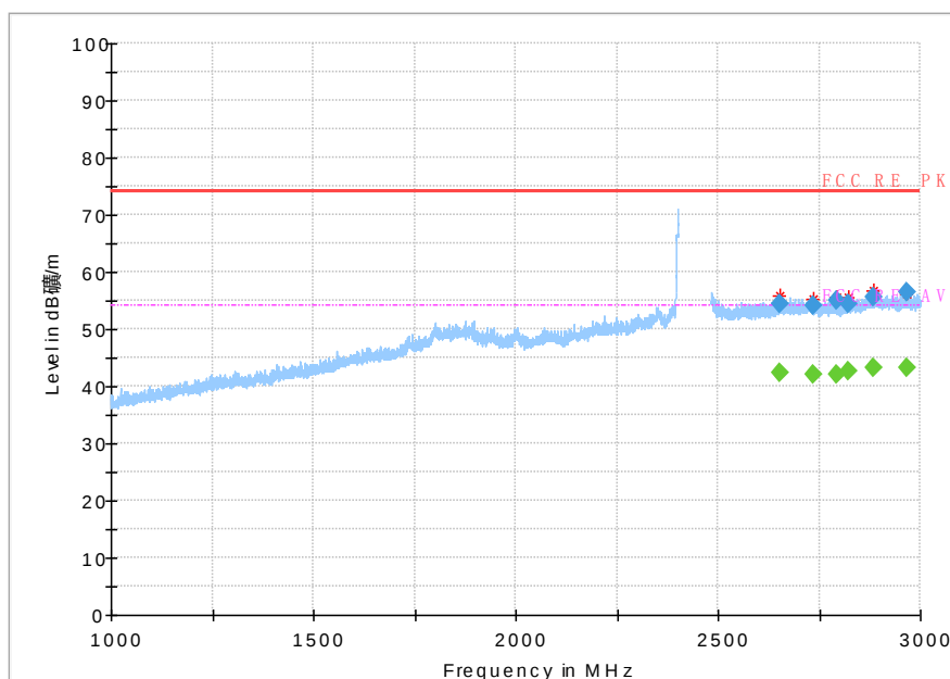
Fig 55. Radiated Spurious Emission (802.11b,Ch1,1GHz~3GHz)
