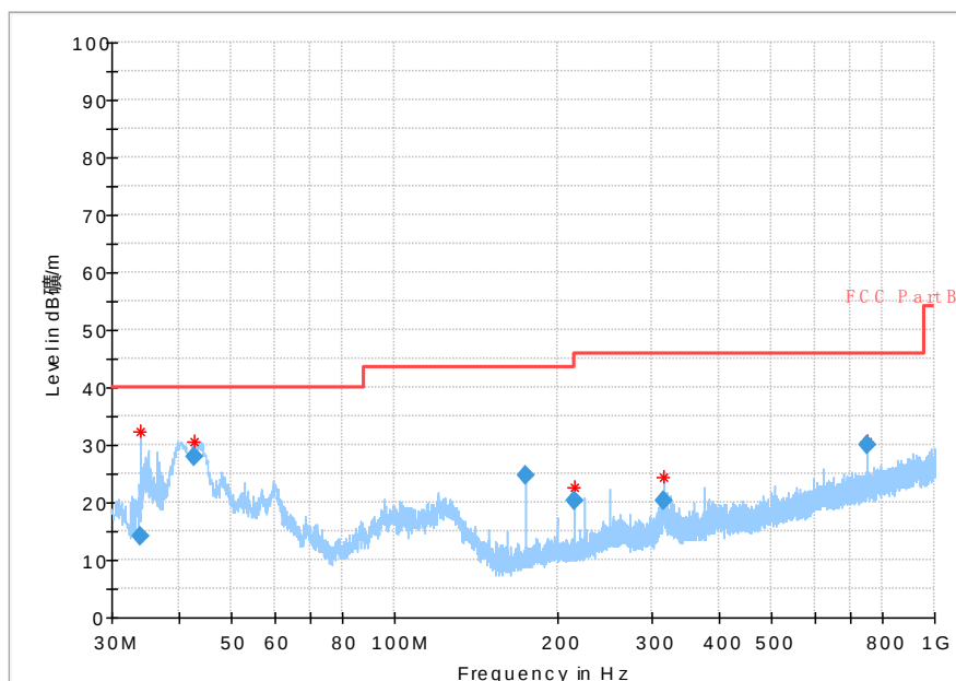
Fig 54. Radiated Spurious Emission (802.11b,Ch1,30MHz~1GHz)
