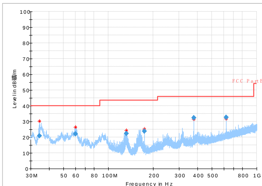
Fig 62. Radiated Spurious Emission (802.11g,Ch11, 30MHz~1GHz)
