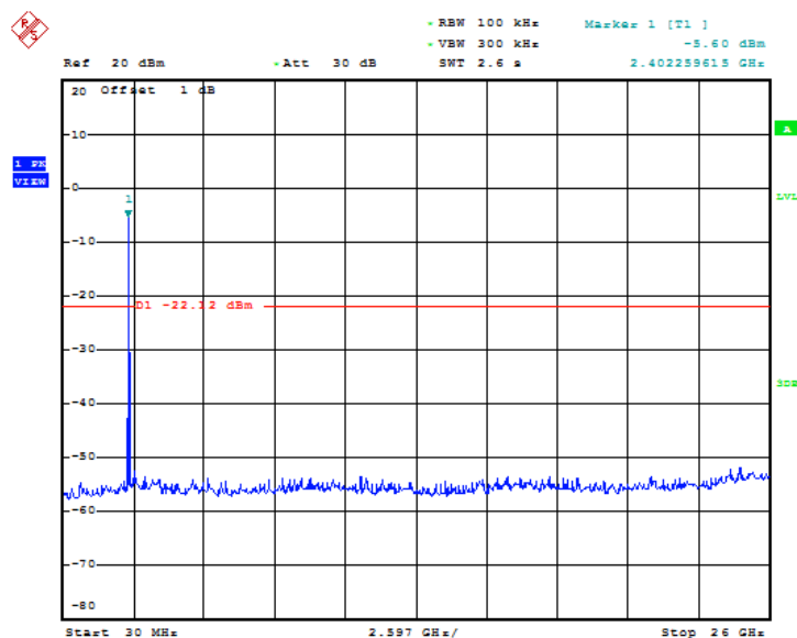
Fig 34. Conducted Spurious Emission (802.11b, Ch1)
