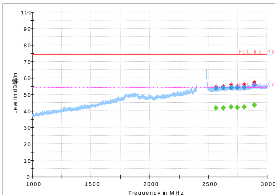
Fig 68. Radiated Spurious Emission (802.11 n-20MHz,Ch11, 1GHz~3GHz)
