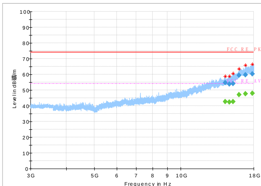
Fig 56. Radiated Spurious Emission (802.11b,Ch1,3GHz~18GHz)
