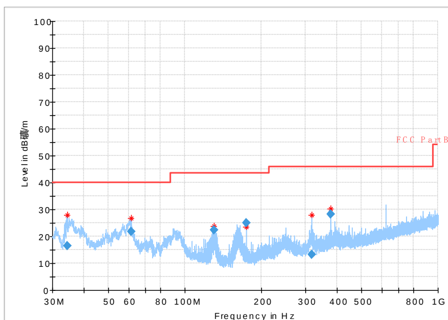
Fig 67. Radiated Spurious Emission (802.11 n-20MHz,Ch11,30MHz~1GHz)
