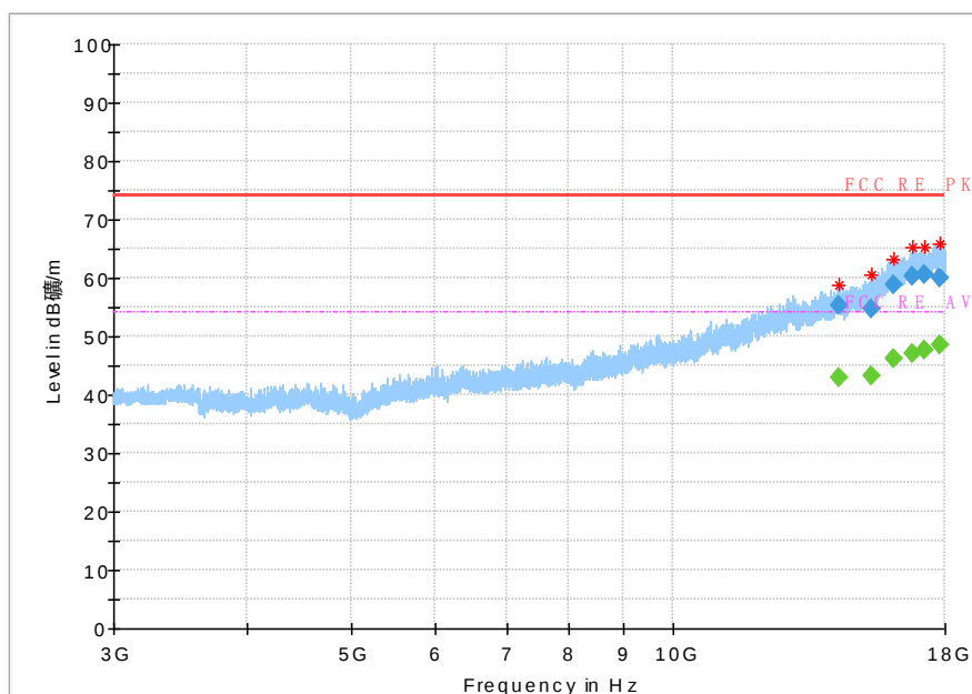
Fig 59. Radiated Spurious Emission (802.11b,Ch11,3GHz~18GHz)
