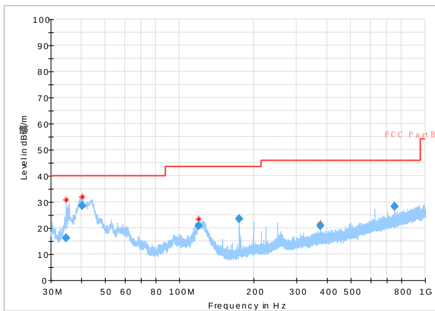
Fig. 31 Radiated Spurious Emission (802.11a, ch36, 30 MHz-1 GHz)
