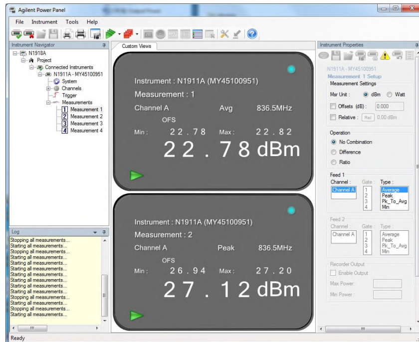
LTE Band 5/26 (824 – 849 MHz)_5M Bandwidth Middle Channel QPSK Full RB
