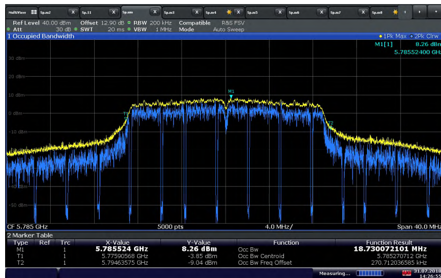
802.11ac (20 MHz BW) U-NII 3 Middle Channel
