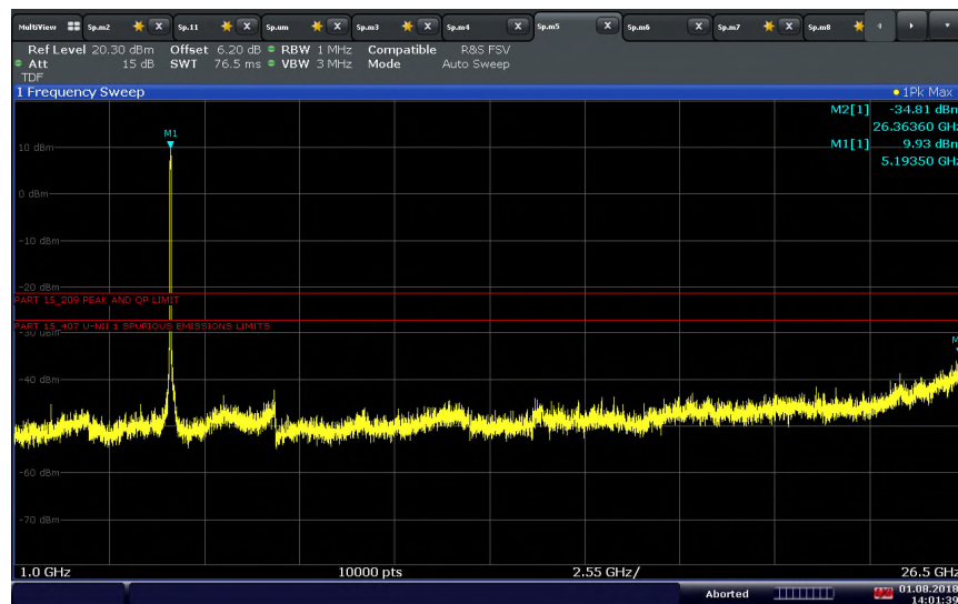
802.11 n (40 MHz) U-NII 1 Low Channel above 1GHz
