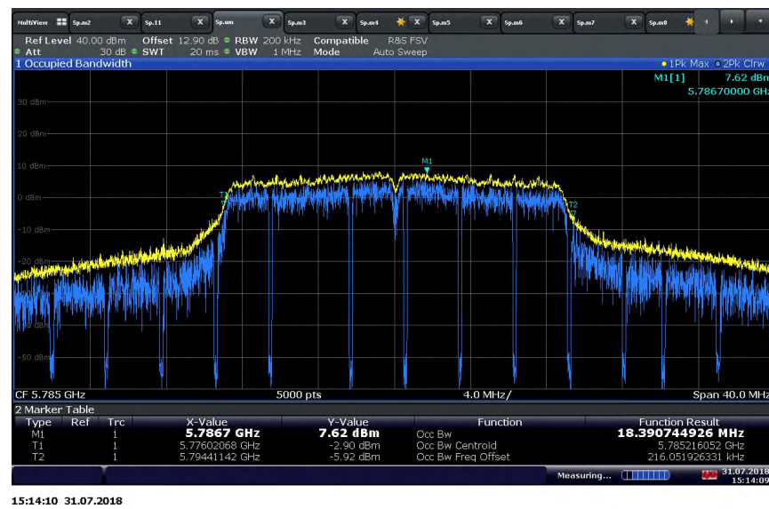
802.11n (20 MHz BW) U-NII 3 Middle Channel
