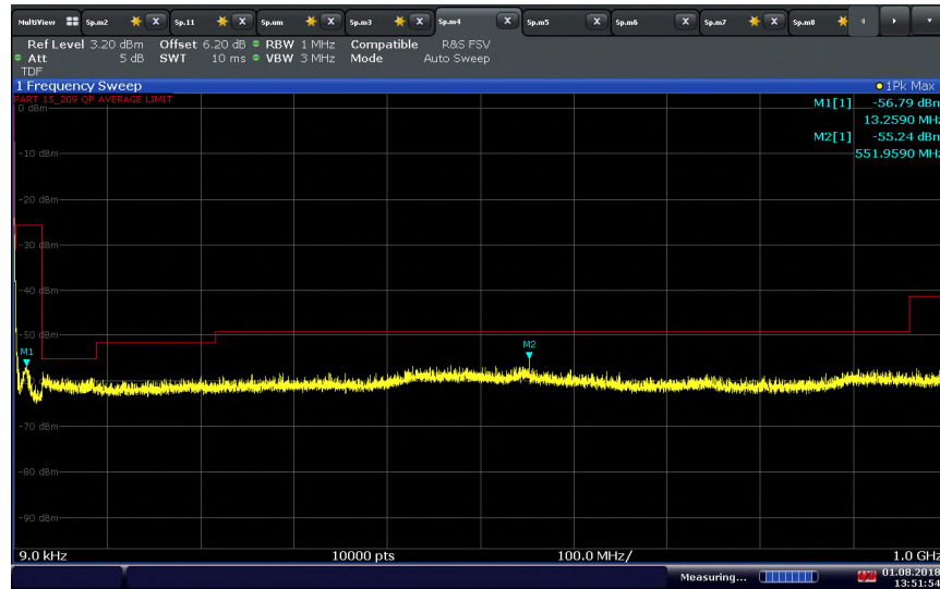
802.11 a U-NII 1 Middle Channel below 1GHz
