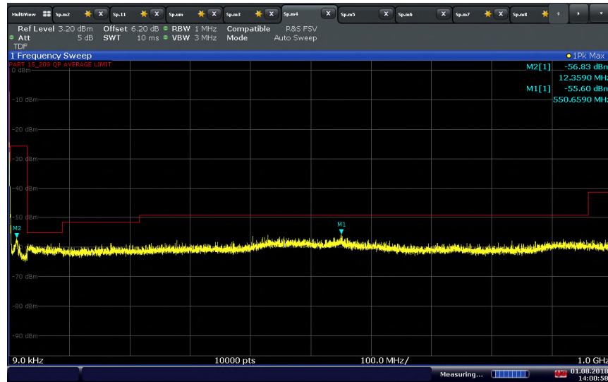
802.11 n (40 MHz) U-NII 1 Low Channel below 1GHz
