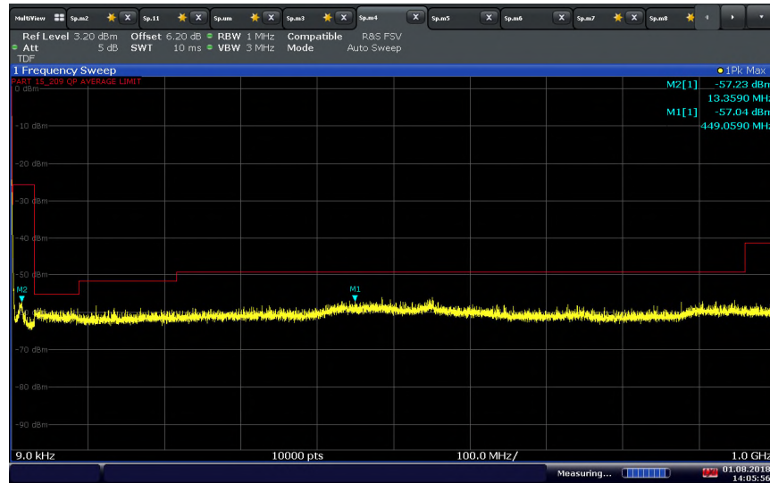
802.11 ac (20 MHz) U-NII 1 Low Channel below 1GHz
