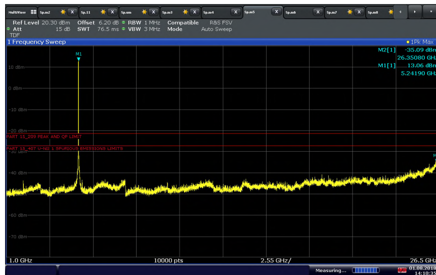
802.11 ac (20 MHz) U-NII 1 High Channel above 1GHz
