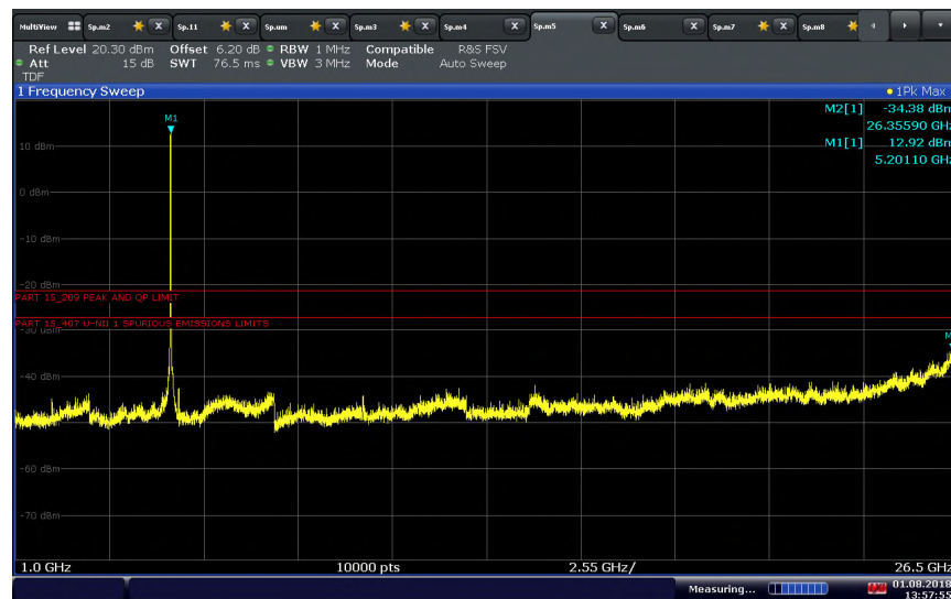
802.11 n (20 MHz) U-NII 1 Middle Channel above 1GHz
