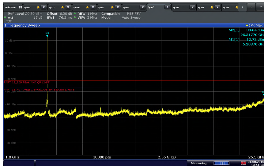
802.11a U-NII 1 Middle Channel above 1GHz
