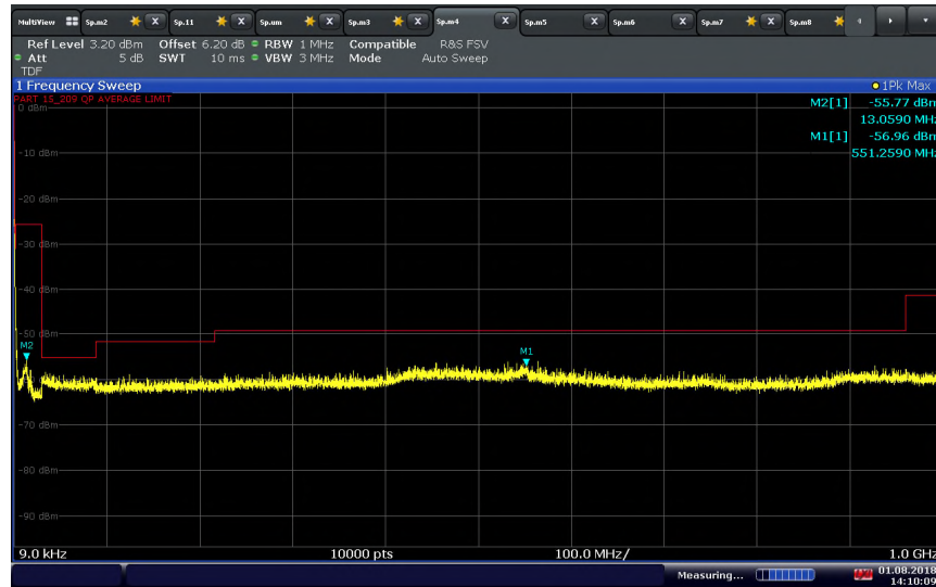
802.11 ac (20 MHz) U-NII 1 High Channel below 1GHz
