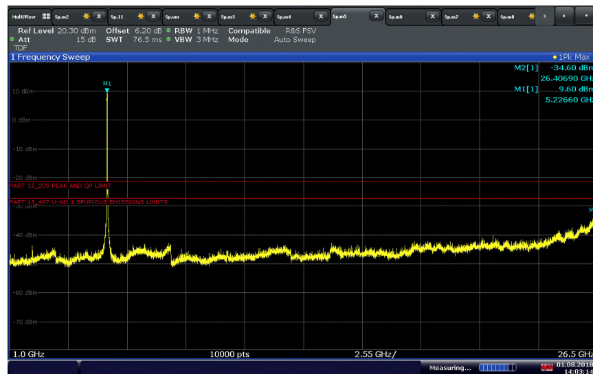
802.11 n (40 MHz) U-NII 1 High Channel above 1GHz
