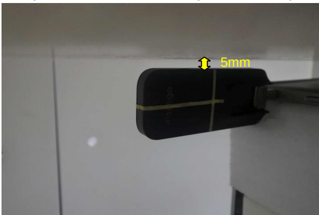
USB Cable Plug-in USB Configuration 4 (Vertical Back, Test Separation 5 mm)
