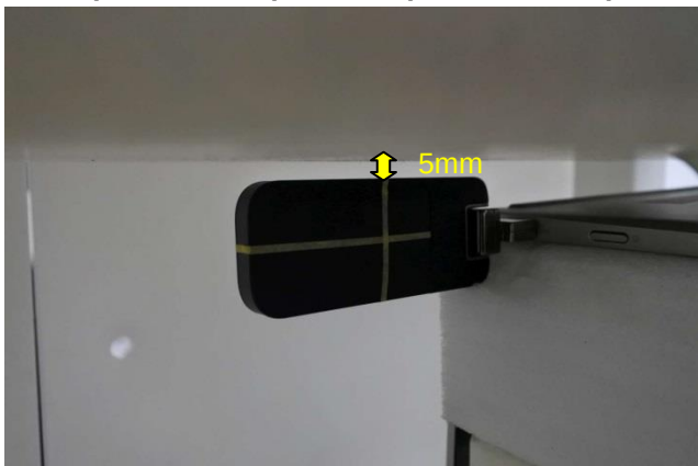
Direct Laptop Plug-in for USB Configuration 3 (Vertical Front, Test Separation 5 mm)
