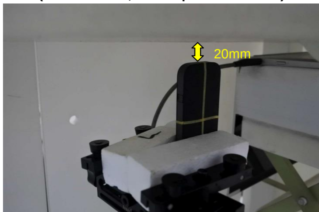
USB Cable Plug-in for USB Configuration 5 (Tip Mode, Test Separation 20 mm)
