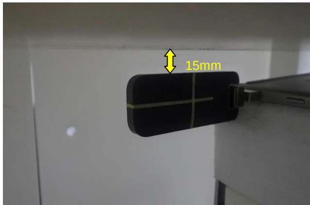
Direct Laptop Plug-in for USB Configuration 3 (Vertical Front, Test Separation 15 mm)
