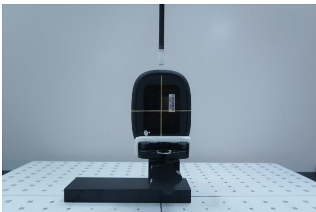
Left Side, Probe sensor to EUT surface distance 10mm
