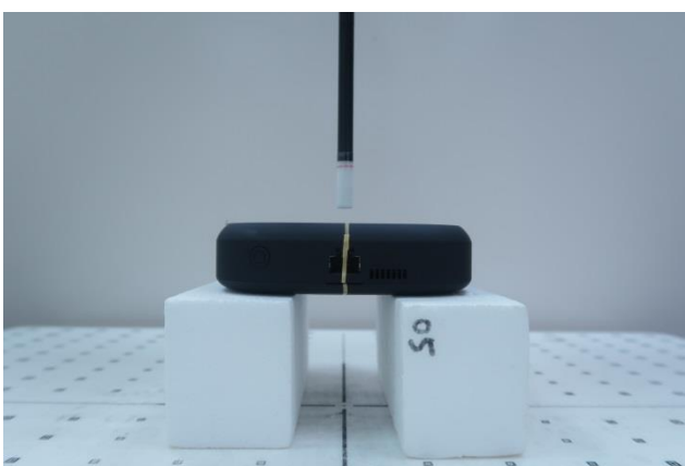
Top Side, Probe sensor to EUT surface distance 10mm
