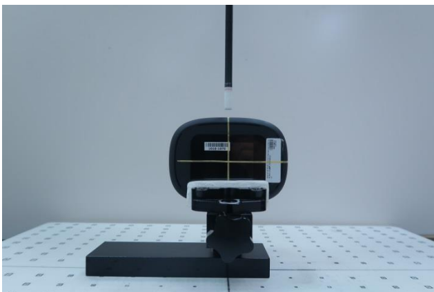
Back, Probe sensor to EUT surface distance 10mm
