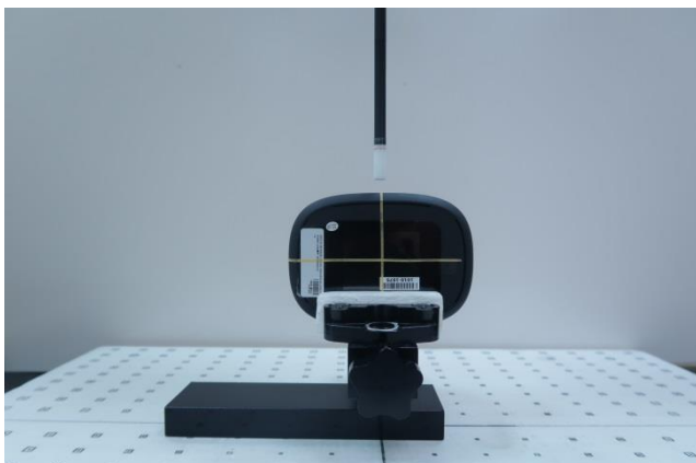
Front, Probe sensor to EUT surface distance 10mm
