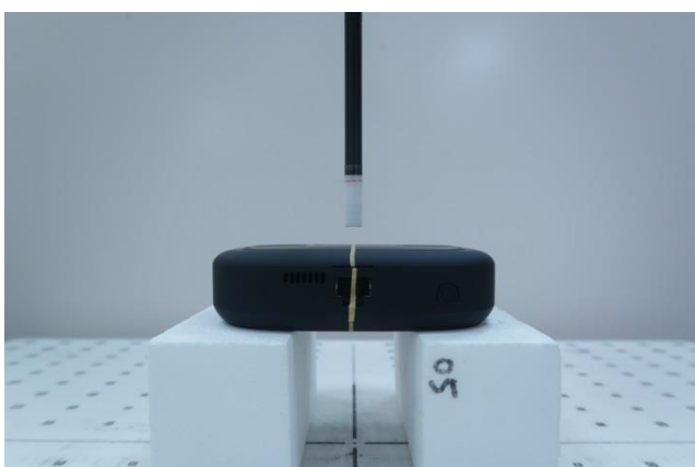
Bottom Side, Probe sensor to EUT surface distance 10mm
