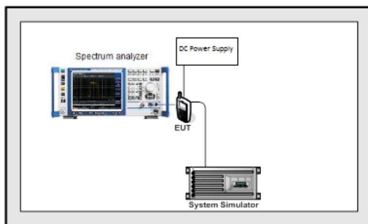
Conducted Setup
