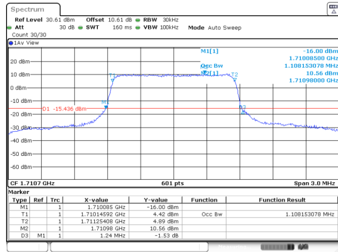
Band66-1.4MHz-QPSK-131979-6RB#0-1.108
