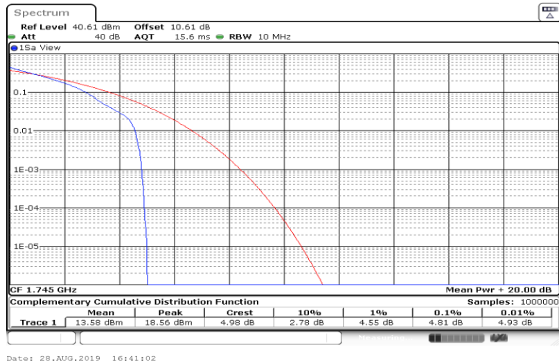
Band66-20MHz-QPSK-132322-100RB#0
