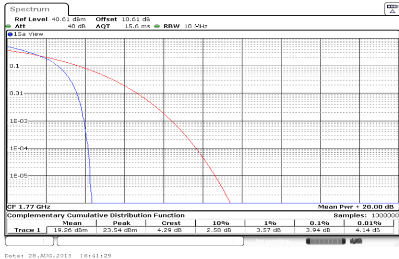
Band66-20MHz-16QAM-132072-1RB#0
