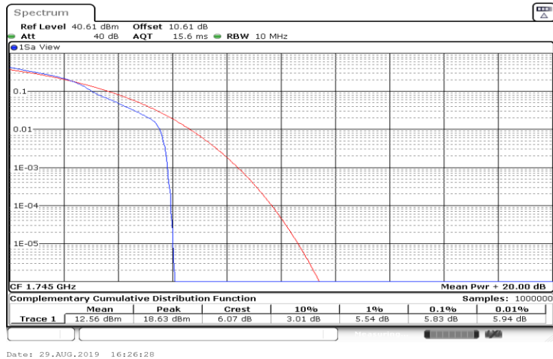
Band66-20MHz-16QAM-132322-100RB#0
