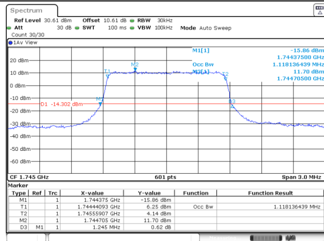
Band66-1.4MHz-QPSK-132322-6RB#0-1.118
