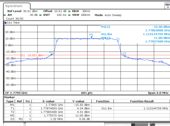
Band66-1.4MHz-QPSK-132665-6RB#0-1.113
