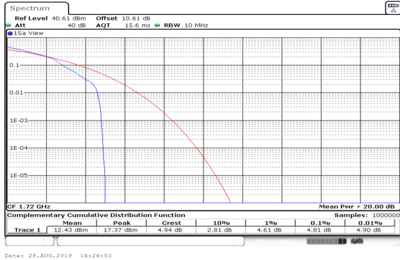
Band66-20MHz-16QAM-132072-100RB#0
