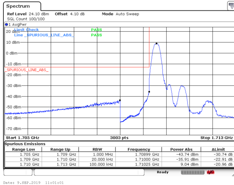
Band66-1.4MHz-QPSK-131979-6RB#0
