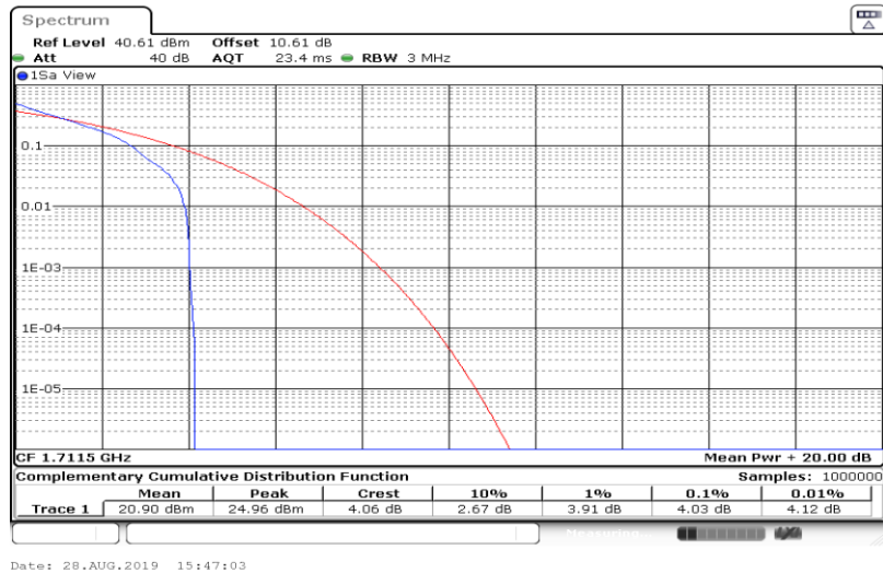
Band66-3MHz-QPSK-131987-15RB#0
