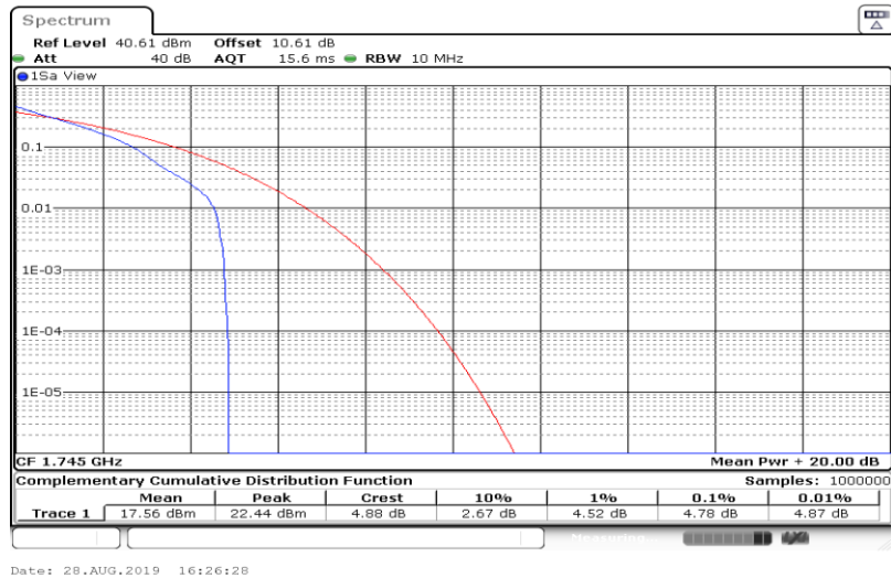
Band66-15MHz-QPSK-132322-75RB#0
