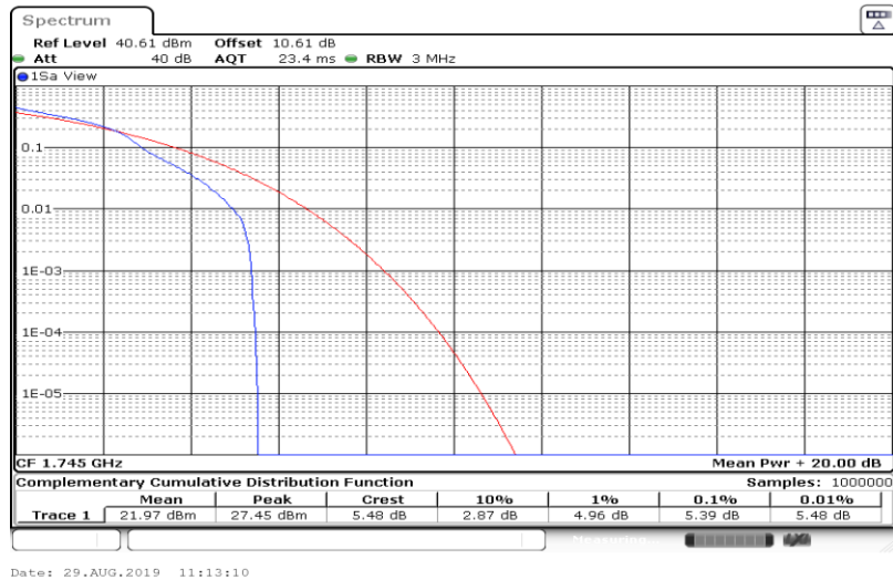
Band66-1.4MHz-16QAM-132322-6RB#0
