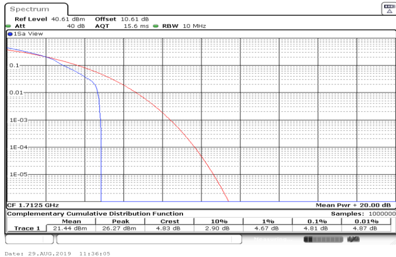
Band66-5MHz-16QAM-131997-25RB#0
