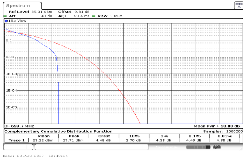
Band12-1.4MHz-QPSK-23017-6RB#0
