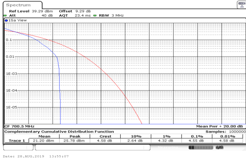
Band12-3MHz-QPSK-23025-15RB#0
