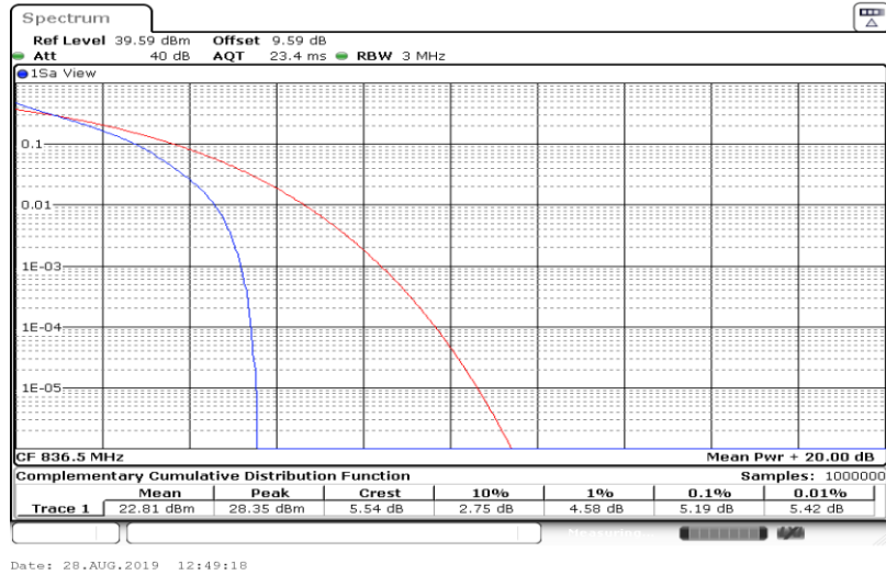
Band5-1.4MHz-QPSK-20643-1RB#0
