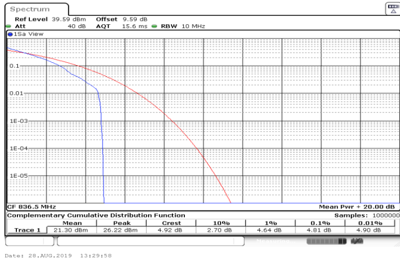
Band5-10MHz-QPSK-20525-50RB#0
