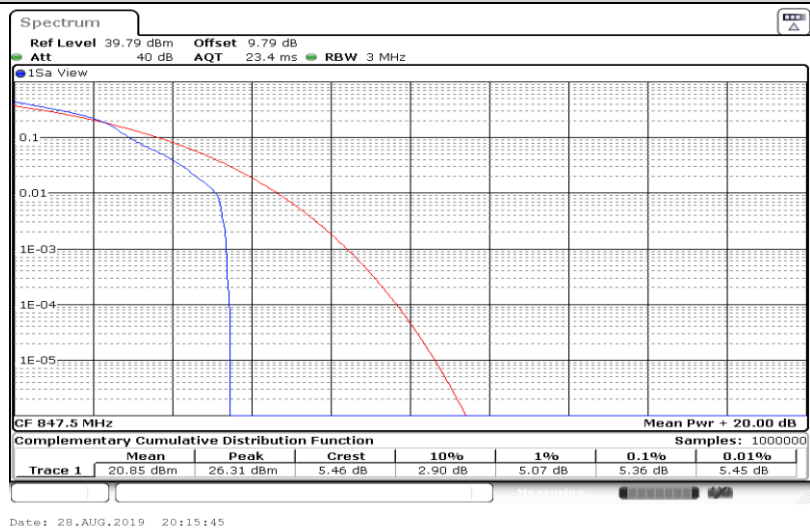
Band5-3MHz-16QAM-20635-15RB#0
