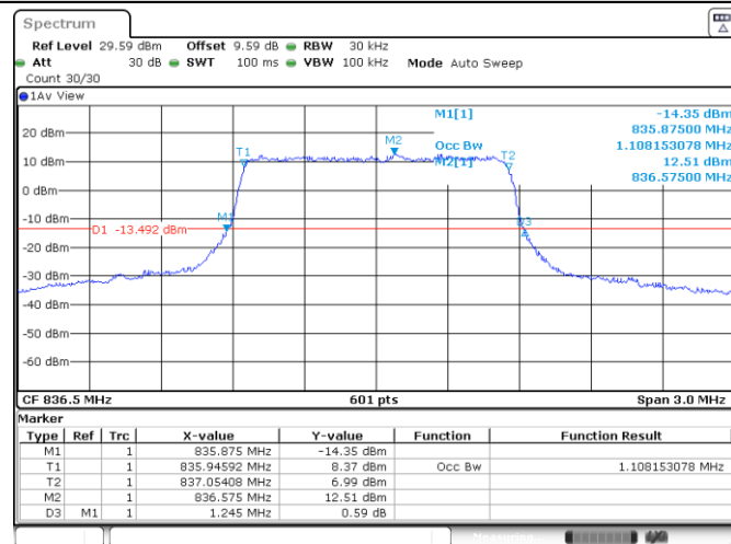
Band5-1.4MHz-QPSK-20525-6RB#0-1.108
