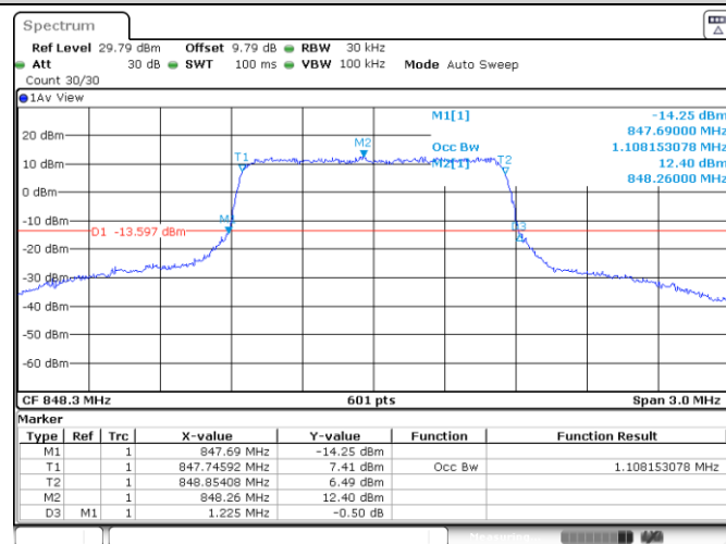
Band5-1.4MHz-QPSK-20643-6RB#0-1.108
