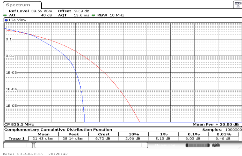
Band5-5MHz-16QAM-20625-1RB#0
