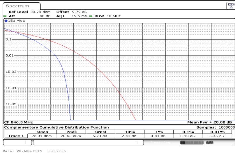
Band5-5MHz-16QAM-20425-1RB#0
