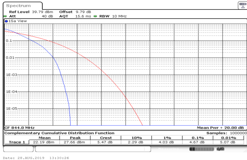
Band5-10MHz-16QAM-20450-1RB#0
