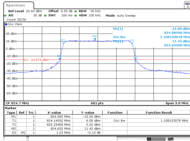
Band5-1.4MHz-QPSK-20407-6RB#0-1.108
