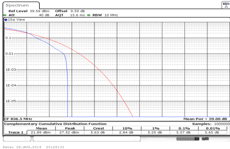
Band5-5MHz-16QAM-20525-25RB#0
