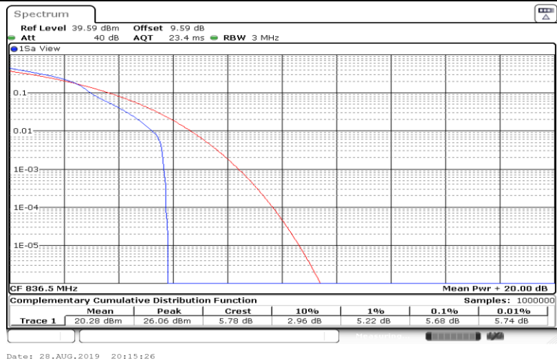
Band5-3MHz-16QAM-20525-15RB#0
