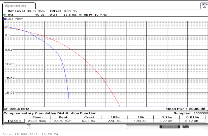
Band5-5MHz-16QAM-20525-1RB#0
