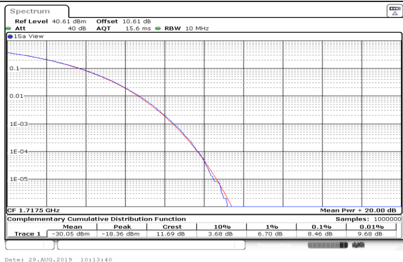
Band4-15MHz-16QAM-20175-1RB#0
