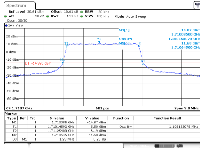
Band4-1.4MHz-QPSK-19957-6RB#0-1.108
