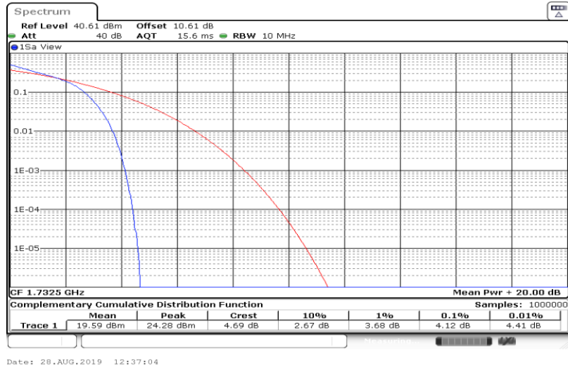
Band4-20MHz-QPSK-20300-1RB#0
