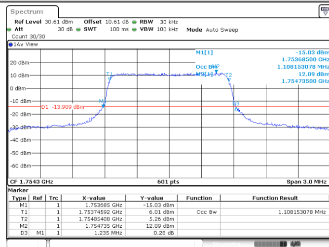
Band4-1.4MHz-QPSK-20393-6RB#0-1.108
