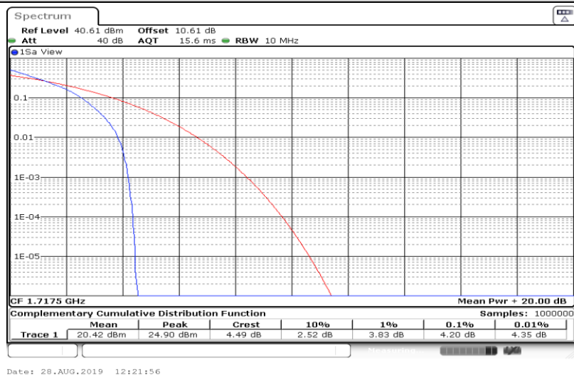
Band4-15MHz-QPSK-20175-1RB#0
