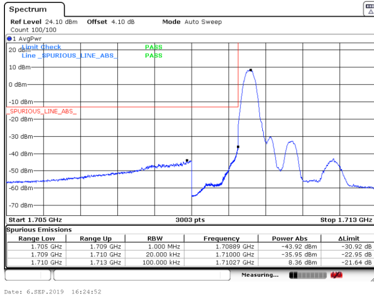
Band4-1.4MHz-QPSK-19957-6RB#0
