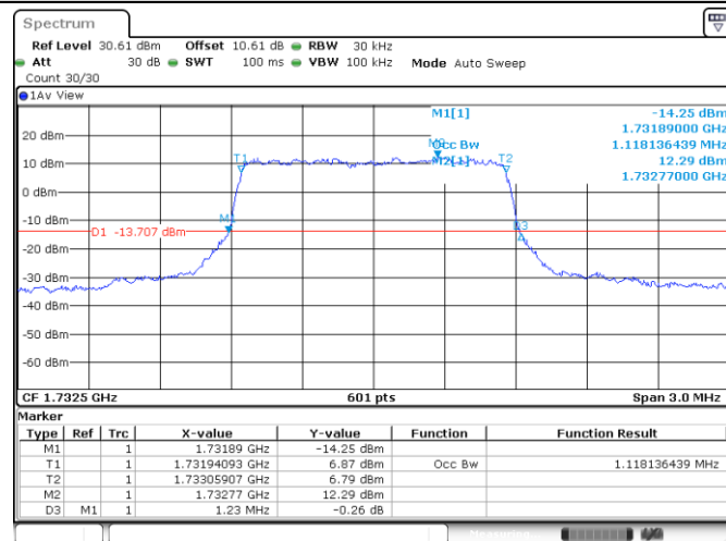
Band4-1.4MHz-QPSK-20175-6RB#0-1.118
