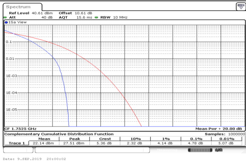
Band4-5MHz-QPSK-20375-25RB#0
