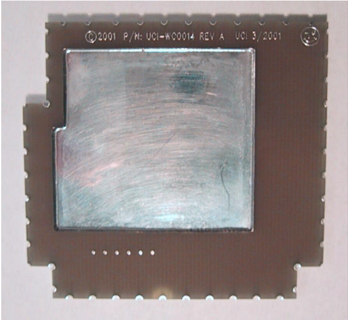
Figure 1 - Bottom View. Bottom Layer Material: FR4
