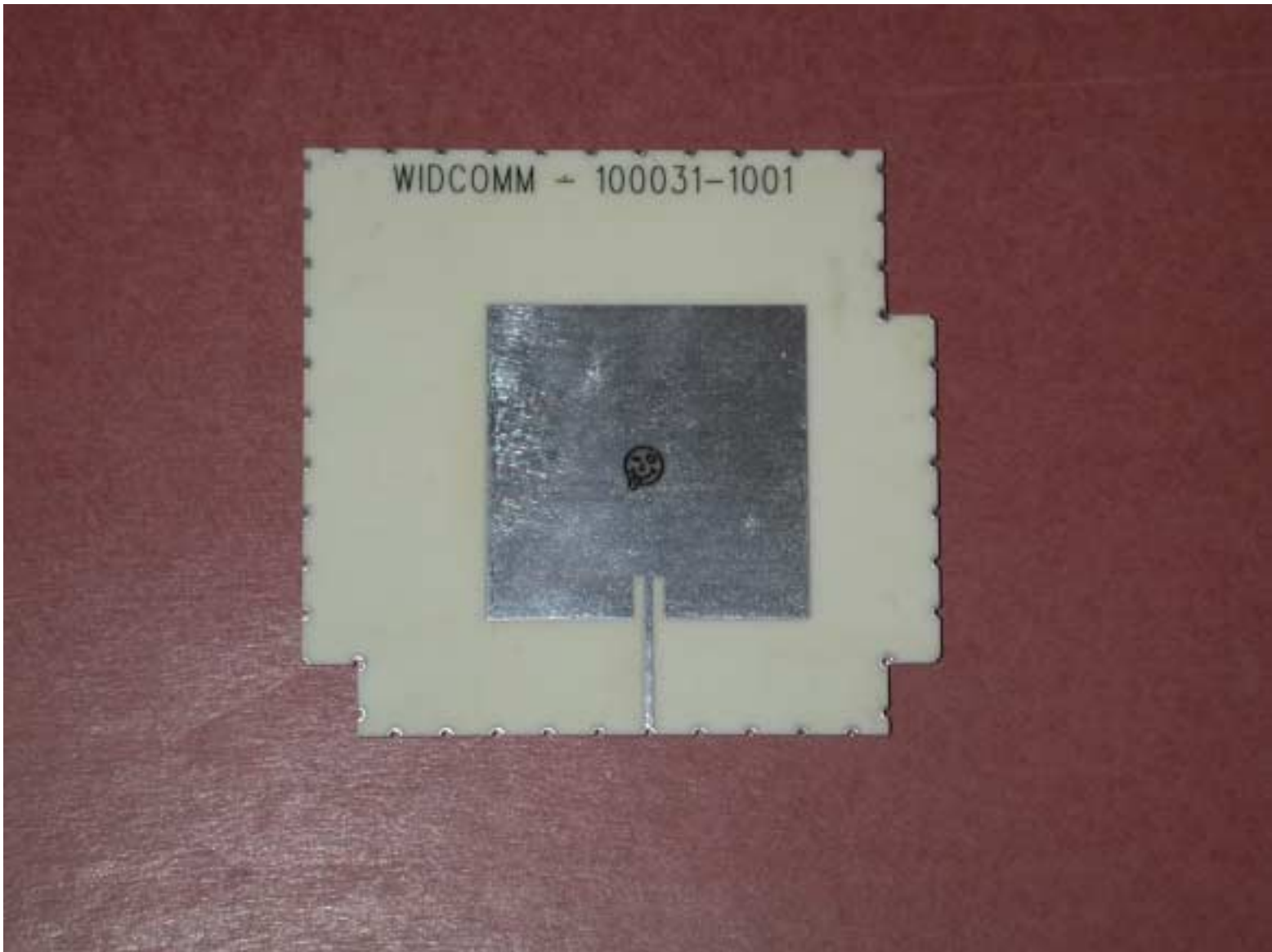
WIDCOMM PCB PATCH ANTENNA TOP ASSY
