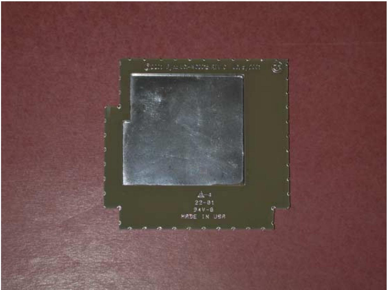
WIDCOMM PCB PATCH ANTENNA BOTTOM
