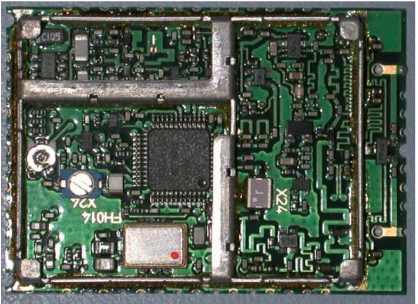
ALPS RF MODULE NO SHIELD TOP
