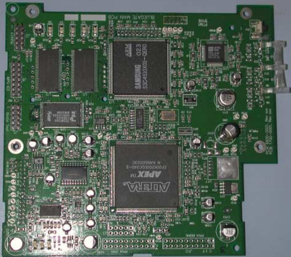
MAIN PCB NO SHIELD TOP
