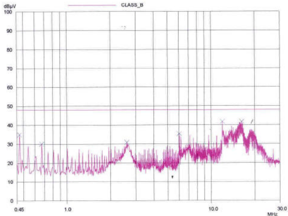
HOT LINE
