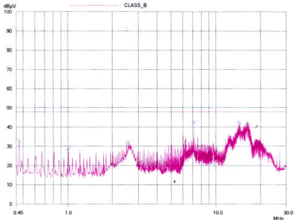
NEUTRAL LINE
