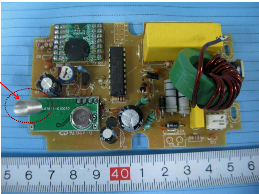
EUT – Main Board Components View
