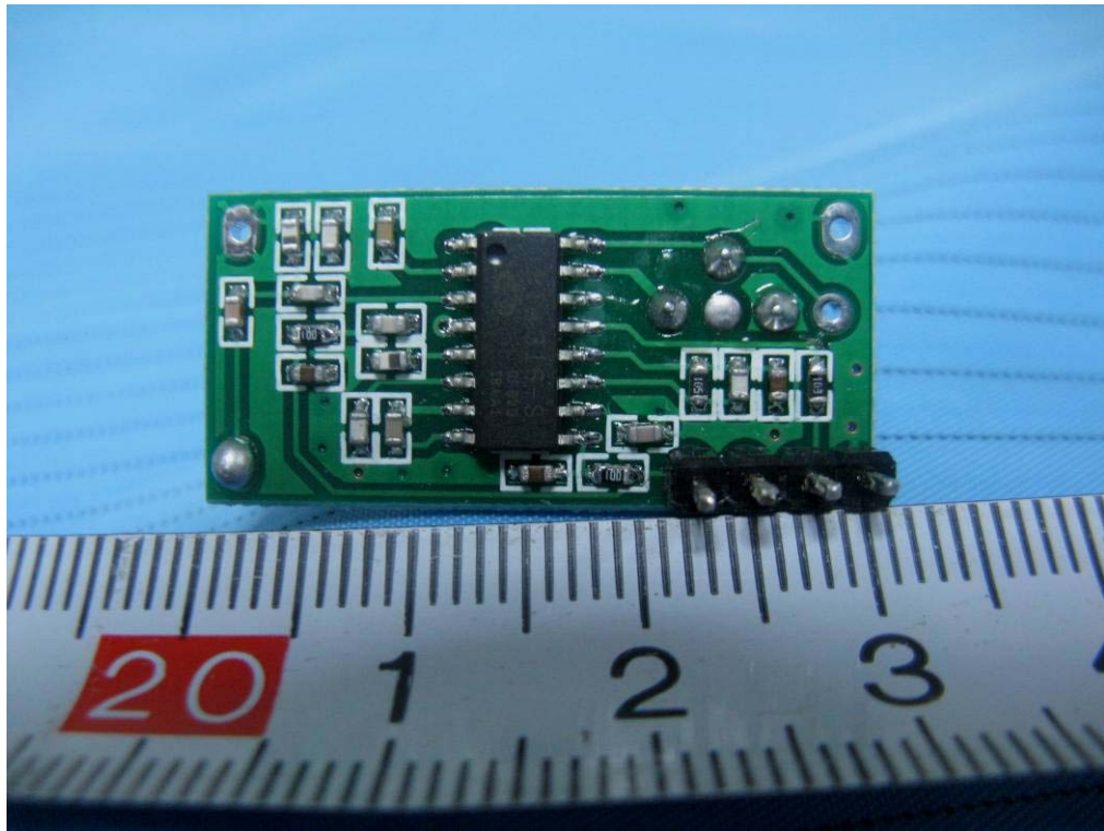
EUT – Receiver Board Bottom Components View
