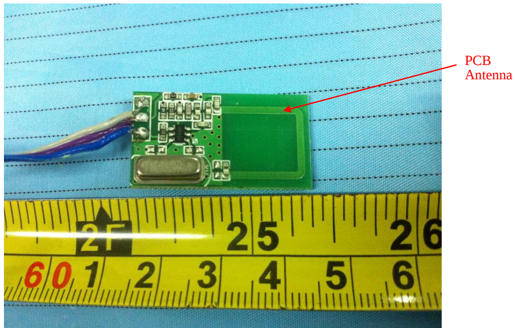
EUT – RF Board Top View
