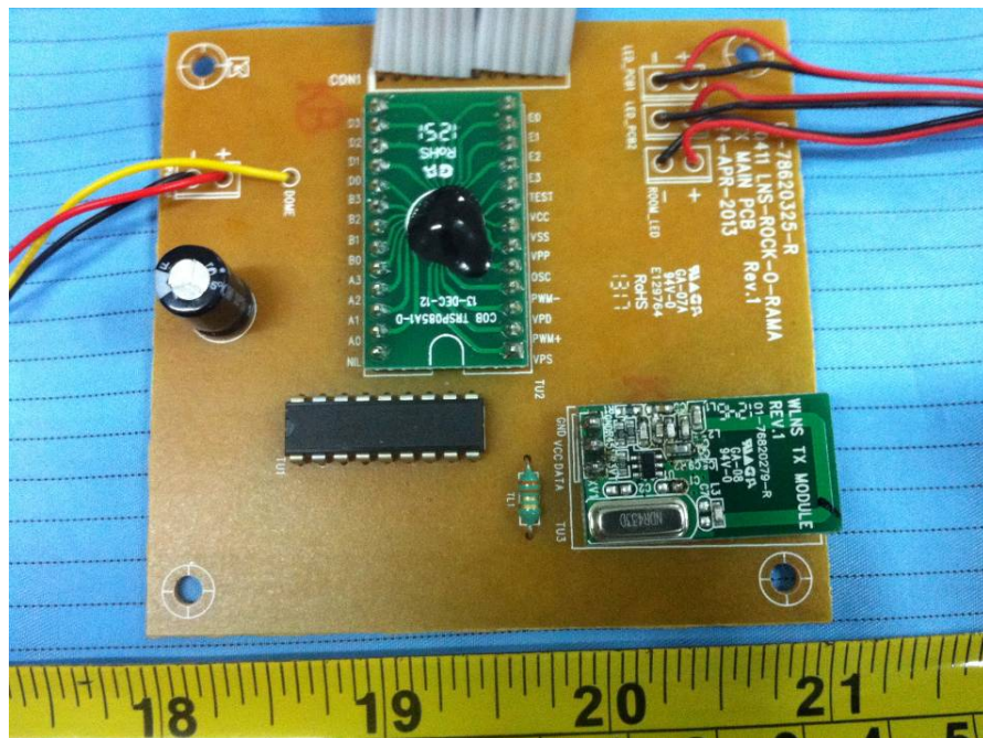
EUT – Main Board Full View
