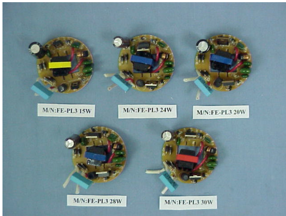
Figure 14. Self-Ballasted Lamp (M/N: FE-PL3 Series) Main Board (Component Side)
