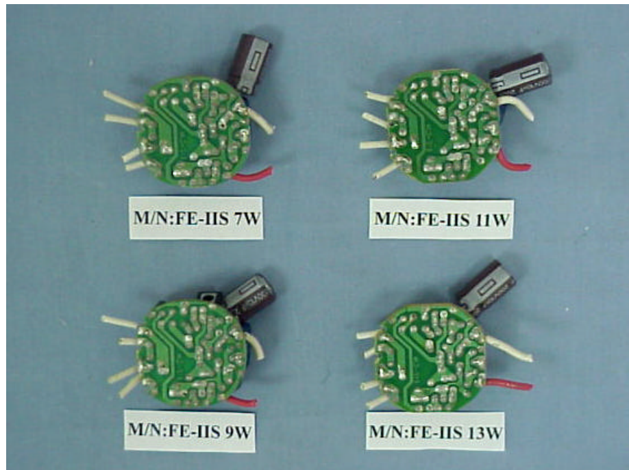
Figure 12. Self-Ballasted Lamp (M/N: FE-IIS Series) Main Board (Soldered Side)
