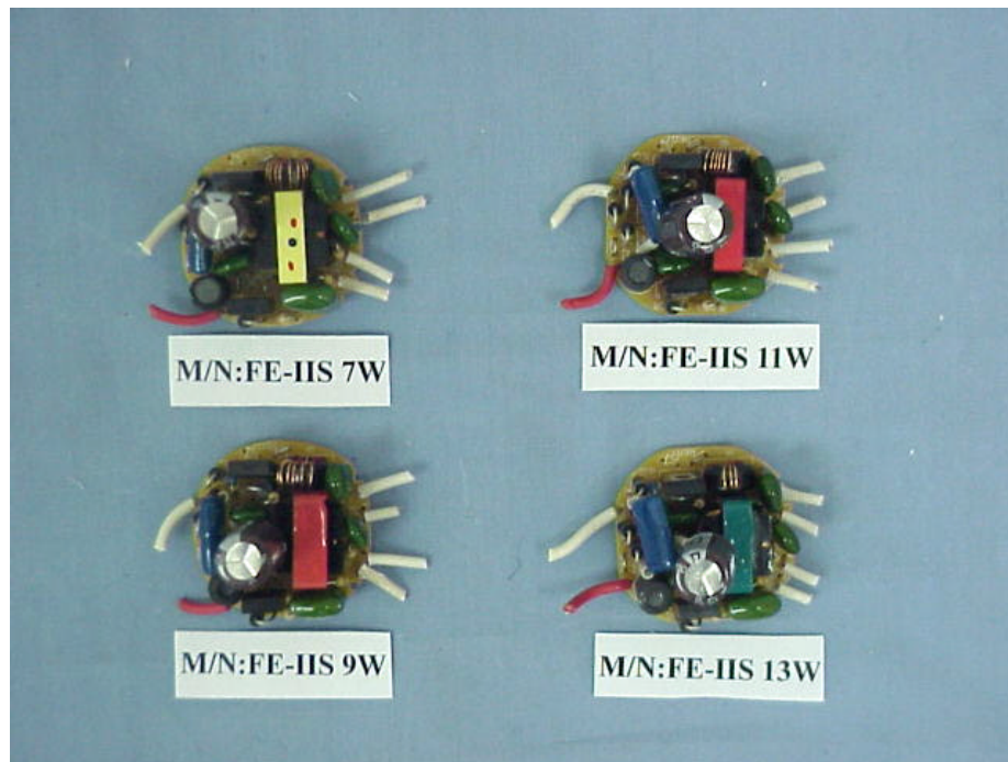
Figure 11. Self-Ballasted Lamp (M/N: FE-IIS Series) Main Board (Component Side)
