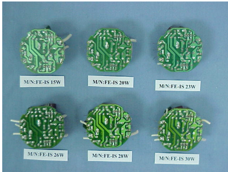
Figure 9. Self-Ballasted Lamp (M/N: FE-IS Series) Main Board (Soldered Side)
