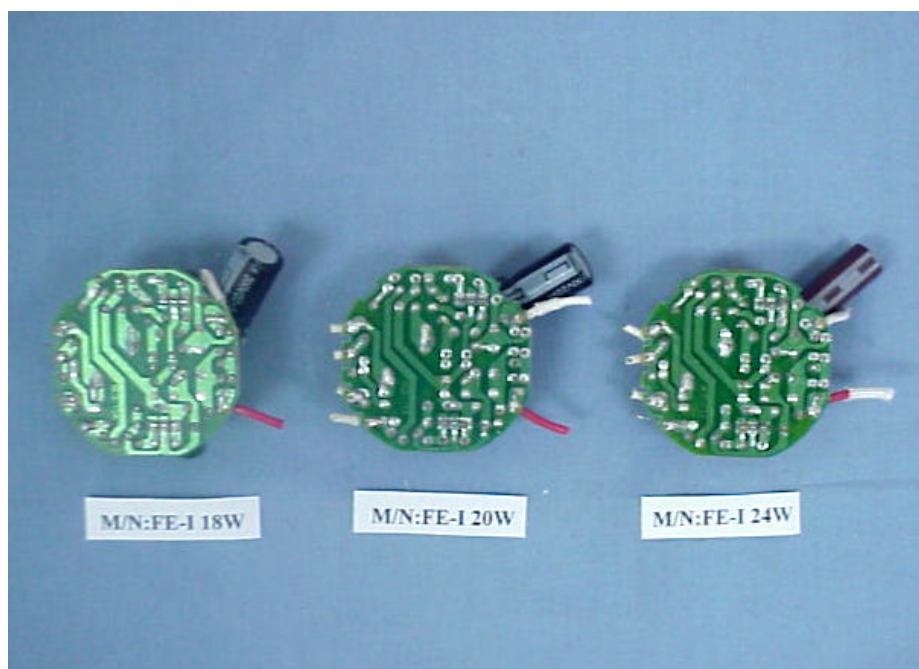
Figure 3. Self-Ballasted Lamp (M/N: FE-I Series) Main Board (Soldered Side)
