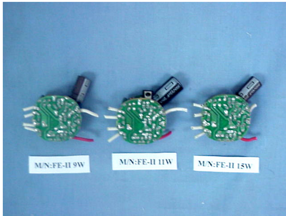
Figure 6. Self-Ballasted Lamp (M/N: FE-II Series) Main Board (Soldered Side)
