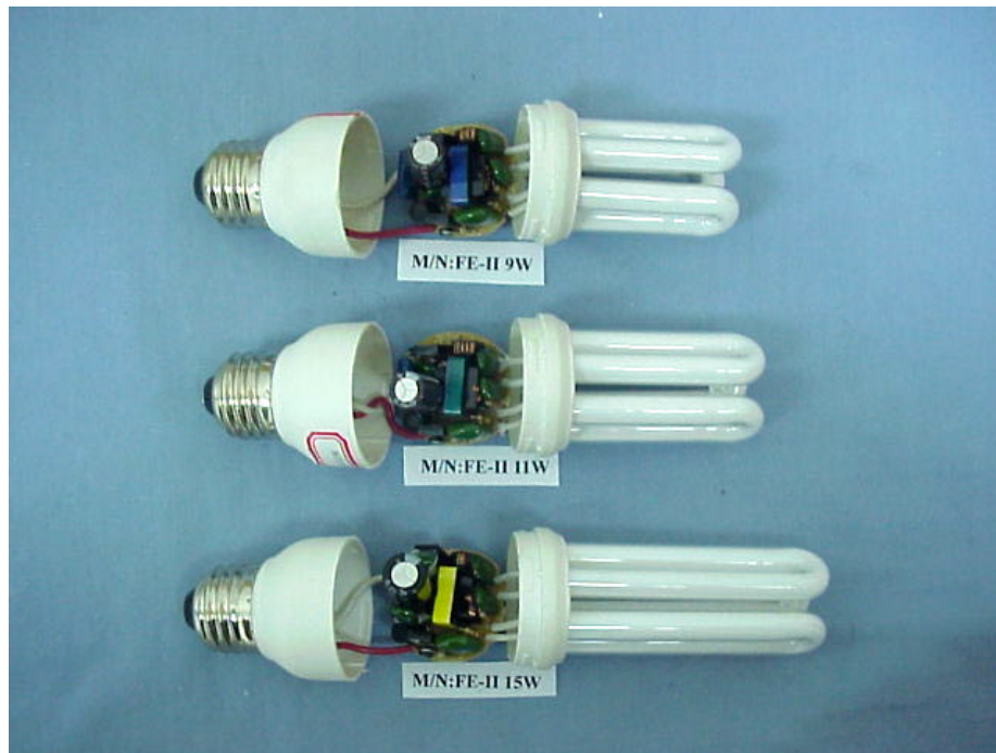
Figure 4. Self-Ballasted Lamp (M/N: FE-II Series) Cover Removed
