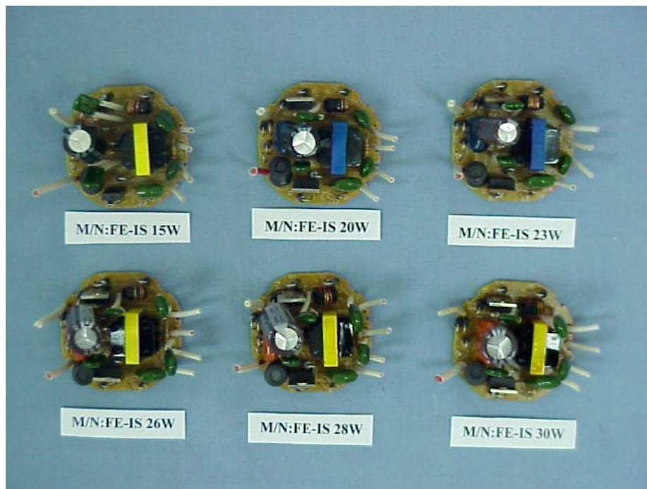
Figure 8. Self-Ballasted Lamp (M/N: FE-IS Series) Main Board (Component Side)
