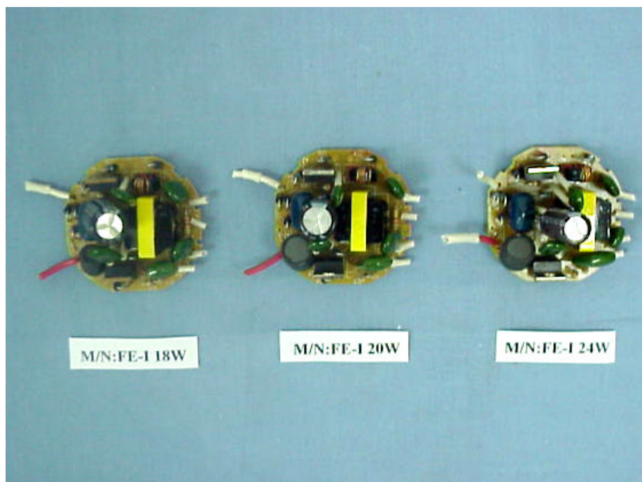
Figure 2. Self-Ballasted Lamp (M/N: FE-I Series) Main Board (Component Side)
