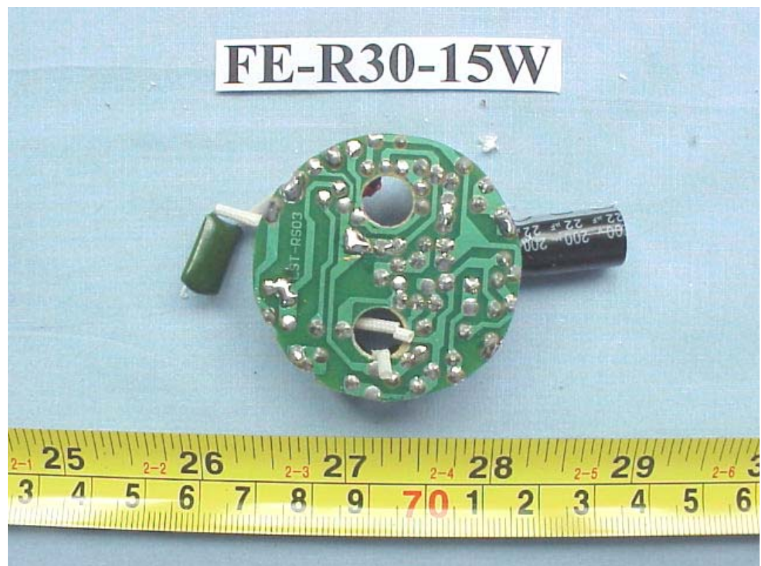
FIGURE 12 ENERGY SAVING LAMP (M/N: FE-R30-15W) MAIN BOARD (SOLDERED SIDE)
