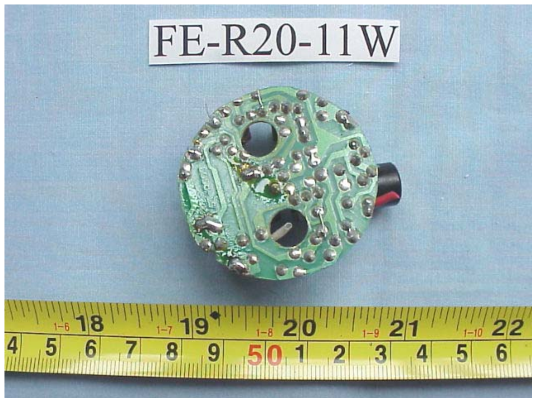
FIGURE 4 ENERGY SAVING LAMP (M/N: FE-R20-11W) MAIN BOARD (SOLDERED SIDE)
