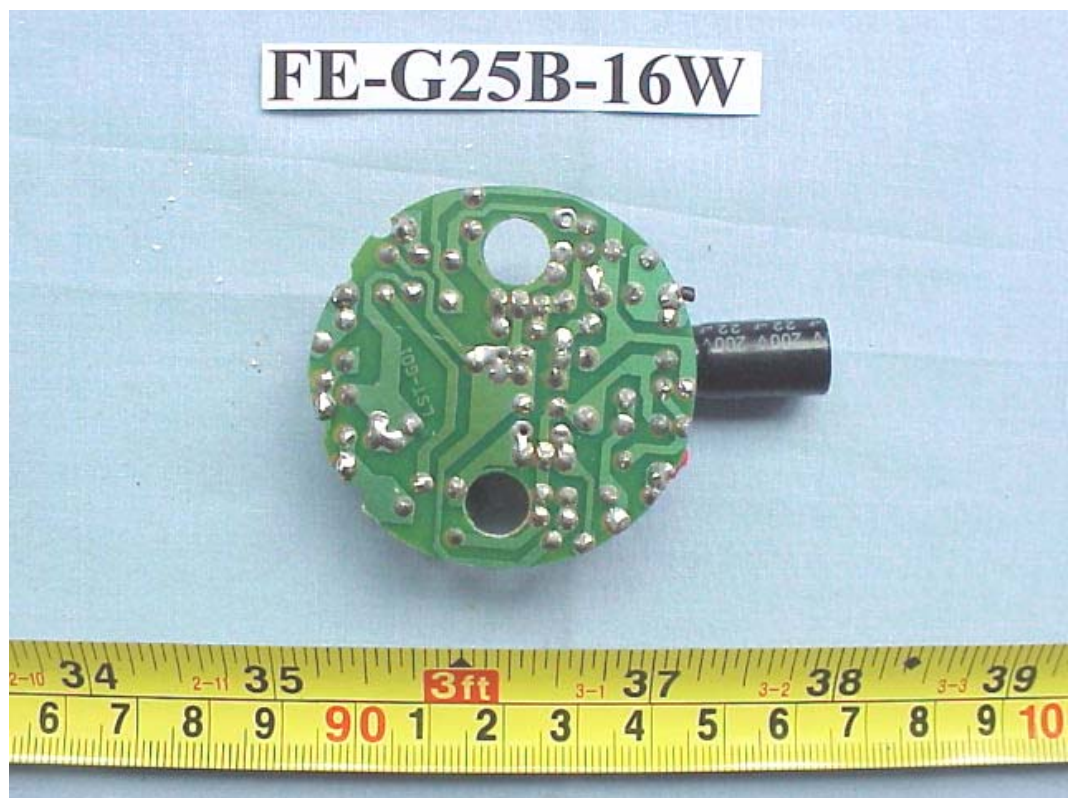
FIGURE 28 ENERGY SAVING LAMP (M/N: FE-G25B-16W) MAIN BOARD (SOLDERED SIDE)
