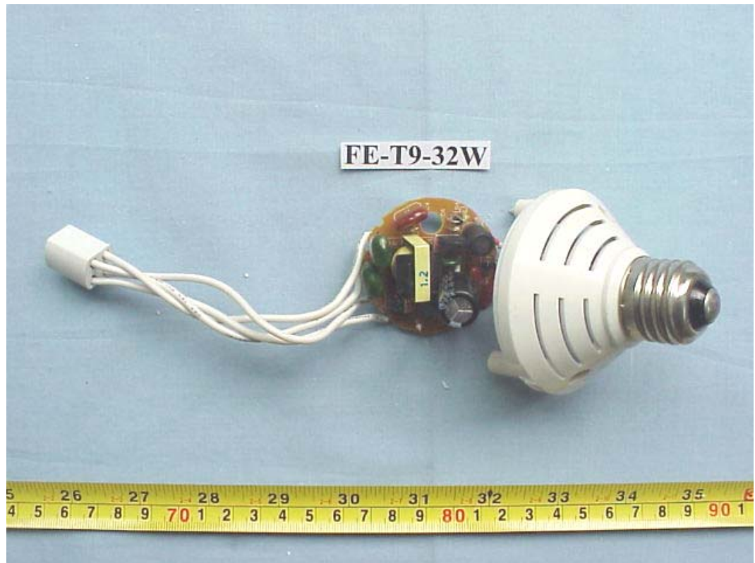
FIGURE 45 ENERGY SAVING LAMP (M/N: FE-T9-32W) COVER REMOVED
