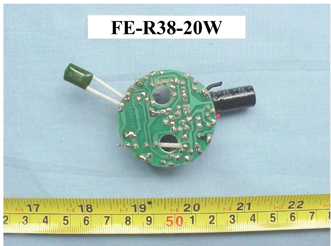
FIGURE 16 ENERGY SAVING LAMP (M/N: FE-R38-20W) MAIN BOARD (SOLDERED SIDE)
