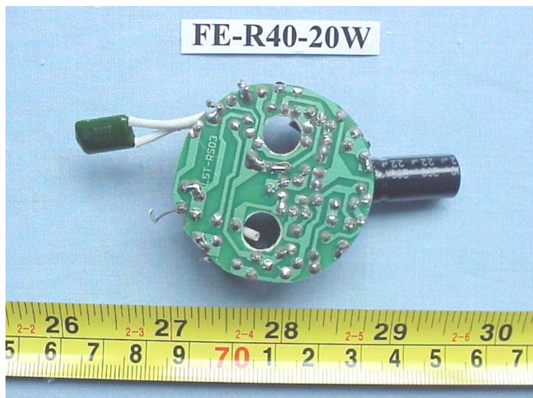
FIGURE 20 ENERGY SAVING LAMP (M/N: FE-R40-20W) MAIN BOARD (SOLDERED SIDE)
