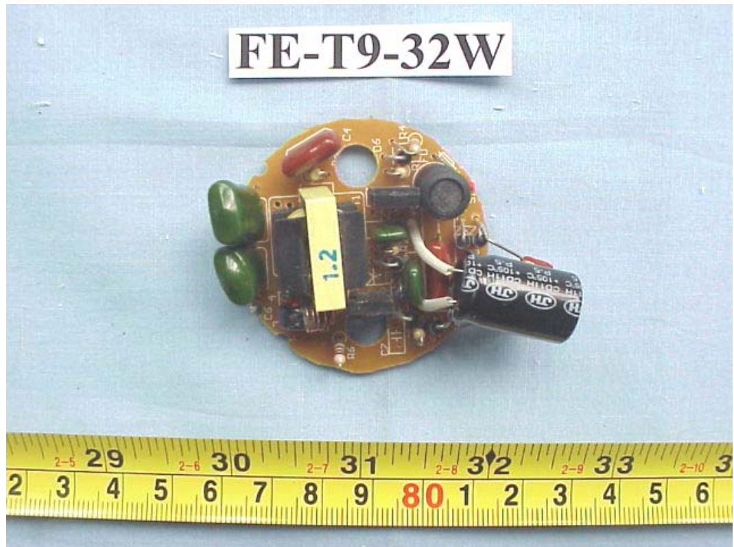
FIGURE 46 ENERGY SAVING LAMP (M/N: FE-T9-32W) MAIN BOARD (COMPONENT SIDE)
