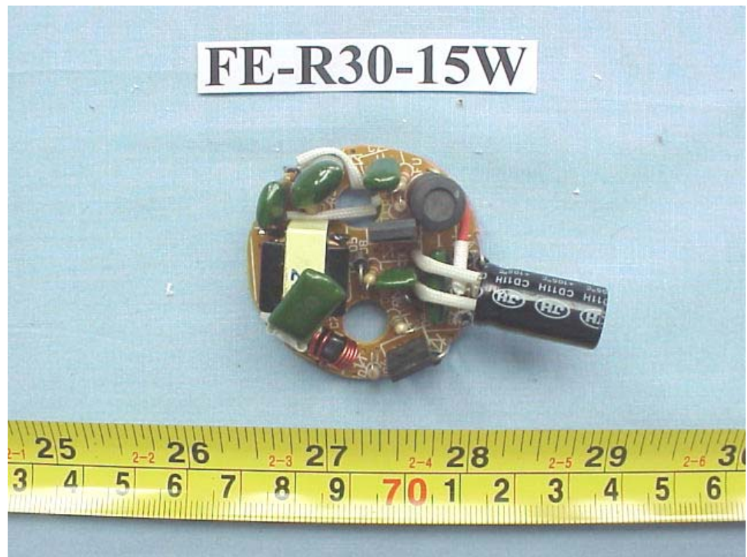
FIGURE 11 ENERGY SAVING LAMP (M/N: FE-R30-15W) MAIN BOARD (COMPONENT SIDE)
