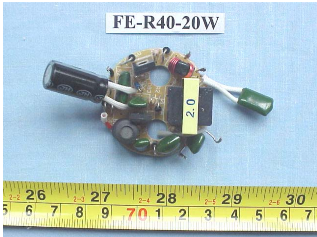
FIGURE 19 ENERGY SAVING LAMP (M/N: FE-R40-20W) MAIN BOARD (COMPONENT SIDE)
