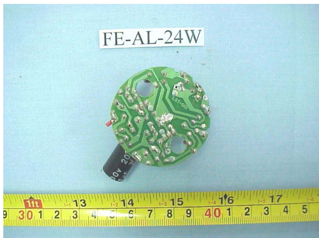
FIGURE 44 ENERGY SAVING LAMP (M/N: FE-AL-24W) MAIN BOARD (SOLDERED SIDE)
