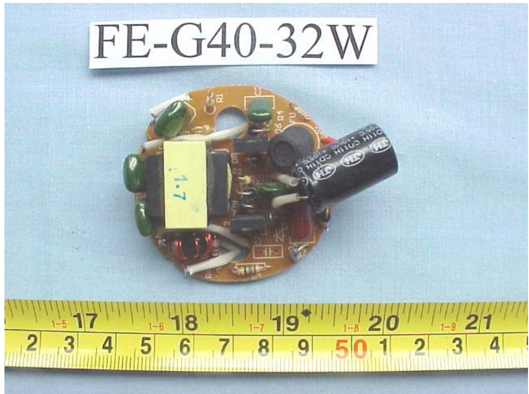
FIGURE 39 ENERGY SAVING LAMP (M/N: FE-G40-32W) MAIN BOARD (COMPONENT SIDE)
