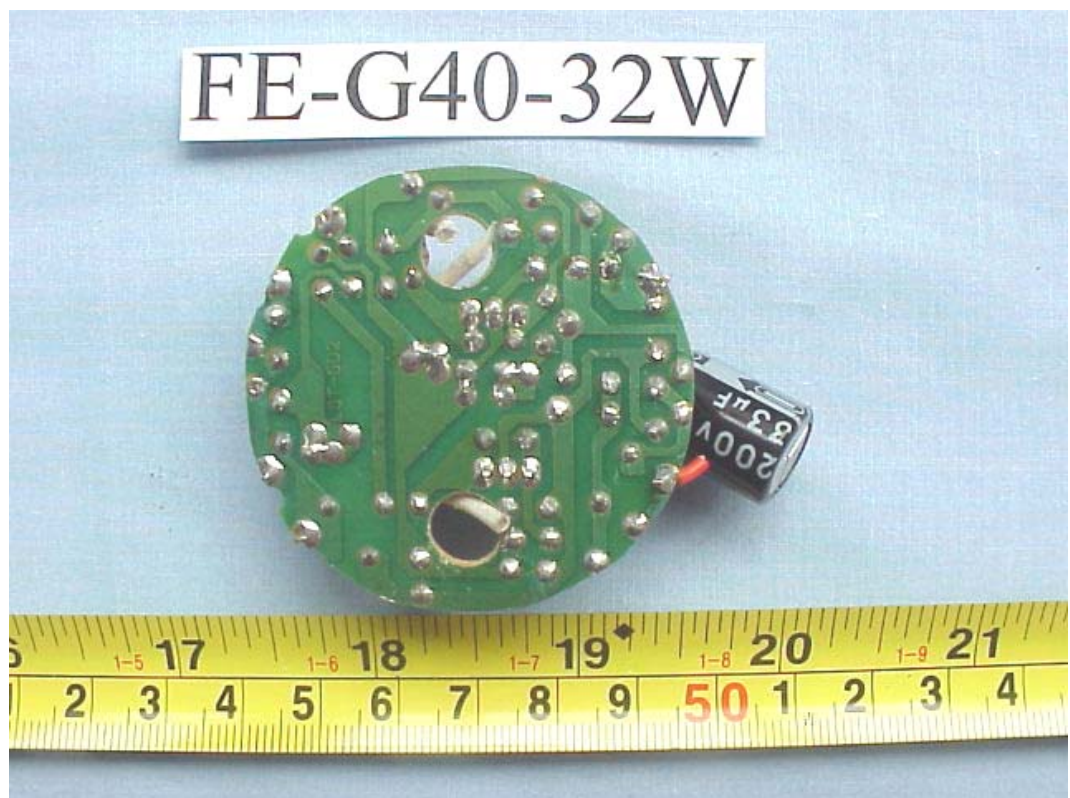
FIGURE 40 ENERGY SAVING LAMP (M/N: FE-G40-32W) MAIN BOARD (SOLDERED SIDE)
