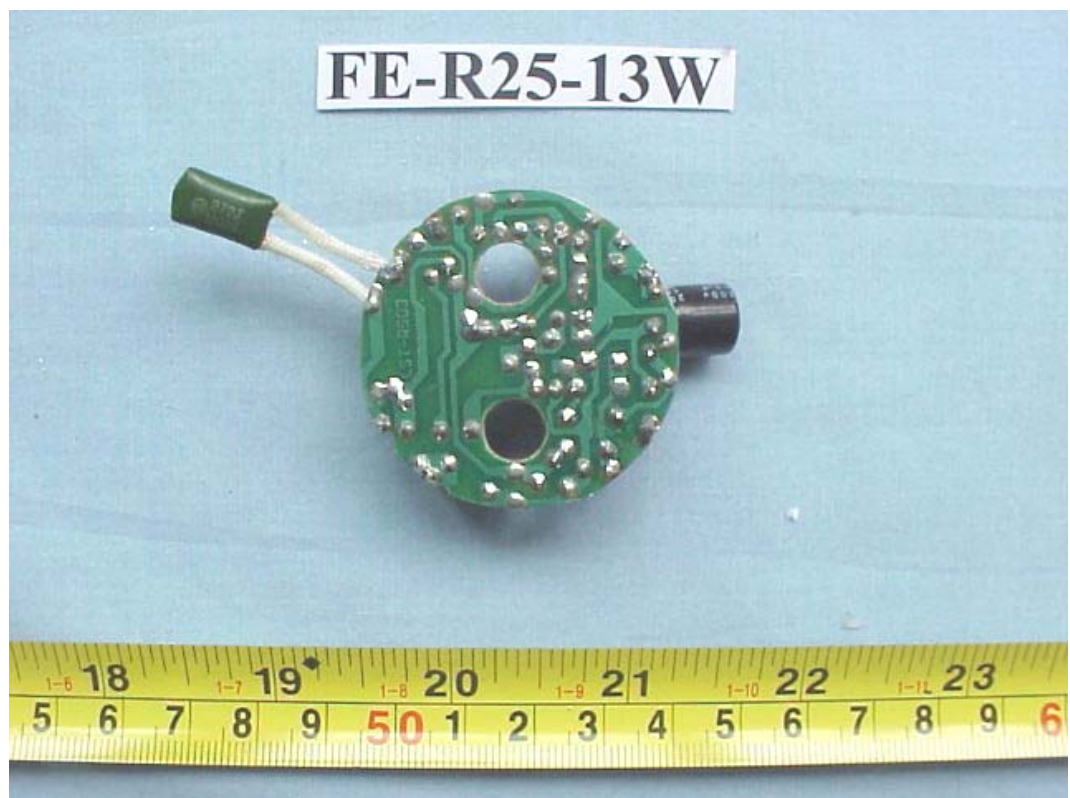
FIGURE 8 ENERGY SAVING LAMP (M/N: FE-R25-13W) MAIN BOARD (SOLDERED SIDE)
