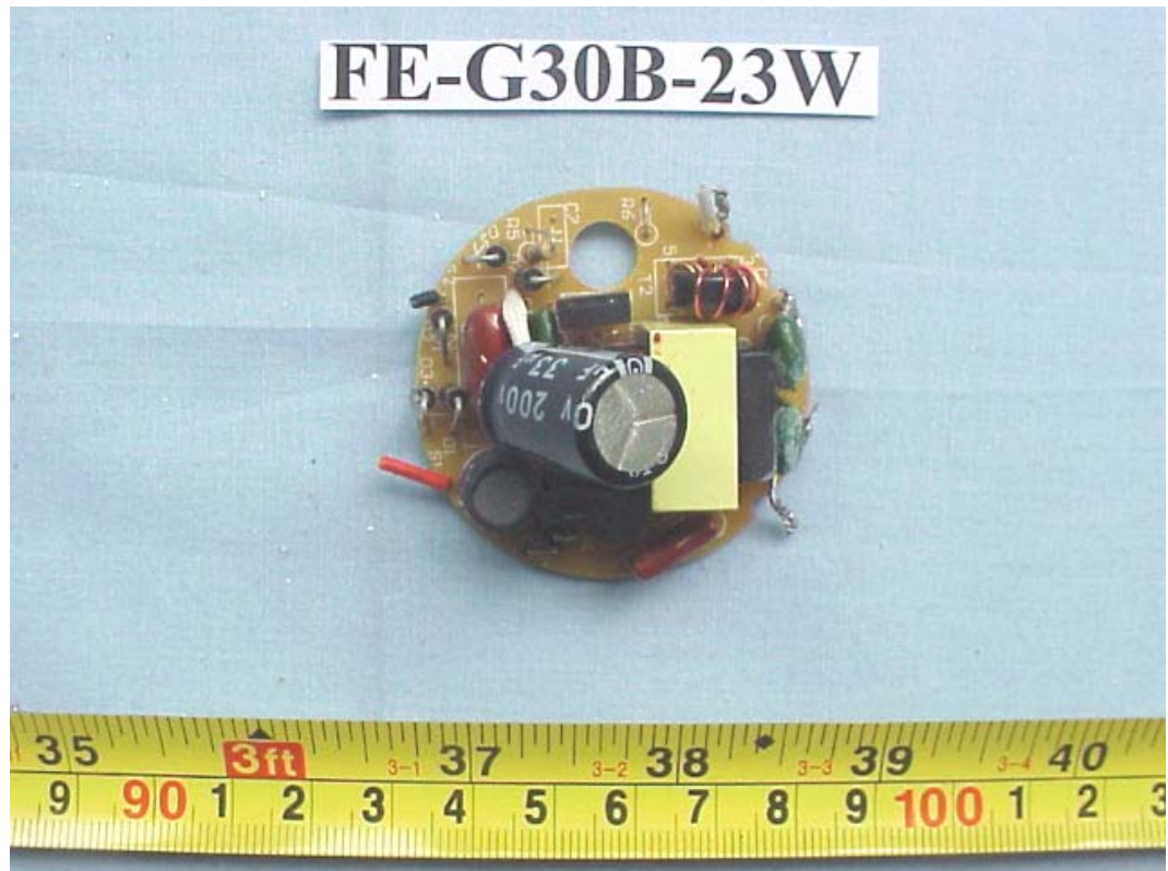
FIGURE 35 ENERGY SAVING LAMP (M/N: FE-G30B-23W) MAIN BOARD (COMPONENT SIDE)
