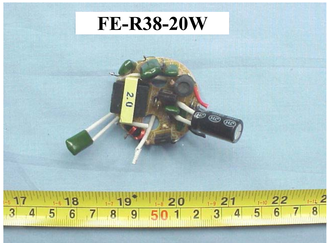
FIGURE 15 ENERGY SAVING LAMP (M/N: FE-R38-20W) MAIN BOARD (COMPONENT SIDE)
