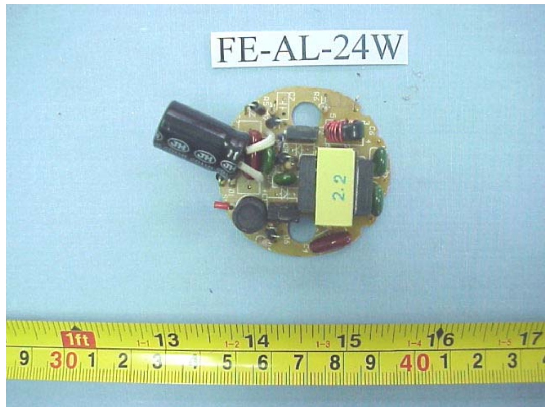
FIGURE 43 ENERGY SAVING LAMP (M/N: FE-AL-24W) MAIN BOARD (COMPONENT SIDE)
