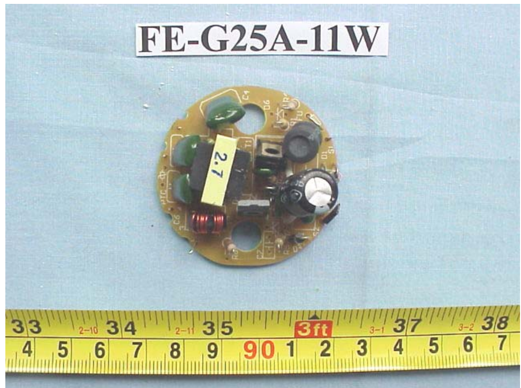
FIGURE 23 ENERGY SAVING LAMP (M/N: FE-G25A-11W) MAIN BOARD (COMPONENT SIDE)
