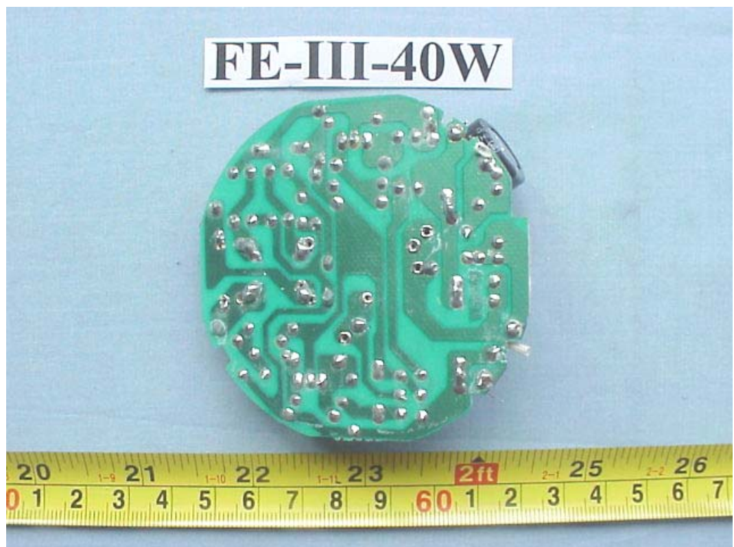
FIGURE 50 ENERGY SAVING LAMP (M/N: FE-III-40W) MAIN BOARD (SOLDERED SIDE)
