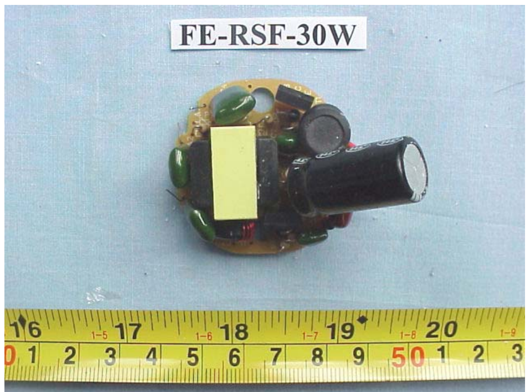
FIGURE 22 ENERGY SAVING LAMP (M/N: FE-RSF-30W) MAIN BOARD (COMPONENT SIDE)
