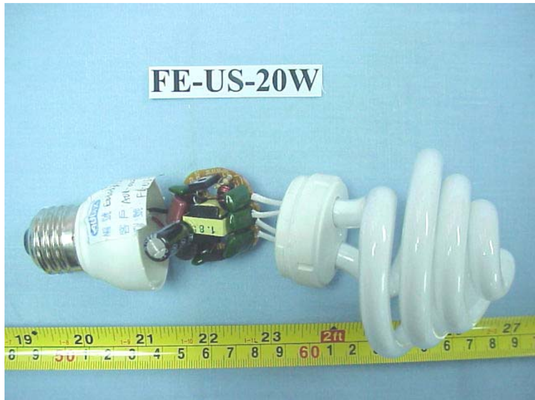
FIGURE 39 ENERGY SAVING LAMP (M/N: FE-US-20W) COVER REMOVED
