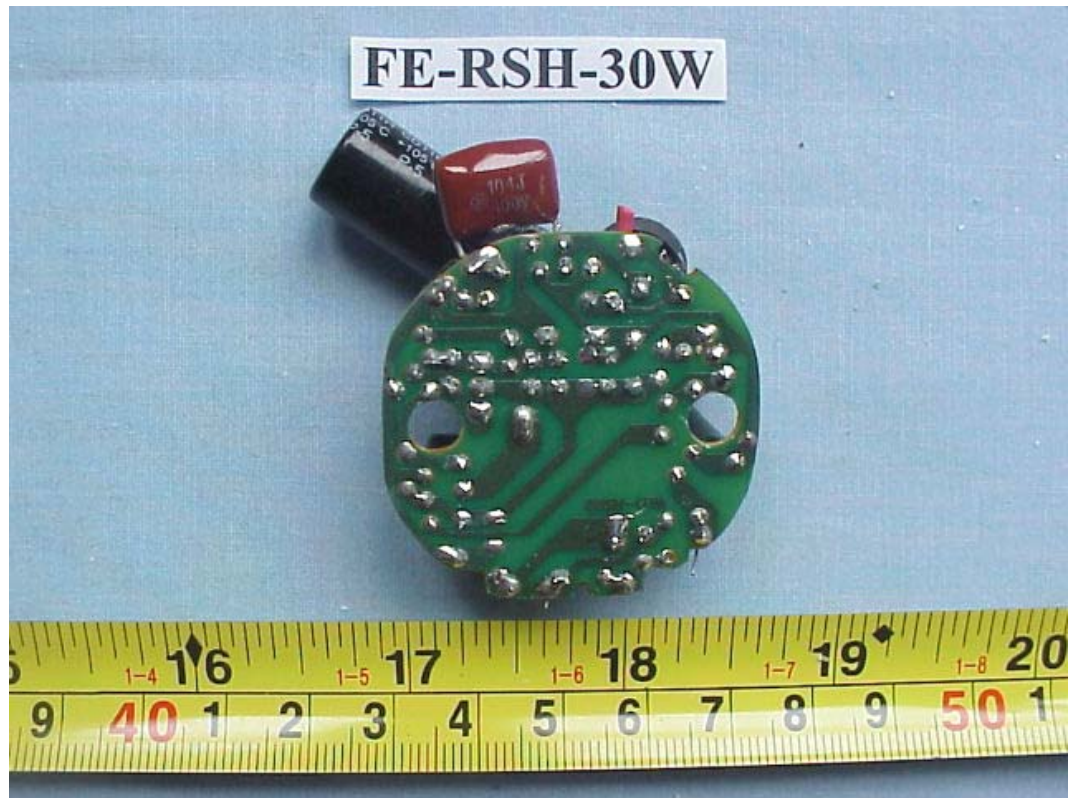
FIGURE 35 ENERGY SAVING LAMP (M/N: FE-RSH-30W) MAIN BOARD (SOLDERED SIDE)
