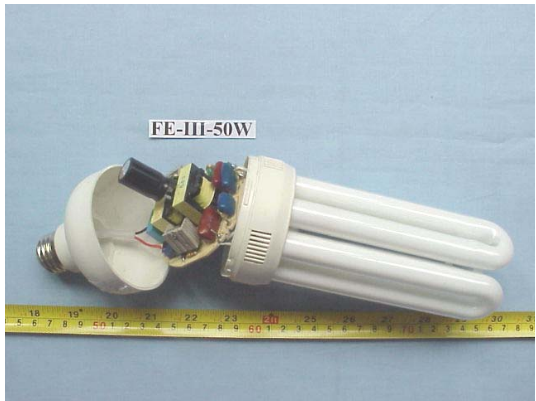
FIGURE 51 ENERGY SAVING LAMP (M/N: FE-III-50W) COVER REMOVED
