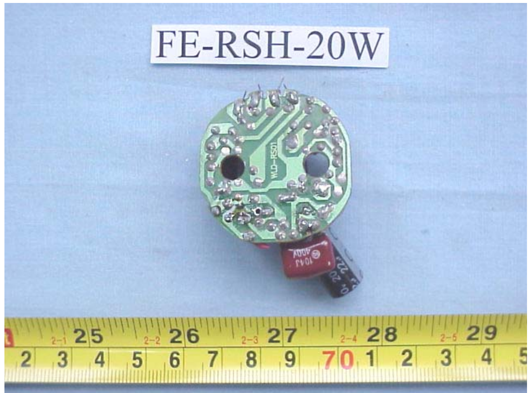
FIGURE 31 ENERGY SAVING LAMP (M/N: FE-RSH-20W) MAIN BOARD (SOLDERED SIDE)
