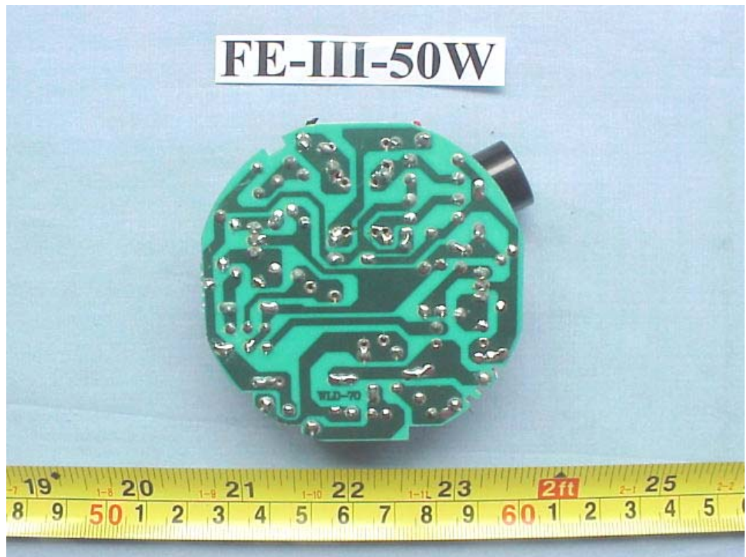
FIGURE 53 ENERGY SAVING LAMP (M/N: FE-III-50W) MAIN BOARD (SOLDERED SIDE)
