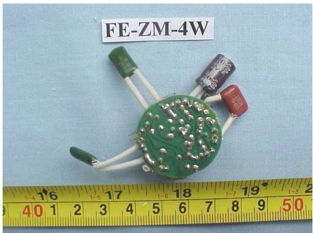
FIGURE 12 ENERGY SAVING LAMP (M/N: FE-ZM-4W) MAIN BOARD (SOLDERED SIDE)
