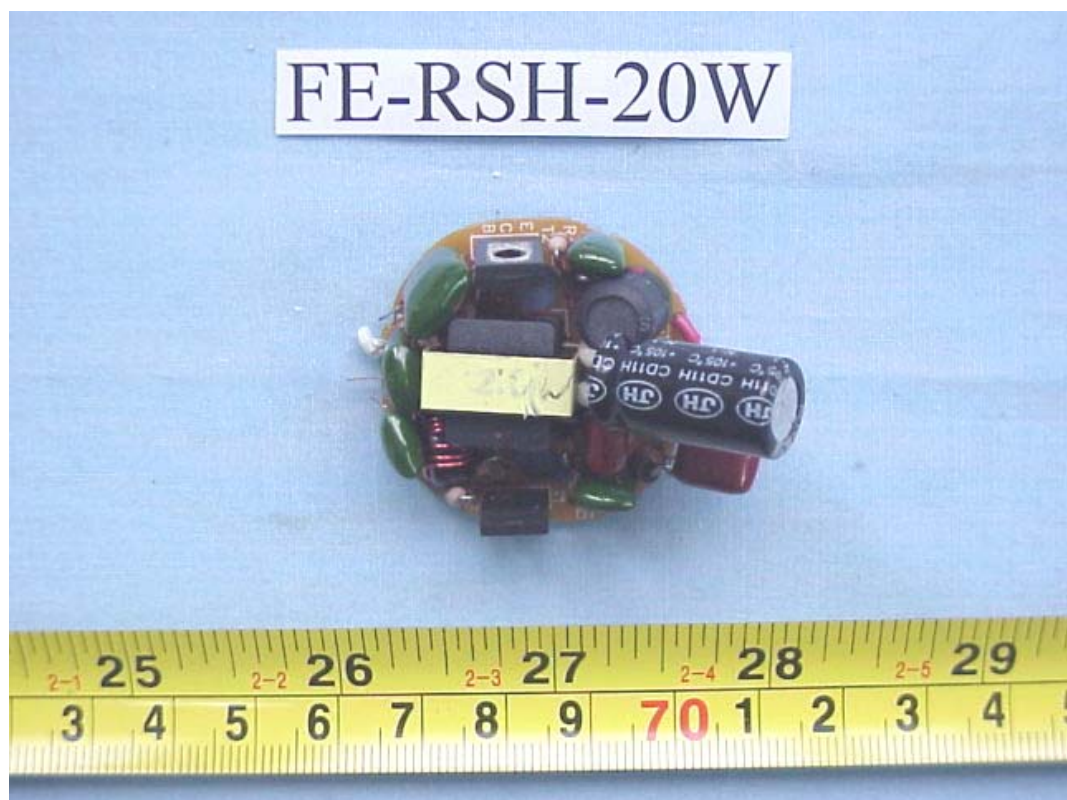
FIGURE 30 ENERGY SAVING LAMP (M/N: FE-RSH-20W) MAIN BOARD (COMPONENT SIDE)
