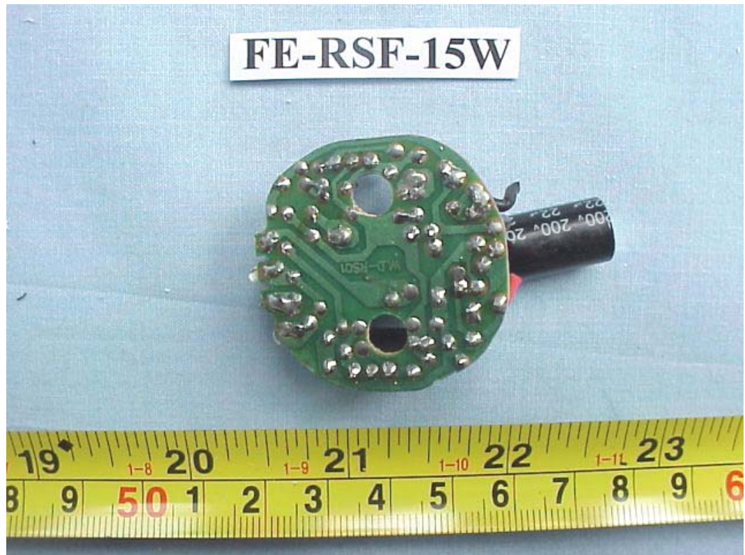
FIGURE 15 ENERGY SAVING LAMP (M/N: FE-RSF-15W) MAIN BOARD (SOLDERED SIDE)
