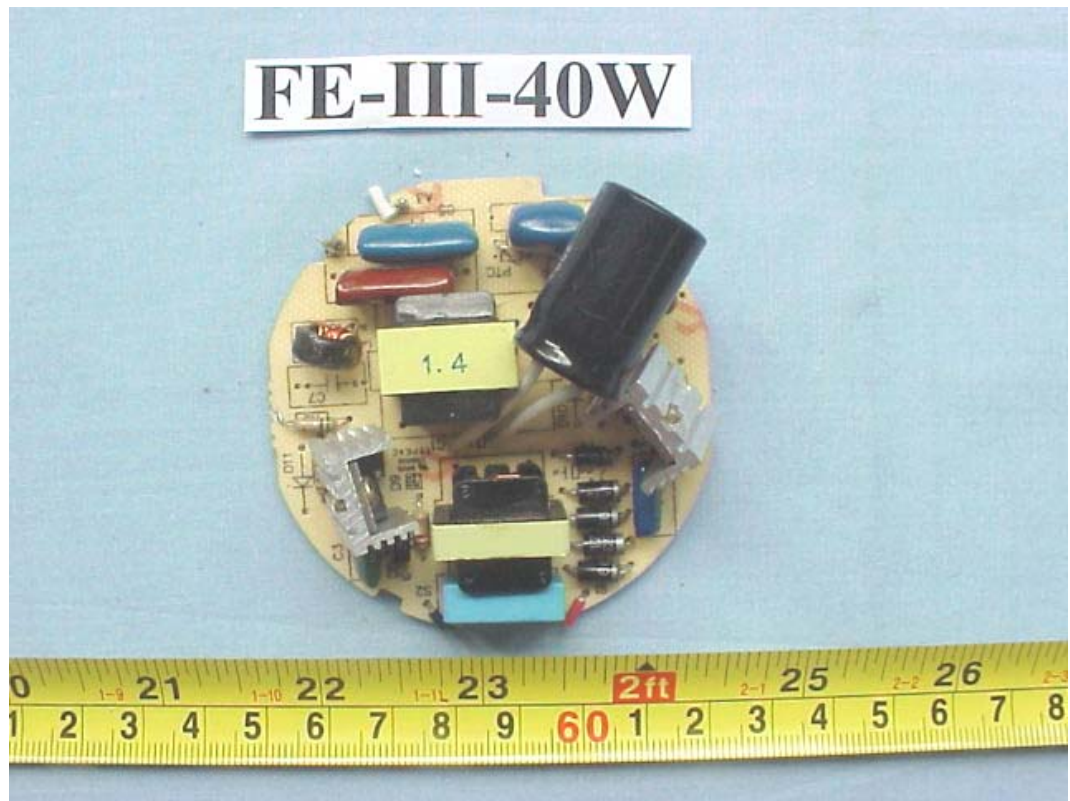
FIGURE 49 ENERGY SAVING LAMP (M/N: FE-III-40W) MAIN BOARD (COMPONENT SIDE)
