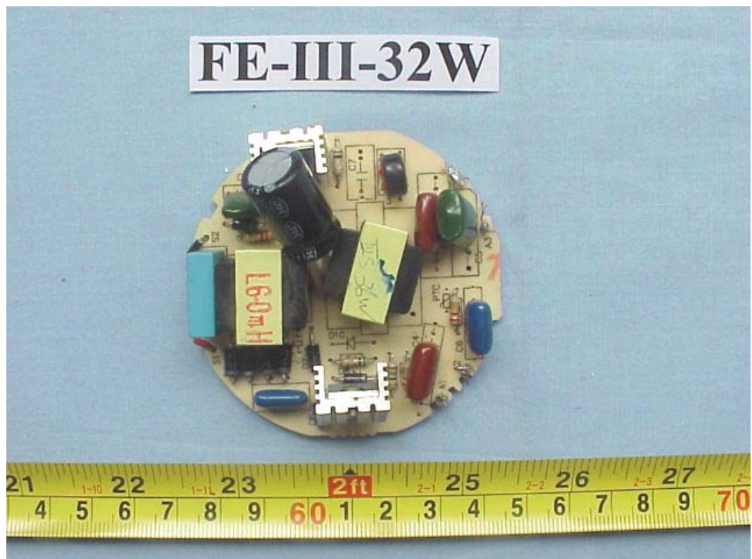
FIGURE 46 ENERGY SAVING LAMP (M/N: FE-III-32W) MAIN BOARD (COMPONENT SIDE)
