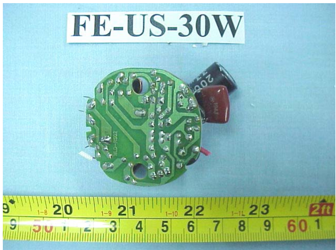
FIGURE 44 ENERGY SAVING LAMP (M/N: FE-US-30W) MAIN BOARD (SOLDERED SIDE)
