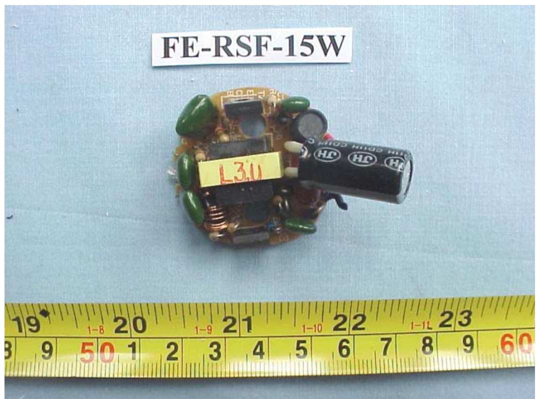
FIGURE 14 ENERGY SAVING LAMP (M/N: FE-RSF-15W) MAIN BOARD (COMPONENT SIDE)
