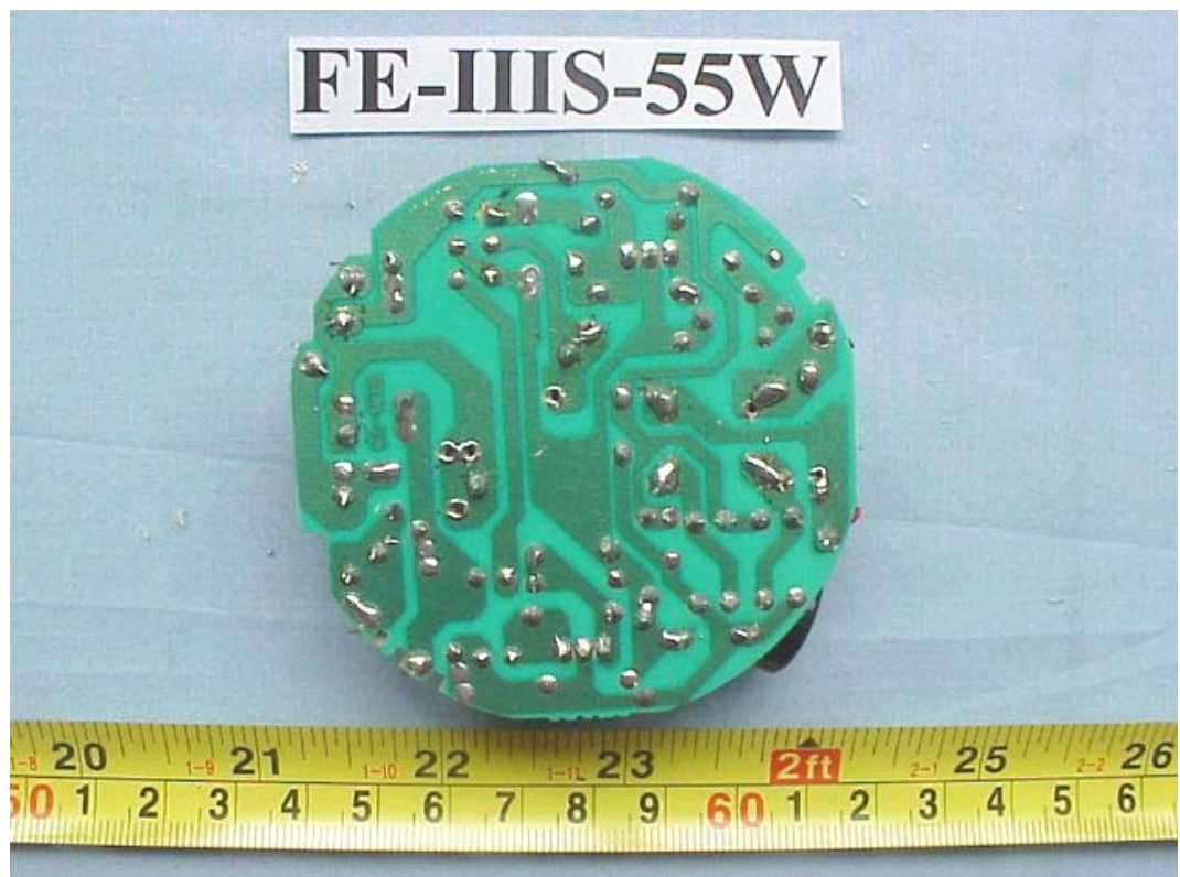
FIGURE 62 ENERGY SAVING LAMP (M/N: FE-IIIIS-55W) MAIN BOARD (SOLDERED SIDE)
