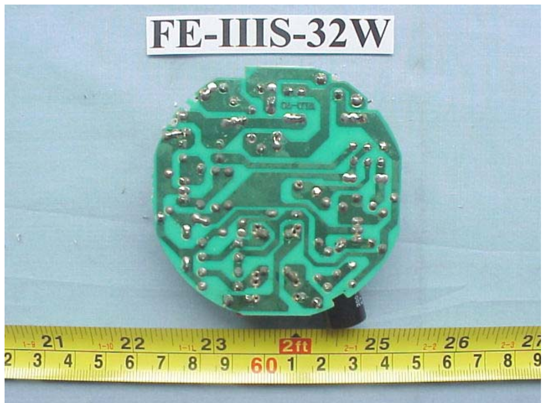
FIGURE 56 ENERGY SAVING LAMP (M/N: FE-IIIIS-32W) MAIN BOARD (SOLDERED SIDE)
