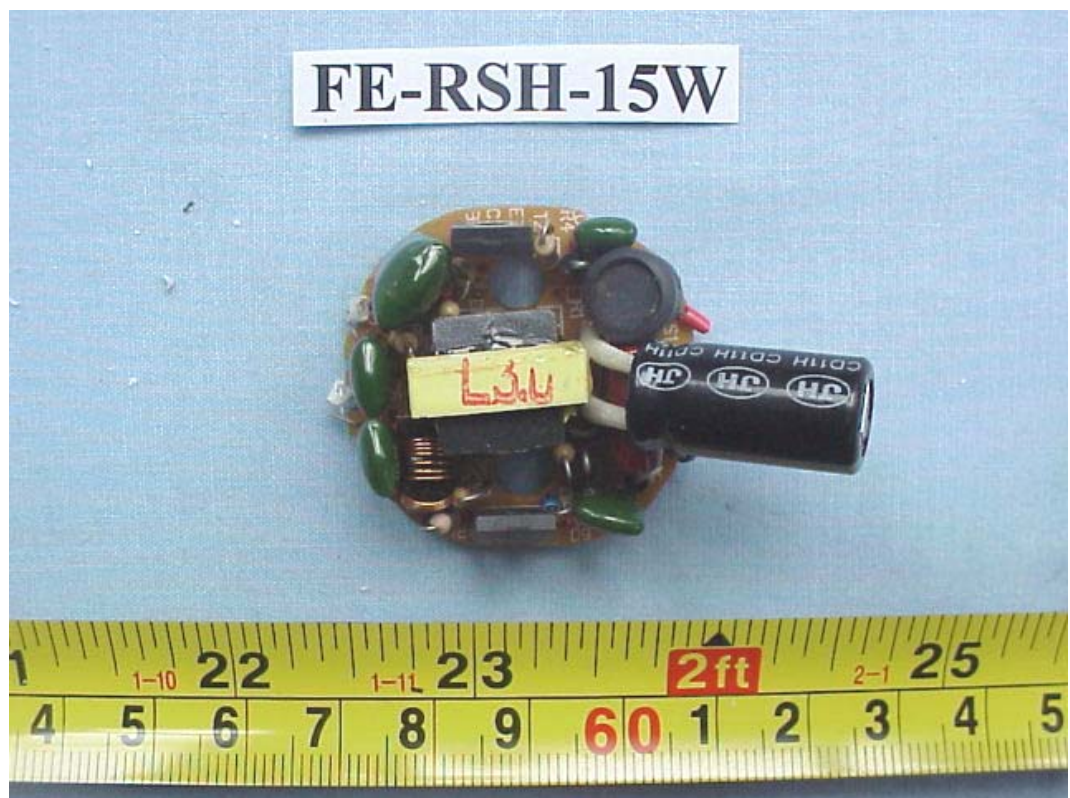
FIGURE 26 ENERGY SAVING LAMP (M/N: FE-RSH-15W) MAIN BOARD (COMPONENT SIDE)
