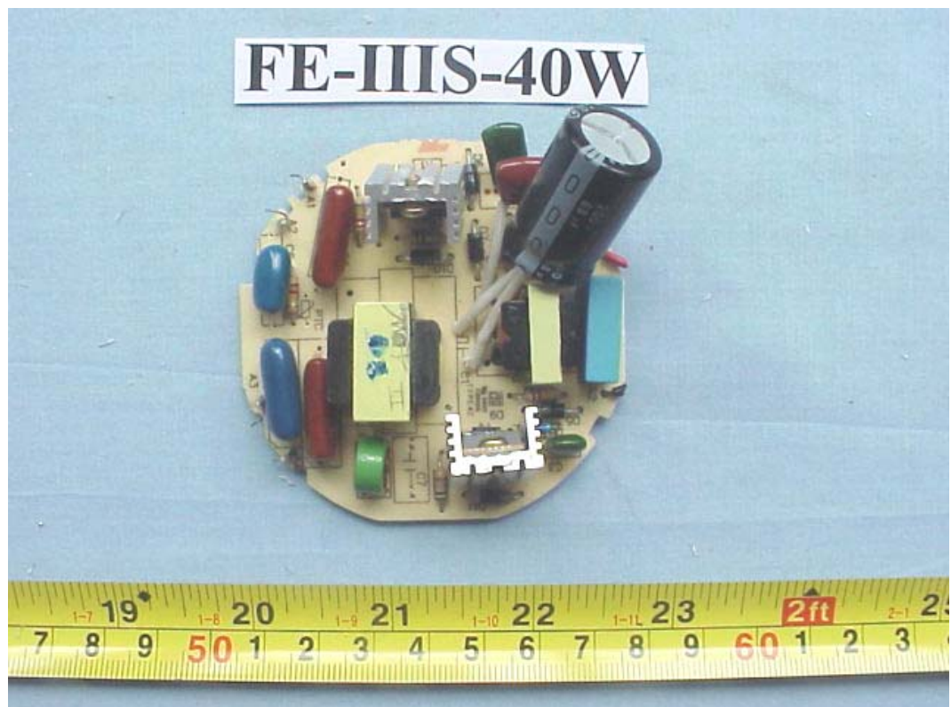
FIGURE 58 ENERGY SAVING LAMP (M/N: FE-IIIIS-40W) MAIN BOARD (COMPONENT SIDE)
