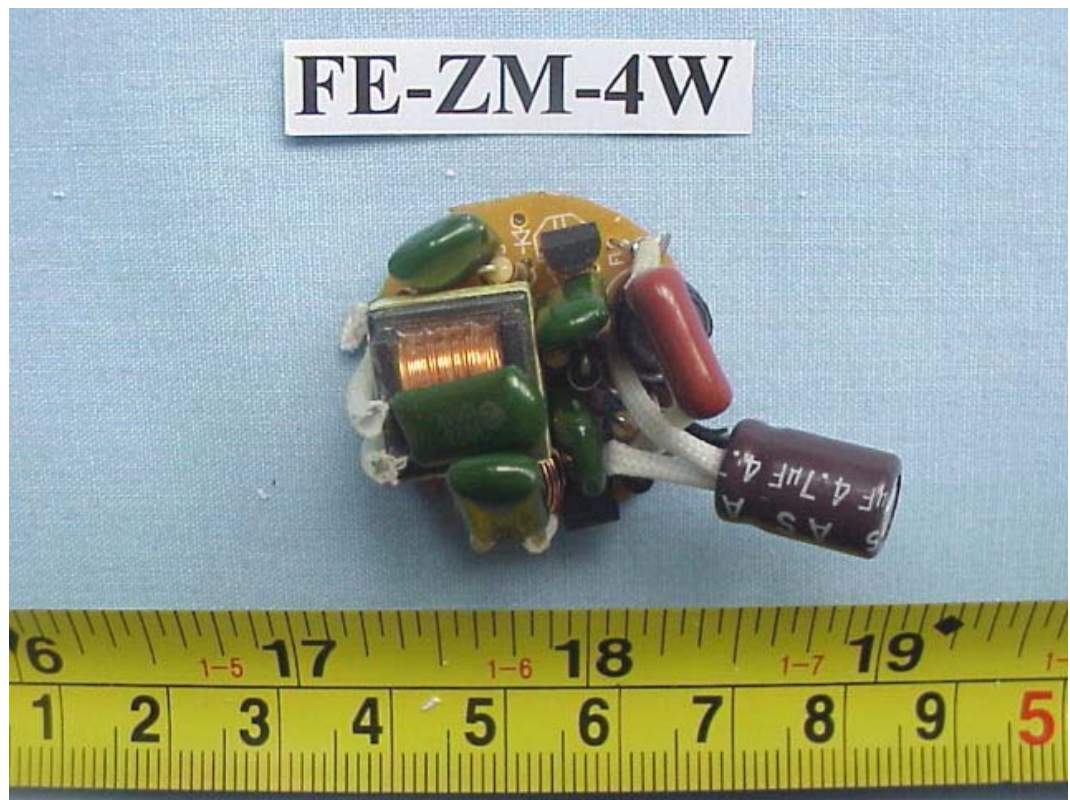
FIGURE 11 ENERGY SAVING LAMP (M/N: FE-ZM-4W) MAIN BOARD (COMPONENT SIDE)
