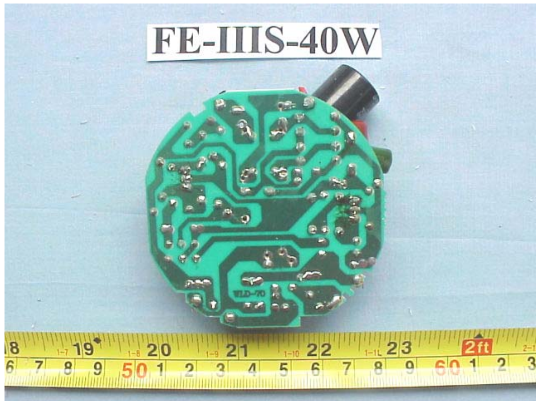
FIGURE 59 ENERGY SAVING LAMP (M/N: FE-IIIIS-40W) MAIN BOARD (SOLDERED SIDE)
