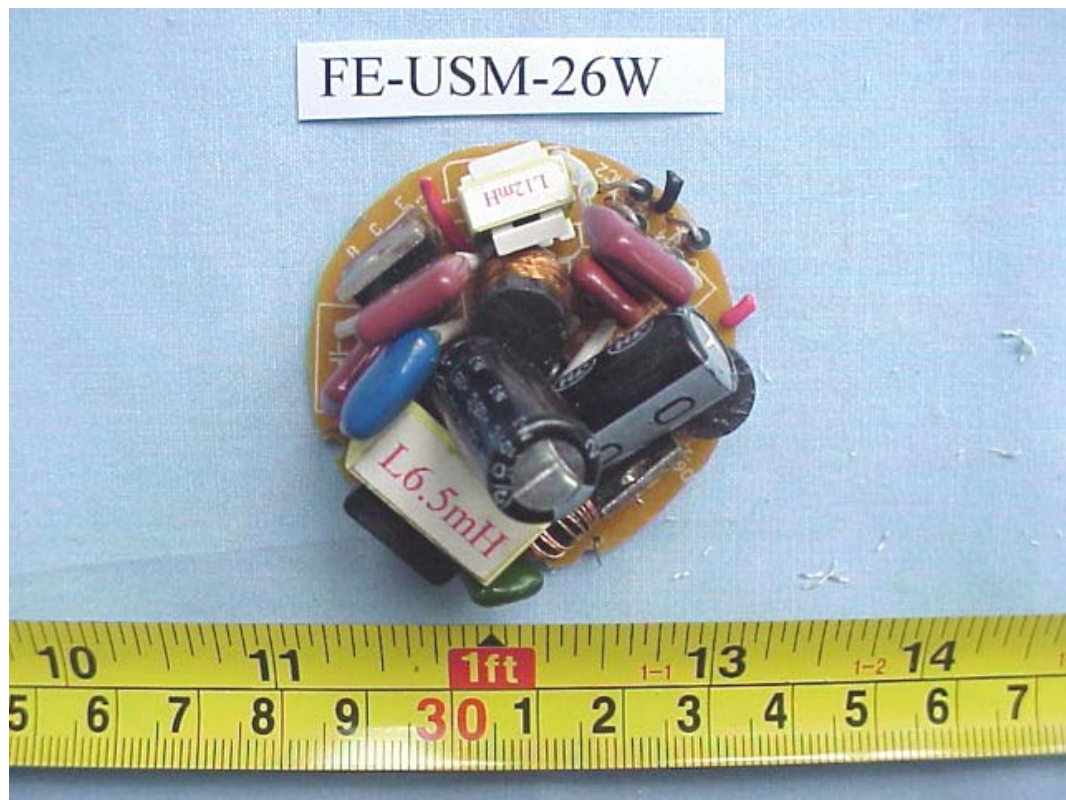
FIGURE 26 ENERGY SAVING LAMP (M/N: FE-USM-26W) MAIN BOARD (COMPONENT SIDE)
