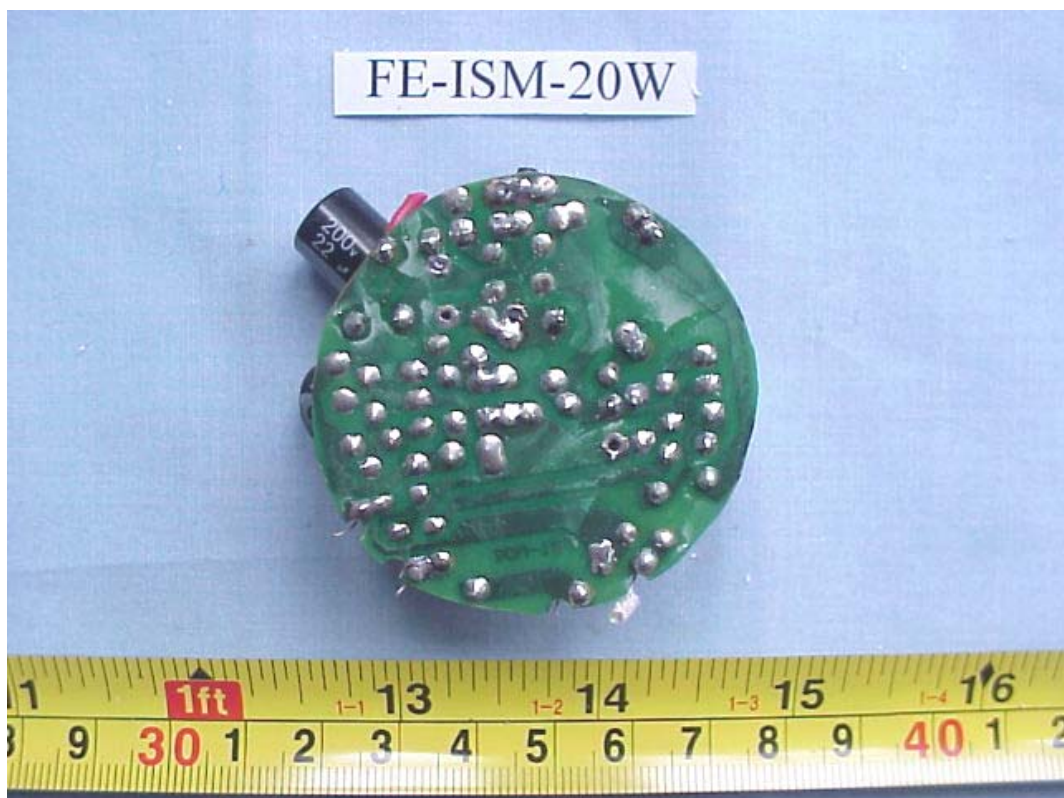
FIGURE 33 ENERGY SAVING LAMP (M/N: FE-ISM-20W) MAIN BOARD (SOLDERED SIDE)
