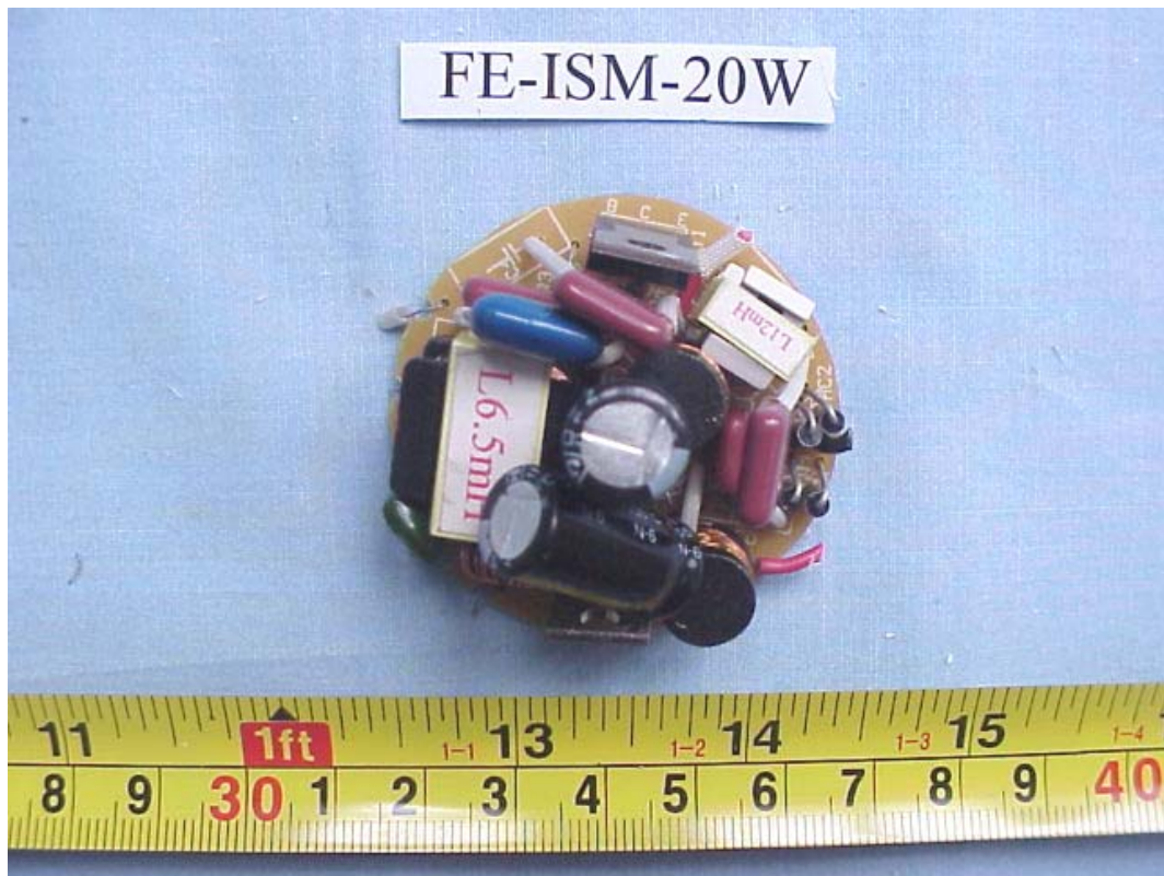
FIGURE 32 ENERGY SAVING LAMP (M/N: FE-ISM-20W) MAIN BOARD (COMPONENT SIDE)
