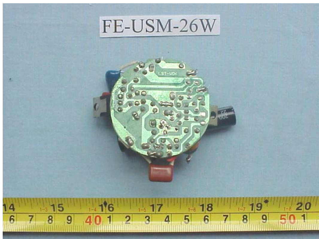
FIGURE 27 ENERGY SAVING LAMP (M/N: FE-USM-26W) MAIN BOARD (SOLDERED SIDE)
