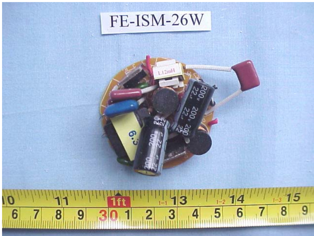
FIGURE 38 ENERGY SAVING LAMP (M/N: FE-ISM-26W) MAIN BOARD (COMPONENT SIDE)
