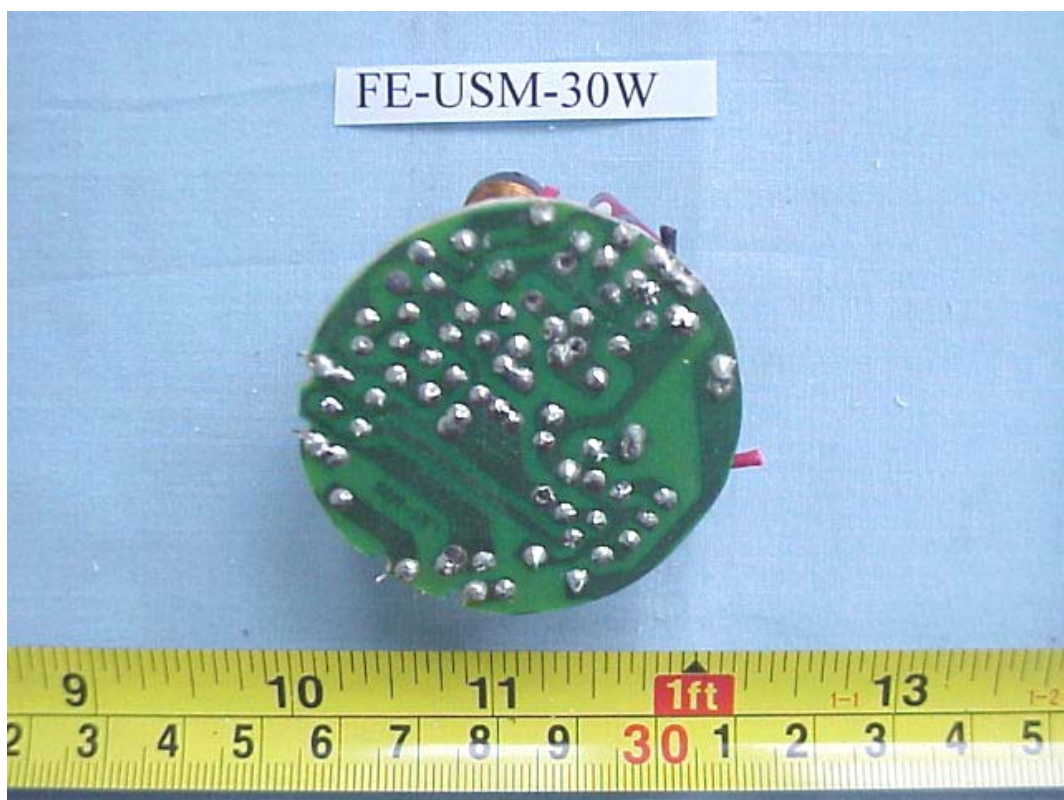
FIGURE 30 ENERGY SAVING LAMP (M/N: FE-USM-30W) MAIN BOARD (SOLDERED SIDE)
