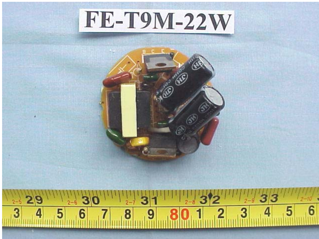
FIGURE 44 ENERGY SAVING LAMP (M/N: FE-T9M-22W) MAIN BOARD (COMPONENT SIDE)
