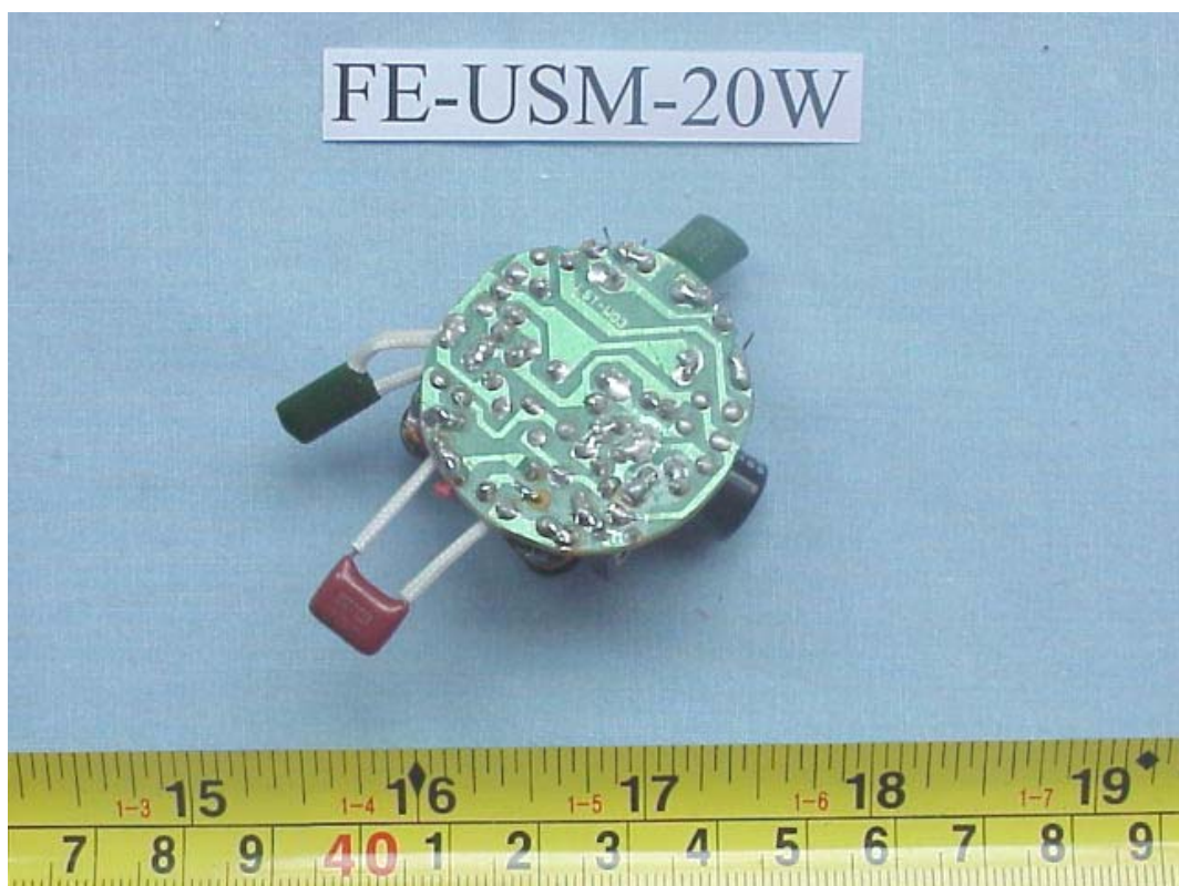
FIGURE 21 ENERGY SAVING LAMP (M/N: FE-USM-20W) MAIN BOARD (SOLDERED SIDE)
