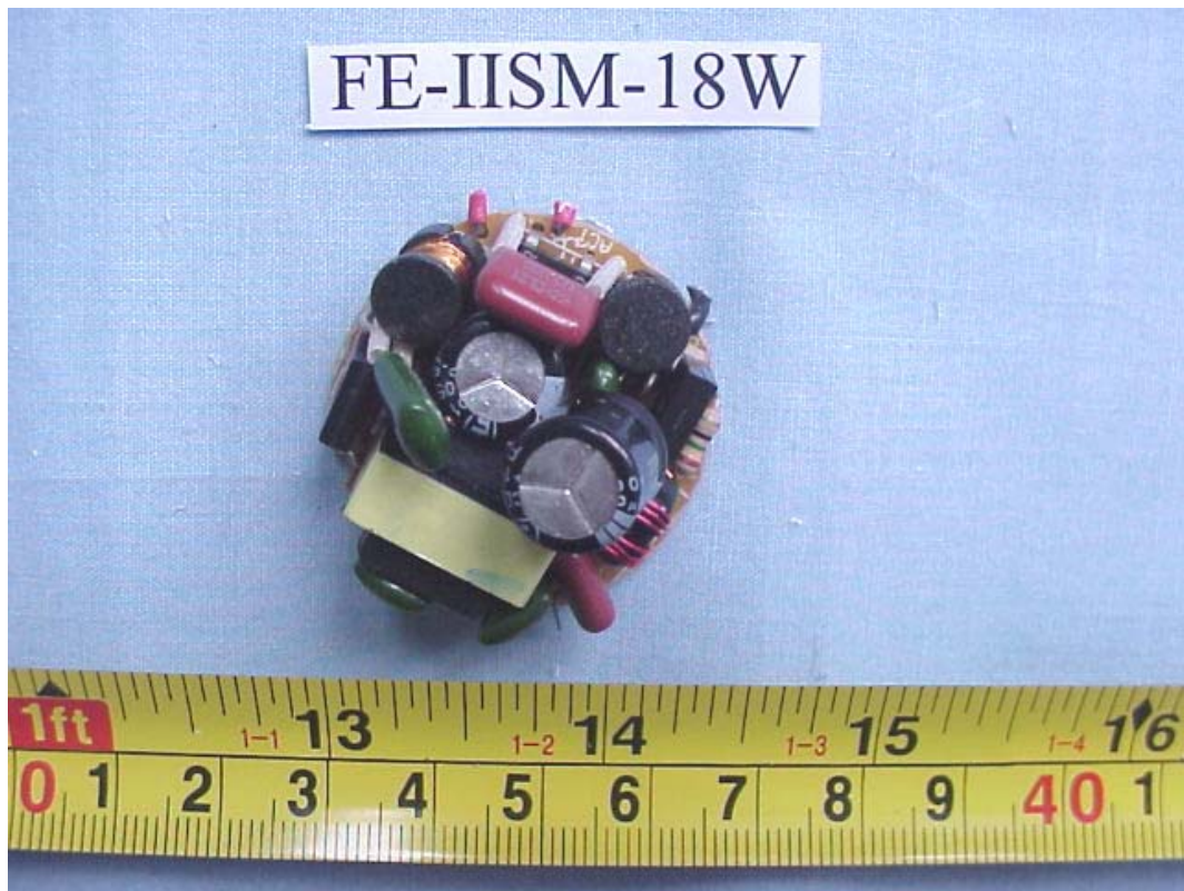
FIGURE 8 ENERGY SAVING LAMP (M/N: FE-IISM-18W) MAIN BOARD (COMPONENT SIDE)
