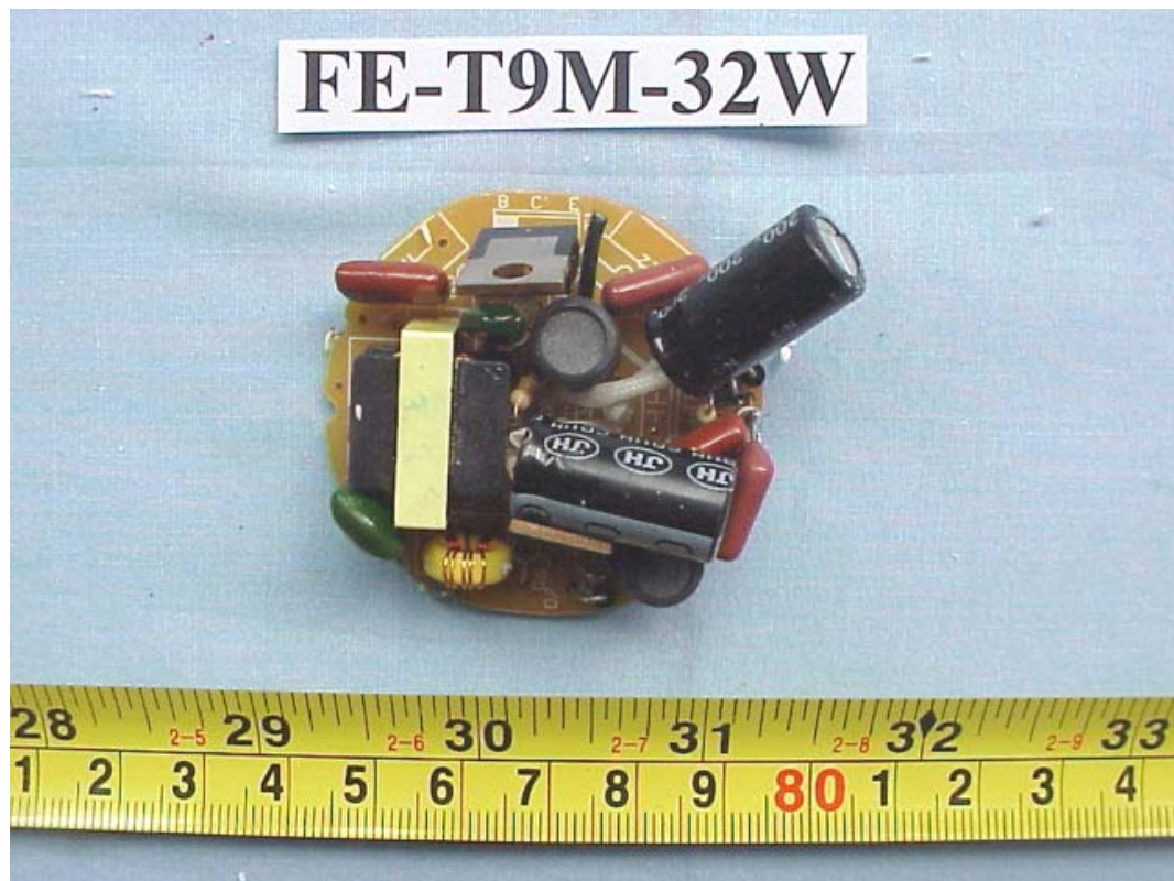
FIGURE 47 ENERGY SAVING LAMP (M/N: FE-T9M-32W) MAIN BOARD (COMPONENT SIDE)
