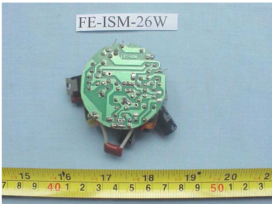
FIGURE 39 ENERGY SAVING LAMP (M/N: FE-ISM-26W) MAIN BOARD (SOLDERED SIDE)
