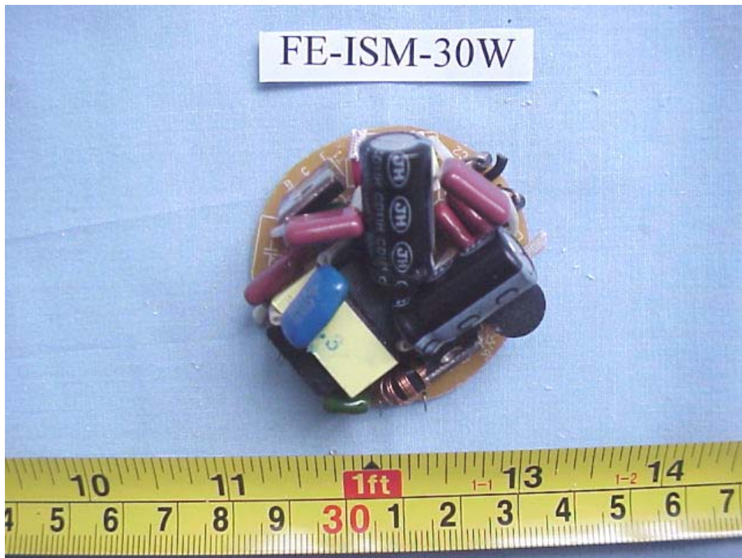
FIGURE 41 ENERGY SAVING LAMP (M/N: FE-ISM-30W) MAIN BOARD (COMPONENT SIDE)
