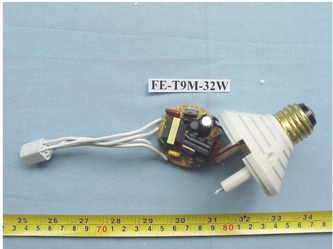
FIGURE 46 ENERGY SAVING LAMP (M/N: FE-T9M-32W) COVER REMOVED
