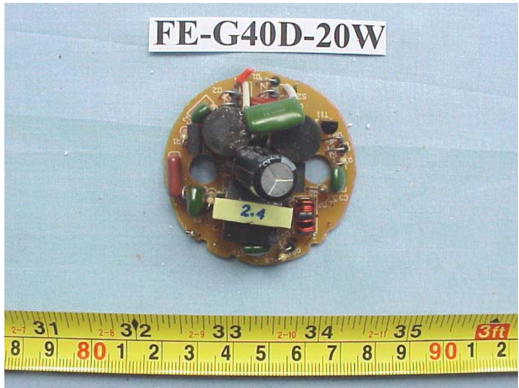
FIGURE 113 ENERGY SAVING LAMP (M/N: FE-G40D-20W) MAIN BOARD (COMPONENT SIDE)
