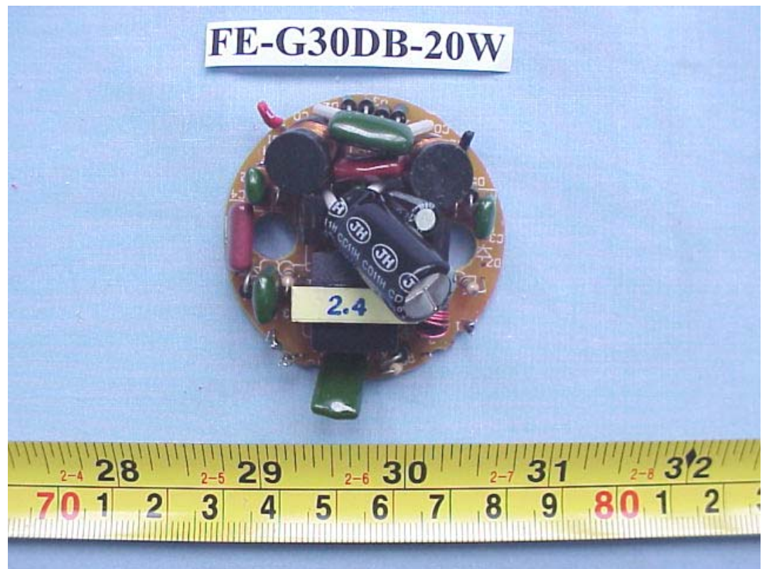
FIGURE 107 ENERGY SAVING LAMP (M/N: FE-G30DB-20W) MAIN BOARD (COMPONENT SIDE)
