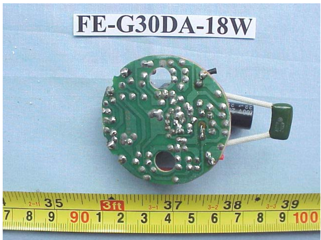
FIGURE 105 ENERGY SAVING LAMP (M/N: FE-G30DA-18W) MAIN BOARD (SOLDERED SIDE)
