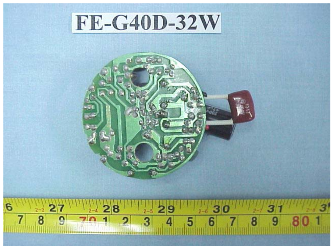
FIGURE 123 ENERGY SAVING LAMP (M/N: FE-G40D-32W) MAIN BOARD (SOLDERED SIDE)
