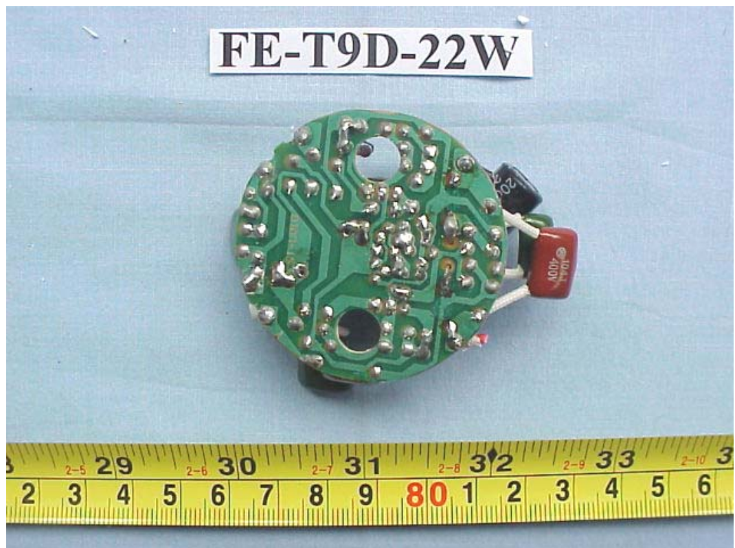
FIGURE 132 ENERGY SAVING LAMP (M/N: FE-T9D-22W) MAIN BOARD (SOLDERED SIDE)
