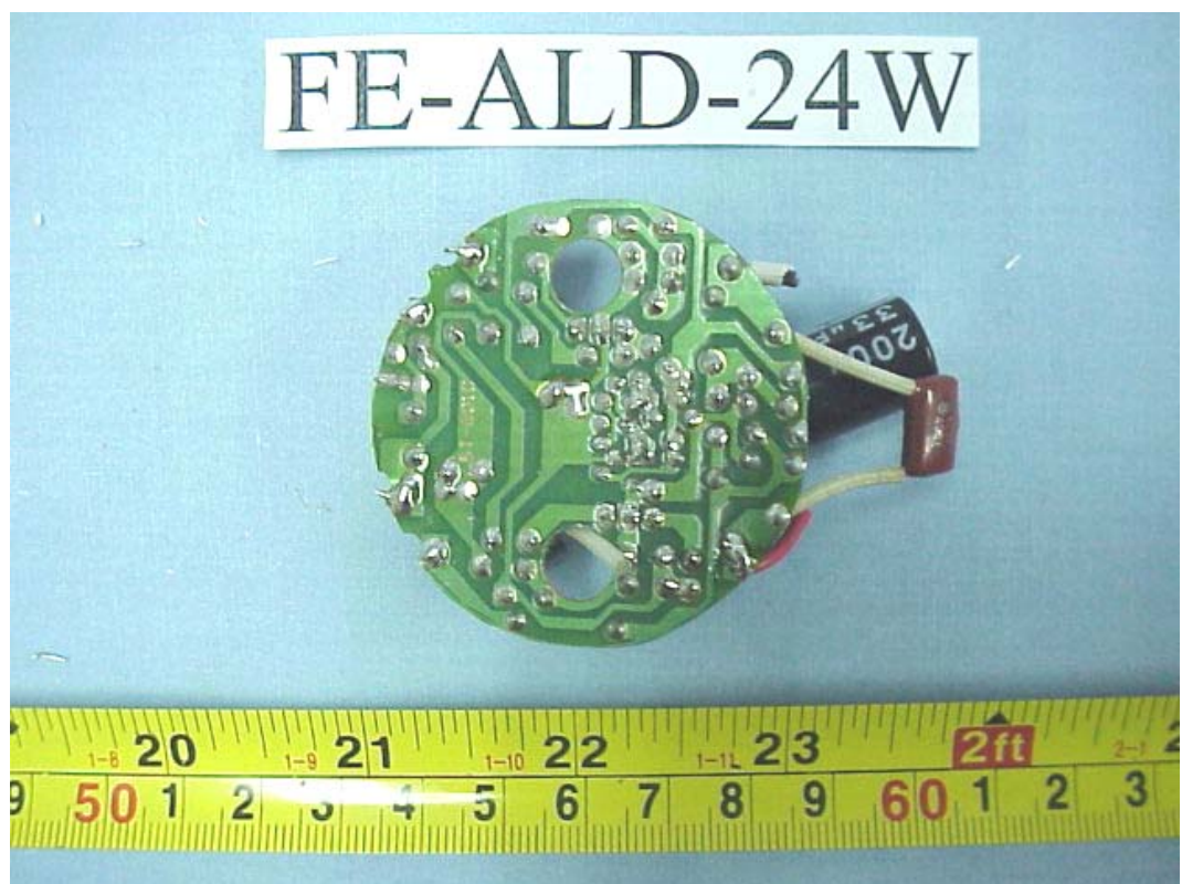
FIGURE 129 ENERGY SAVING LAMP (M/N: FE-ALD-24W) MAIN BOARD (SOLDERED SIDE)
