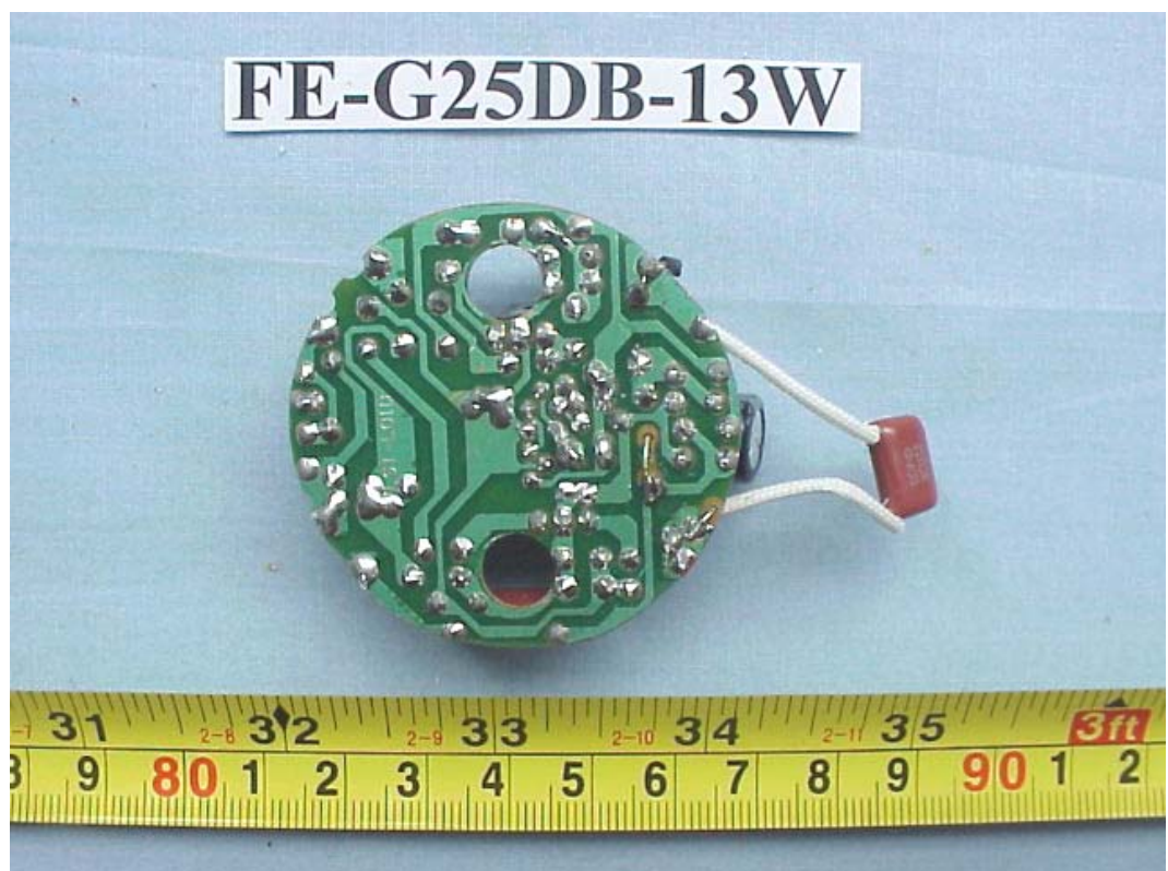
FIGURE 96 ENERGY SAVING LAMP (M/N: FE-G25DB-13W) MAIN BOARD (SOLDERED SIDE)
