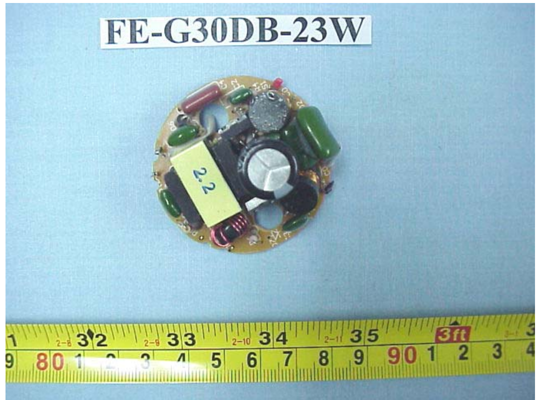
FIGURE 110 ENERGY SAVING LAMP (M/N: FE-G30DB-23W) MAIN BOARD (COMPONENT SIDE)
