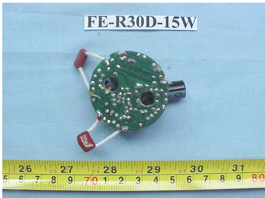
FIGURE 75 ENERGY SAVING LAMP (M/N: FE-R30D-15W) MAIN BOARD (SOLDERED SIDE)
