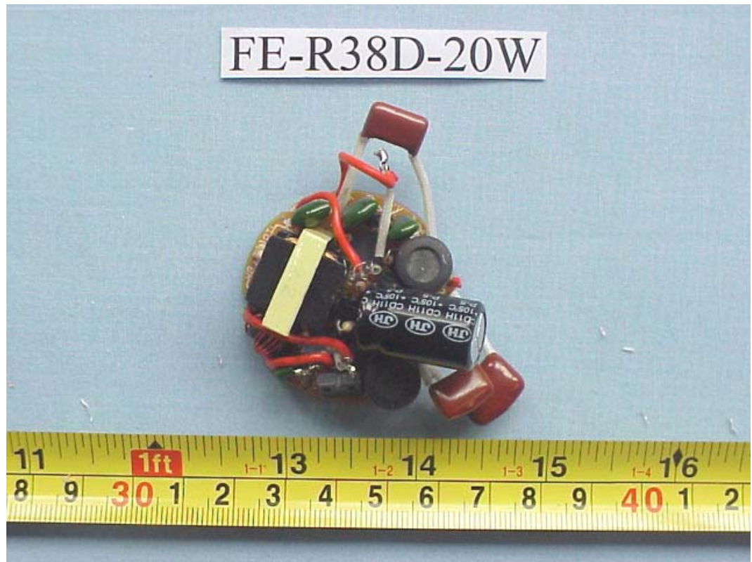
FIGURE 80 ENERGY SAVING LAMP (M/N: FE-R38D-20W) MAIN BOARD (COMPONENT SIDE)
