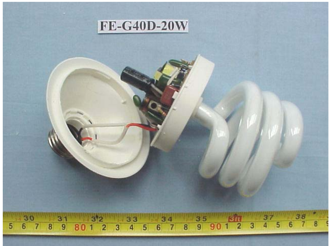
FIGURE 112 ENERGY SAVING LAMP (M/N: FE-G40D-20W) COVER REMOVED
