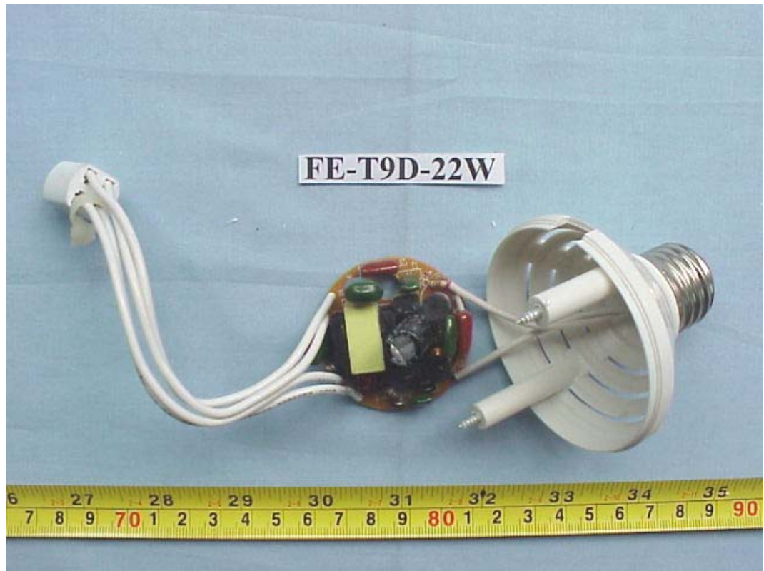
FIGURE 130 ENERGY SAVING LAMP (M/N: FE-T9D-22W) COVER REMOVED
