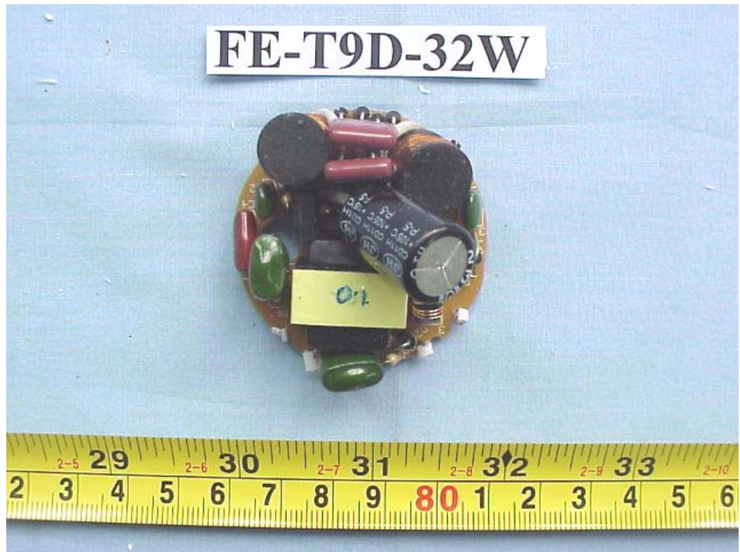
FIGURE 134 ENERGY SAVING LAMP (M/N: FE-T9D-32W) MAIN BOARD (COMPONENT SIDE)
