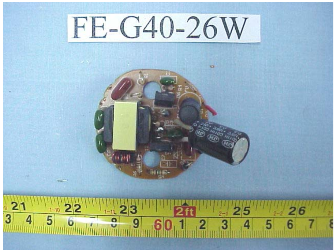
FIGURE 119 ENERGY SAVING LAMP (M/N: FE-G40D-26W) MAIN BOARD (COMPONENT SIDE)
