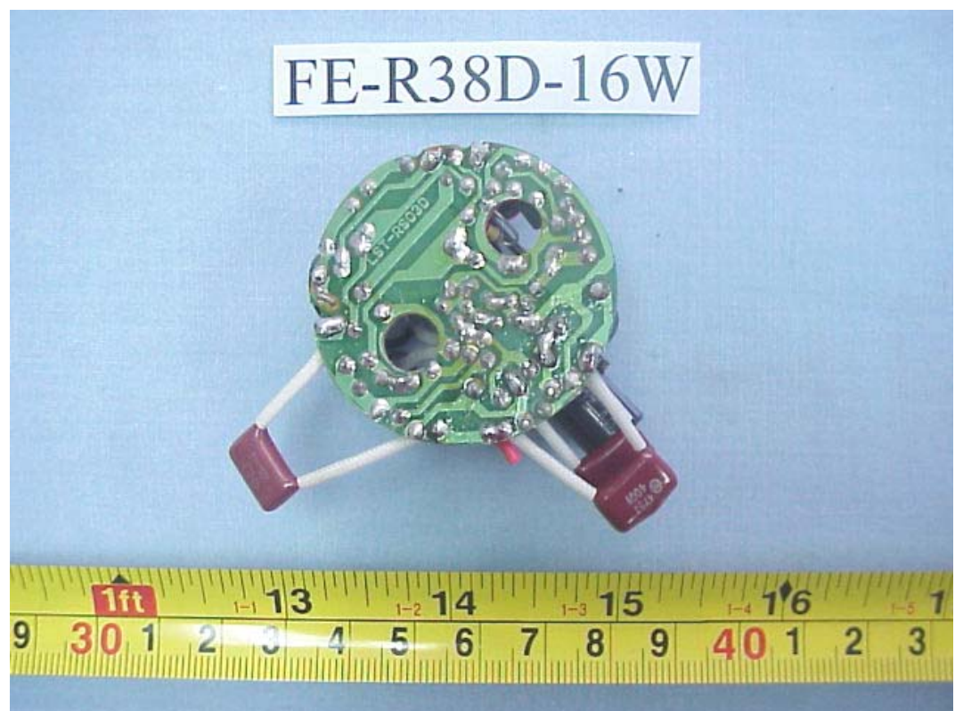
FIGURE 78 ENERGY SAVING LAMP (M/N: FE-R38D-16W) MAIN BOARD (SOLDERED SIDE)
