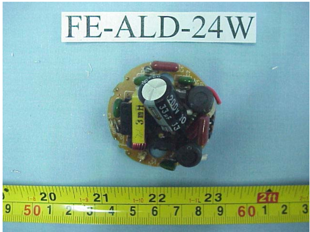
FIGURE 128 ENERGY SAVING LAMP (M/N: FE-ALD-24W) MAIN BOARD (COMPONENT SIDE)
