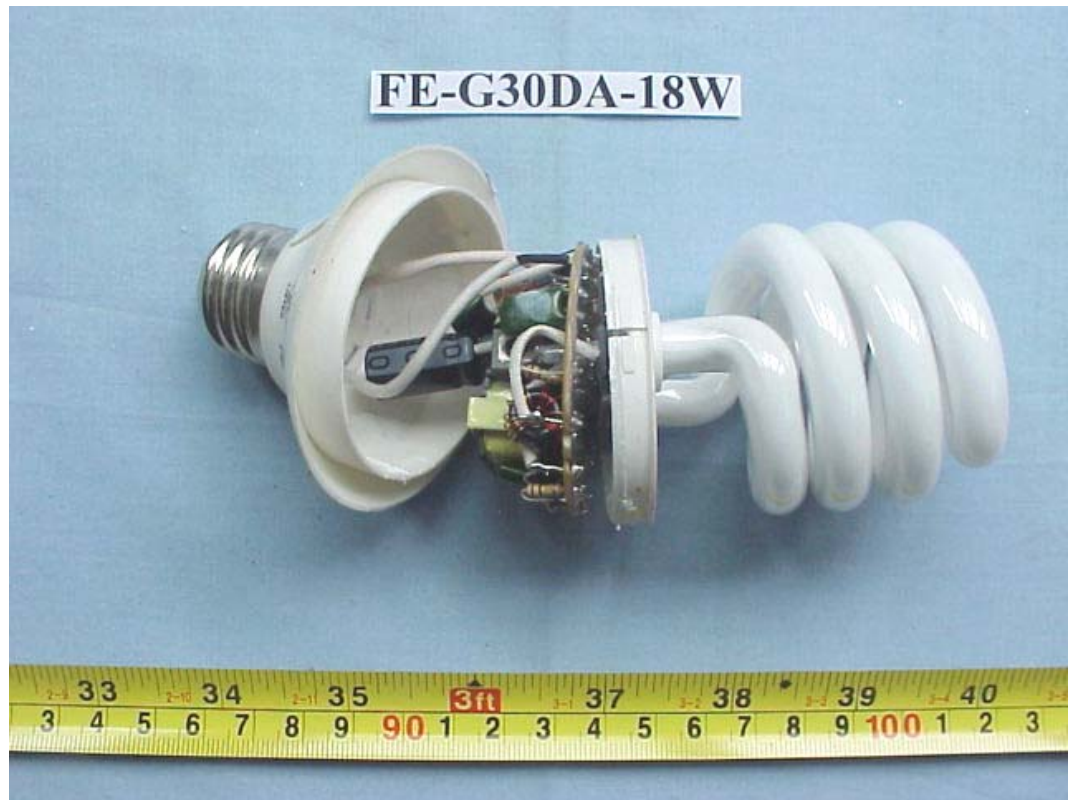
FIGURE 103 ENERGY SAVING LAMP (M/N: FE-G30DA-18W) COVER REMOVED
