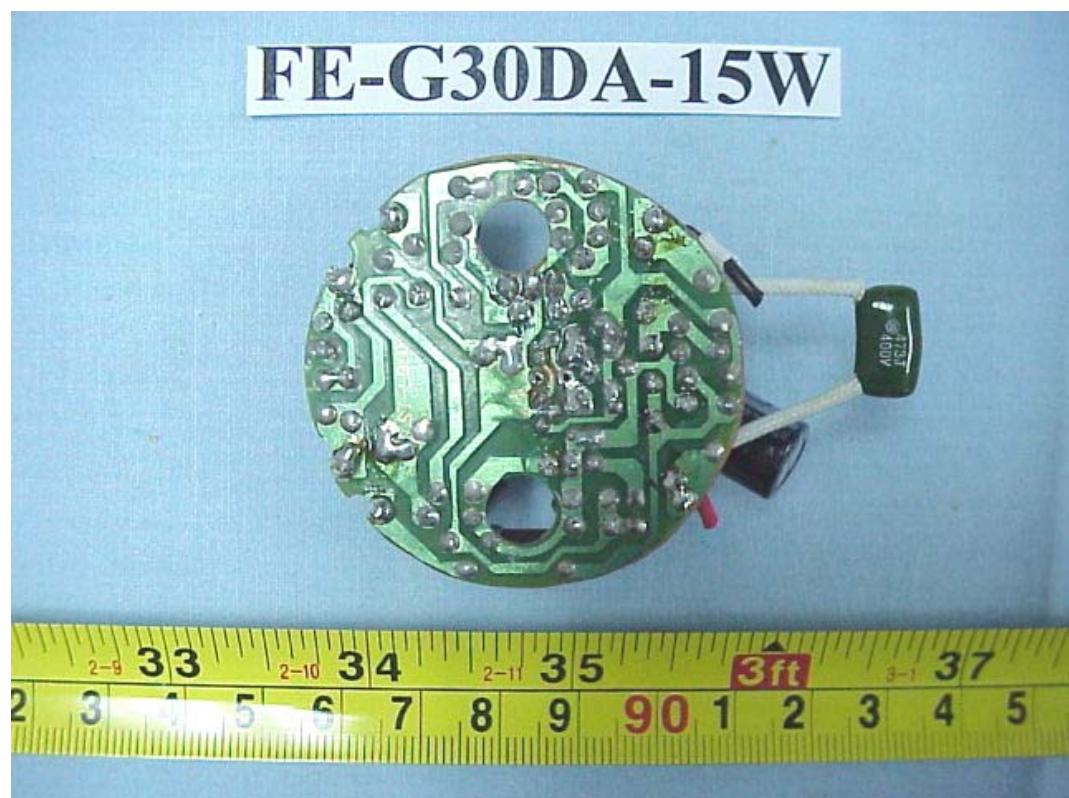
FIGURE 102 ENERGY SAVING LAMP (M/N: FE-G30DA-15W) MAIN BOARD (SOLDERED SIDE)
