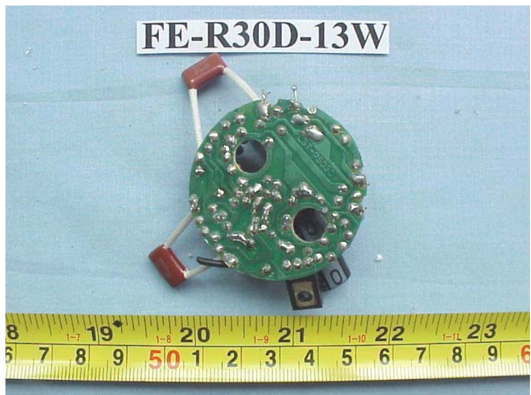
FIGURE 72 ENERGY SAVING LAMP (M/N: FE-R30D-13W) MAIN BOARD (SOLDERED SIDE)
