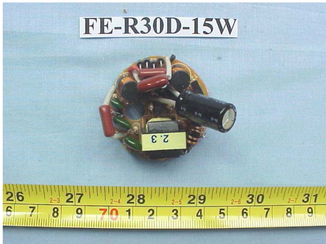
FIGURE 74 ENERGY SAVING LAMP (M/N: FE-R30D-15W) MAIN BOARD (COMPONENT SIDE)
