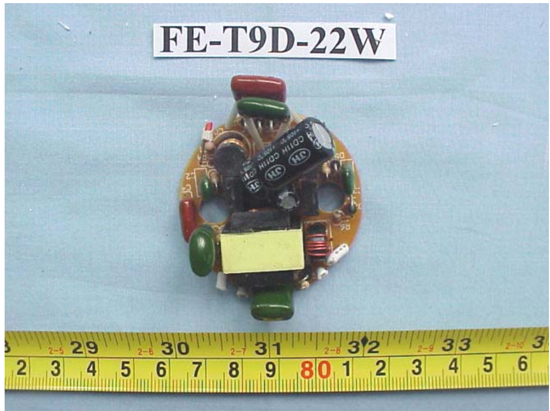
FIGURE 131 ENERGY SAVING LAMP (M/N: FE-T9D-22W) MAIN BOARD (COMPONENT SIDE)
