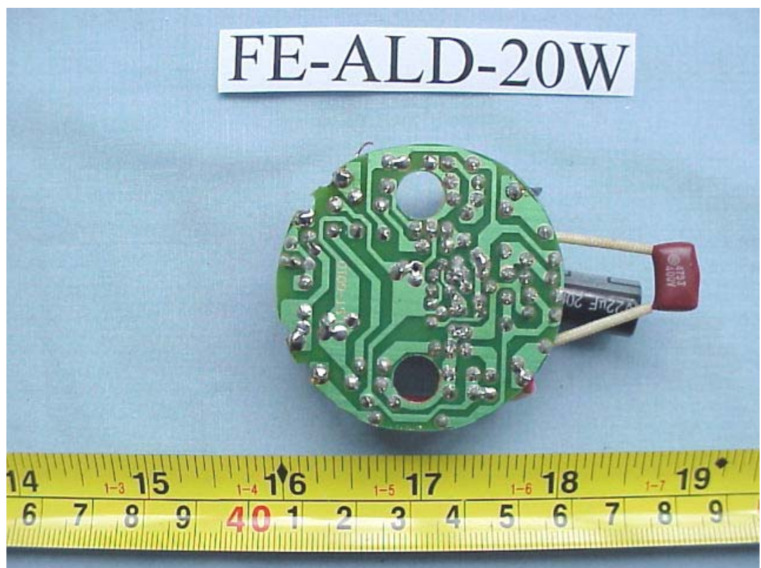
FIGURE 126 ENERGY SAVING LAMP (M/N: FE-ALD-20W) MAIN BOARD (SOLDERED SIDE)
