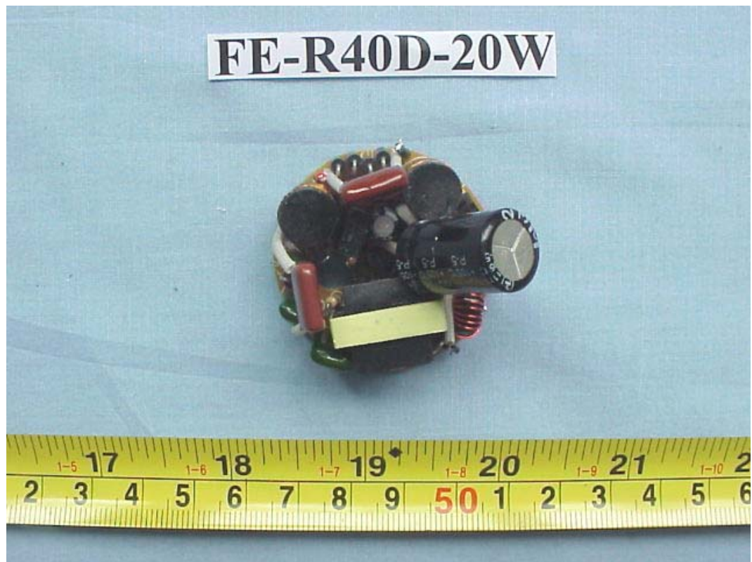
FIGURE 86 ENERGY SAVING LAMP (M/N: FE-R40D-20W) MAIN BOARD (COMPONENT SIDE)
