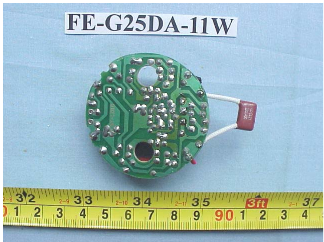
FIGURE 93 ENERGY SAVING LAMP (M/N: FE-G25DA-11W) MAIN BOARD (SOLDERED SIDE)
