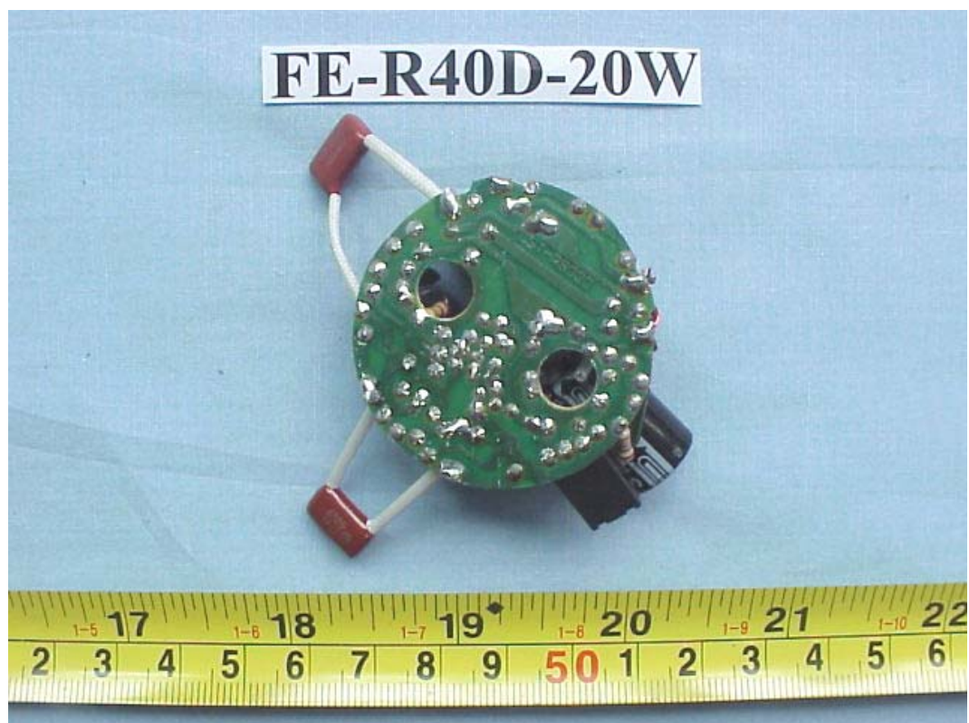
FIGURE 87 ENERGY SAVING LAMP (M/N: FE-R40D-20W) MAIN BOARD (SOLDERED SIDE)
