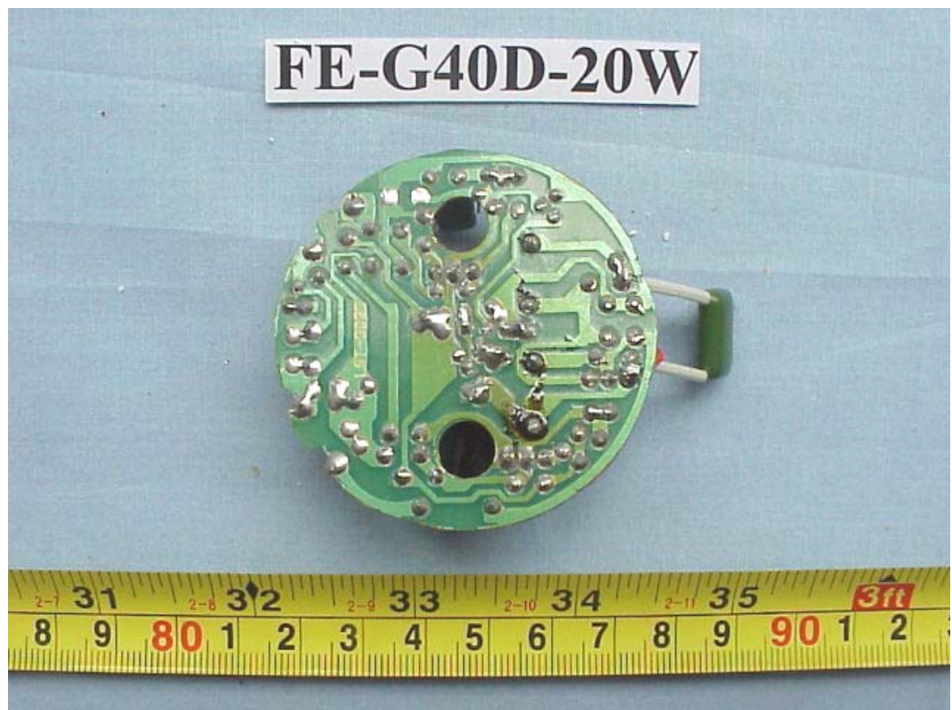
FIGURE 114 ENERGY SAVING LAMP (M/N: FE-G40D-20W) MAIN BOARD (SOLDERED SIDE)
