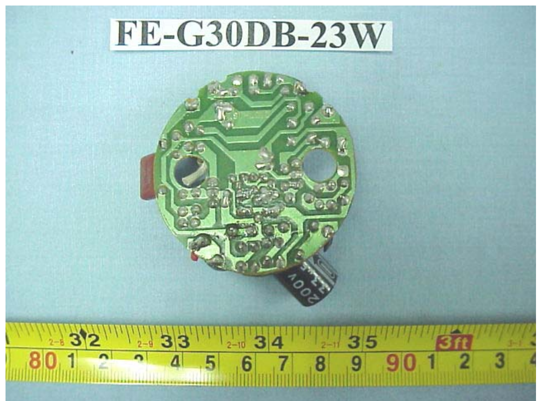
FIGURE 111 ENERGY SAVING LAMP (M/N: FE-G30DB-23W) MAIN BOARD (SOLDERED SIDE)
