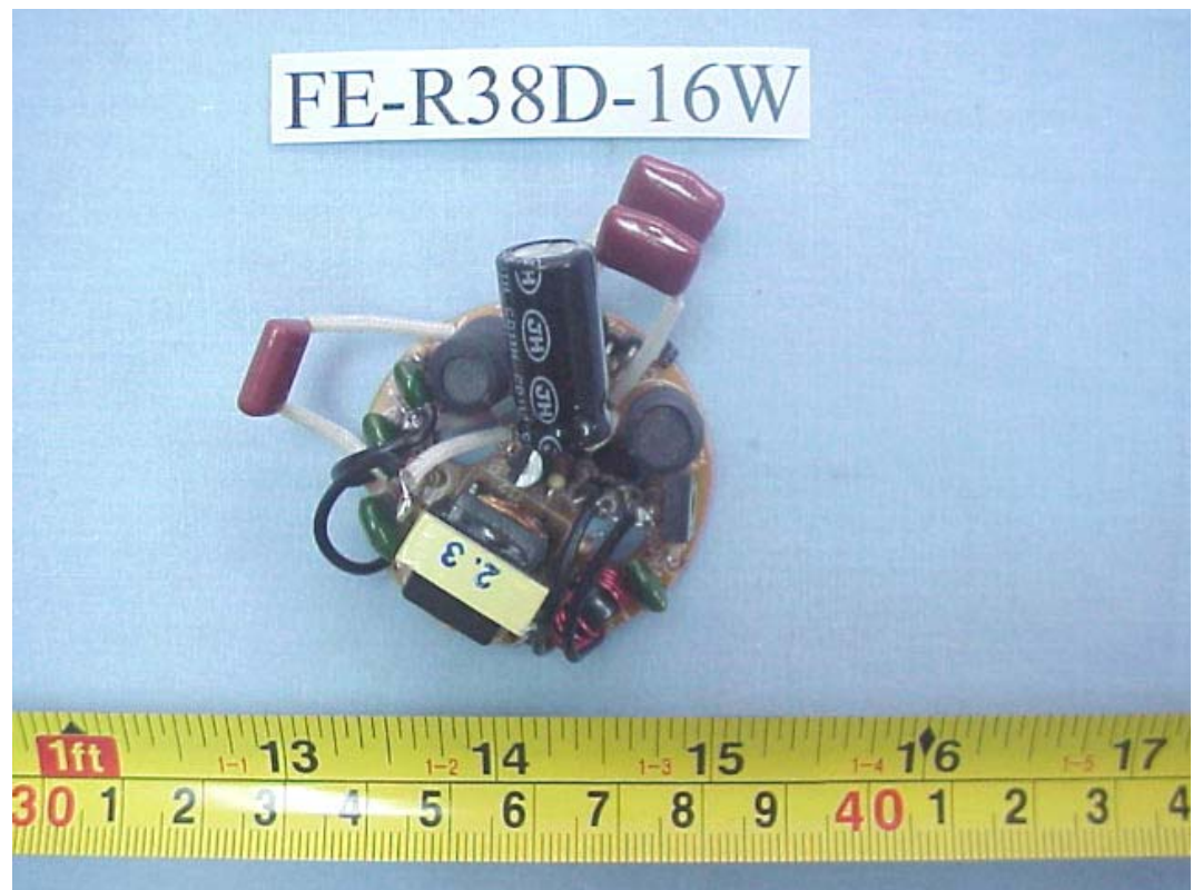
FIGURE 77 ENERGY SAVING LAMP (M/N: FE-R38D-16W) MAIN BOARD (COMPONENT SIDE)
