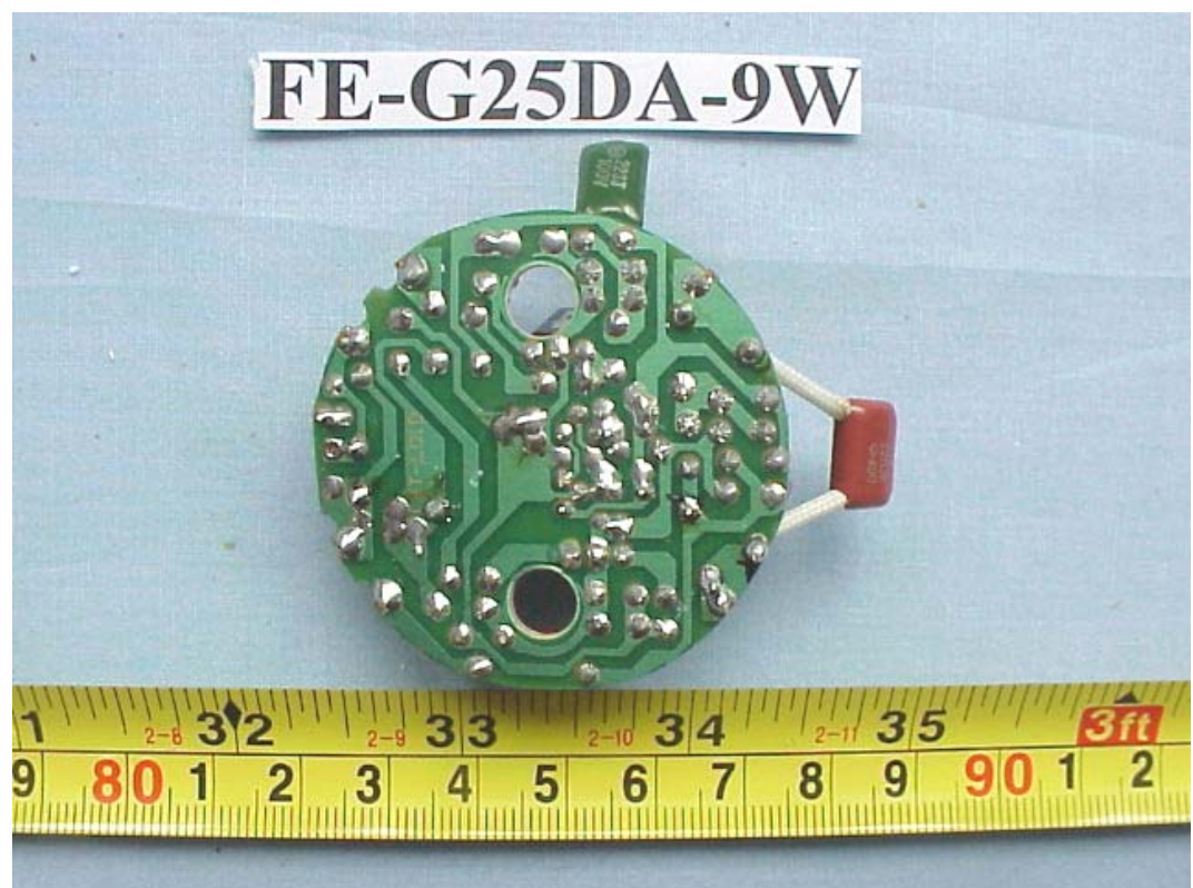
FIGURE 90 ENERGY SAVING LAMP (M/N: FE-G25DA-9W) MAIN BOARD (SOLDERED SIDE)
