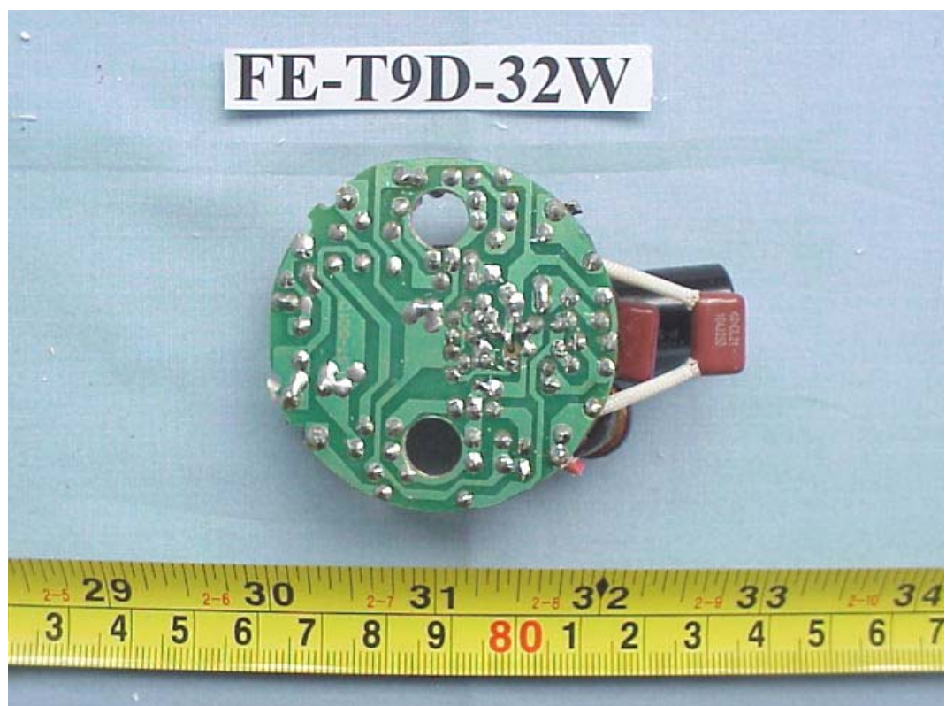
FIGURE 135 ENERGY SAVING LAMP (M/N: FE-T9D-32W) MAIN BOARD (SOLDERED SIDE)
