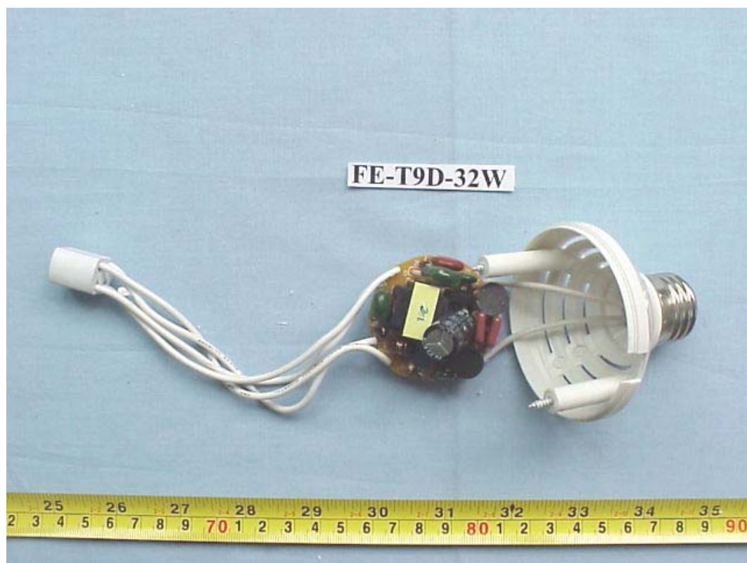
FIGURE 133 ENERGY SAVING LAMP (M/N: FE-T9D-32W) COVER REMOVED
