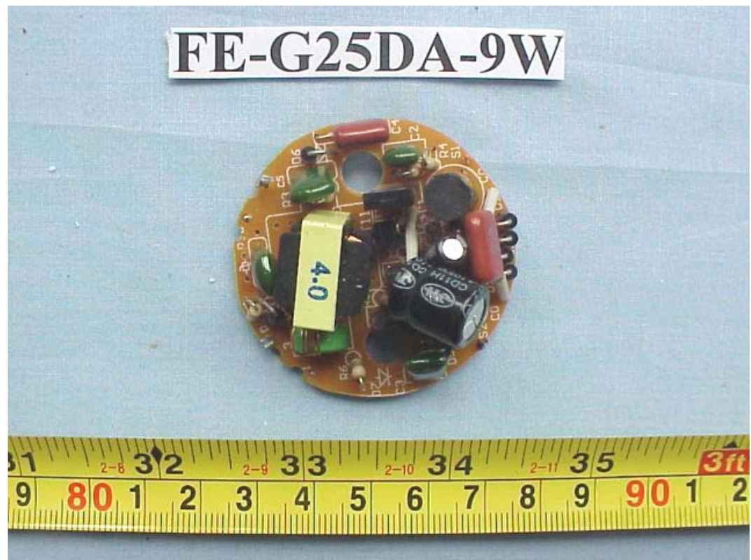
FIGURE 89 ENERGY SAVING LAMP (M/N: FE-G25DA-9W) MAIN BOARD (COMPONENT SIDE)
