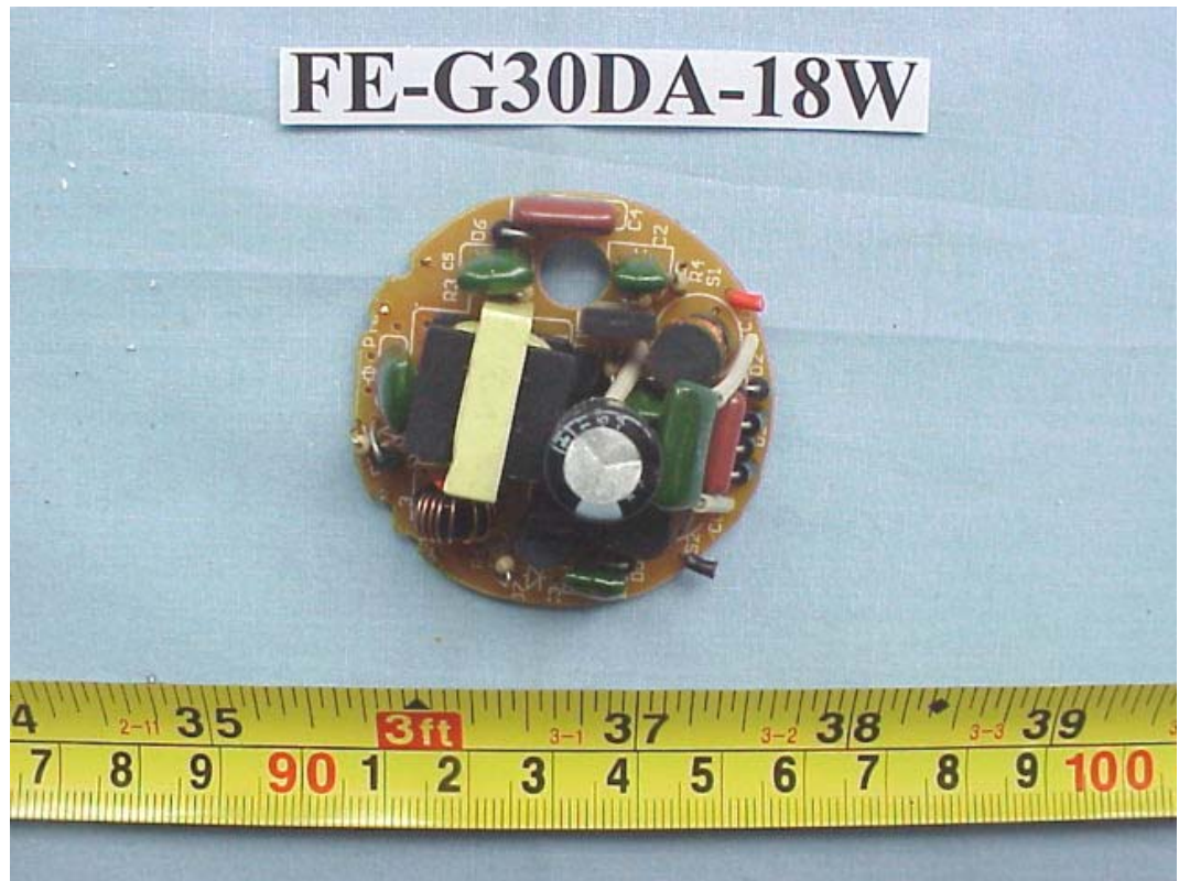
FIGURE 104 ENERGY SAVING LAMP (M/N: FE-G30DA-18W) MAIN BOARD (COMPONENT SIDE)
