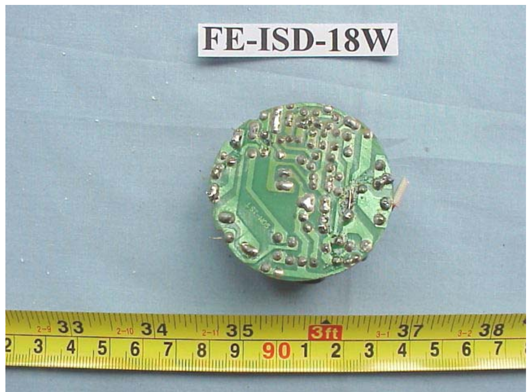
FIGURE 45 ENERGY SAVING LAMP (M/N: FE- ISD-18W) MAIN BOARD (SOLDERED SIDE)
