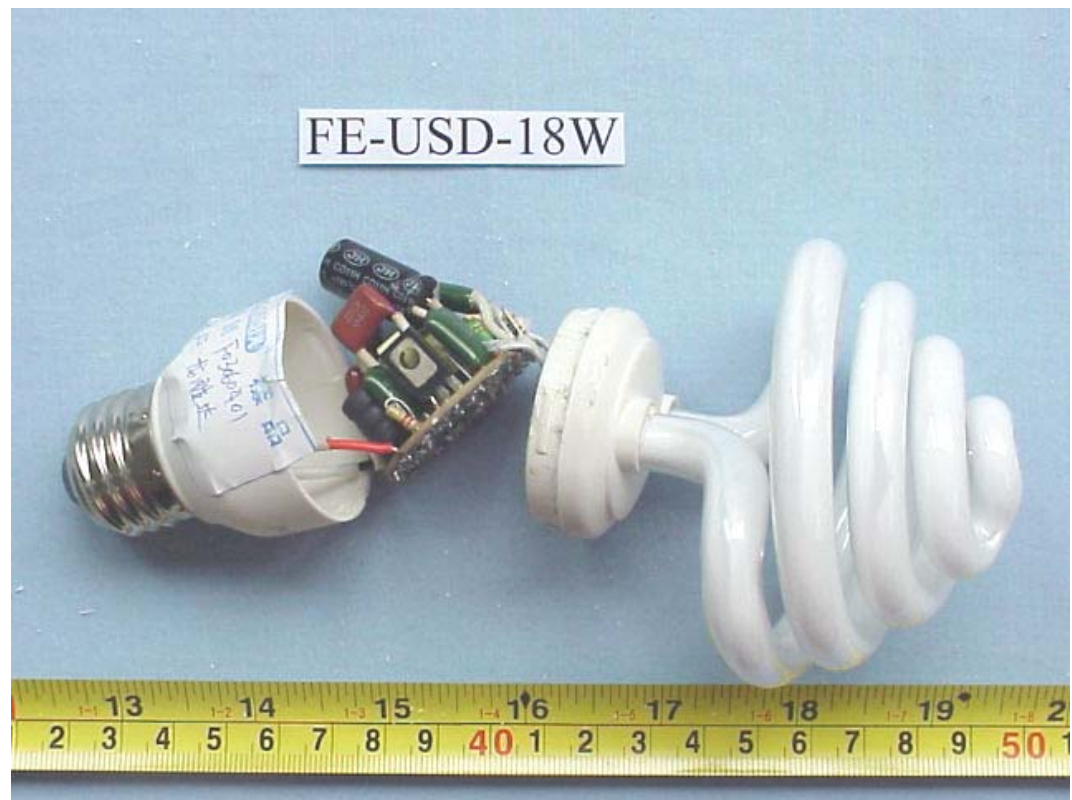
FIGURE 25 ENERGY SAVING LAMP (M/N: FE-USD-18W) COVER REMOVED
