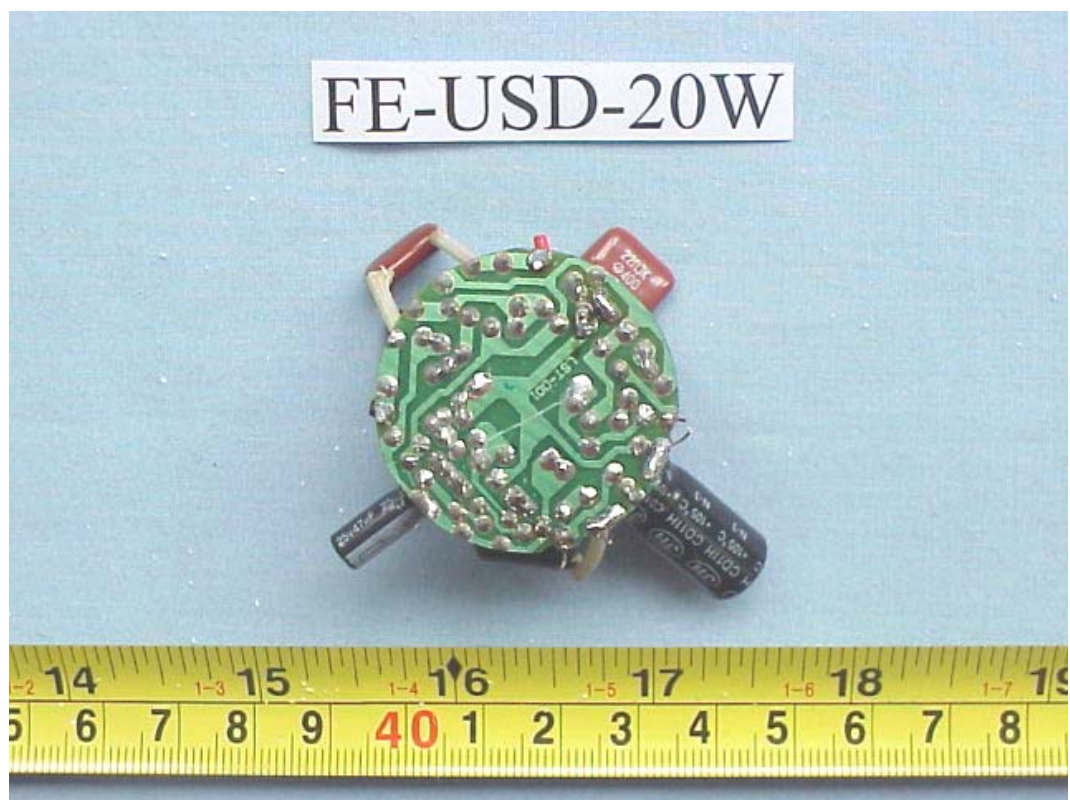
FIGURE 30 ENERGY SAVING LAMP (M/N: FE-USD-20W) MAIN BOARD (SOLDERED SIDE)
