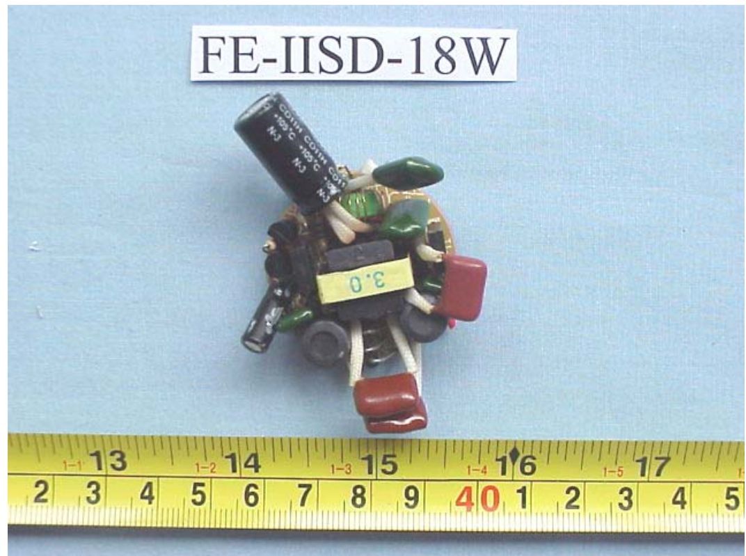
FIGURE 14 ENERGY SAVING LAMP (M/N: FE-IISD-18W) MAIN BOARD (COMPONENT SIDE)
