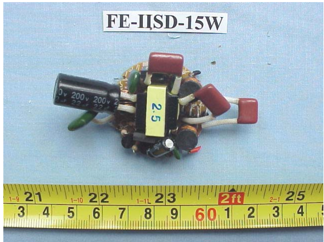
FIGURE 11 ENERGY SAVING LAMP (M/N: FE-IIISD-15W) MAIN BOARD (COMPONENT SIDE)
