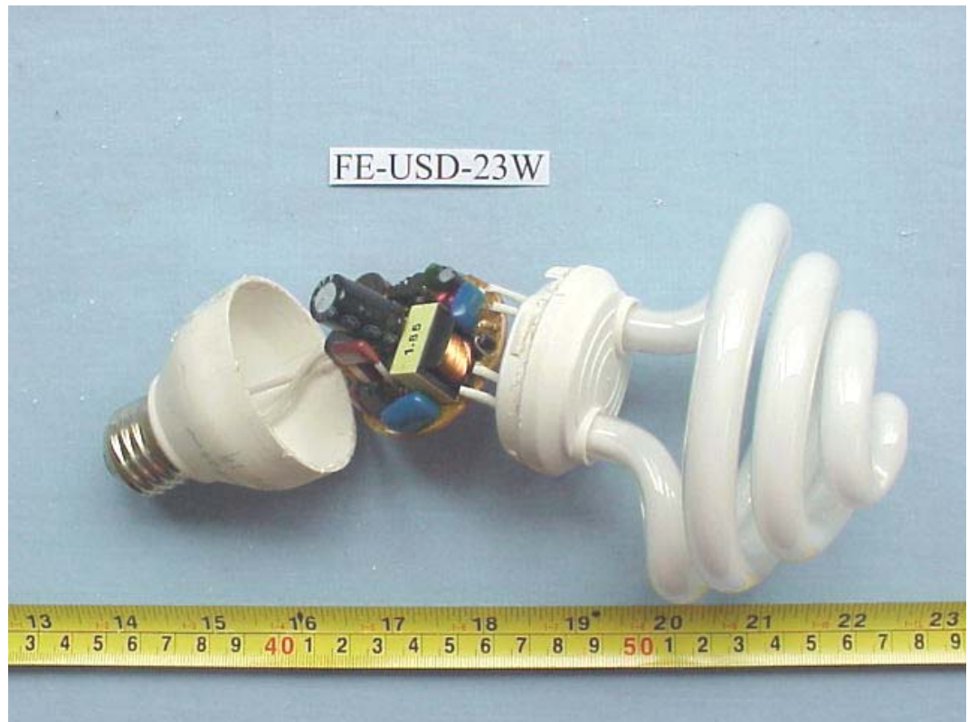
FIGURE 31 ENERGY SAVING LAMP (M/N: FE-USD-23W) COVER REMOVED
