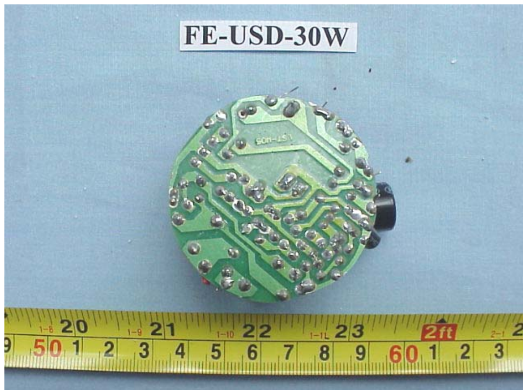
FIGURE 39 ENERGY SAVING LAMP (M/N: FE-USD-30W) MAIN BOARD (SOLDERED SIDE)
