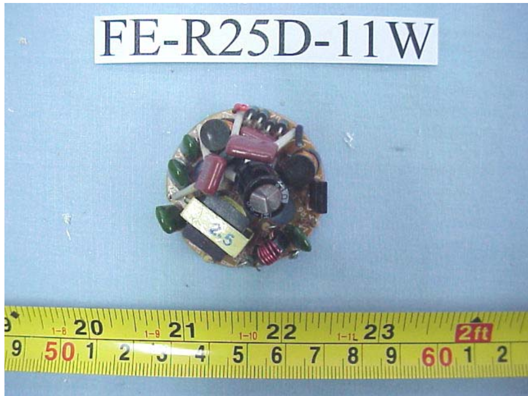
FIGURE 65 ENERGY SAVING LAMP (M/N: FE-R25D-11W) MAIN BOARD (COMPONENT SIDE)
