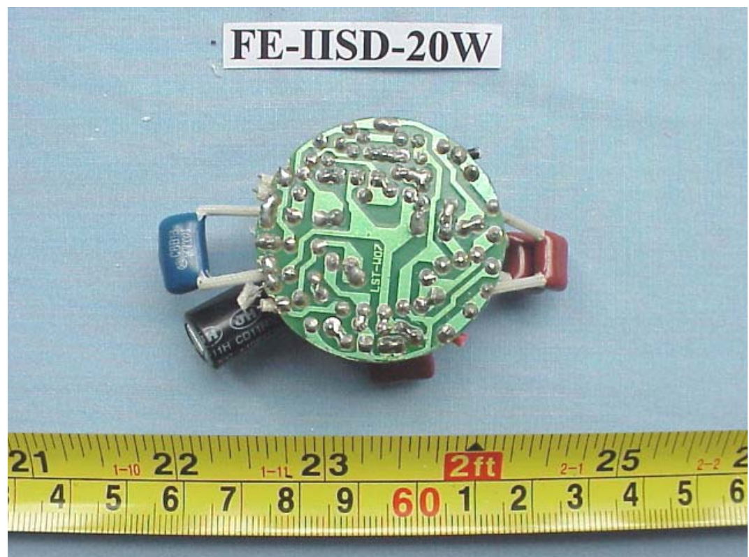
FIGURE 18 ENERGY SAVING LAMP (M/N: FE-IISD-20W) MAIN BOARD (SOLDERED SIDE)
