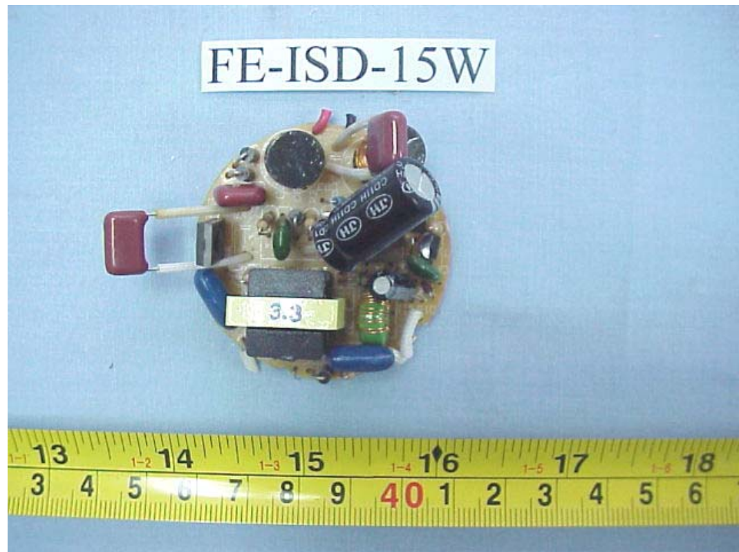
FIGURE 41 ENERGY SAVING LAMP (M/N: FE- ISD-15W) MAIN BOARD (COMPONENT SIDE)
