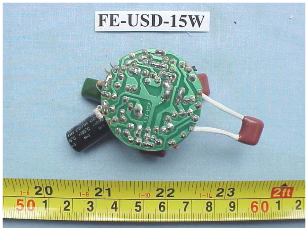
FIGURE 24 ENERGY SAVING LAMP (M/N: FE-USD-15W) MAIN BOARD (SOLDERED SIDE)
