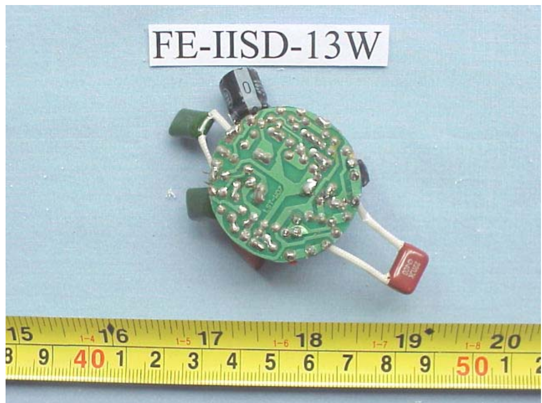
FIGURE 9 ENERGY SAVING LAMP (M/N: FE-IISD-13W) MAIN BOARD (SOLDERED SIDE)
