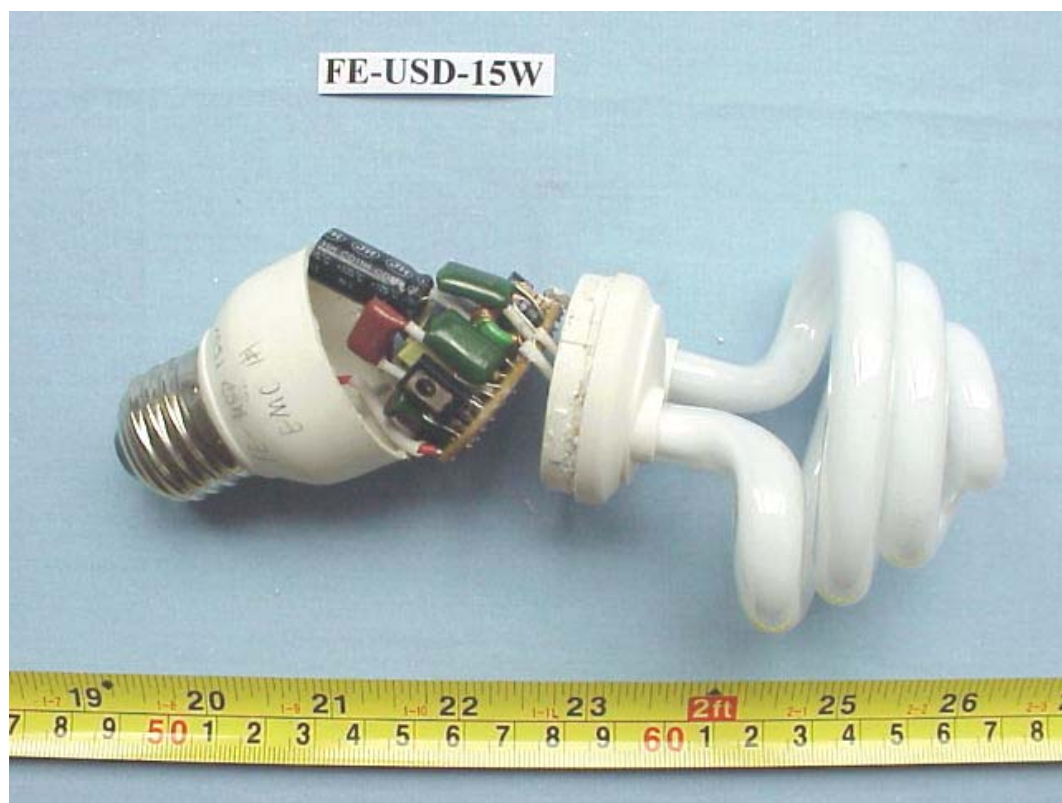
FIGURE 22 ENERGY SAVING LAMP (M/N: FE-USD-15W) COVER REMOVED
