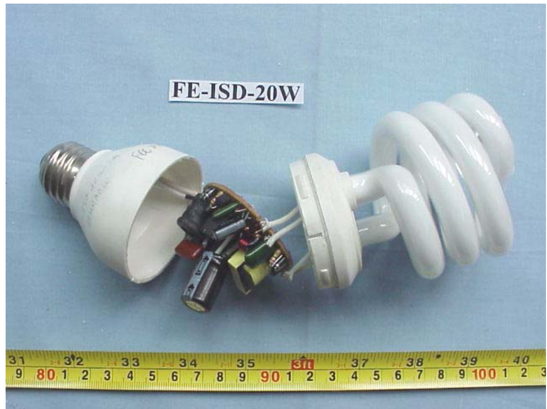
FIGURE 46 ENERGY SAVING LAMP (M/N: FE- ISD-20W) COVER REMOVED
