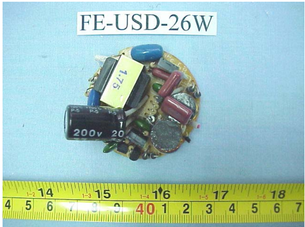
FIGURE 35 ENERGY SAVING LAMP (M/N: FE-USD-26W) MAIN BOARD (COMPONENT SIDE)
