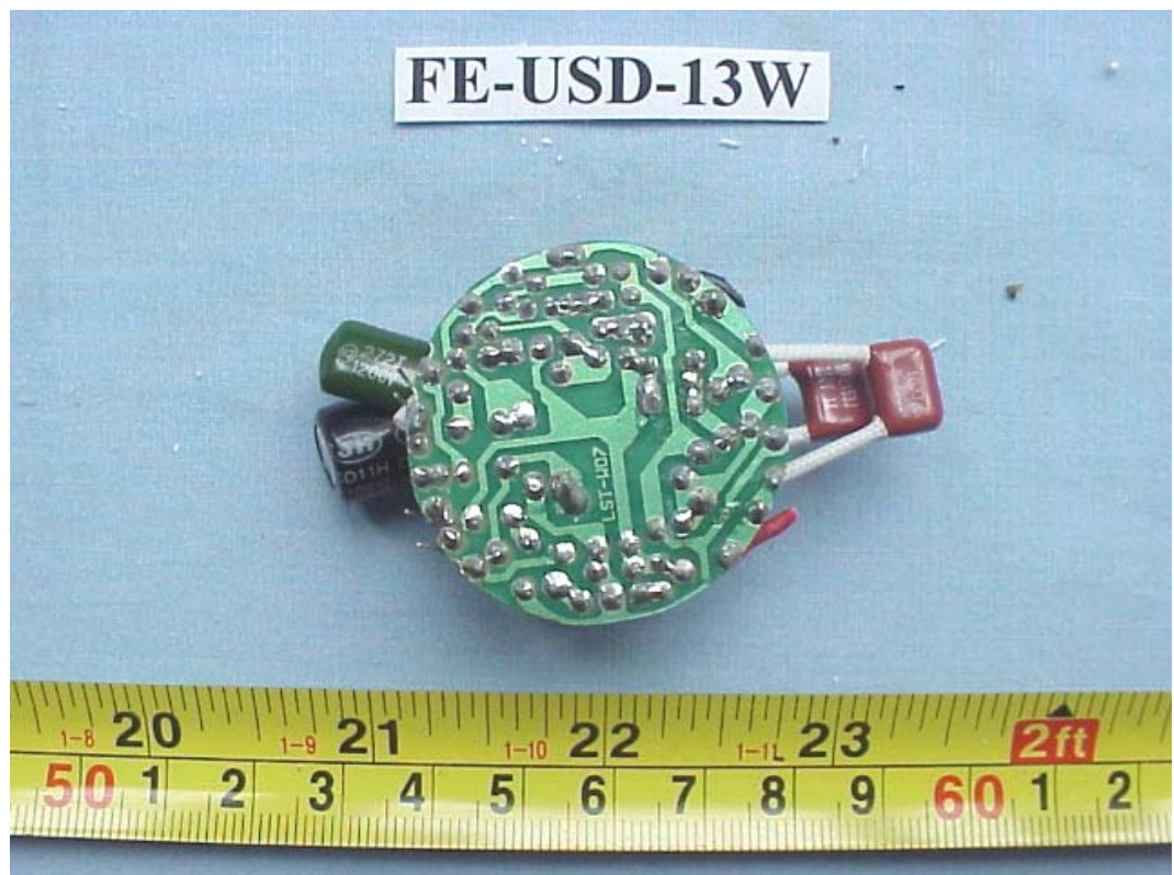
FIGURE 21 ENERGY SAVING LAMP (M/N: FE-USD-13W) MAIN BOARD (SOLDERED SIDE)
