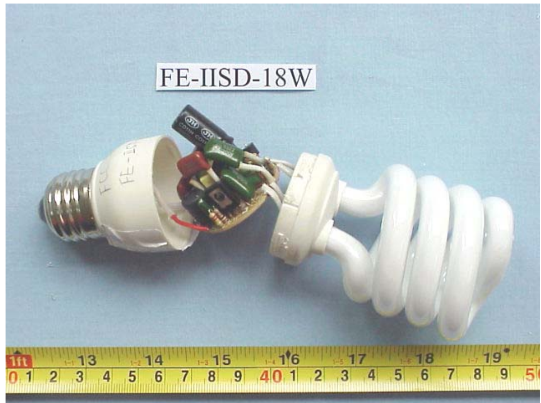
FIGURE 13 ENERGY SAVING LAMP (M/N: FE-IIISD-18W) COVER REMOVED
