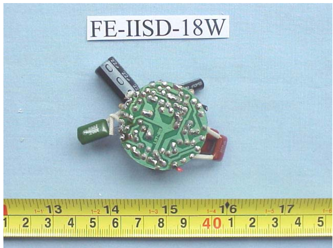
FIGURE 15 ENERGY SAVING LAMP (M/N: FE-IISD-18W) MAIN BOARD (SOLDERED SIDE)
