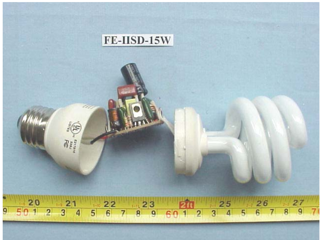
FIGURE 10 ENERGY SAVING LAMP (M/N: FE-IIISD-15W) COVER REMOVED
