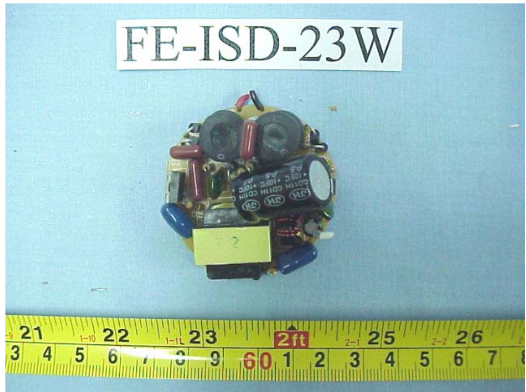
FIGURE 50 ENERGY SAVING LAMP (M/N: FE- I SD-23(24)W) MAIN BOARD (COMPONENT SIDE)
