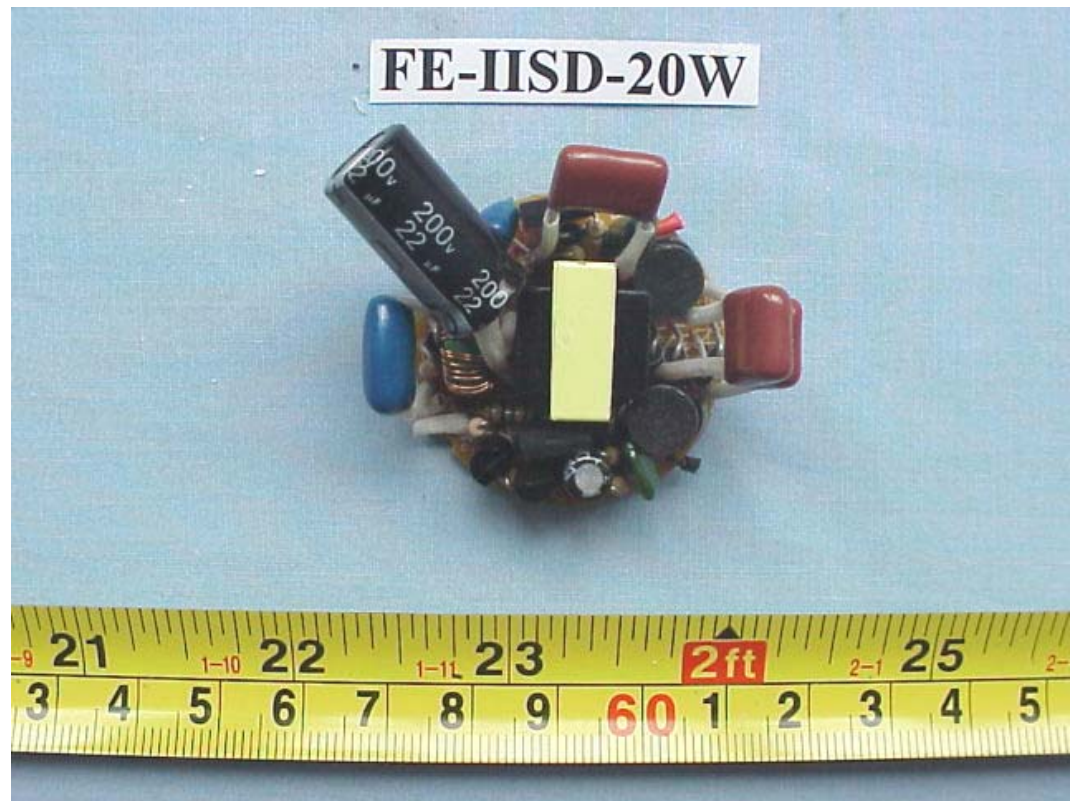
FIGURE 17 ENERGY SAVING LAMP (M/N: FE-IISD-20W) MAIN BOARD (COMPONENT SIDE)
