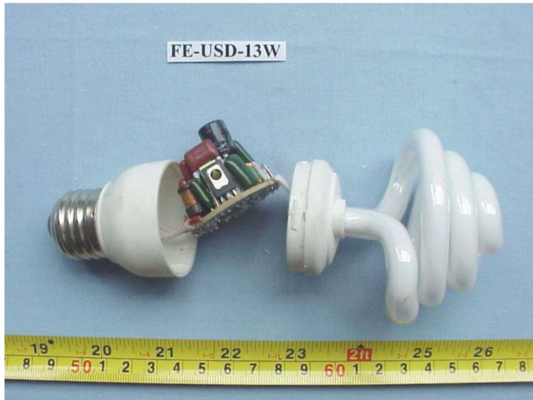
FIGURE 19 ENERGY SAVING LAMP (M/N: FE-USD-13W) COVER REMOVED
