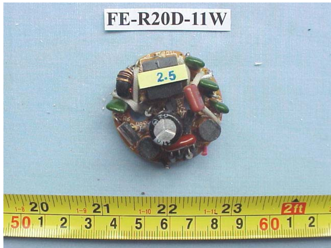
FIGURE 62 ENERGY SAVING LAMP (M/N: FE-R20D-11W) MAIN BOARD (COMPONENT SIDE)
