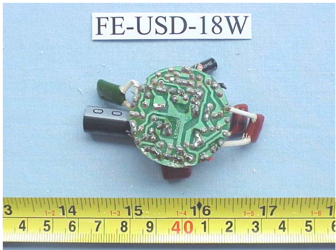
FIGURE 27 ENERGY SAVING LAMP (M/N: FE-USD-18W) MAIN BOARD (SOLDERED SIDE)
