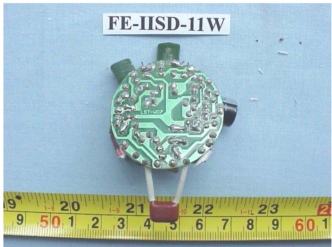
FIGURE 6 ENERGY SAVING LAMP (M/N: FE-IISD-11W) MAIN BOARD (SOLDERED SIDE)
