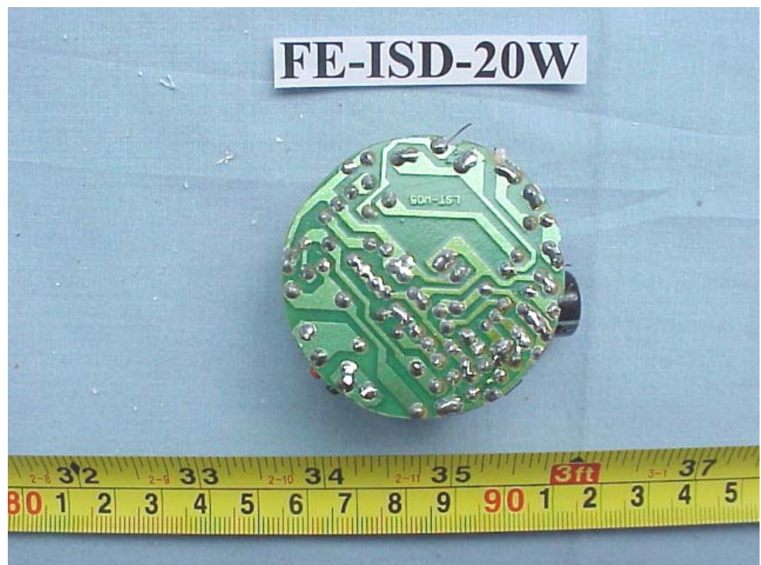
FIGURE 48 ENERGY SAVING LAMP (M/N: FE- I SD-20W) MAIN BOARD (SOLDERED SIDE)
