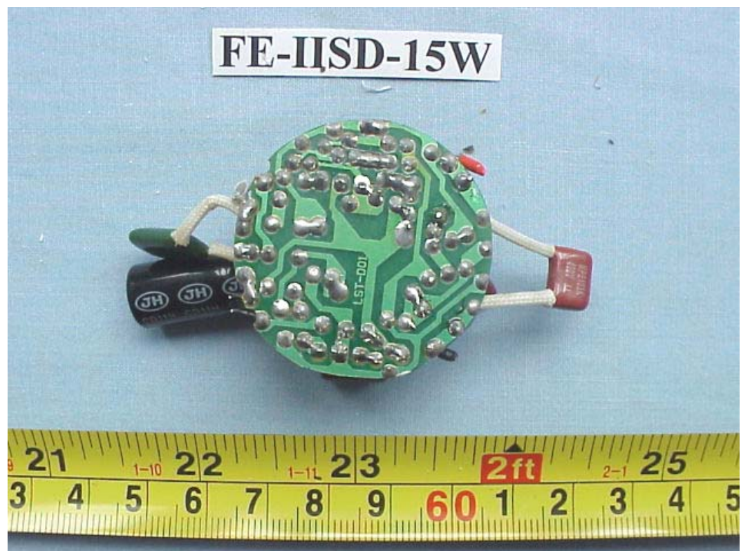
FIGURE 12 ENERGY SAVING LAMP (M/N: FE-IIISD-15W) MAIN BOARD (SOLDERED SIDE)
