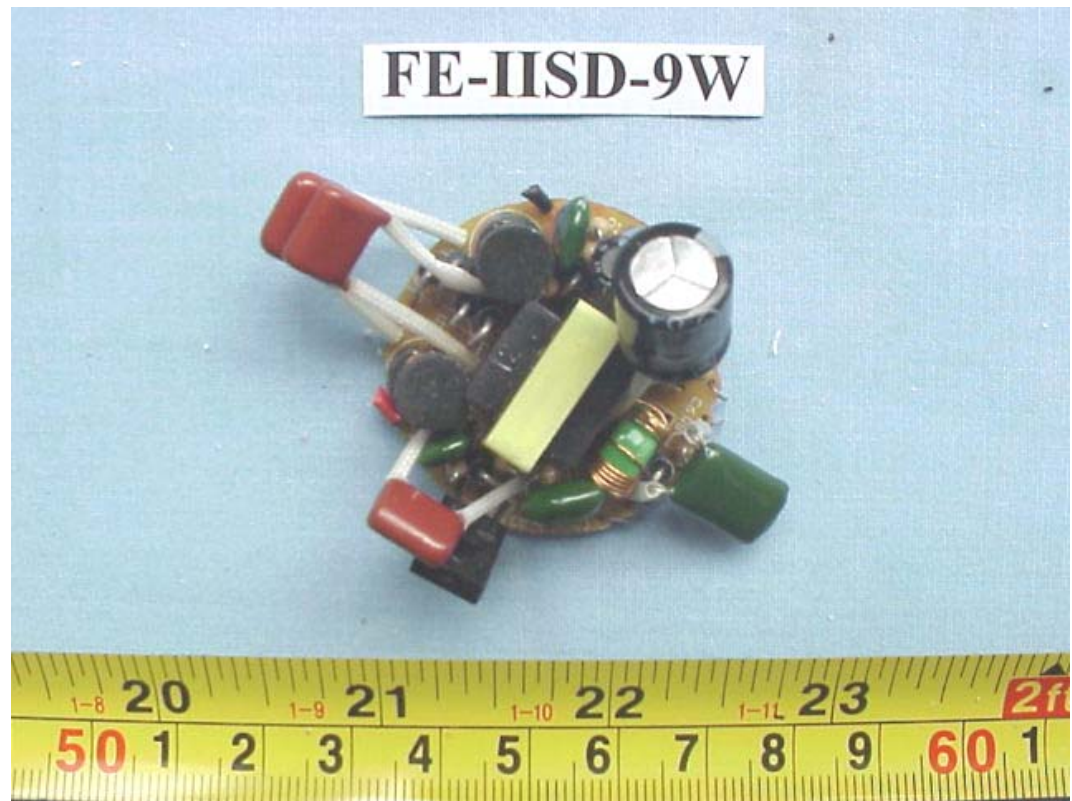
FIGURE 2 ENERGY SAVING LAMP (M/N: FE-IISD-9W) MAIN BOARD (COMPONENT SIDE)
