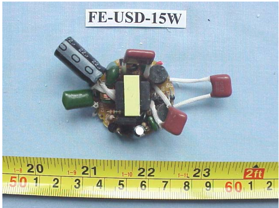
FIGURE 23 ENERGY SAVING LAMP (M/N: FE-USD-15W) MAIN BOARD (COMPONENT SIDE)
