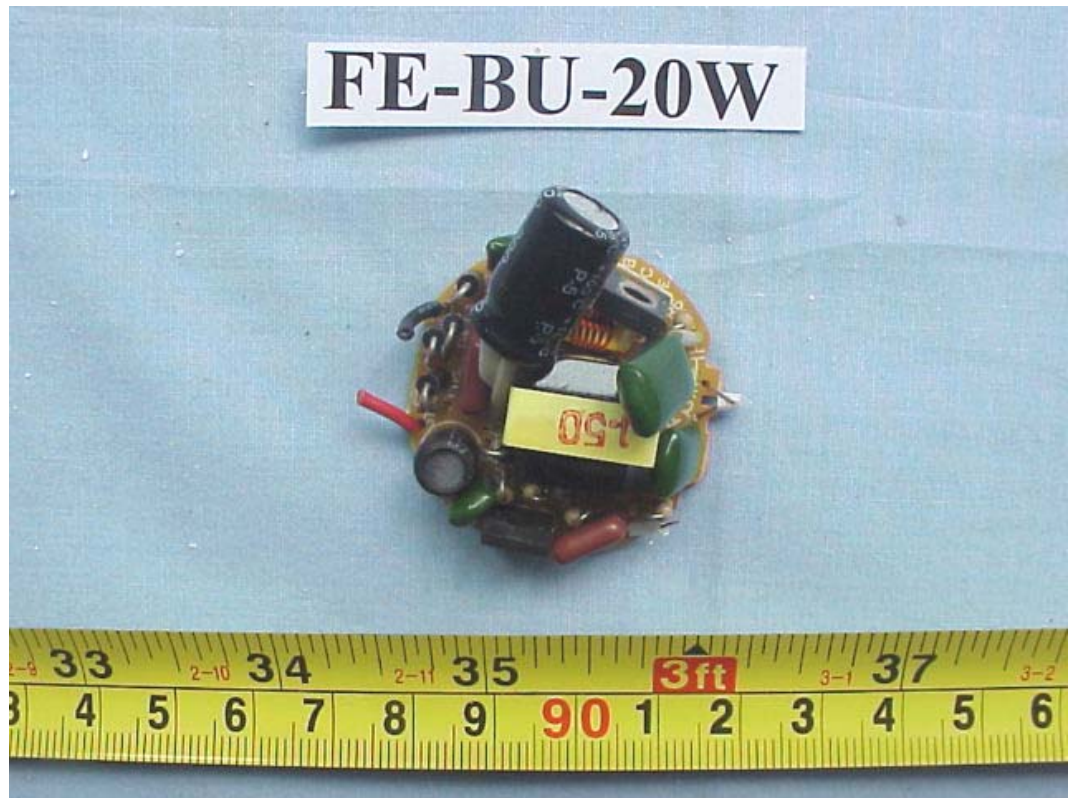
FIGURE 19 ENERGY SAVING LAMP (M/N: FE-BU-20W) MAIN BOARD (COMPONENT SIDE)
