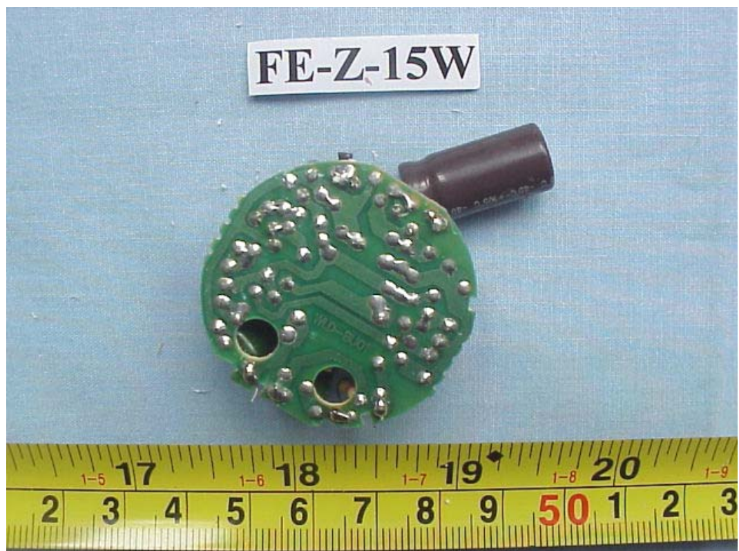
FIGURE 28 ENERGY SAVING LAMP (M/N: FE-Z-15W) MAIN BOARD (SOLDERED SIDE)
