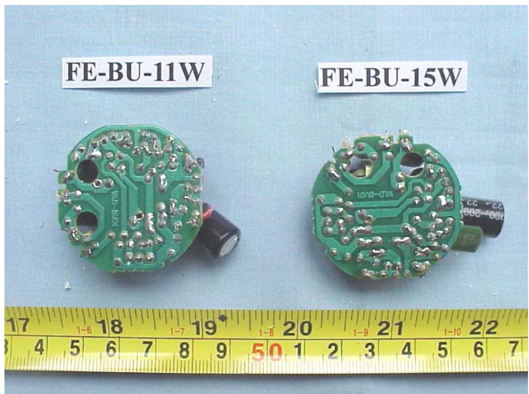
FIGURE 8 ENERGY SAVING LAMP (M/N: FE-BU-11/15W) MAIN BOARD (SOLDERED SIDE)
