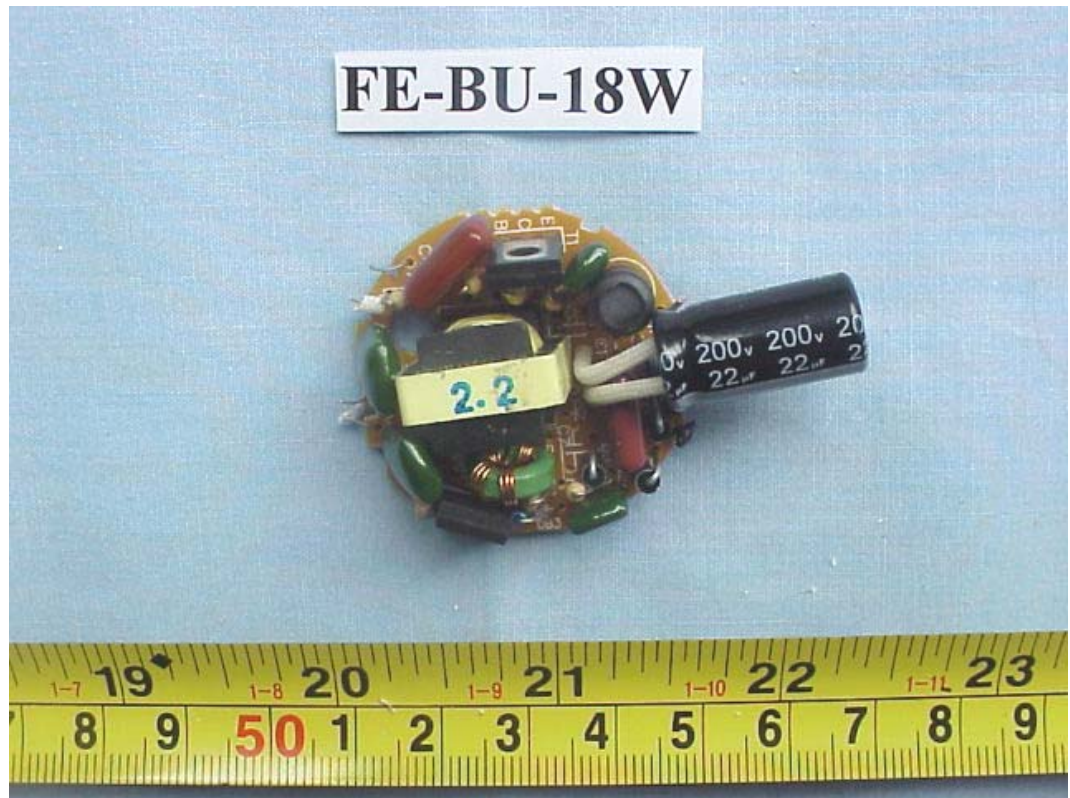
FIGURE 15 ENERGY SAVING LAMP (M/N: FE-BU-18W) MAIN BOARD (COMPONENT SIDE)
