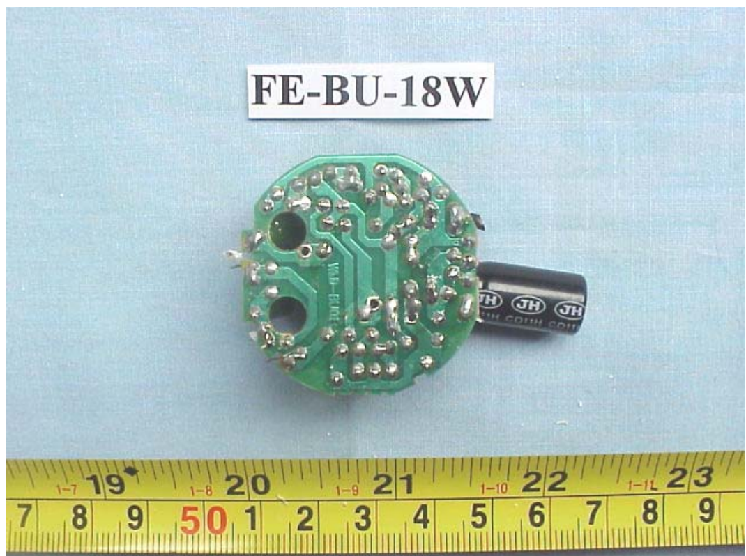
FIGURE 16 ENERGY SAVING LAMP (M/N: FE-BU-18W) MAIN BOARD (SOLDERED SIDE)
