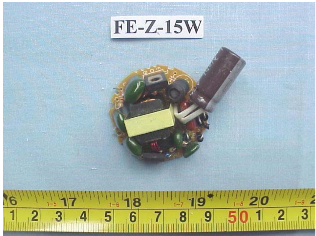
FIGURE 27 ENERGY SAVING LAMP (M/N: FE-Z-15W) MAIN BOARD (COMPONENT SIDE)
