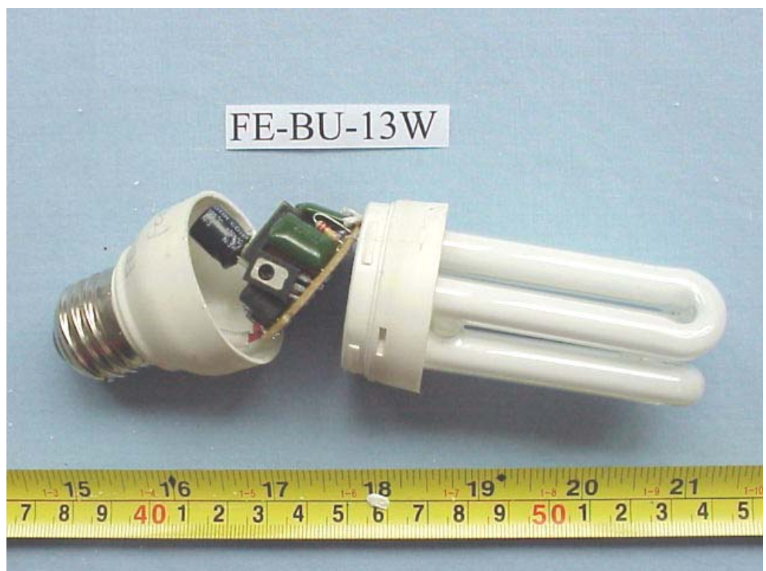
FIGURE 10 ENERGY SAVING LAMP (M/N: FE-BU-13W) COVER REMOVED 2
