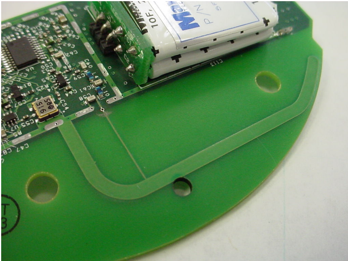
Photo Five – Internal Printed Circuit Board Antenna
