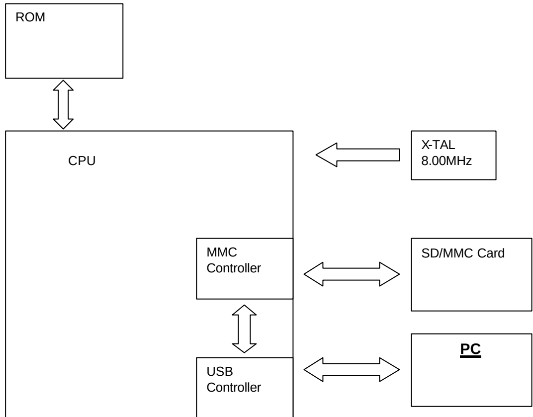
SD/MMC Read Writer Block Diagram
