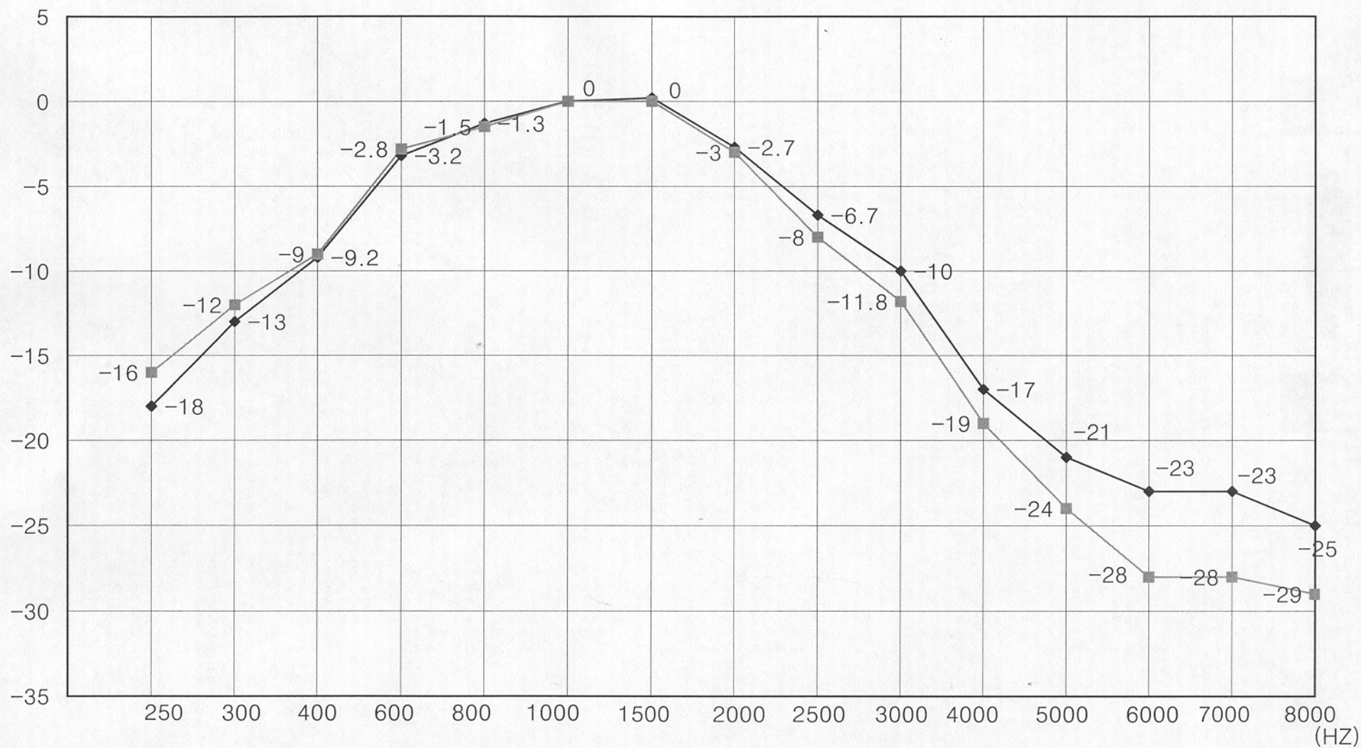
(DB) TX Audio Low Pass Filter Response
