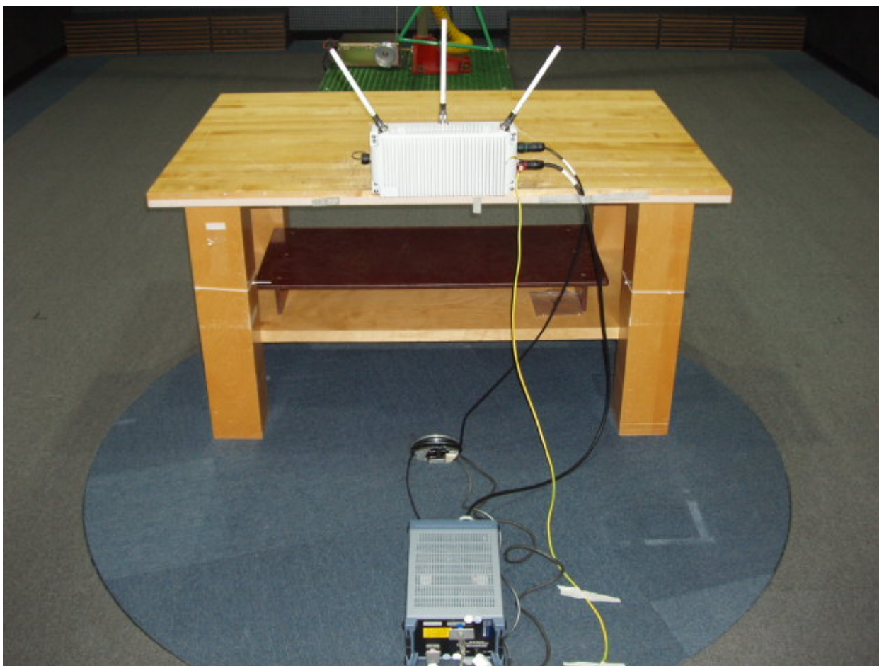
Photo 4.4-2 – Rear View of Conducted Emissions Test Set-up
