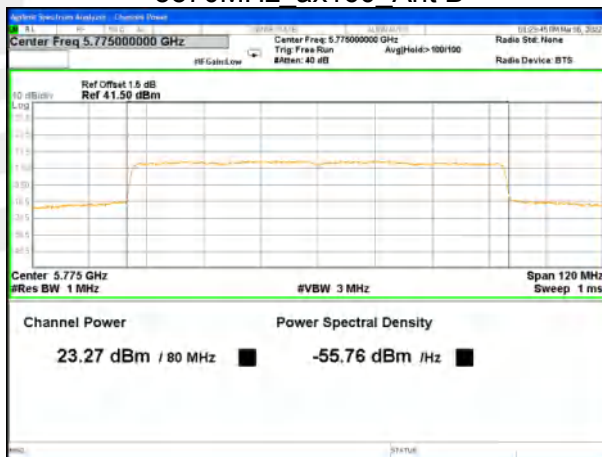
5775MHz_ax80_Ant B
