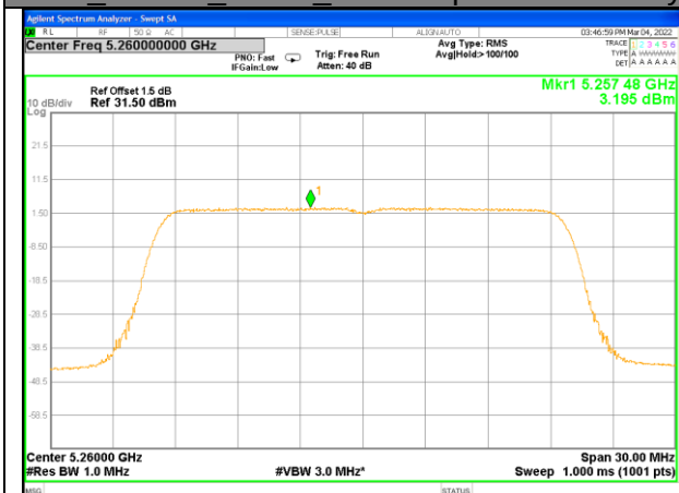
W53_11ax20_Higher_Power Spectrum Density
