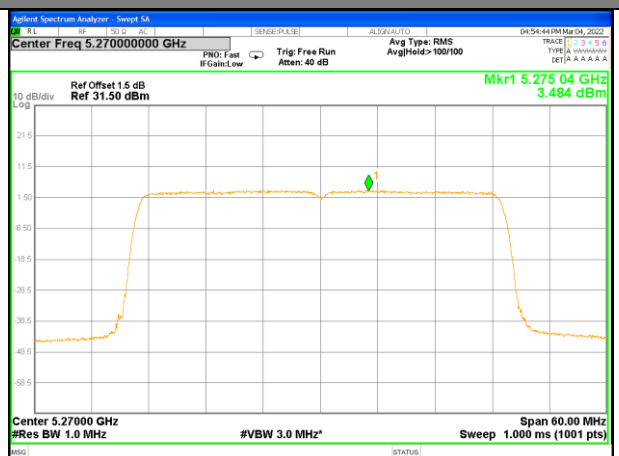
W53_11ax40_Lower_Power Spectrum Density
