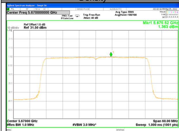
W56_11ax40_Higher_Power Spectrum Density
