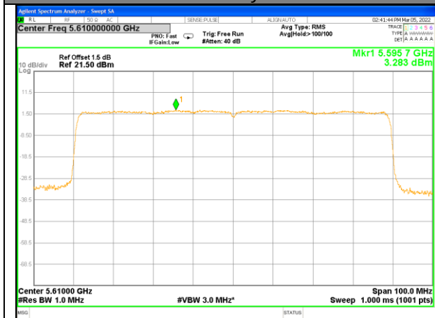
W56_11ax80_Higher_Power Spectrum Density
