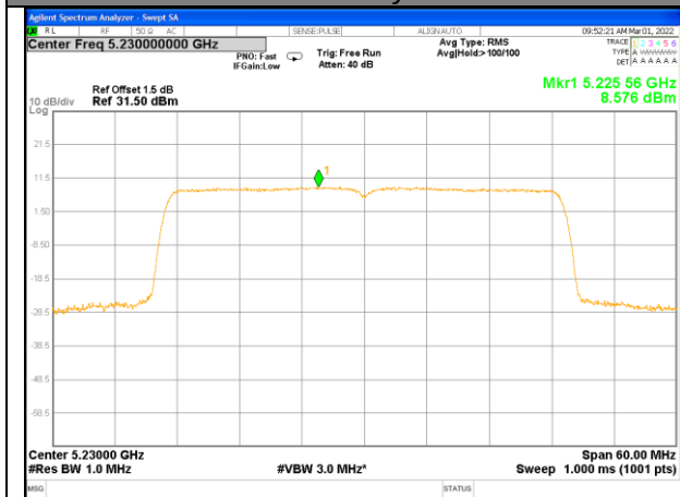
W52_11ax40_Higher_Power Spectrum Density
