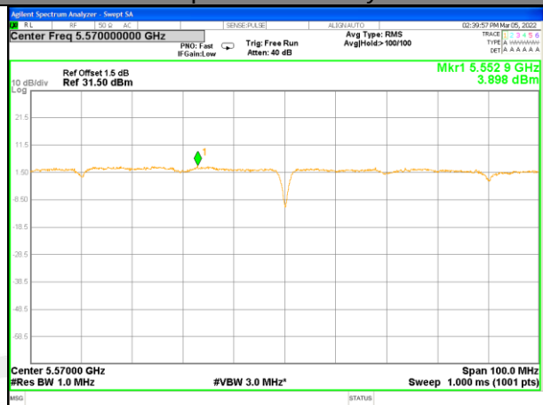
W56_11ax160_CH114(5570MHz)_Power Spectrum Density
