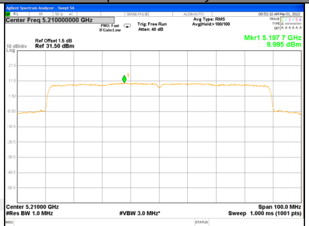
W52_11ax80_CH42(5210MHz)_Power Spectrum Density
