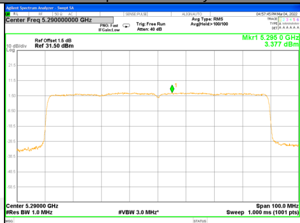
W53_11ax80_CH58(5290MHz)_Power Spectrum Density
