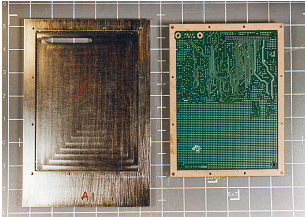
Front PBC, Back With Backing Split
