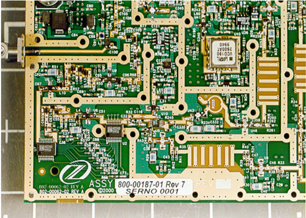
ODU A – Inside Back PCB, Quarter Clasp
