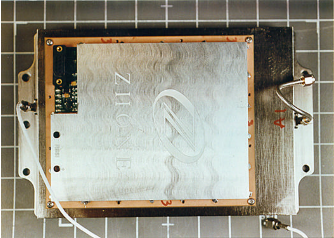
ODU A – Inside Front Without Enclosure Attached
