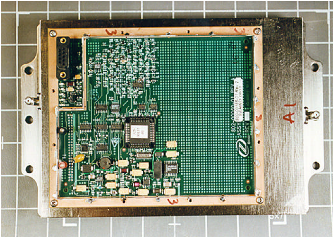
ODU A – Inside Front Without Enclosure & Shielding
