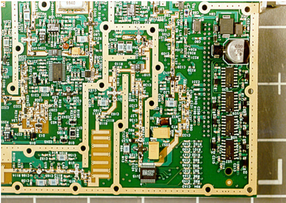
ODU A – Inside Back PCB, Quarter Close-up
