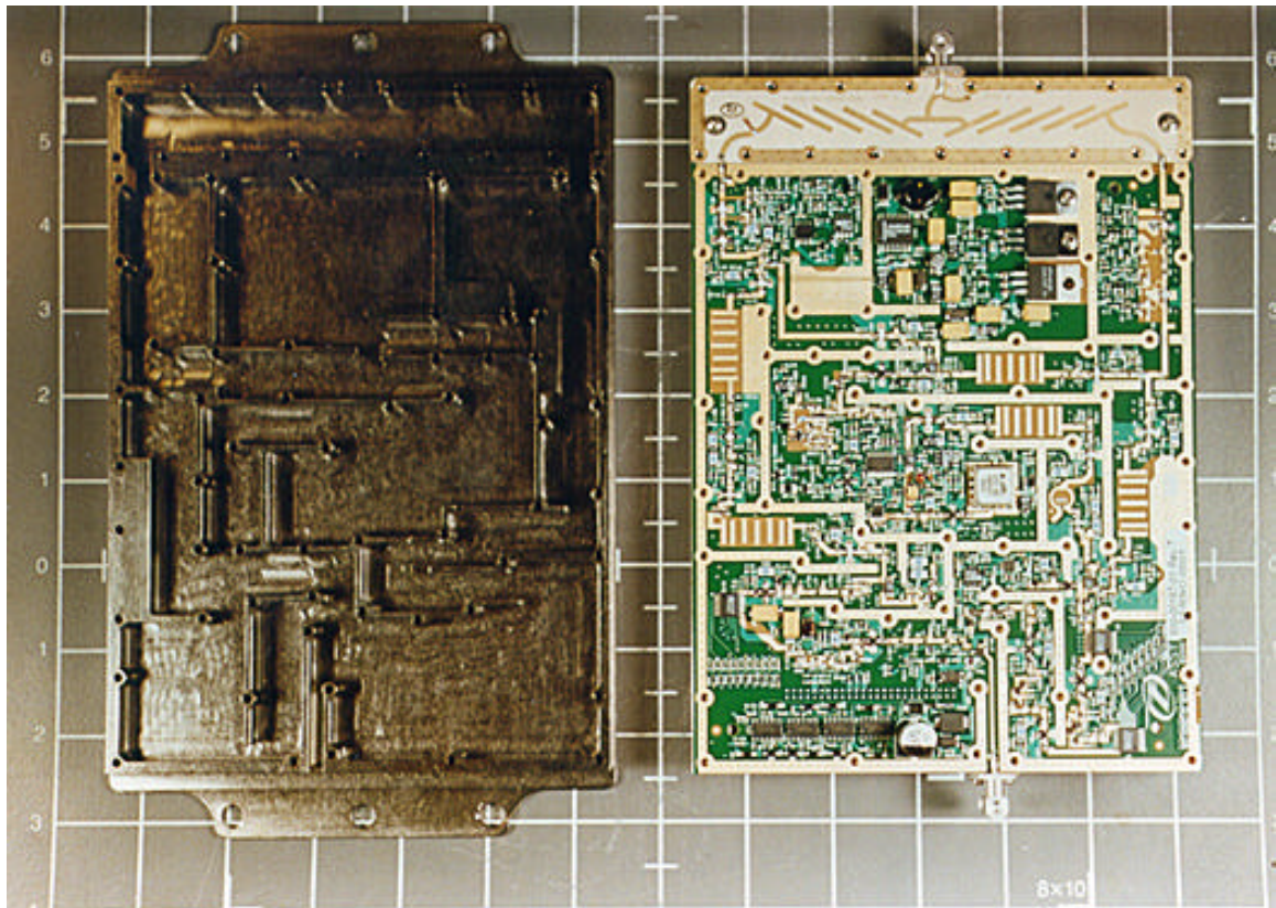
ODU A – Inside Back With Metal Enclosure Split
