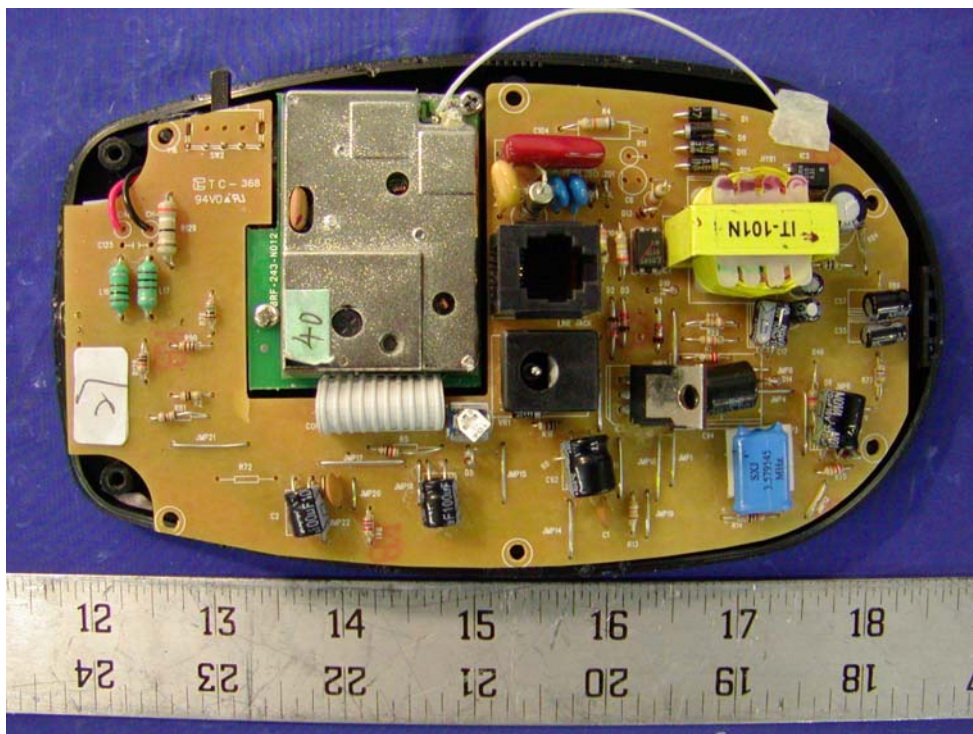
Base - Cover Off View
