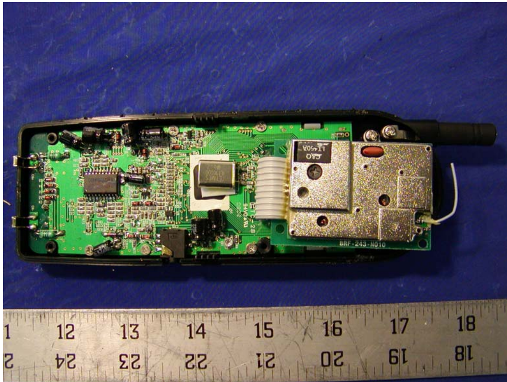
Handset - Cover Off View
