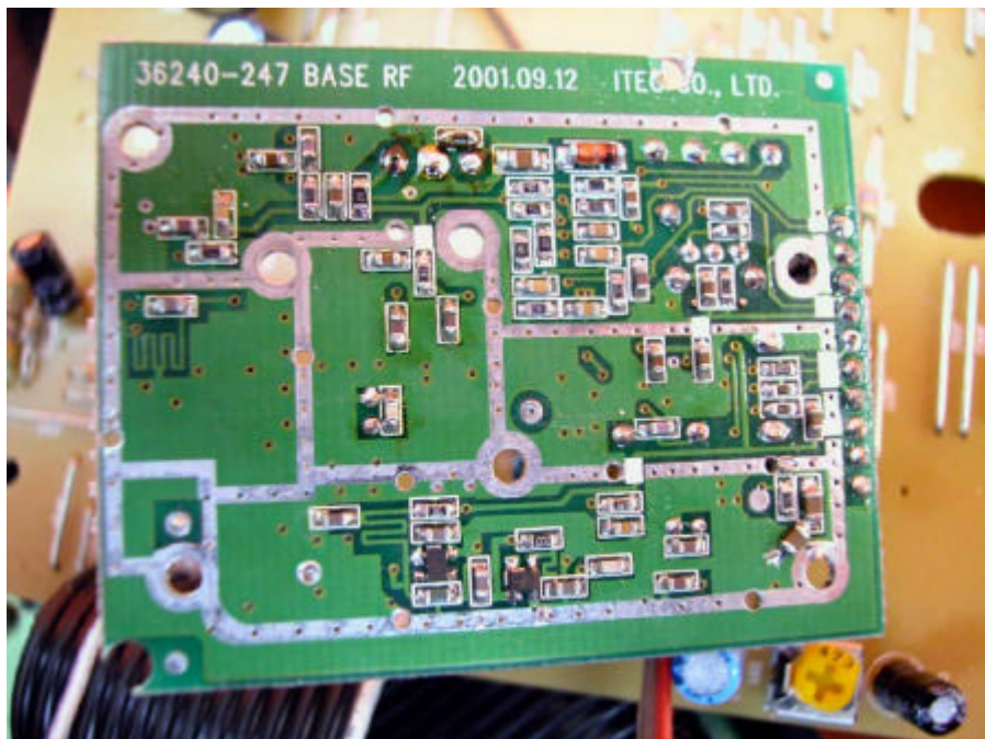
Base Oscillator PCB solder side
