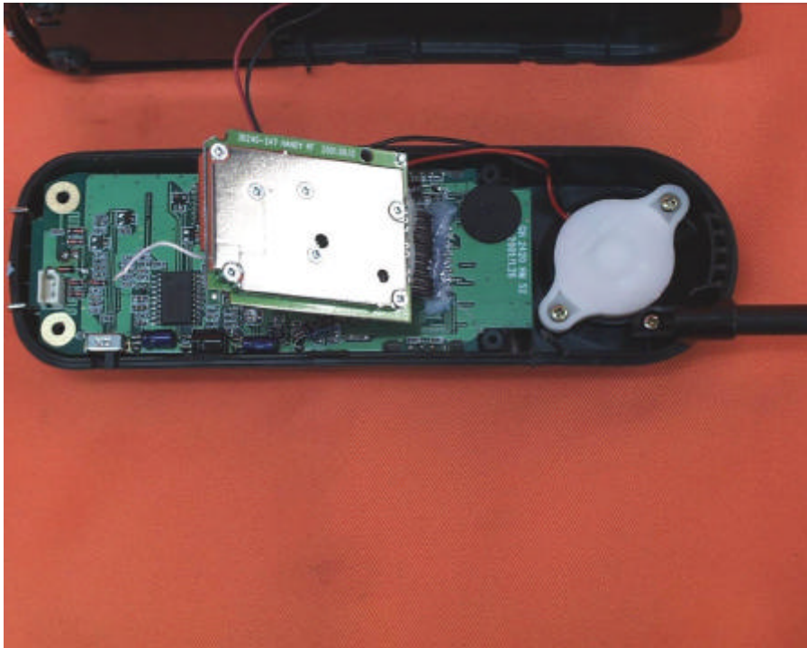
Handset Main PCB comp side (View 2)
