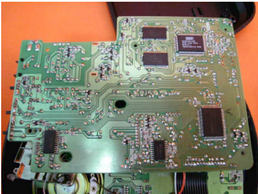
Base Main PCB solder side
