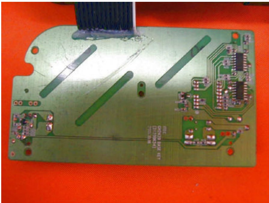
Answering Machine solder side
