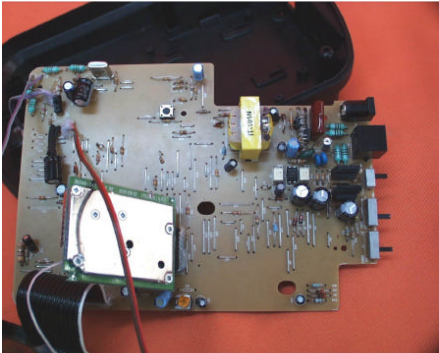
Base Main PCB comp side (View 2)
