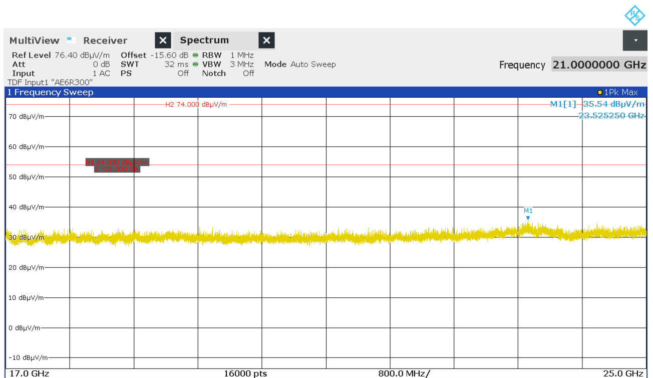
Figure 35: Chart of exploratory emission test from 17 GHz to 25 GHz on middle channel at 0.5 m, EUT position X, antenna polarization vertical
