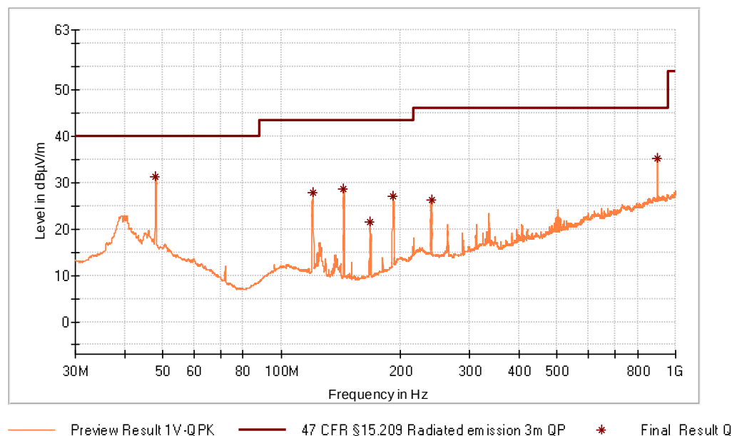
Figure 31: Chart of radiated emissions test from 30 MHz to 1 GHz on lowest channel, EUT position X, antenna polarization vertical
