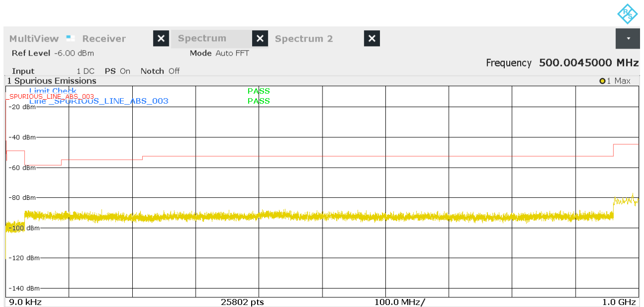
Figure 28: Chart of emissions test from 9 kHz to 1 GHz on highest channel, PK
