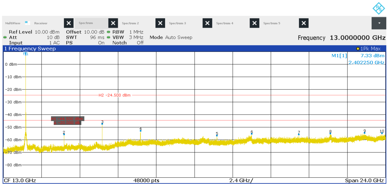
Figure 25: Chart of emissions test from 1 GHz to 25 GHz on lowest channel, Pk
