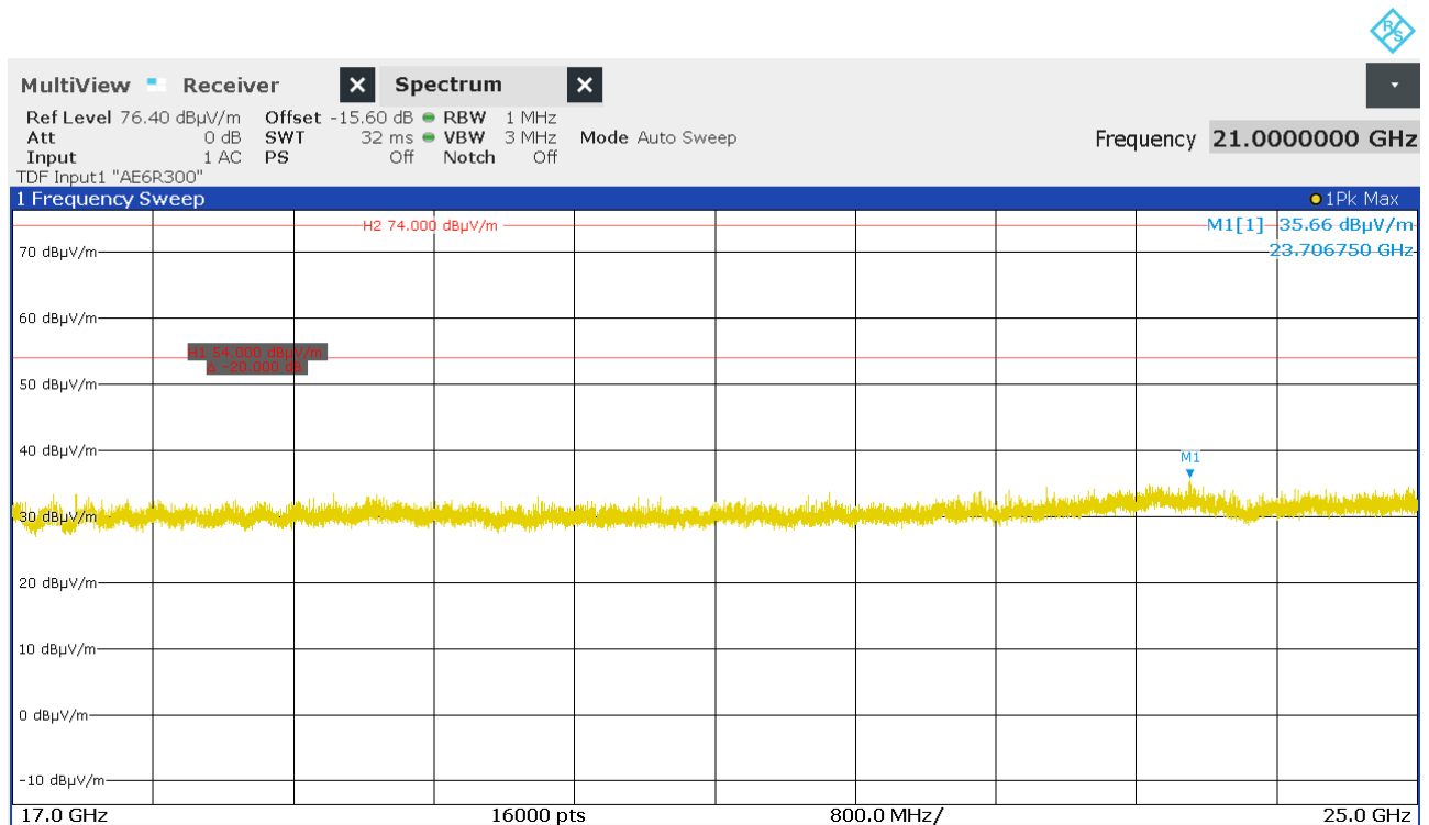
Figure 33: Chart of exploratory emission test from 17 GHz to 25 GHz on lowest channel at 0.5 m, EUT position X, antenna polarization vertical
