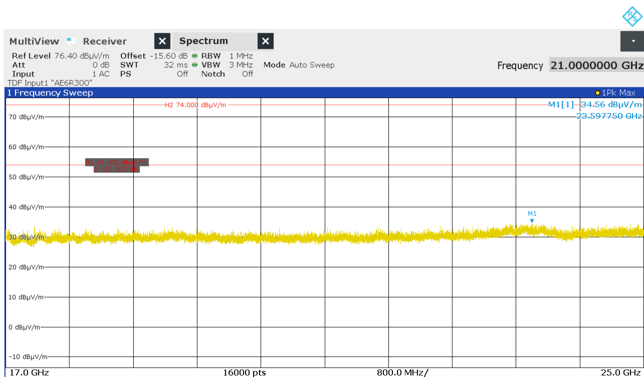
Figure 37: Chart of exploratory emission test from 17 GHz to 25 GHz on highest channel at 0.5 m, EUT position X, antenna polarization vertical
