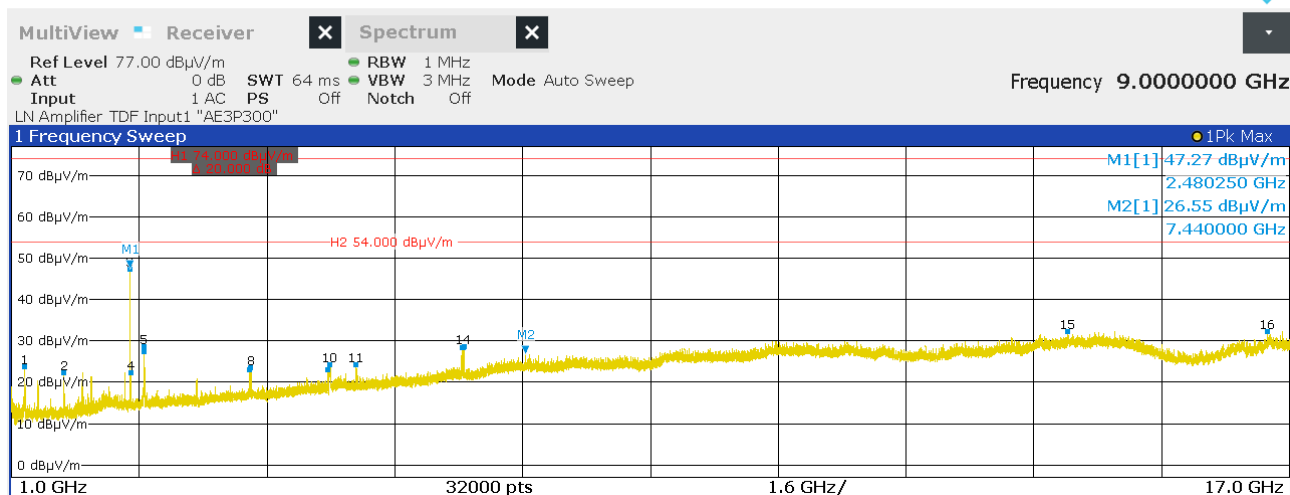
Figure 36: Chart of emissions test from 1 GHz to 17 GHz on highest channel, EUT position Y, antenna polarization vertical
