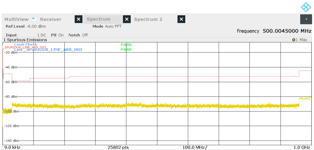
Figure 26: Chart of emissions test from 9 kHz to 1 GHz on middle channel, PK
