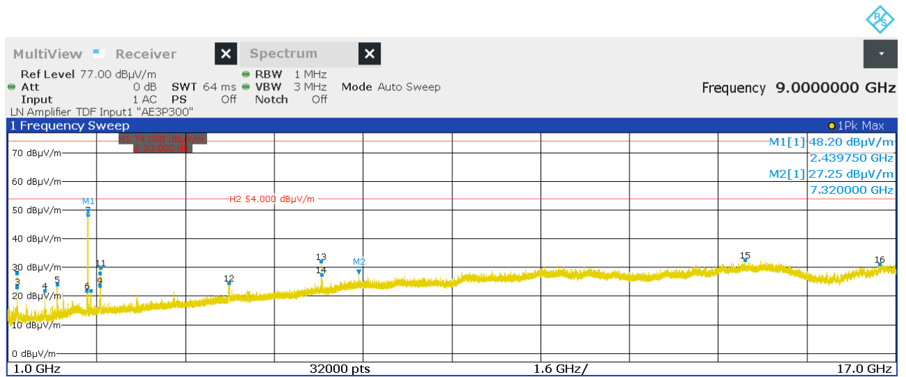
Figure 34: Chart of radiated emissions pre-measurement from 1 GHz to 17 GHz on middle channel, EUT position Y, antenna polarization vertical
