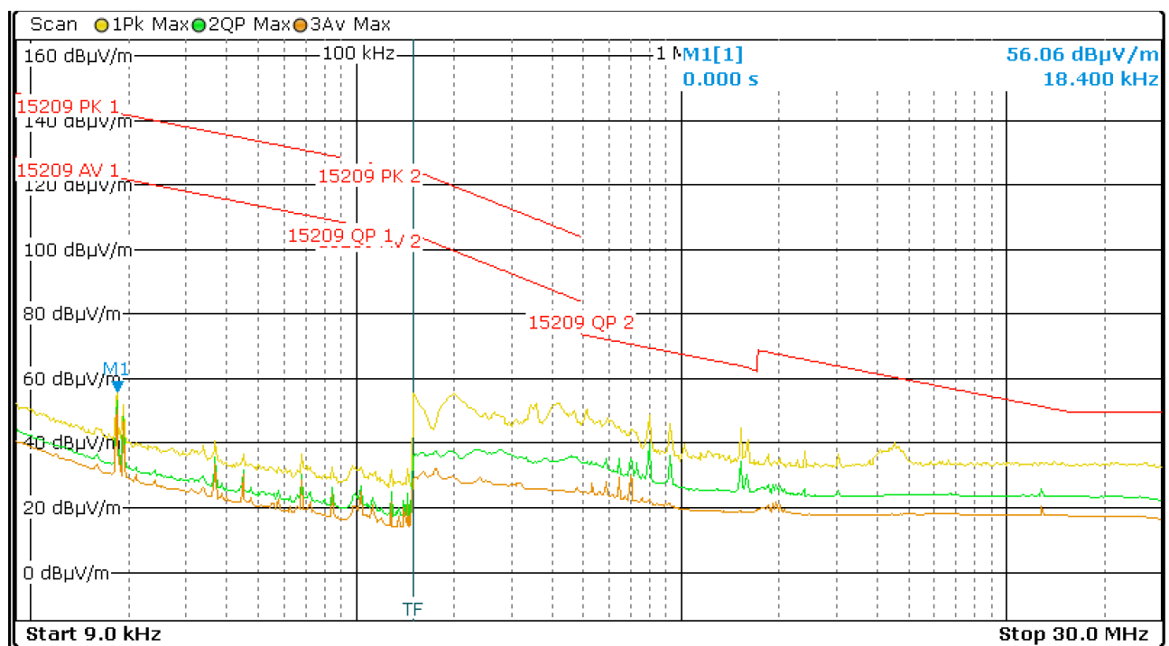
Figure 30: Chart of emissions test below 30 MHz on lowest channel, EUT position X, antenna parallel
