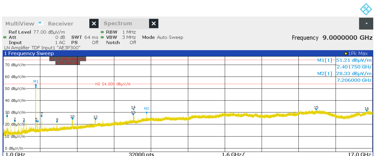
Figure 32: Chart of radiated emissions pre-measurement from 1 GHz to 17 GHz on lowest channel, EUT position Y, antenna polarization vertical
