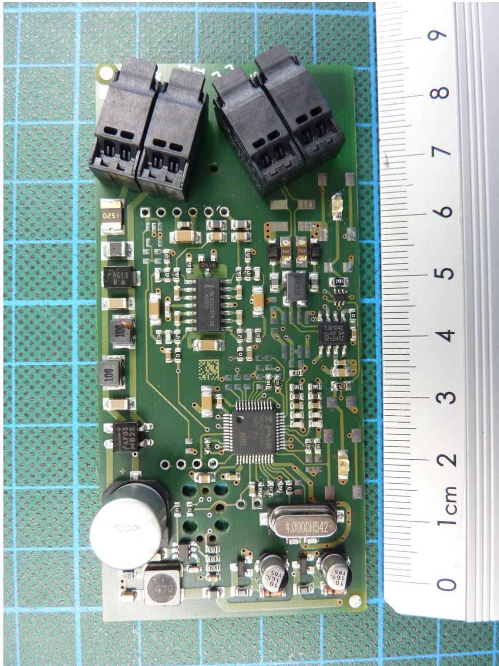
160532_9.jpg: MWD BPC-HU, PCB, top view, radar module removed
