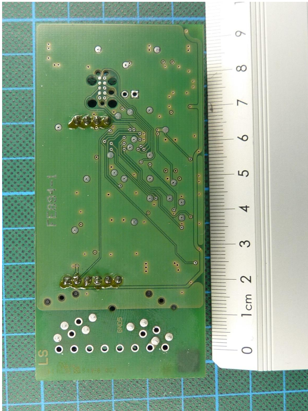
160532_8.jpg: MWD BPC-HU, PCB, bottom view
