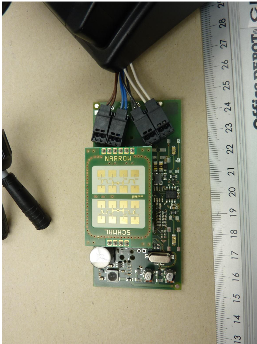
160532_5.jpg: MWD BPC-HU, internal view 2
