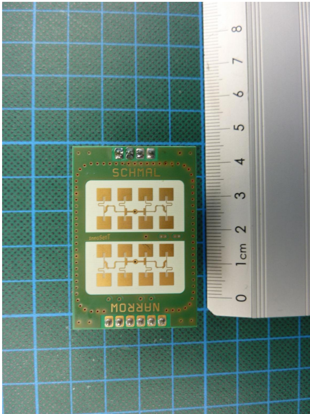
160532_11.jpg: MWD BPC-HU, radar module, top view
