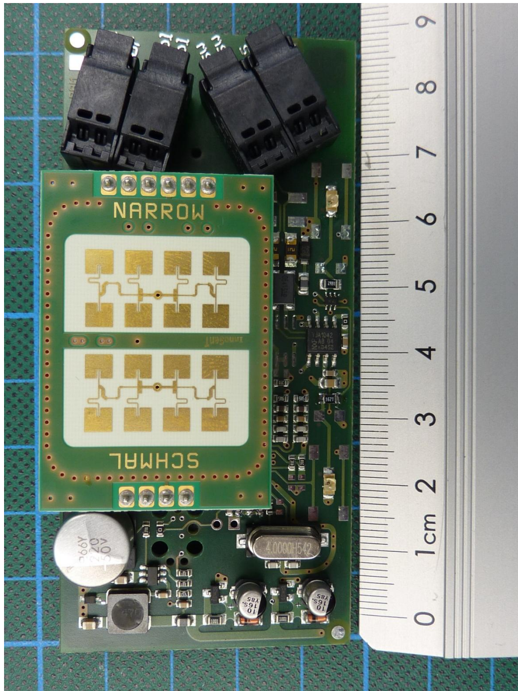
160532_7.jpg: MWD BPC-HU, PCB, top view
