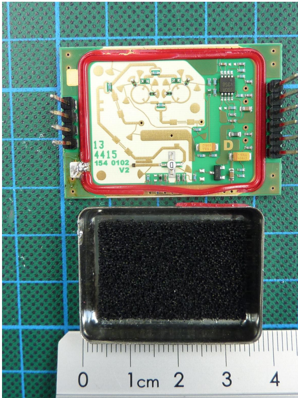
160532_12.jpg: MWD BPC-HU, radar module, shielding removed
