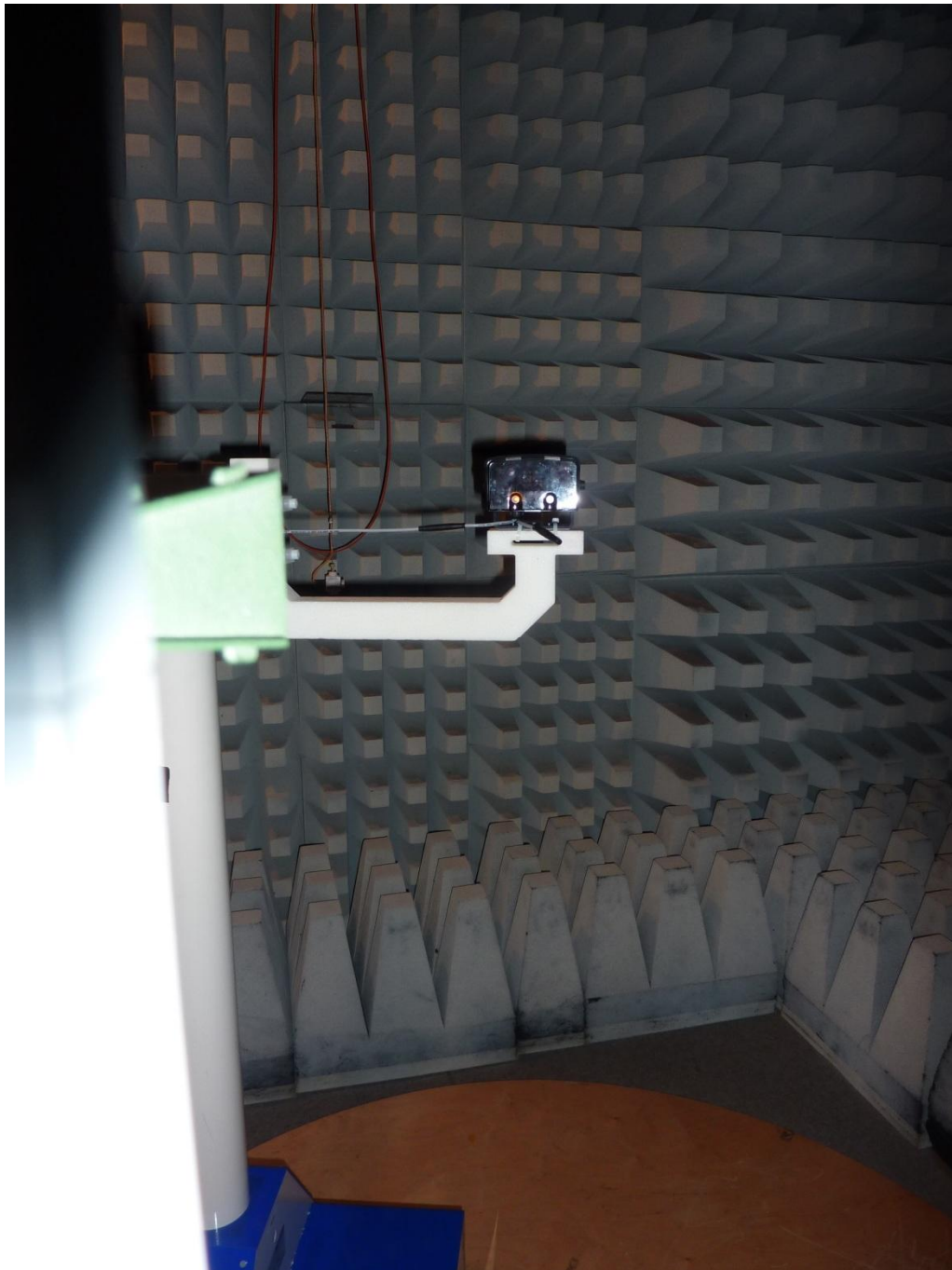
160532_106.jpg: MWD BPC-HU, test setup fully anechoic chamber >1 GHz
