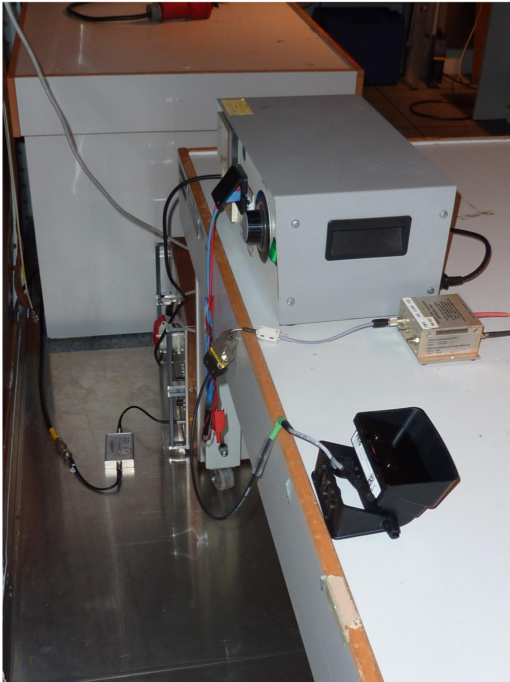
160532_112.jpg: MWD BPC-HU (AC supplied), test setup shielded room
