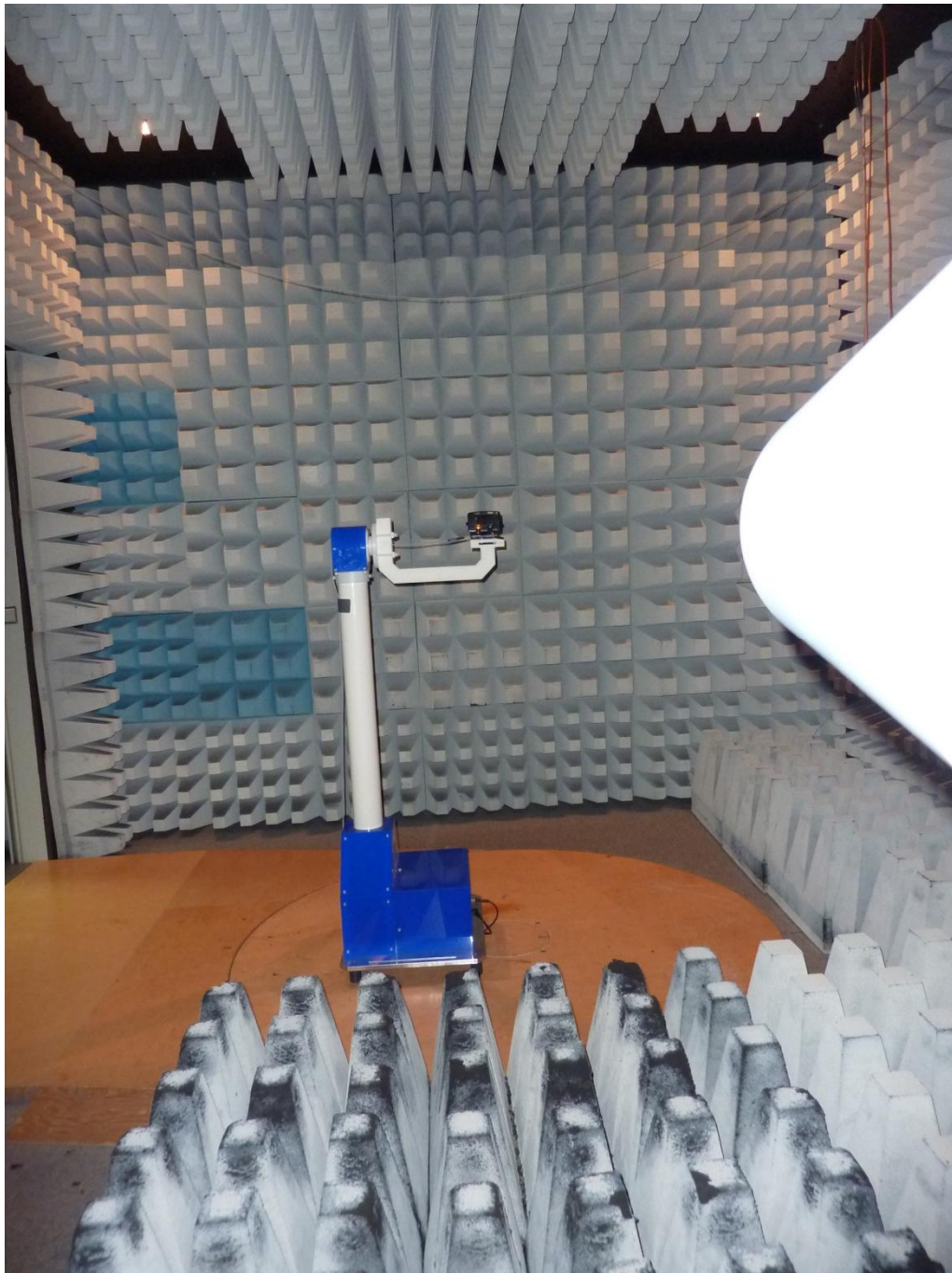
160532_105.jpg: MWD BPC-HU, test setup fully anechoic chamber >1 GHz
