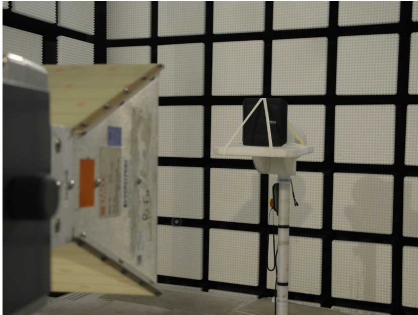
EUT with internal antenna
