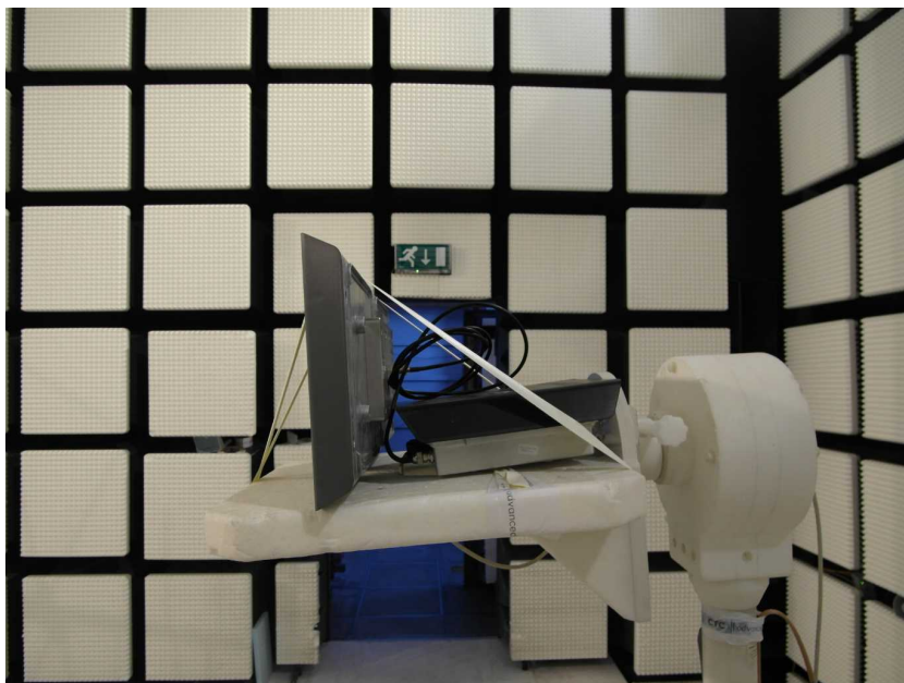
EUT with external antenna ID Ant.U580/290-FCC
