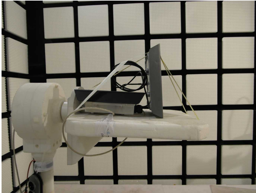
EUT with external antenna ID Ant.U290/290-FCC
