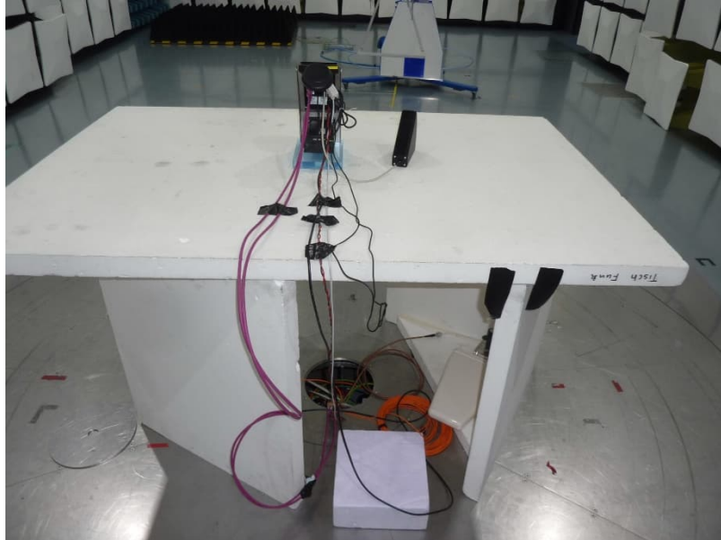
Test setup EUT, view 1
