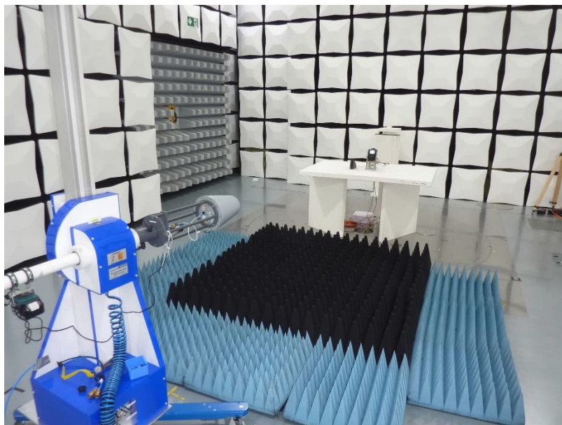
Test setup SAC Measurement of E-Field 1 GHz – 18 GHz
