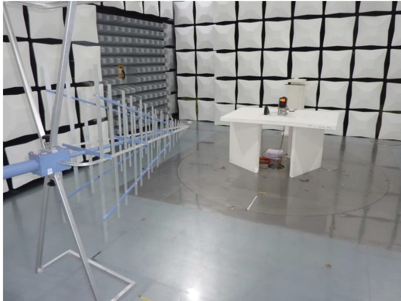
Test setup SAC Measurement of E-Field 30 MHz – 1000 MHz
