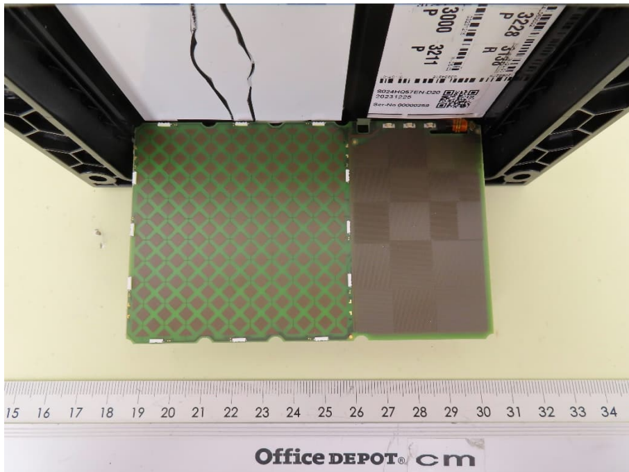
PCB PAY cVEND Touch – Sensor, top view
