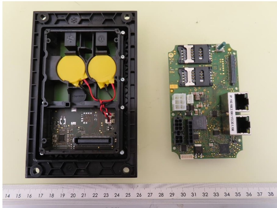
EUT, PCB PAY cVEND Touch – Interface removed
