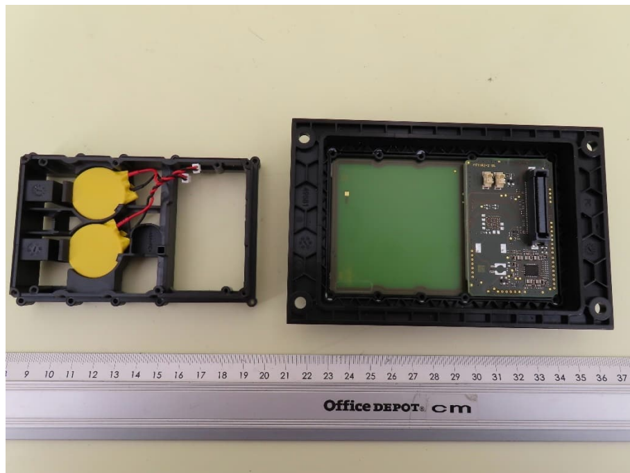
EUT, battery holder removed
