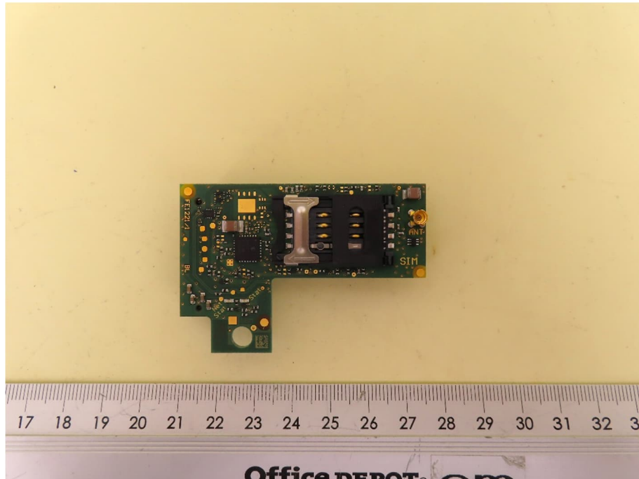
PCB PAY cVEND EXT-LTE-A, bottom view
