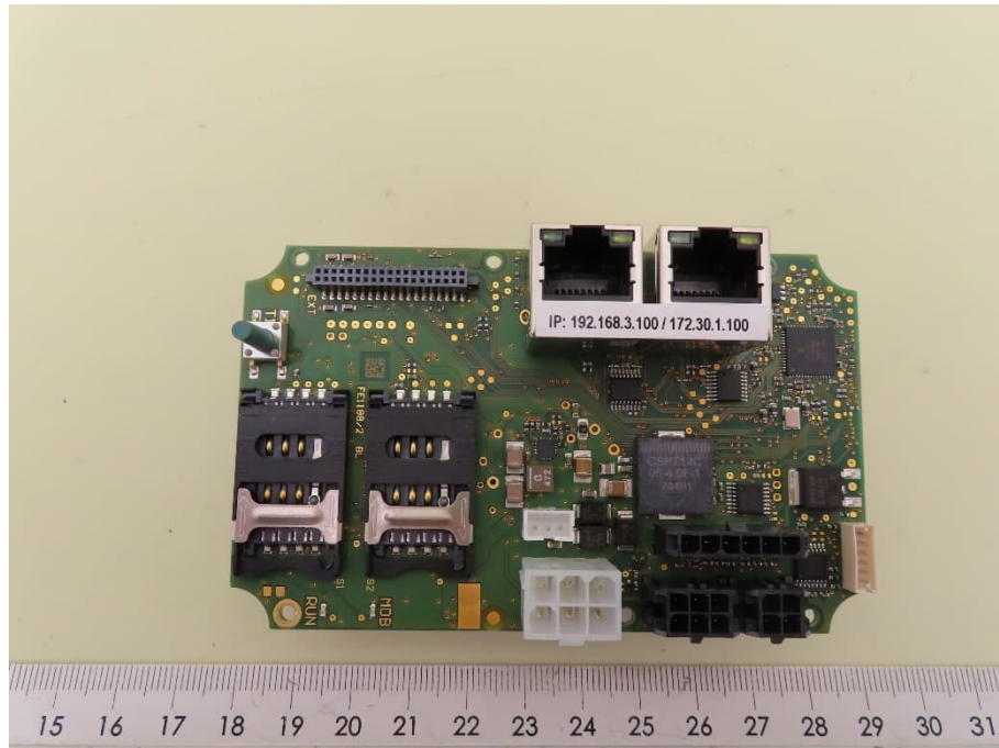
PCB PAY cVEND Touch – Interface, bottom view
