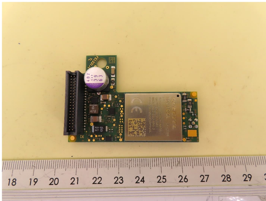
PCB PAY cVEND EXT-LTE-A, top view
