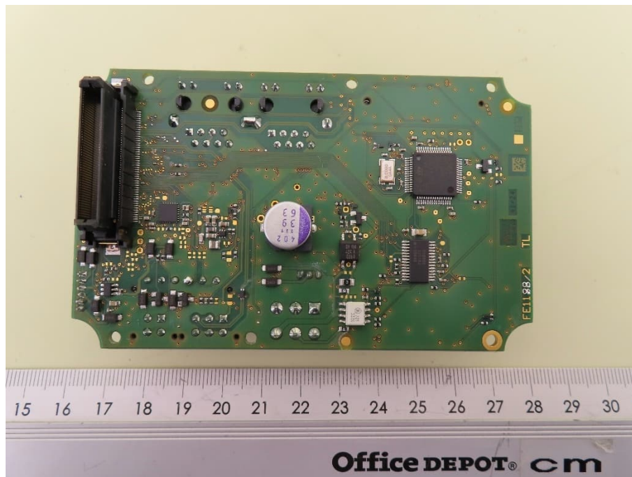
PCB PAY cVEND Touch – Interface, top view
