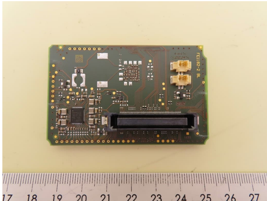
PCB PAY cVEND Touch – Core, bottom view
