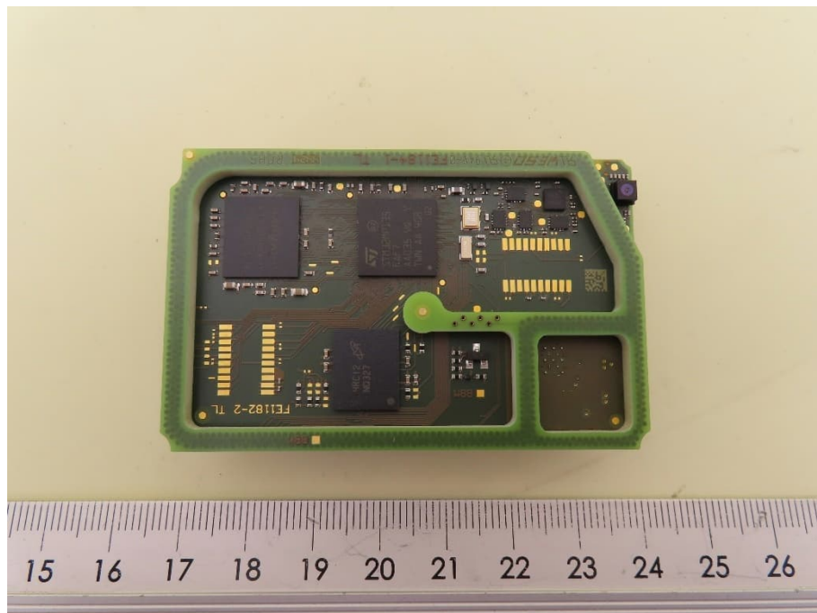
PCB PAY cVEND Touch – Core, top view
