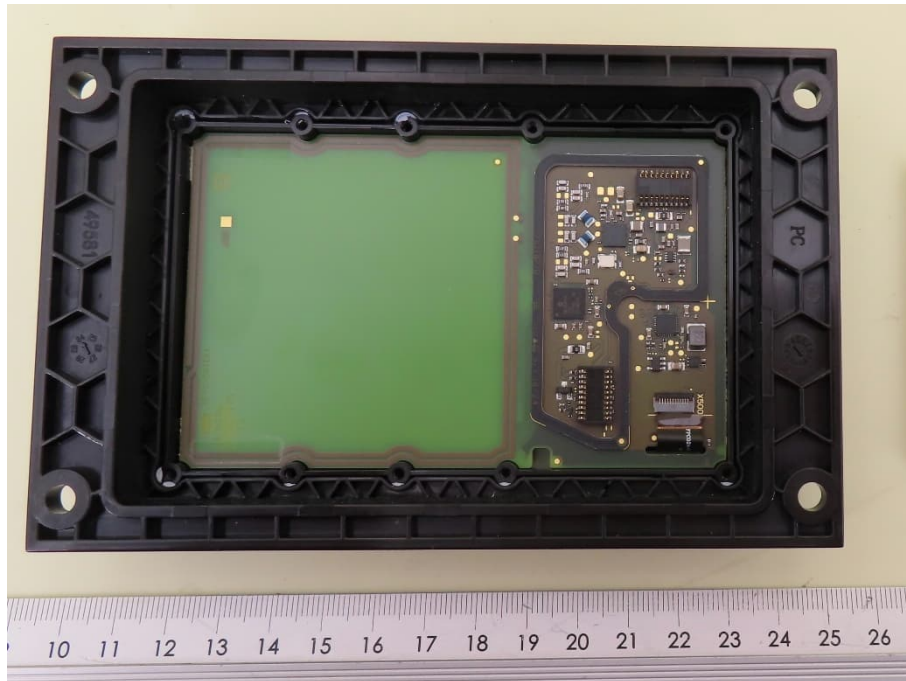
PCB PAY cVEND Touch – Sensor, bottom view
