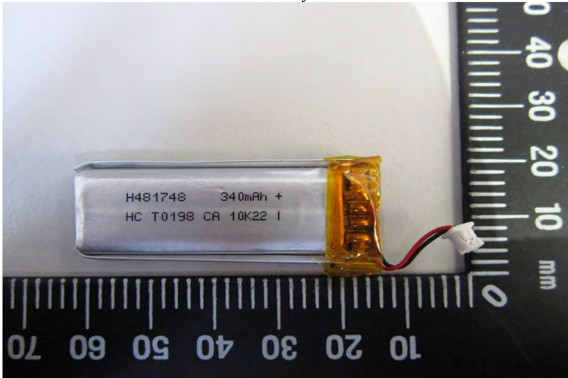
Battery
