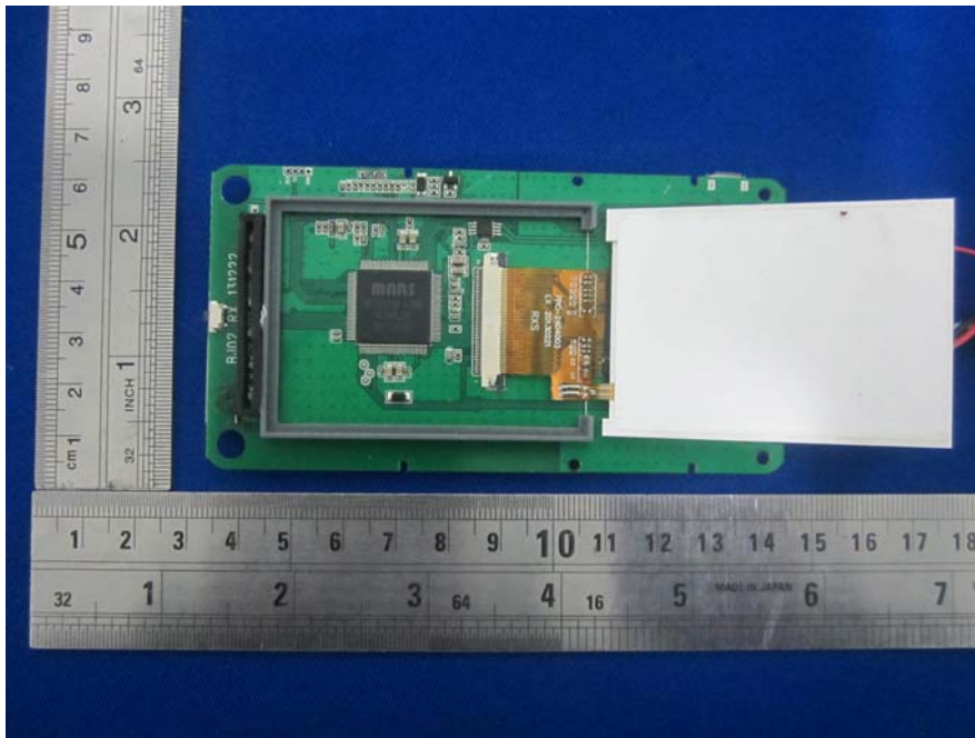
EUT- LCD Uncover View
