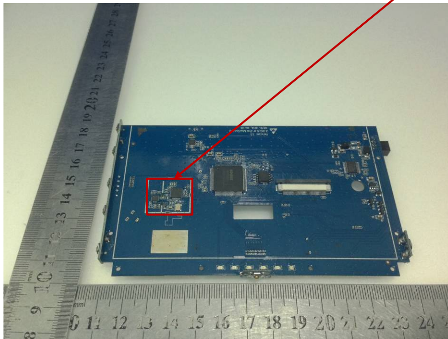
Wireless Module
