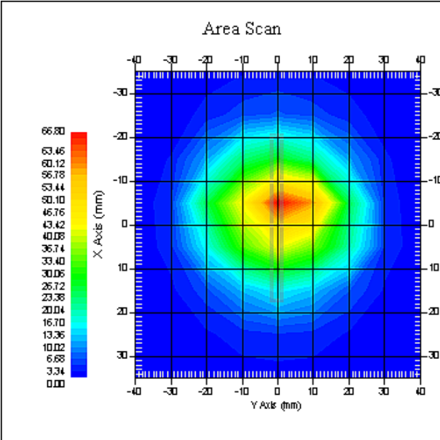
2450 MHz System Body Validation
