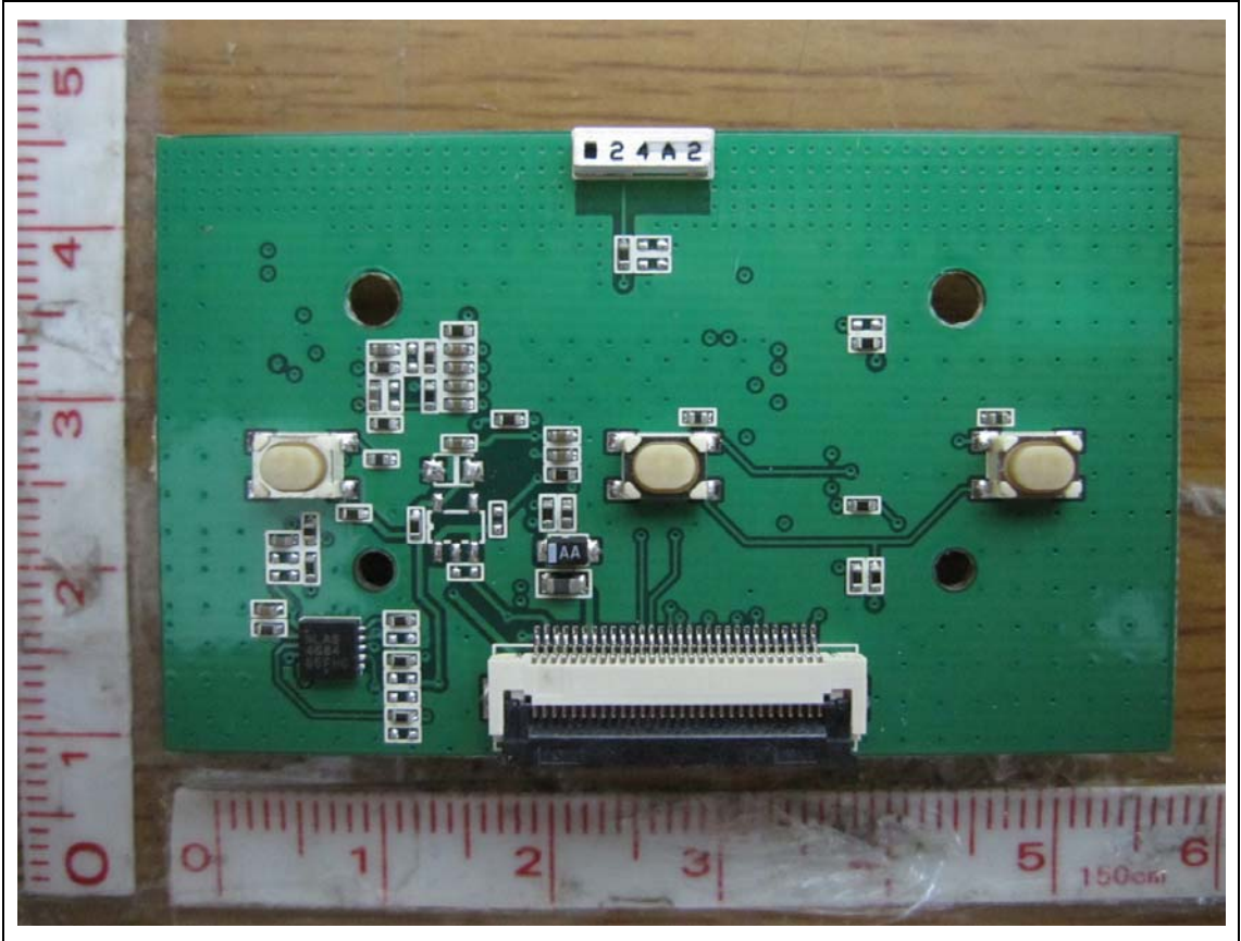
BT Module Board - Rear
